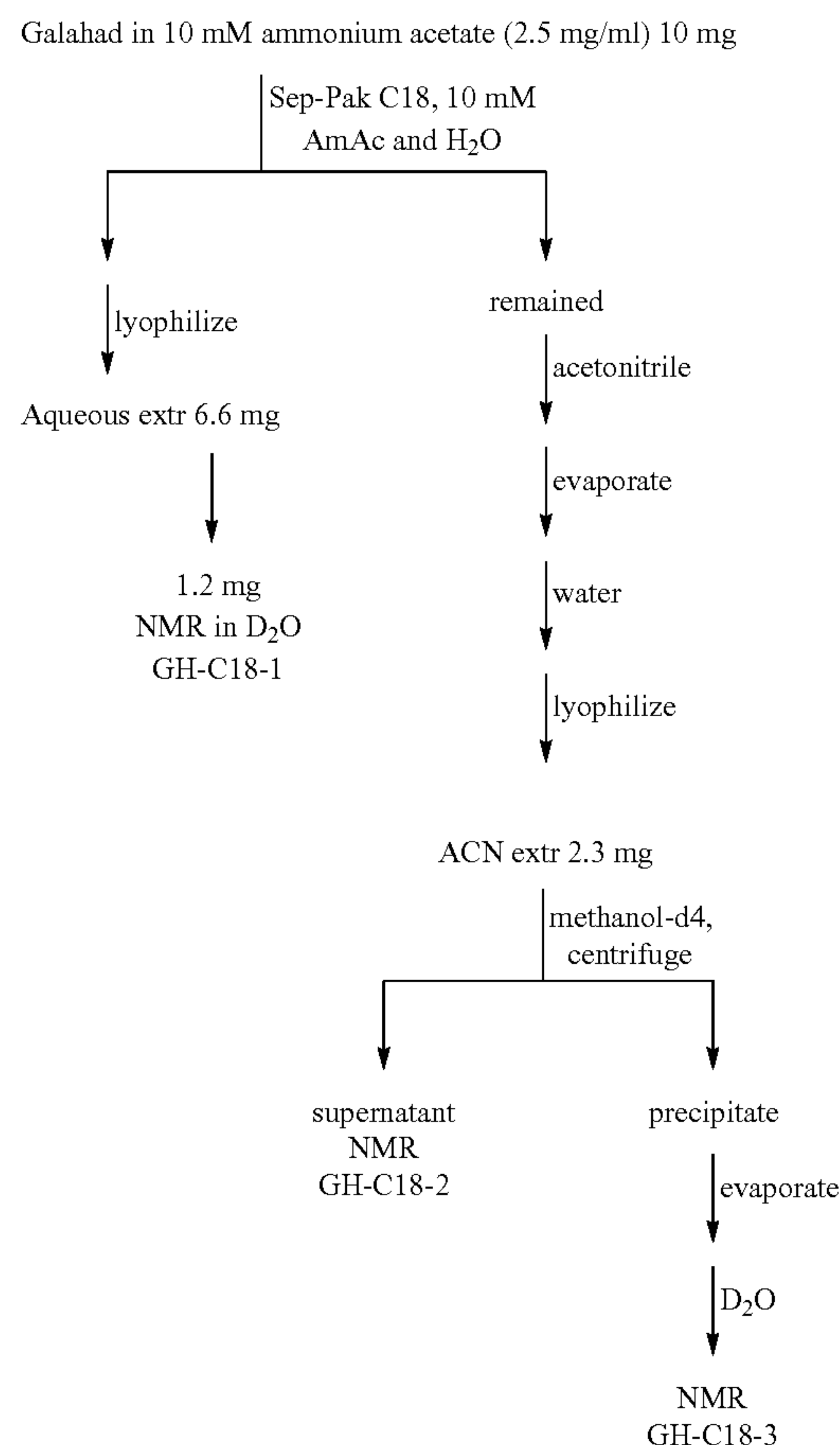
Scheme 1: Solid phase extraction of Galahad with Sep-Pak C18
