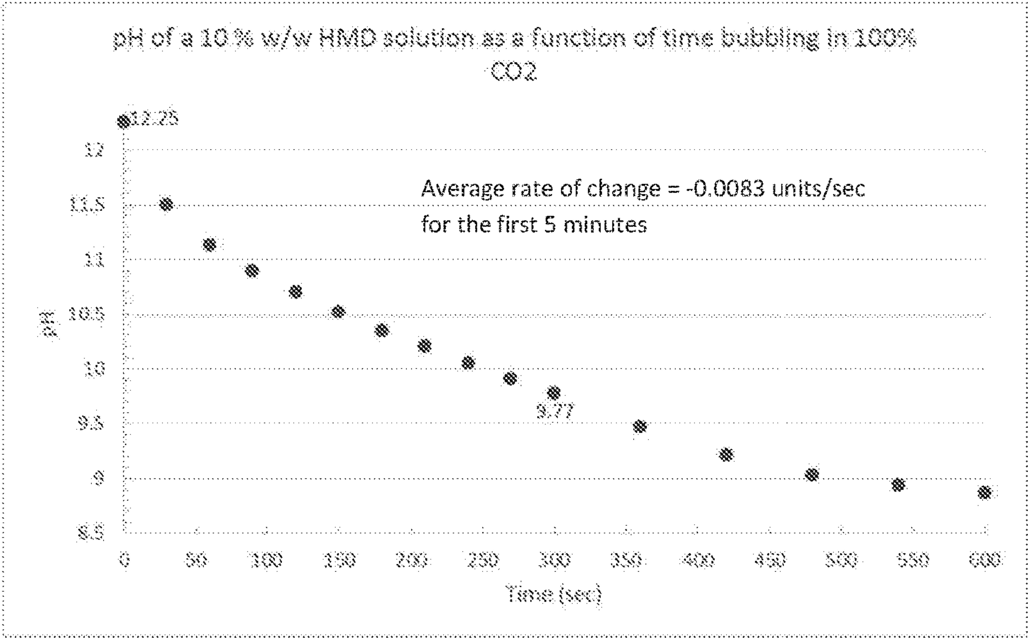
Graph 1-2: pH as a function of time bubbling in CO 2 first 10 minutes.
