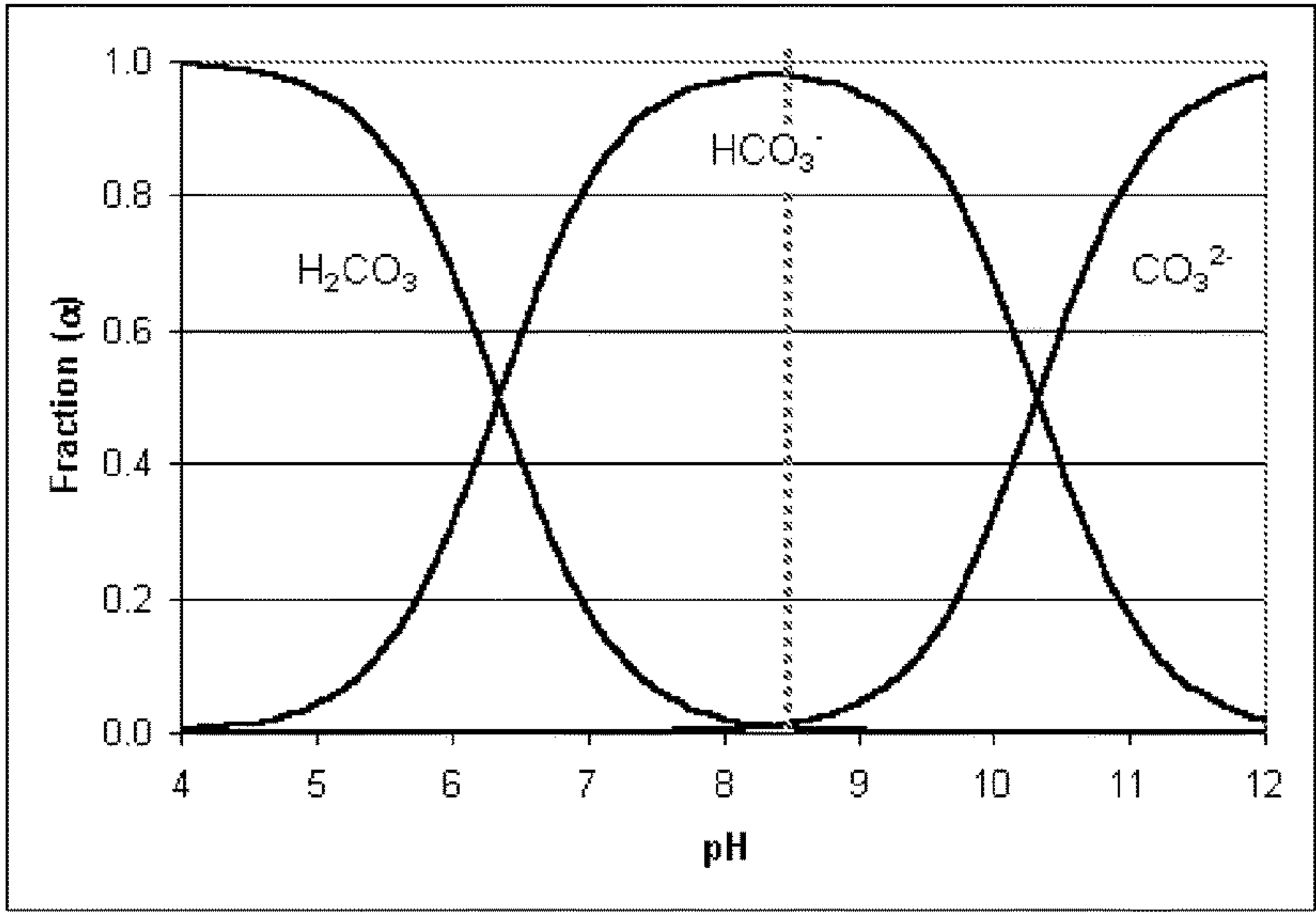
Graph 2-3: Carbonate species as a function of pH
