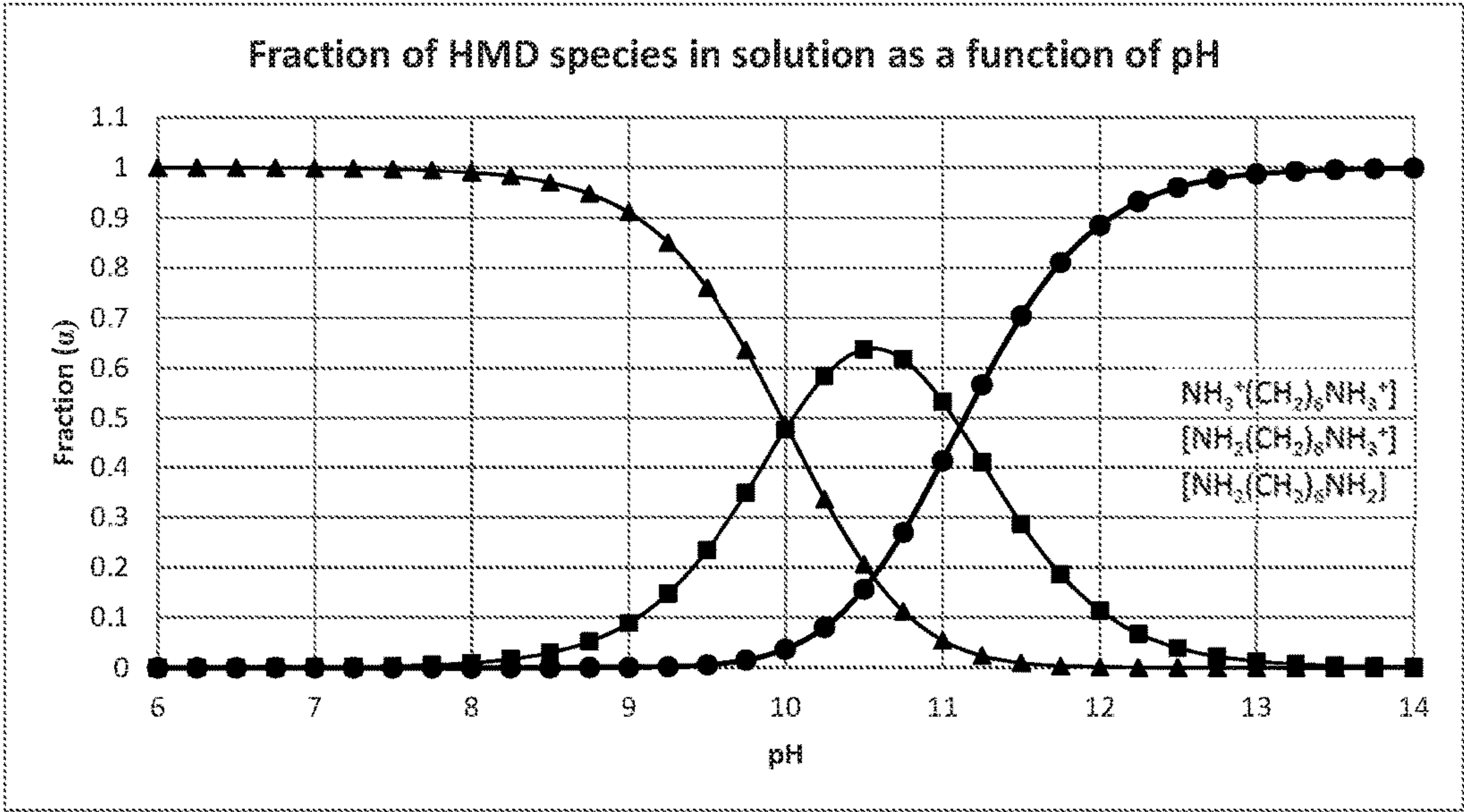
Graph 2-2: Concentration of HMD species as a function of pH
