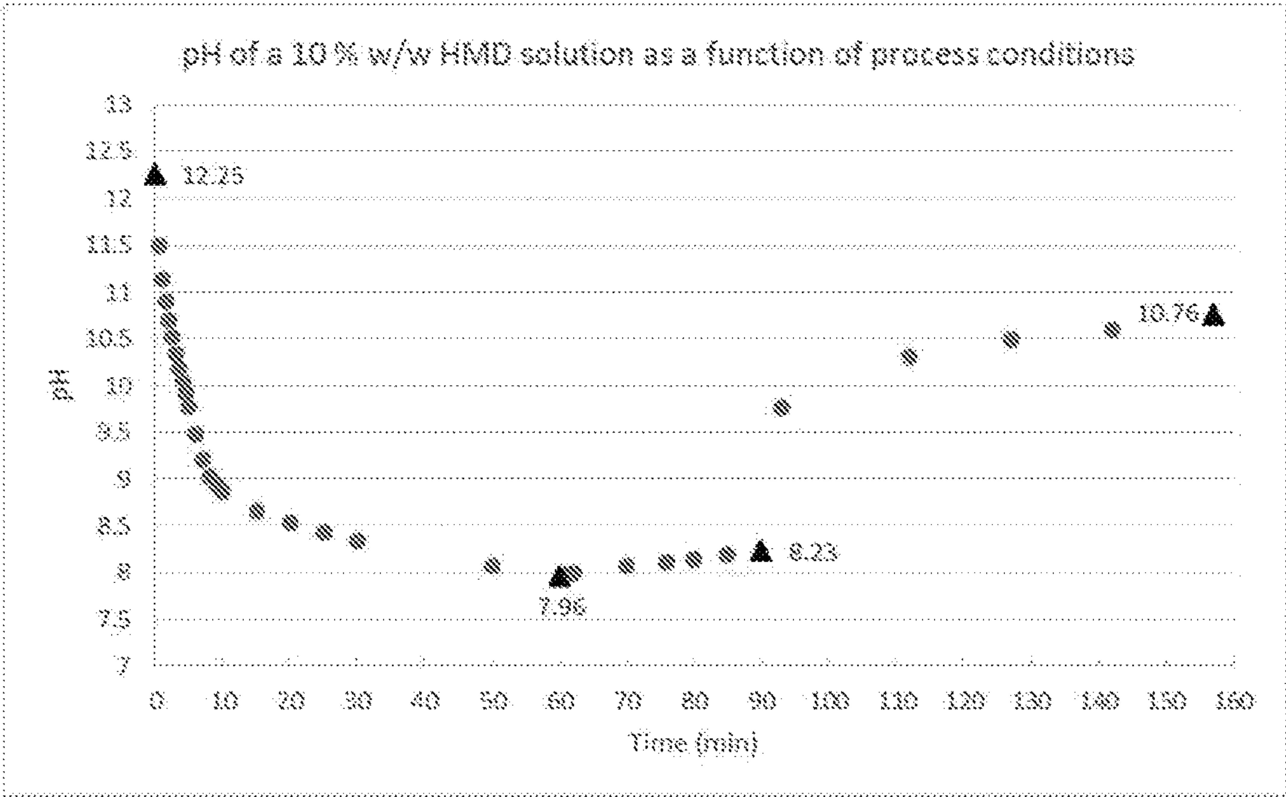
Graph 1-3: pH as a function of process conditions, refer to Table 1-1 above.
