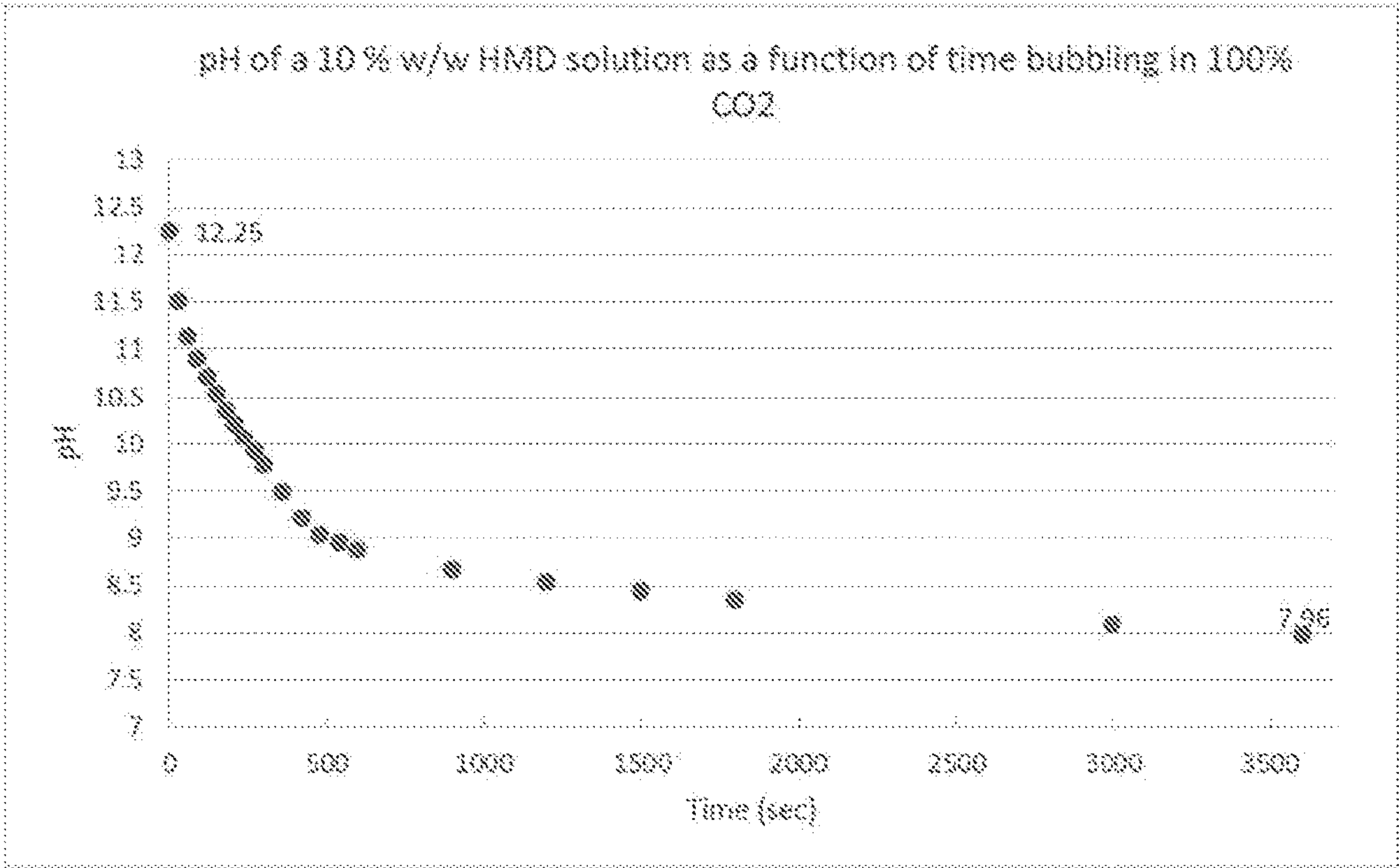
Graph 1-1: pH as a function of time bubbling in CO 2 over 60 minutes.
