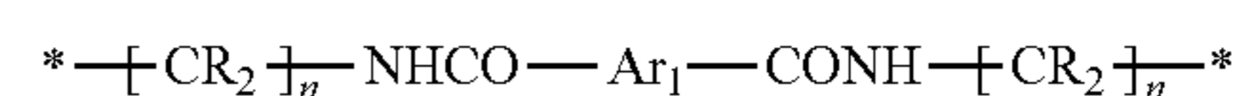
[Chemical Formula 1-1]
