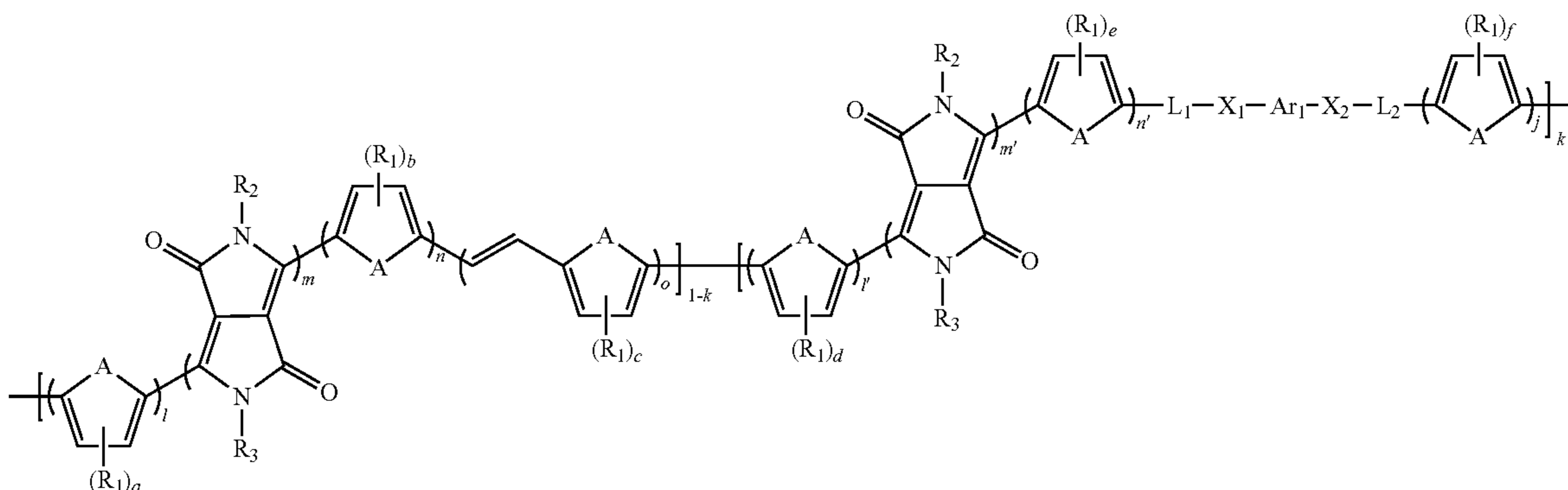
[Chemical Formula 3]
