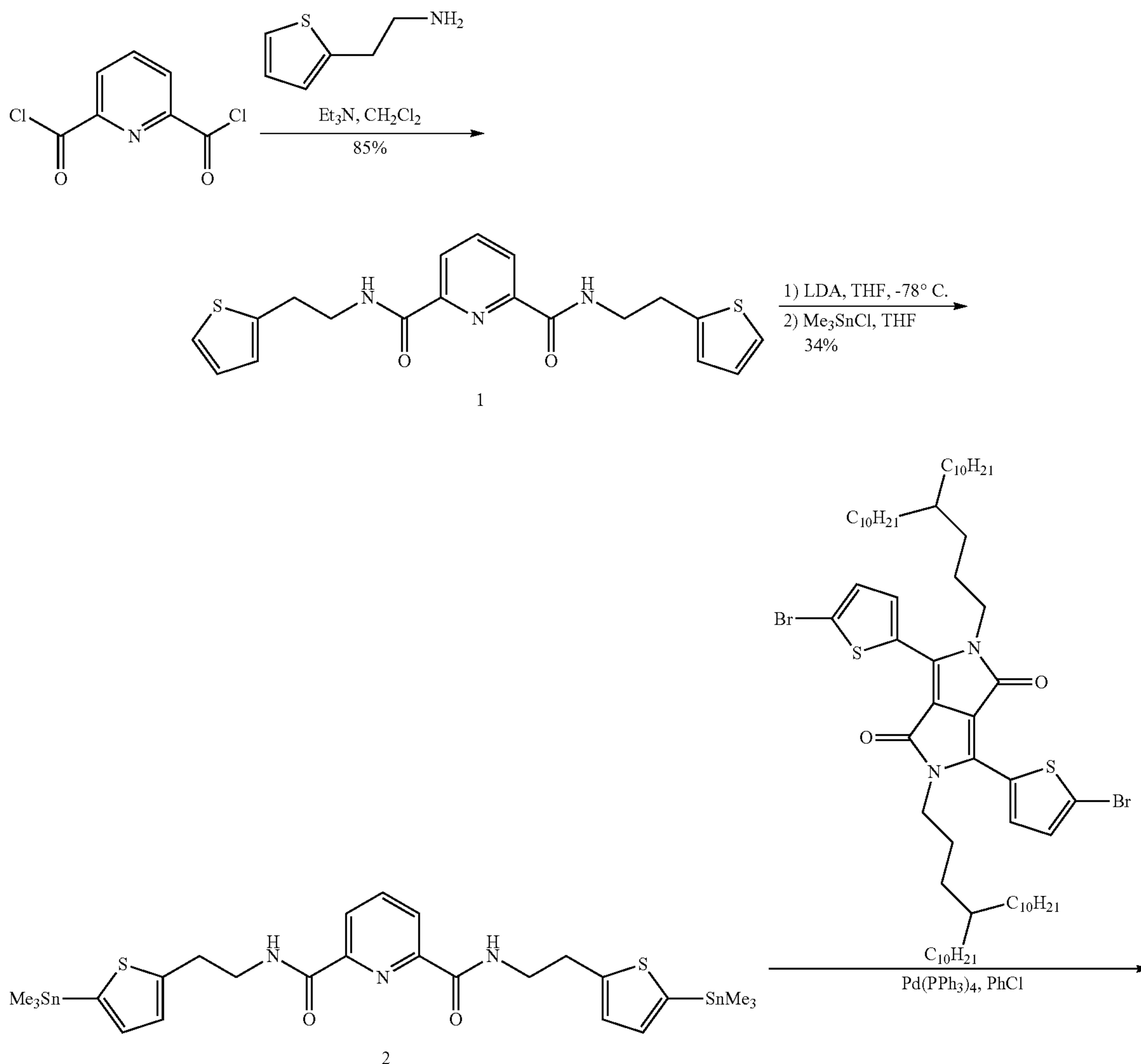
Reaction Scheme 1. Synthetic route for Second Monomer 2 and Model Compound M1
