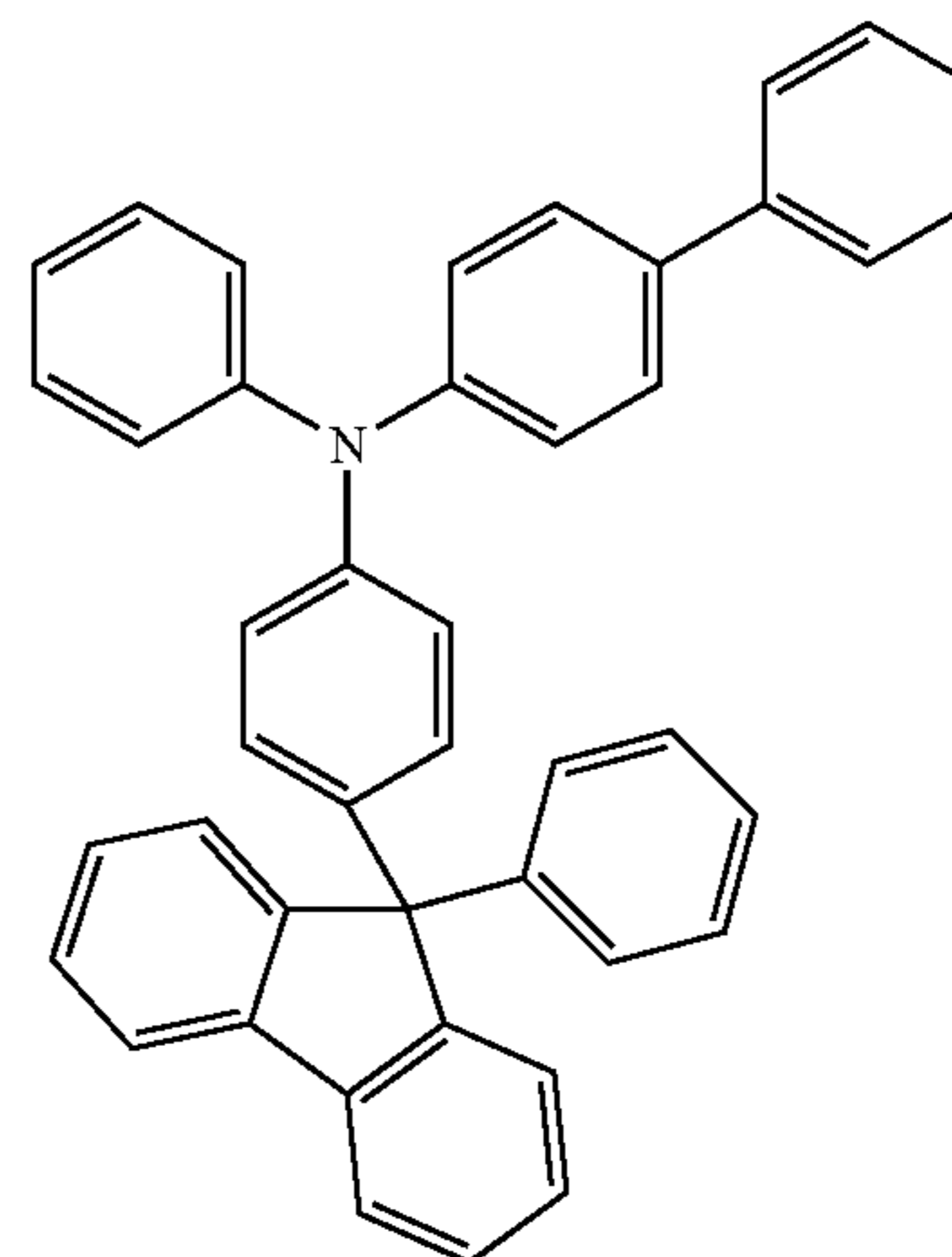
BPAFLP
