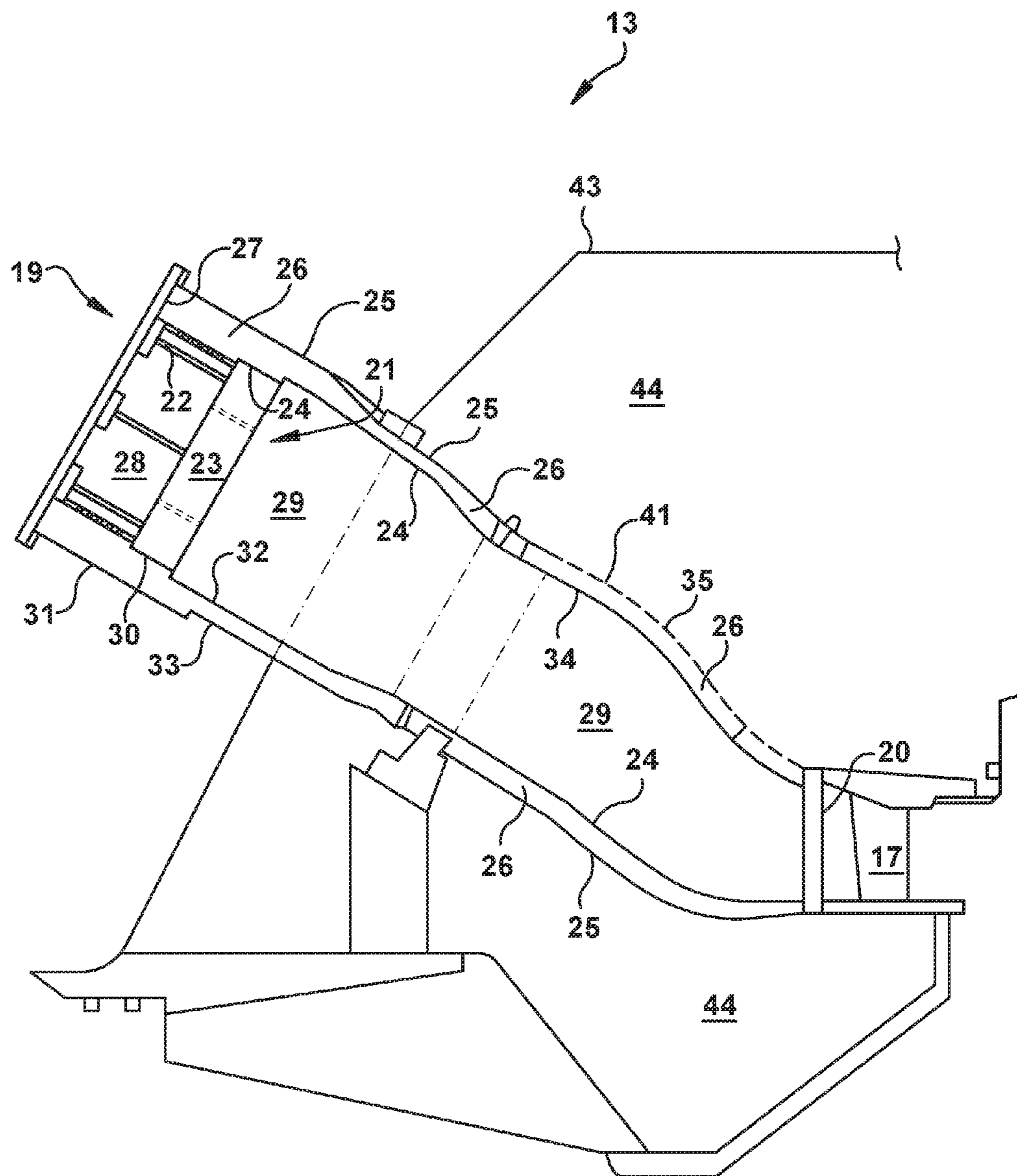
Figure 2 (Prior Art)
