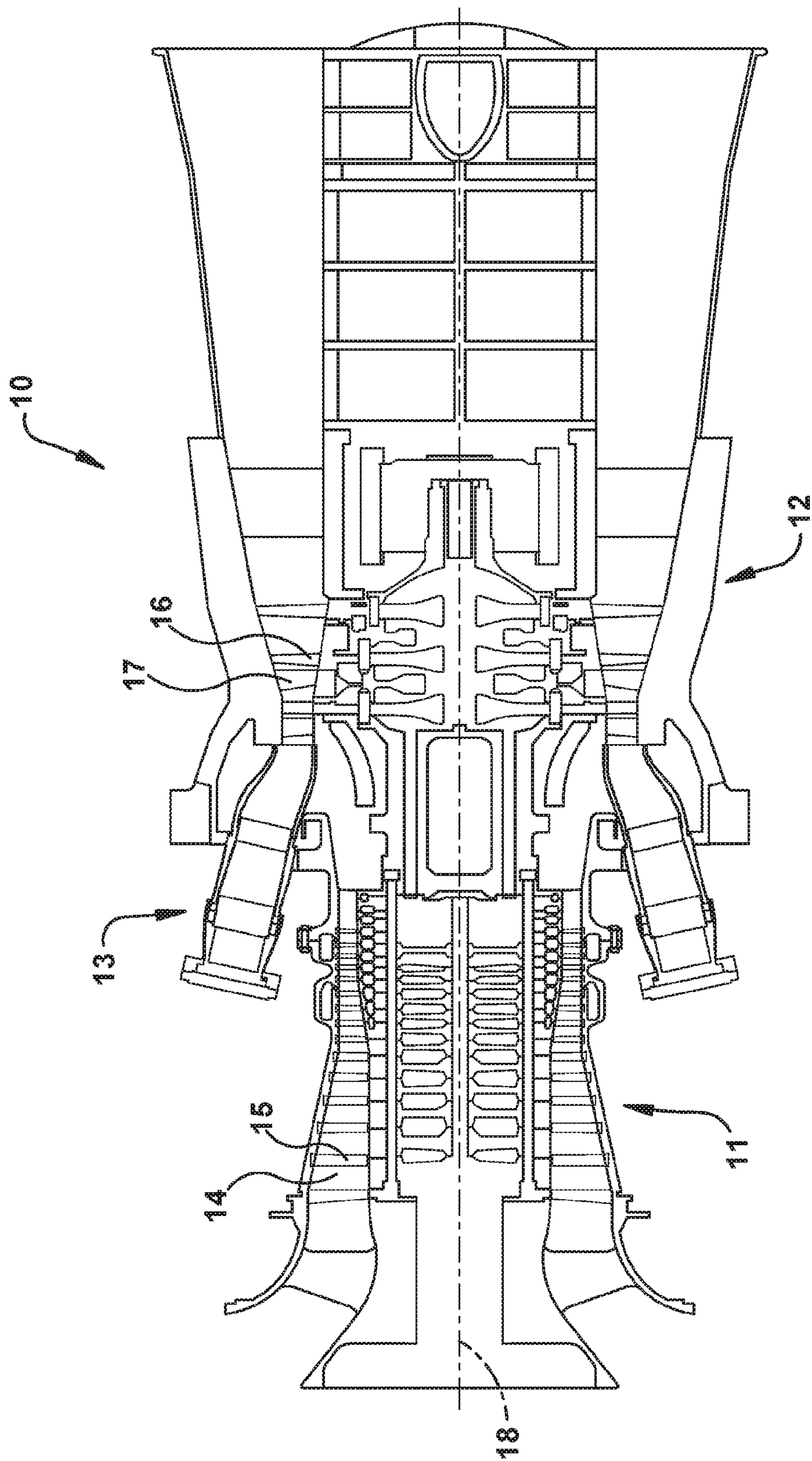
Figure 1 (Prior Art)
