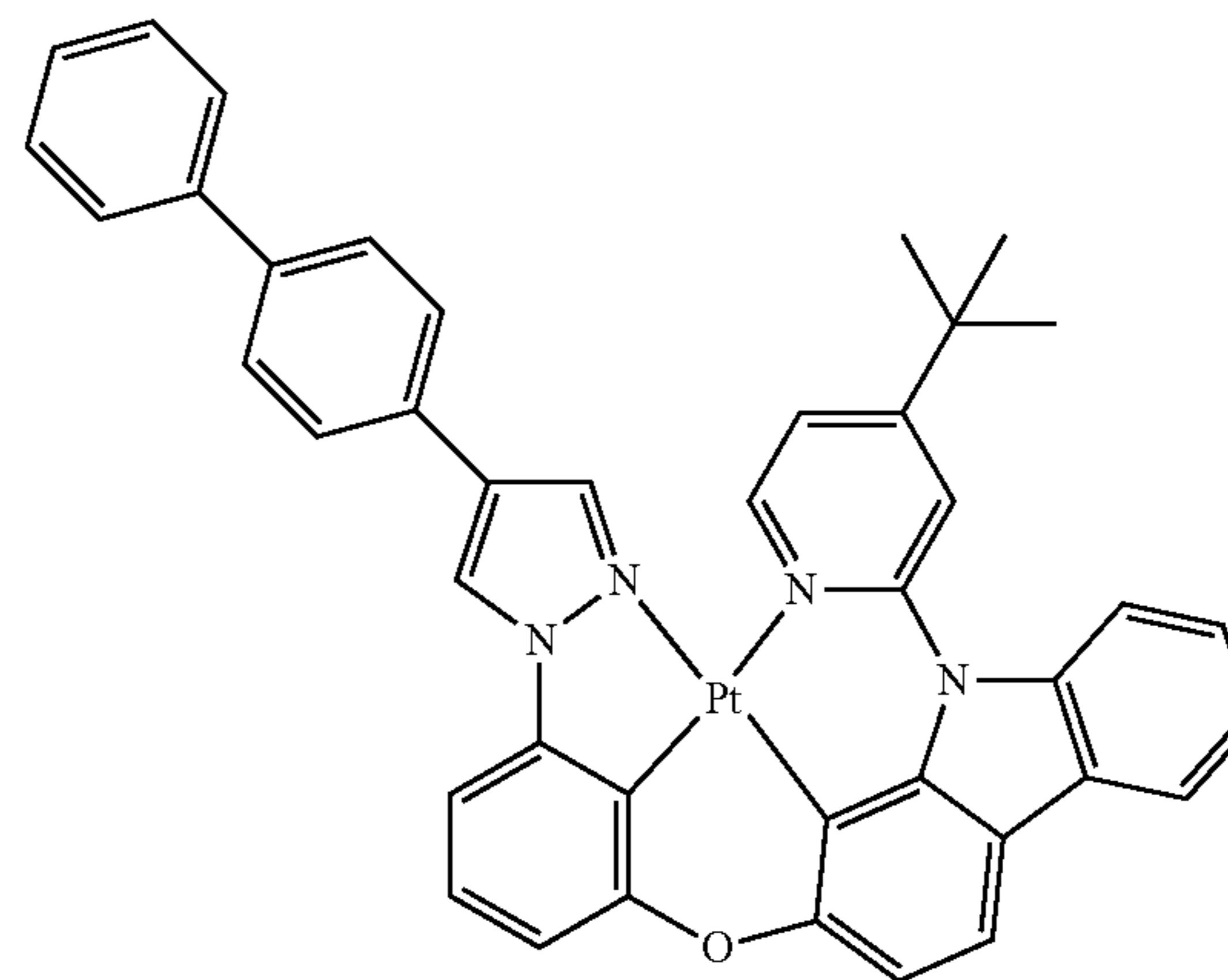
PtON1a- t -Bu
