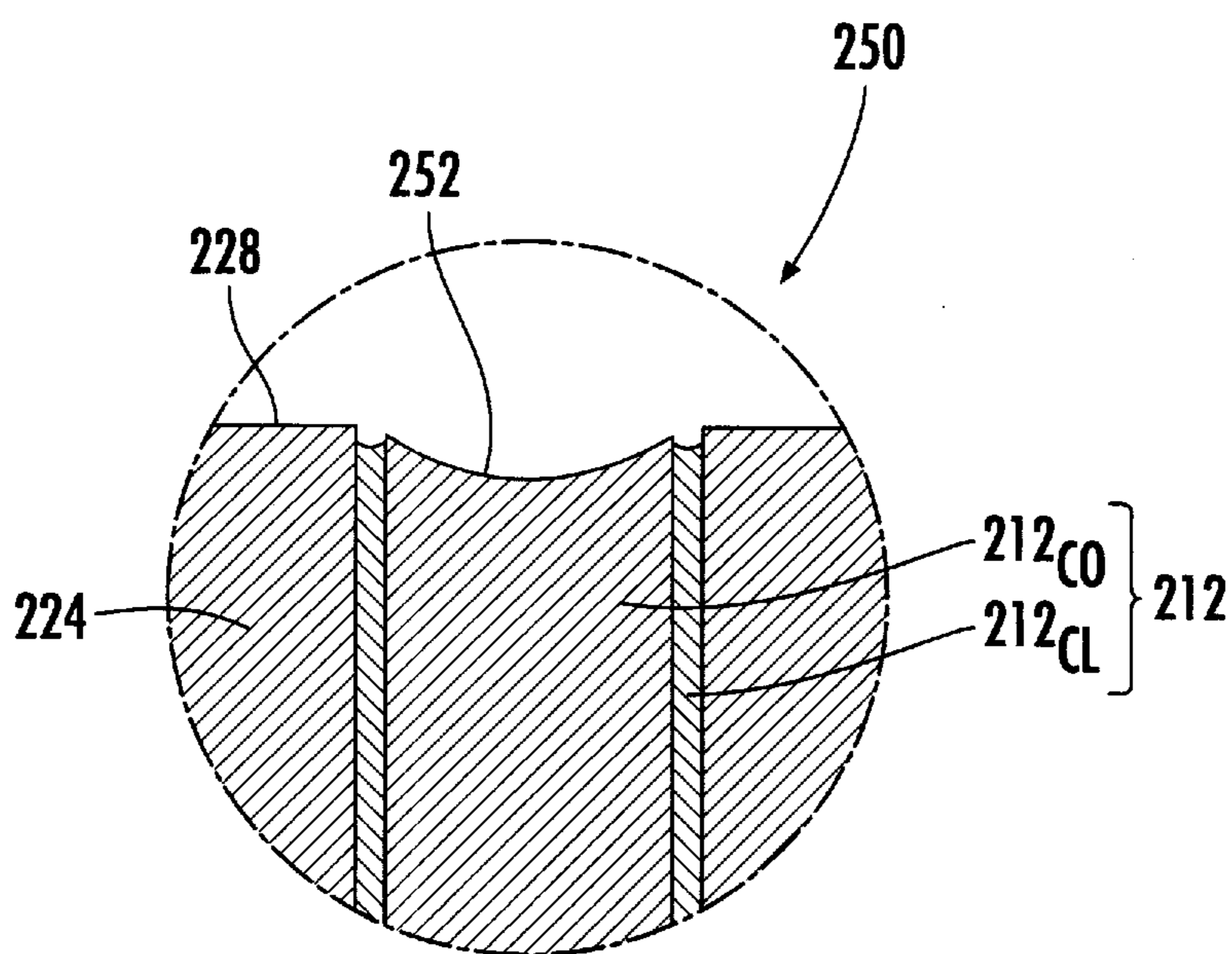
FIG. 21 (PRIOR ART)
