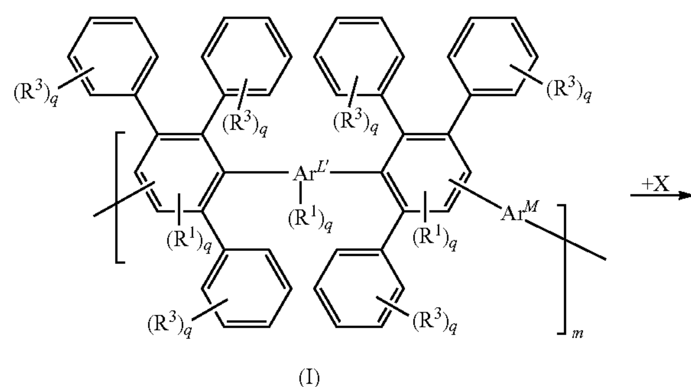
Scheme IIIa
