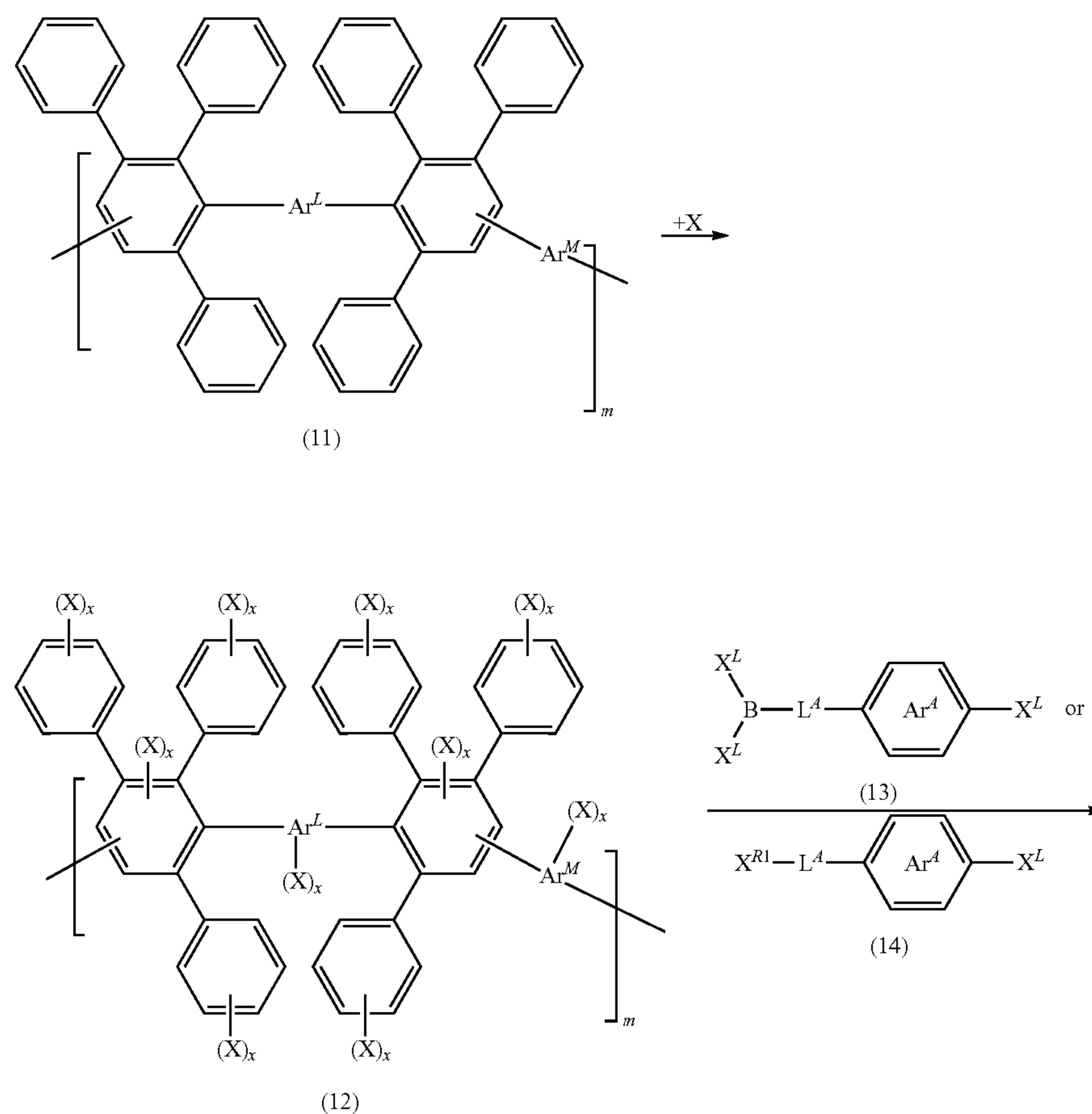
Scheme IIIb
