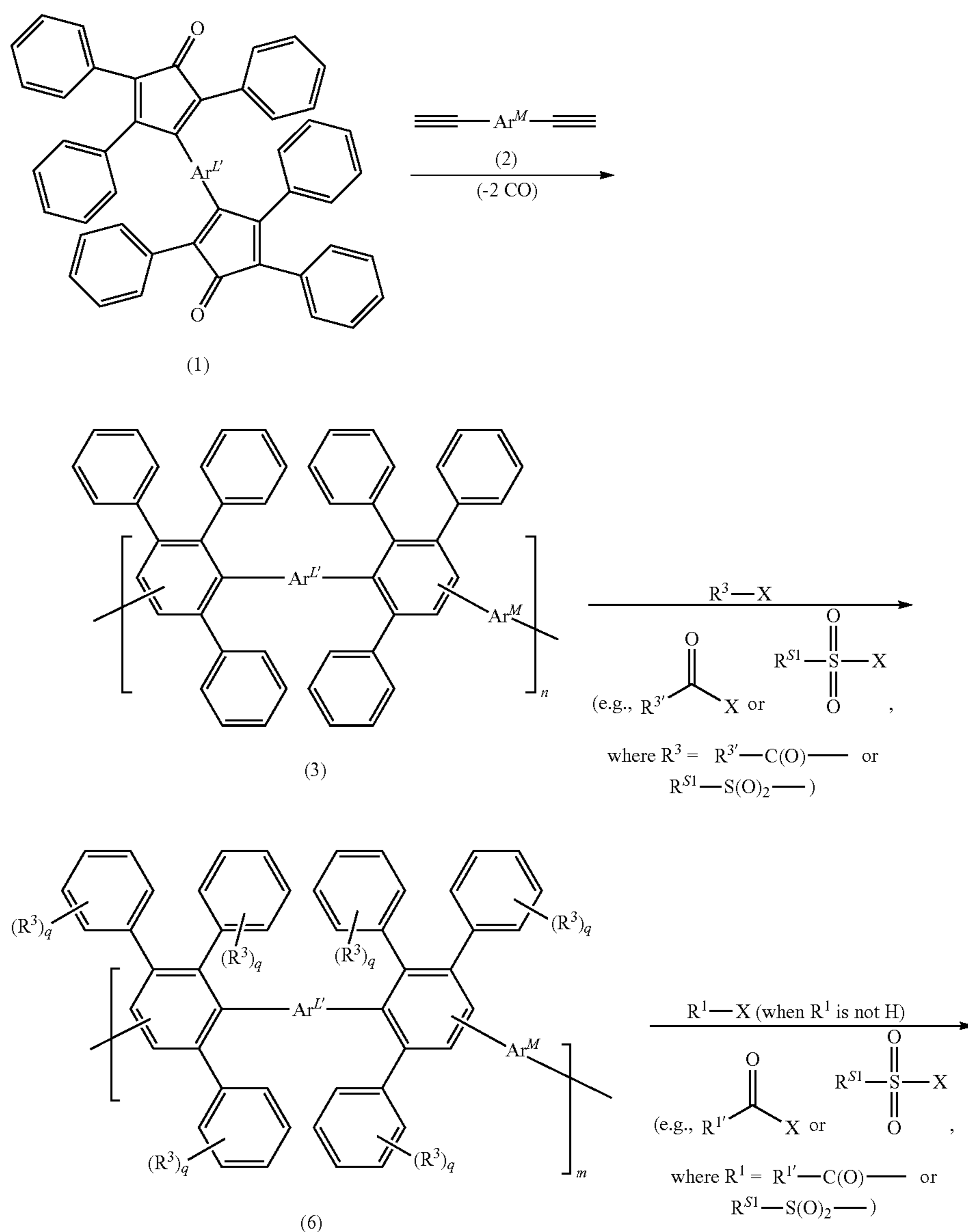
Scheme IIa
