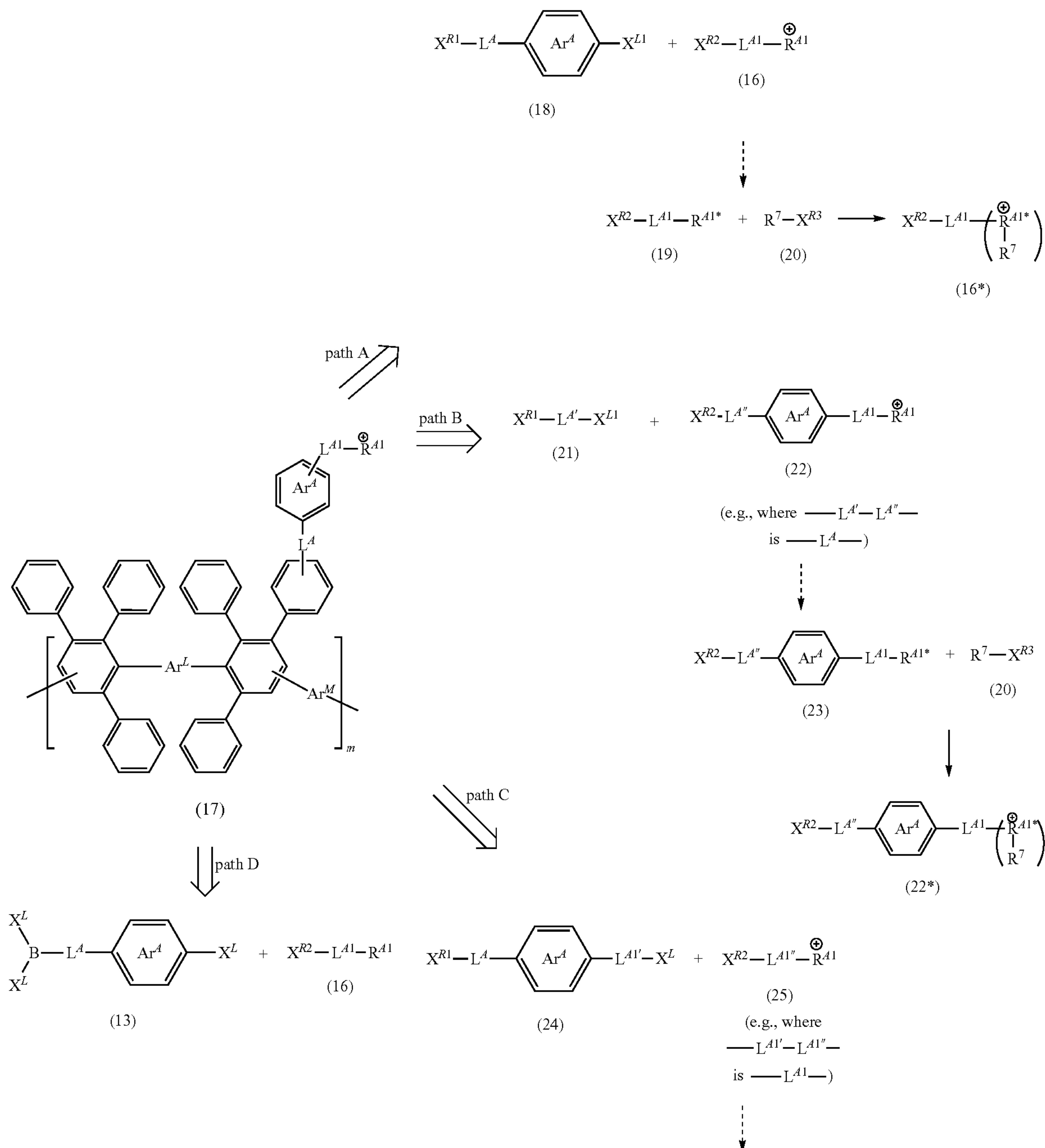
Scheme IV
