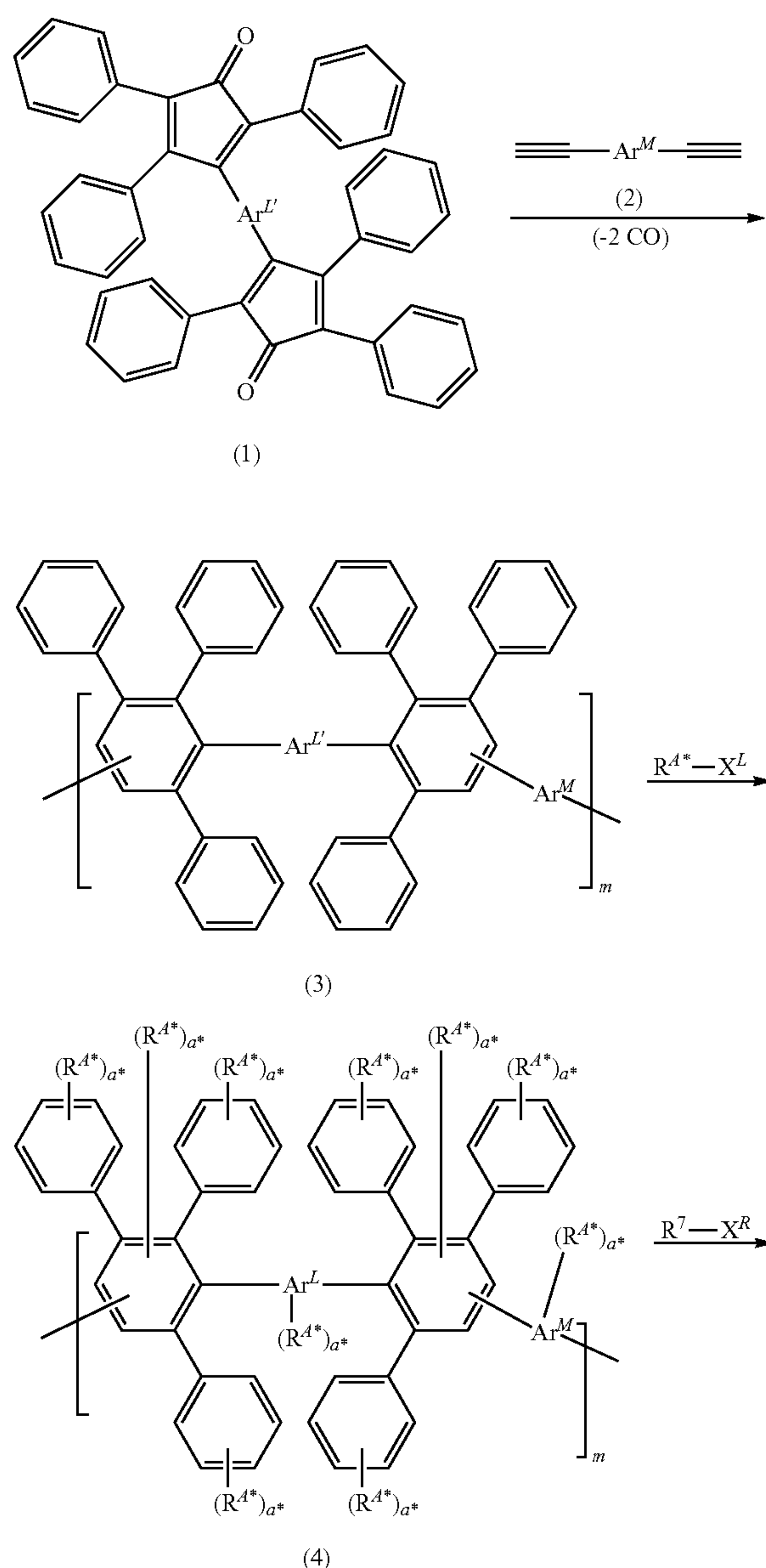
Scheme Ib
