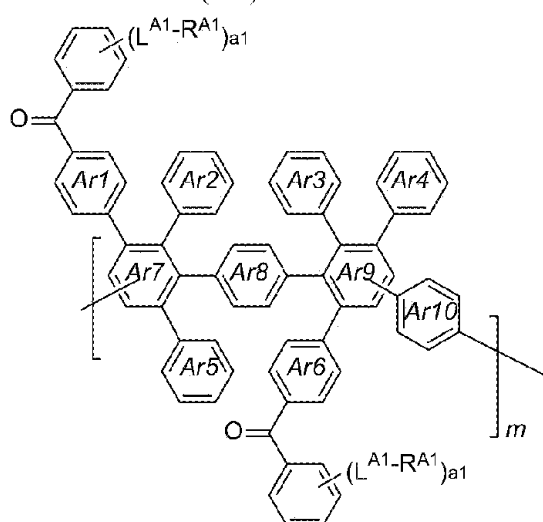
(II-7)
