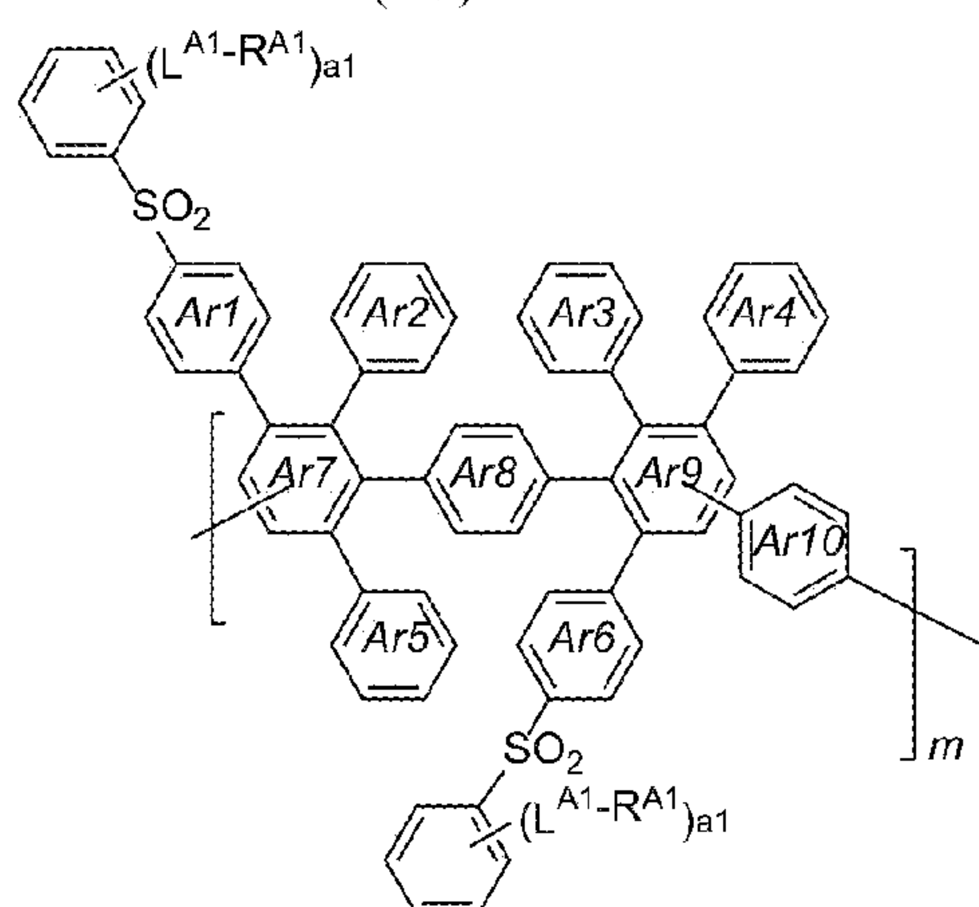
(II-8)
