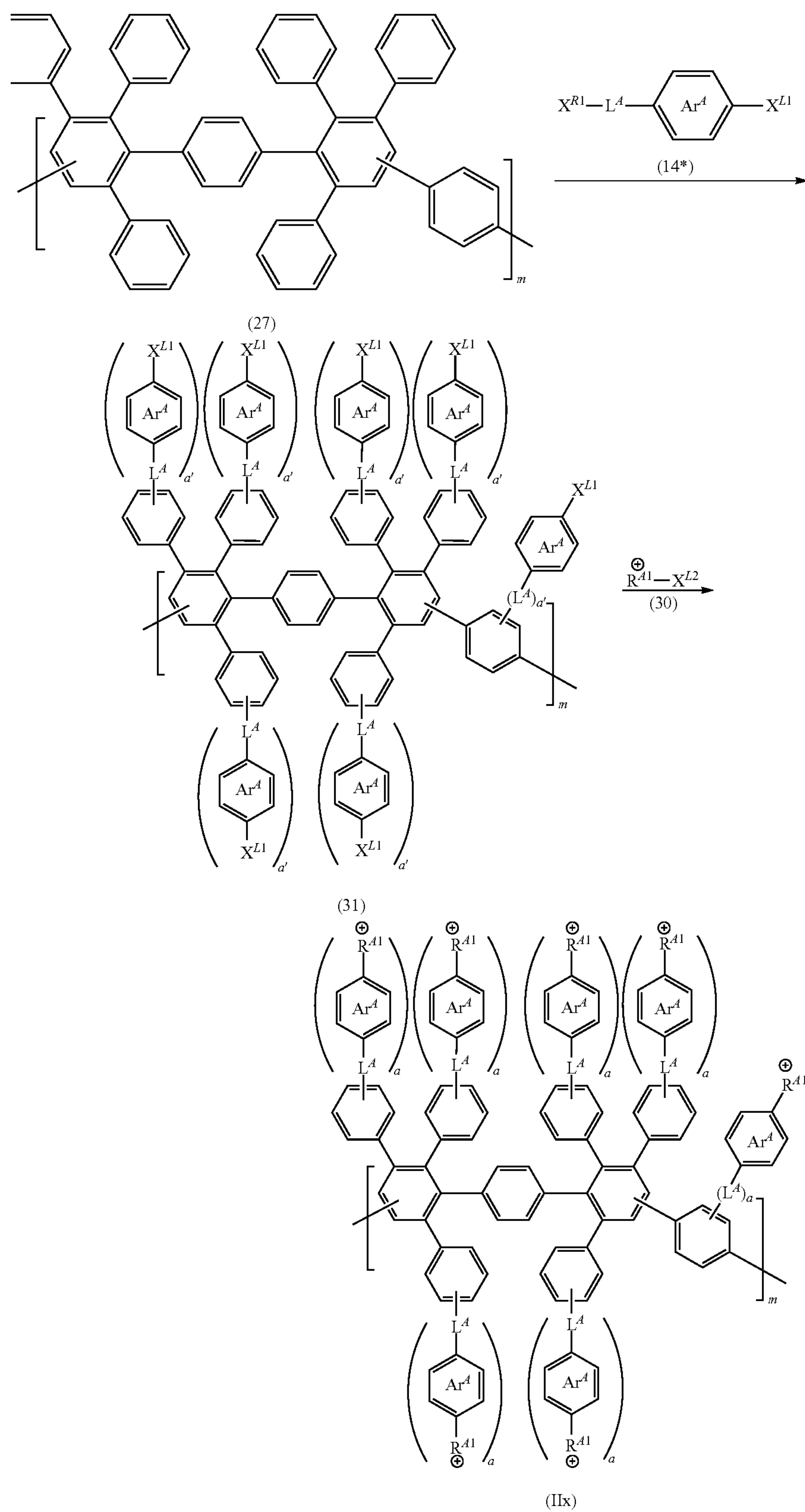
Scheme B
