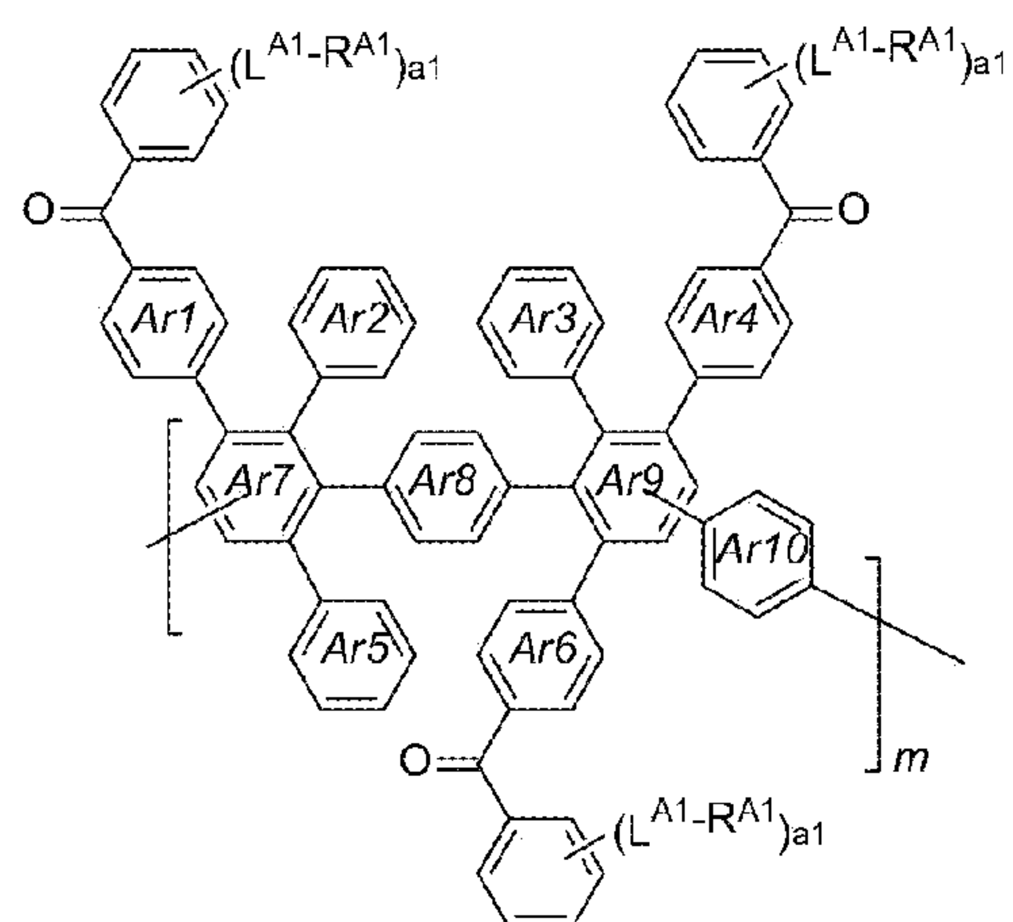
(II-5)
