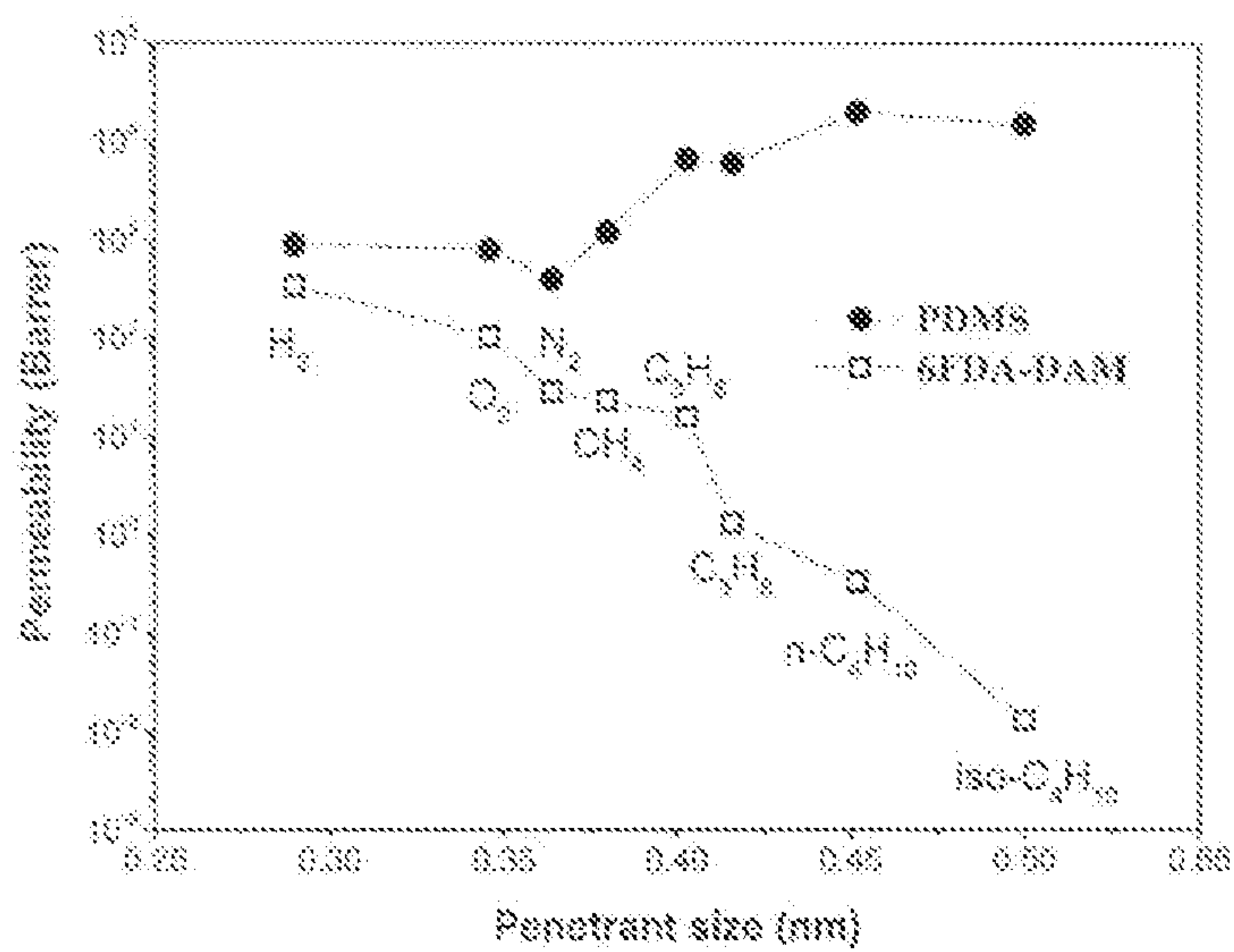
Figure 4: Permeability data in PDMS and SFDA-DAM. 1 Barrer=3.347x10 -10 mol·m/m 2 ·s·Pa 296x209mm (300 x 300 DPI)
