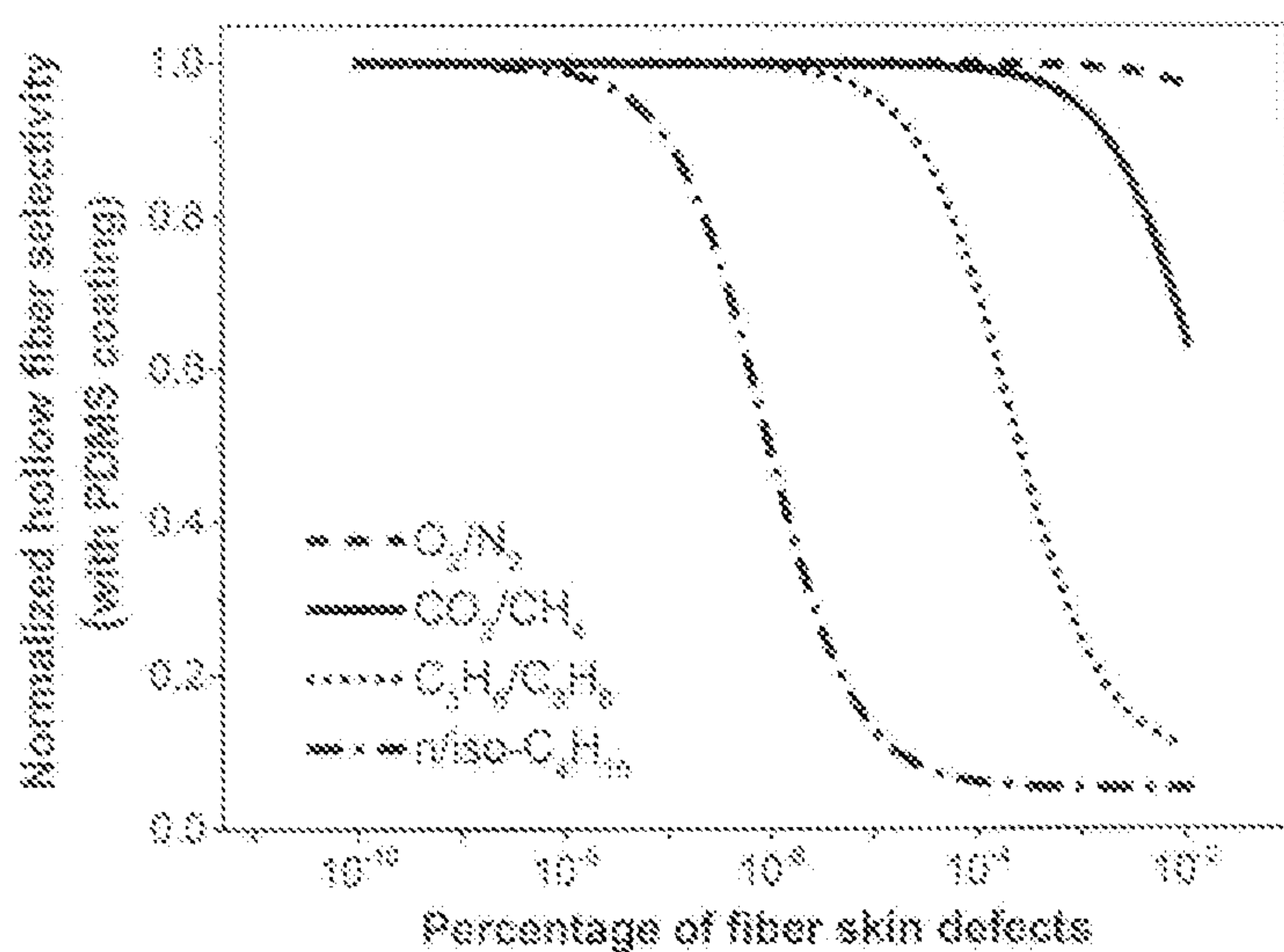
Figure 5x: Normalized selectivity of PDMS-coated 6FDA-DAM hollow fiber vs. percentage of fiber skin defects. It is assumed that PDMS fills the defects as well as forms a continuous layer on top of the fiber surface.
