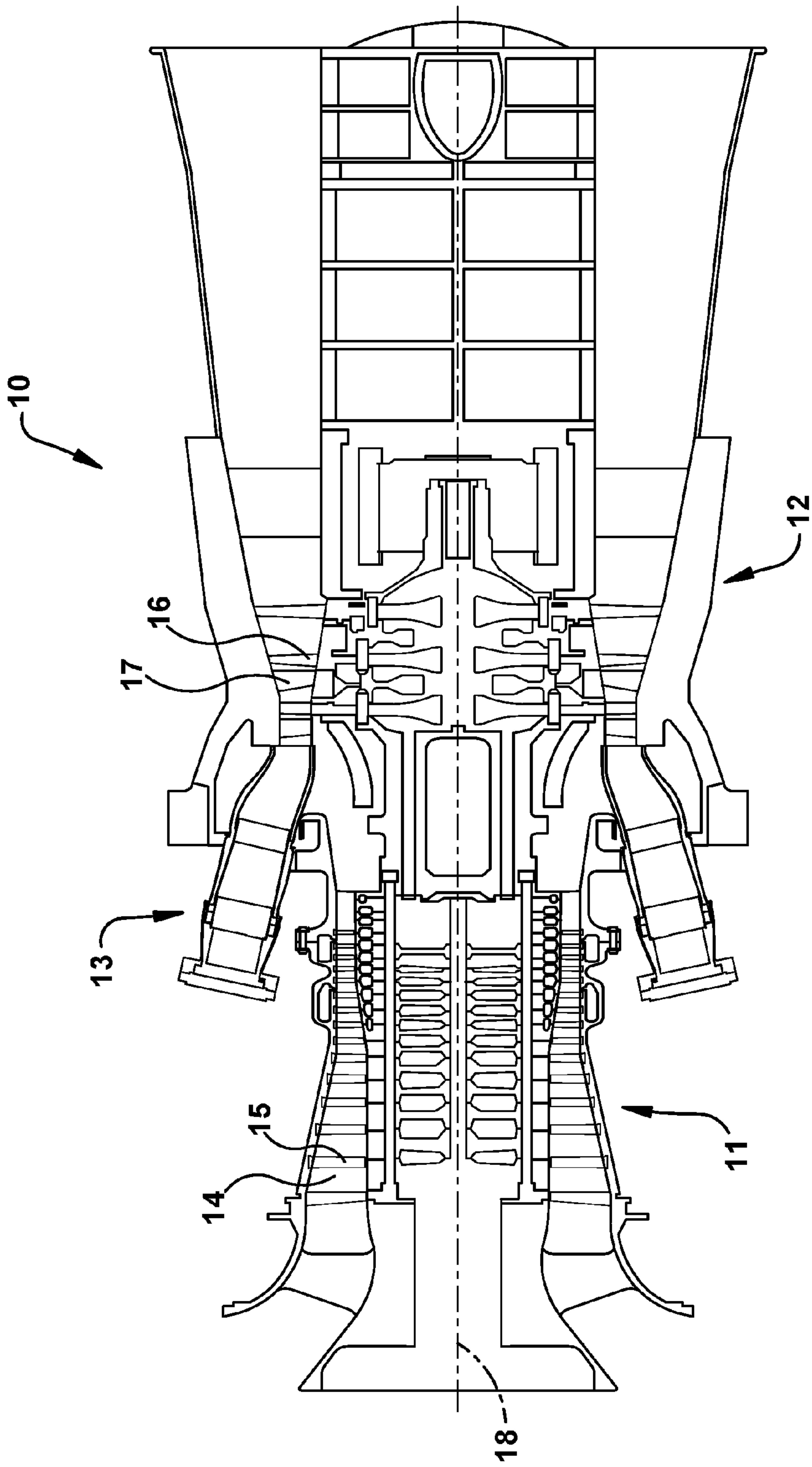
Figure 1 (Prior Art)
