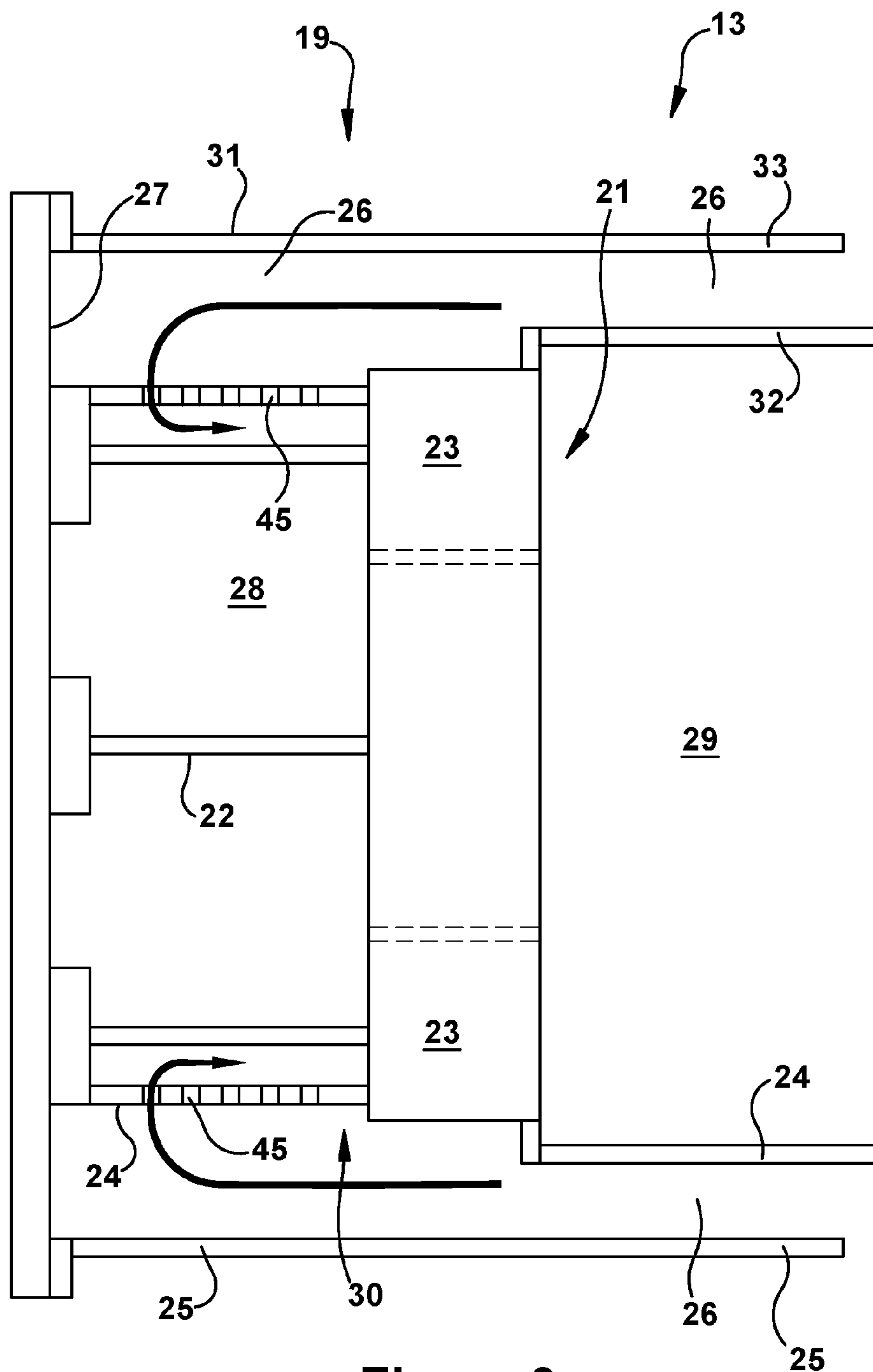
Figure 3 (Prior Art)
