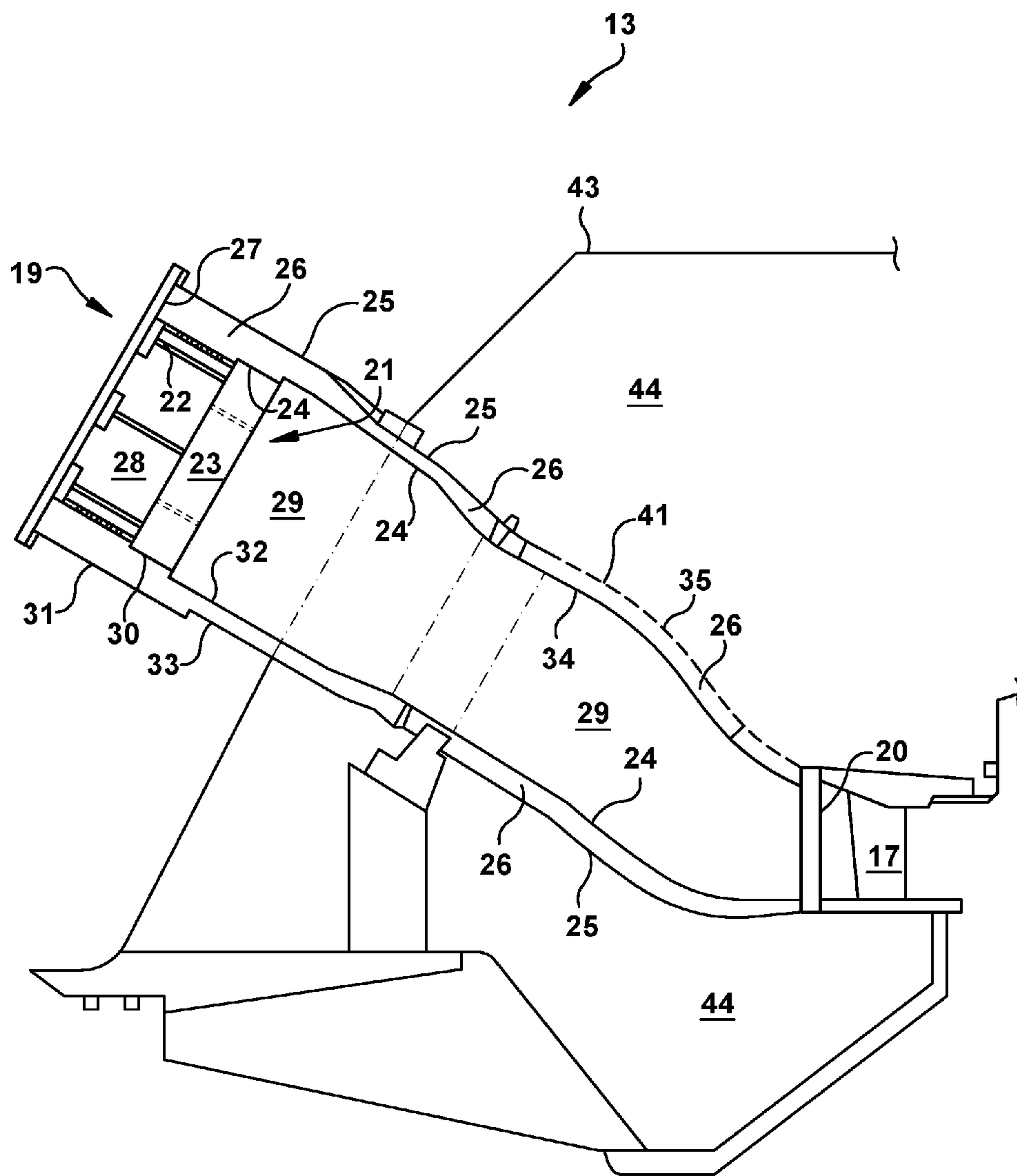
Figure 2 (Prior Art)
