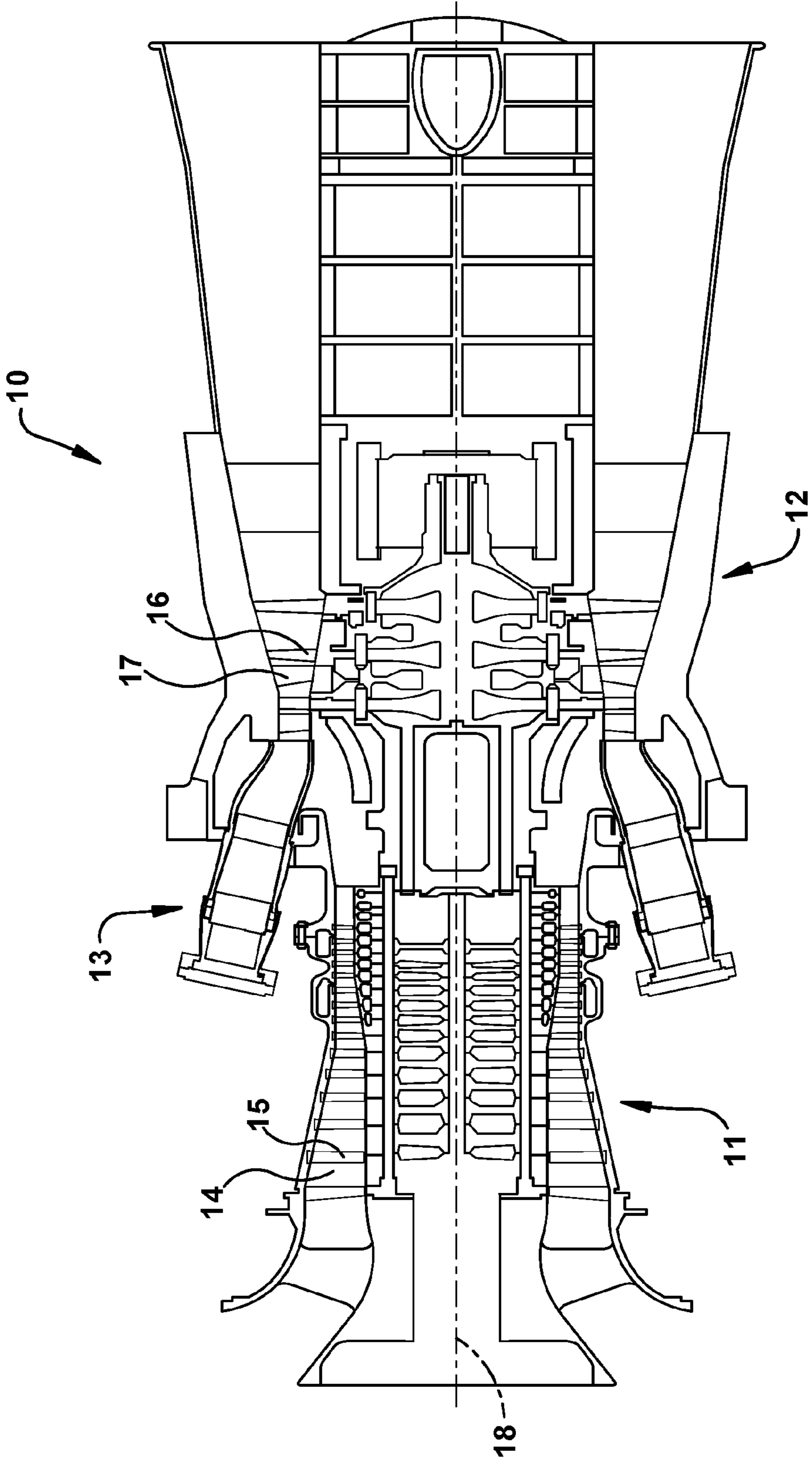
Figure 1 (Prior Art)
