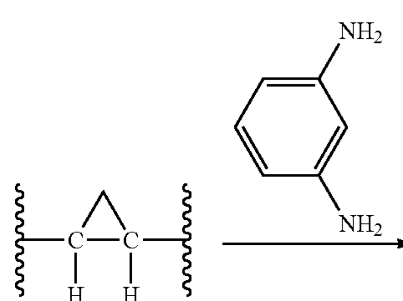
Scheme 1
