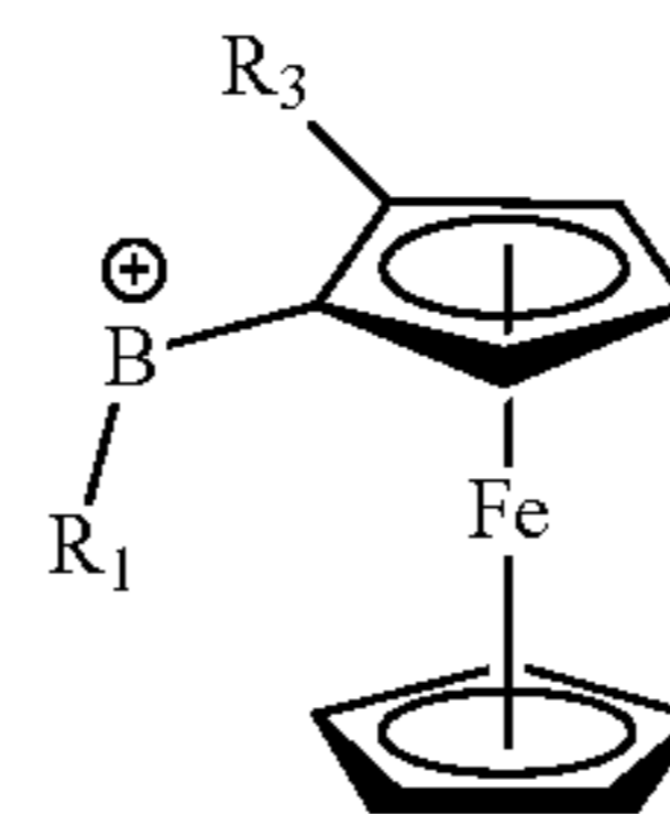
borenium ferrocene
