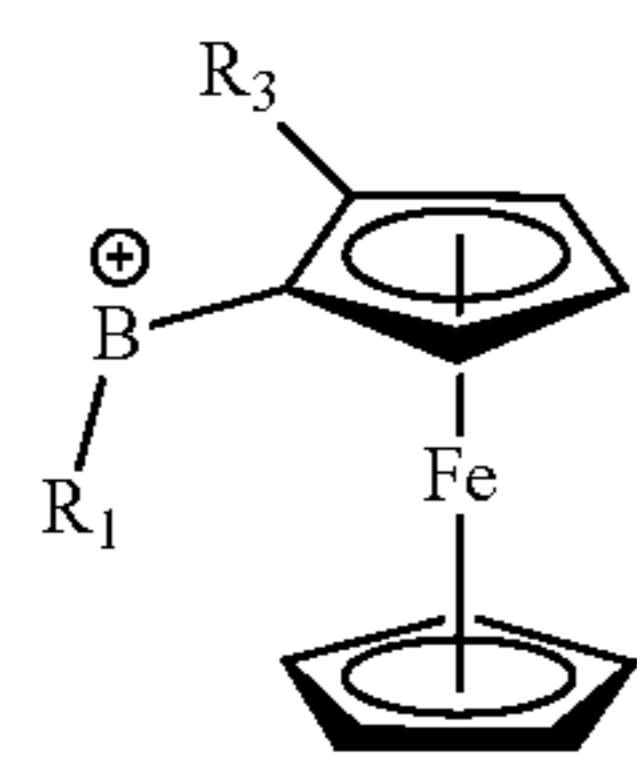
borenium ferrocene
