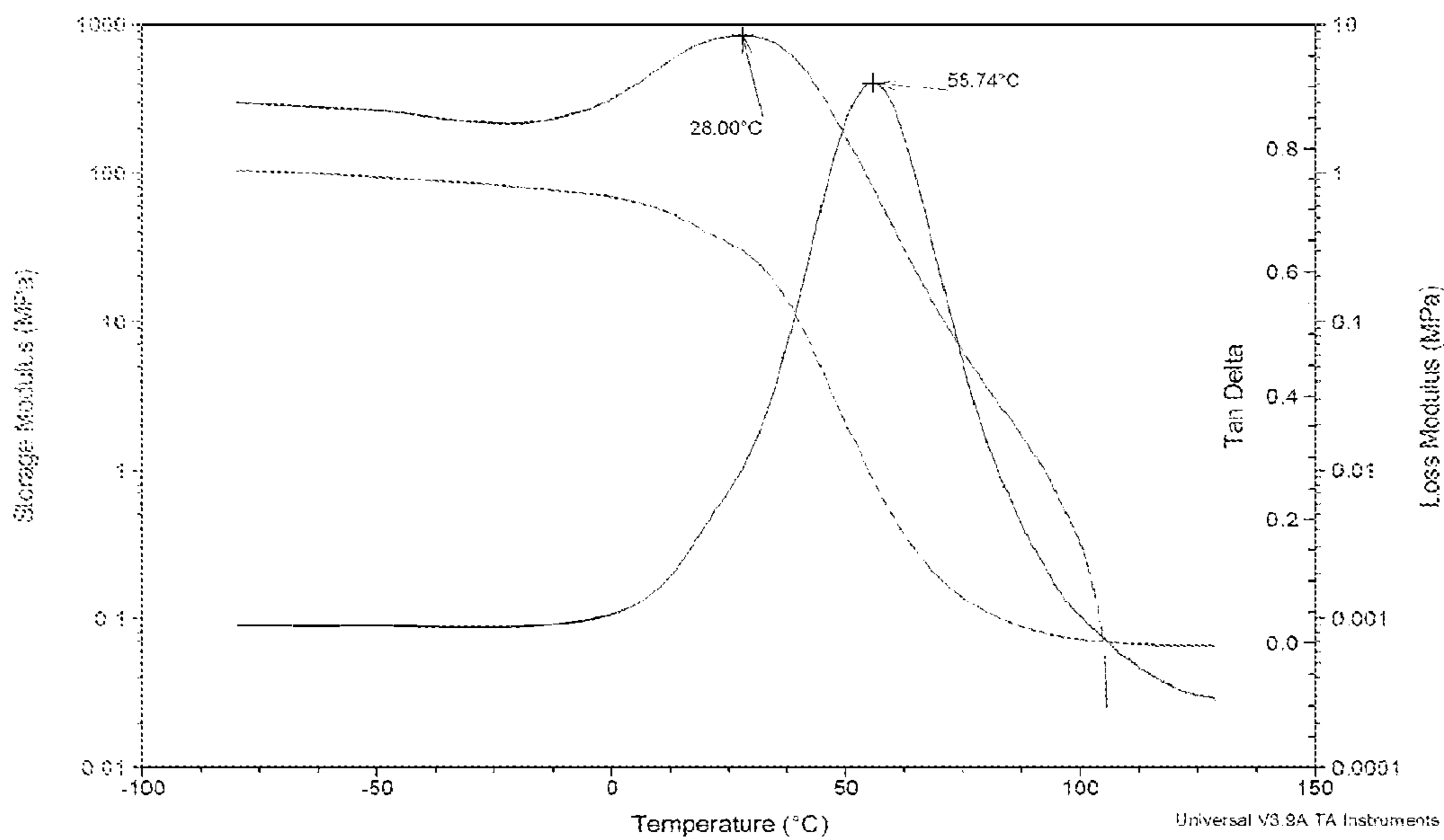
Figure 20b. DMA graph of foam prepared with a mixture of three different Novomer Polyols (Formulation #6 in Table 5B)
