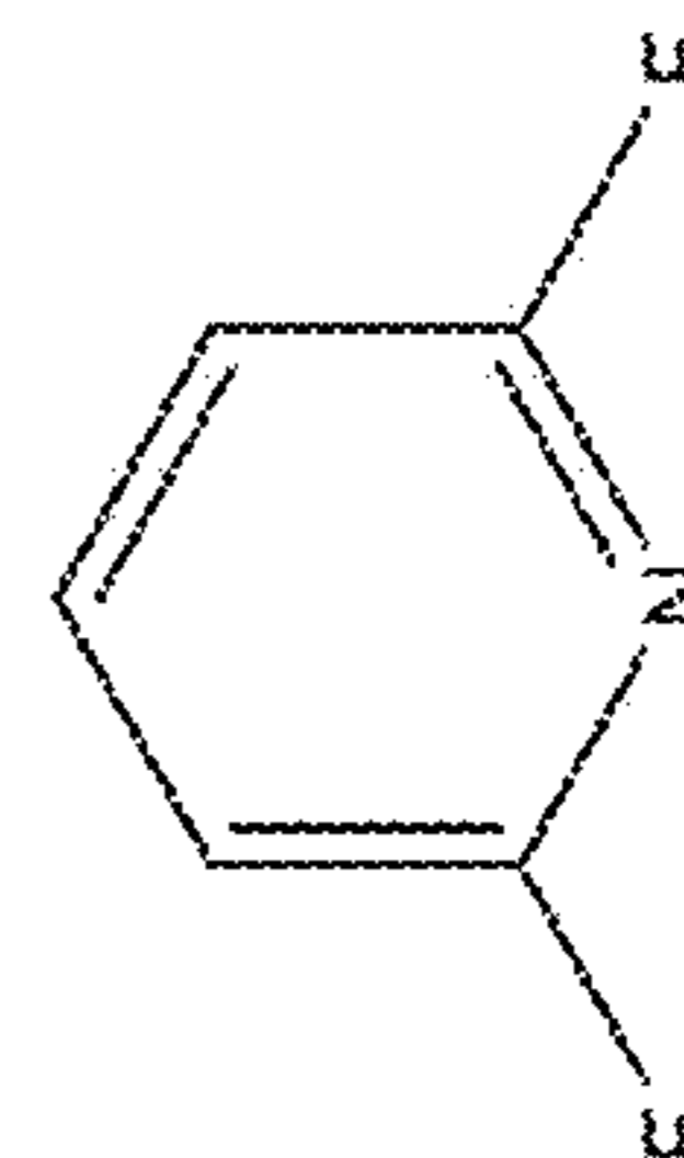
2,6-difluoropyridine (2,6-F 2 Py);
