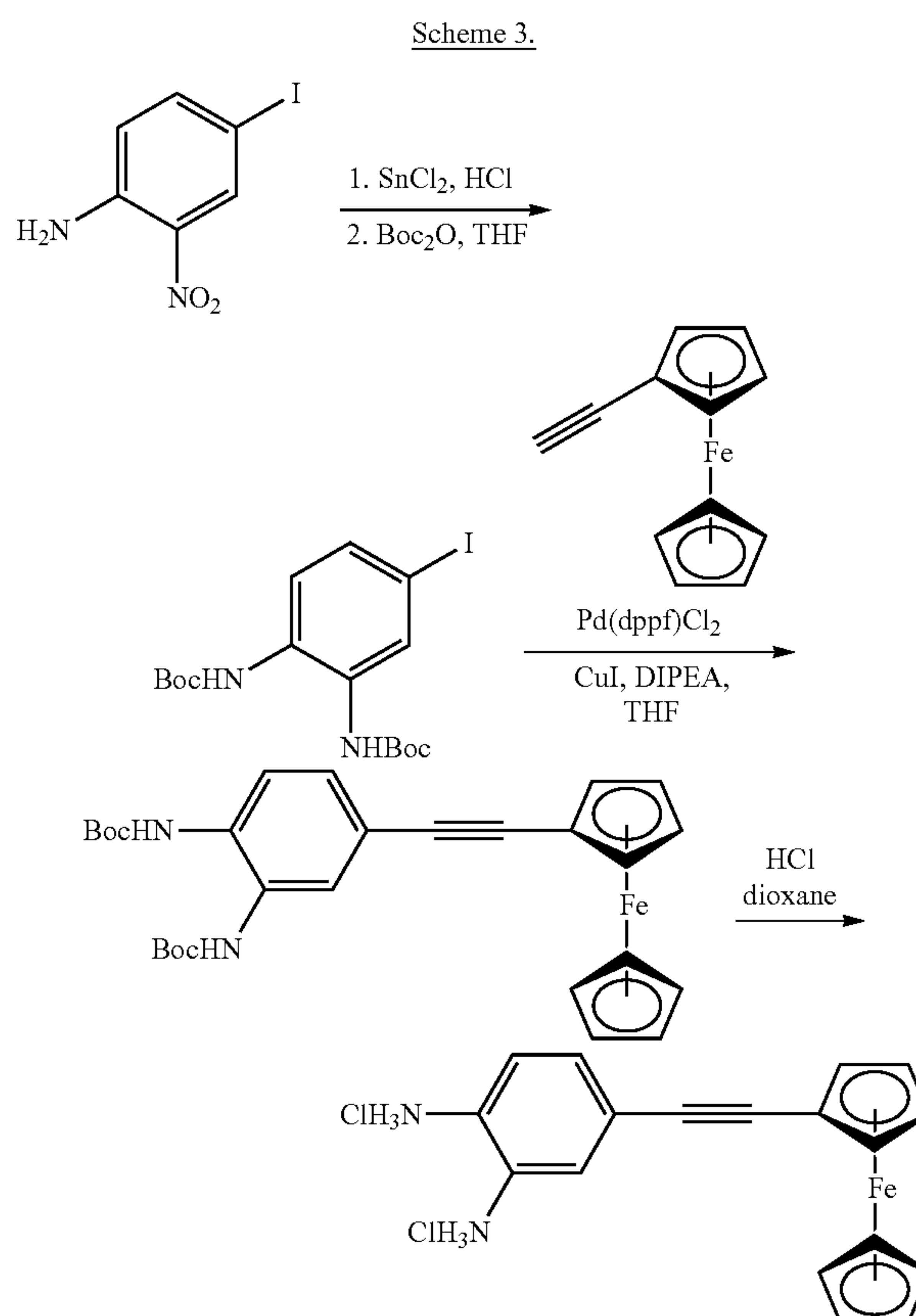
Synthetic scheme for ferrocenyl 4-ethynylbenzene-1,2-diamine (Compound 39).
