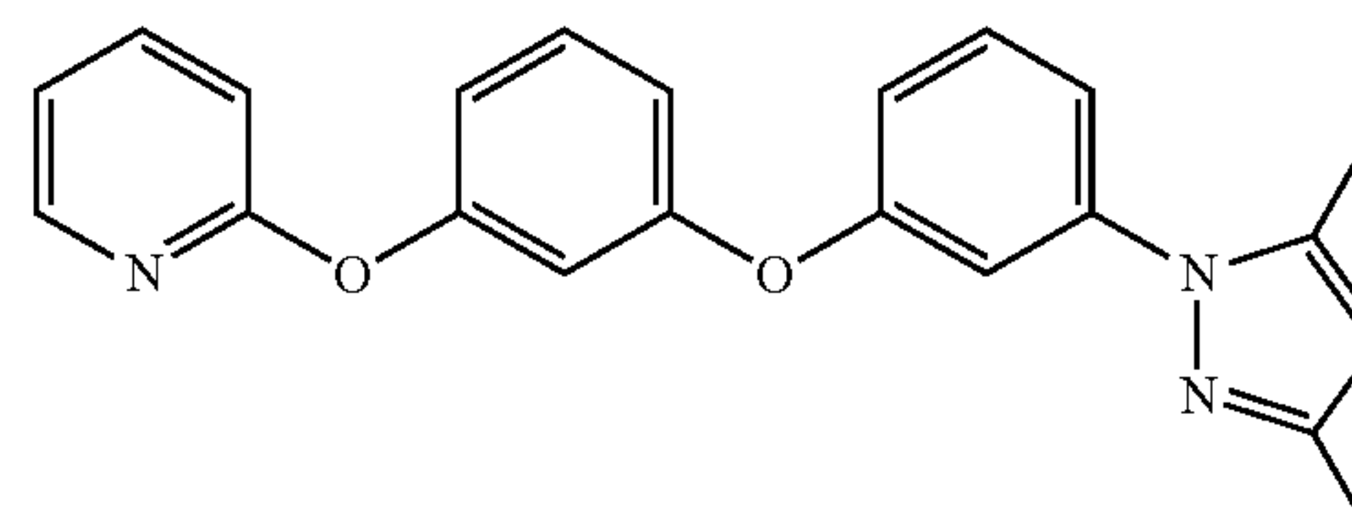
2-(3-(3-(3,5-dimethyl-1H-pyrazol-1-yl)phenoxy)phenoxy)pyridine
