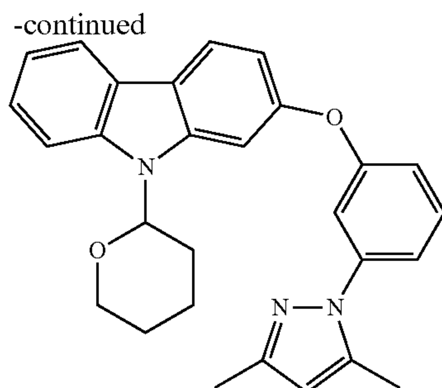
2-[3-(3,5-Dimethylpyrazol-1-yl)-phenoxy]- N-(tetrahydropyranyl)carbazole
