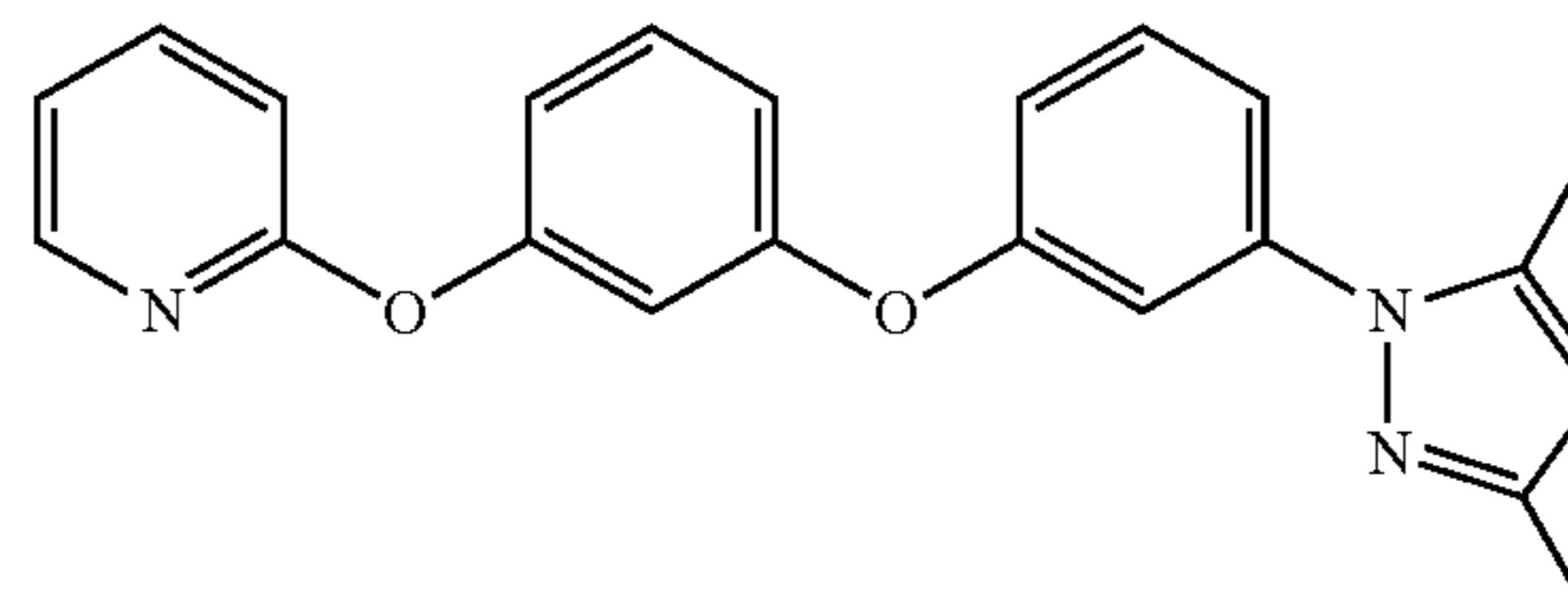
2-(3-(3-(3,5-dimethyl-1H-pyrazol-1-yl)phenoxy)phenoxy)pyridine
