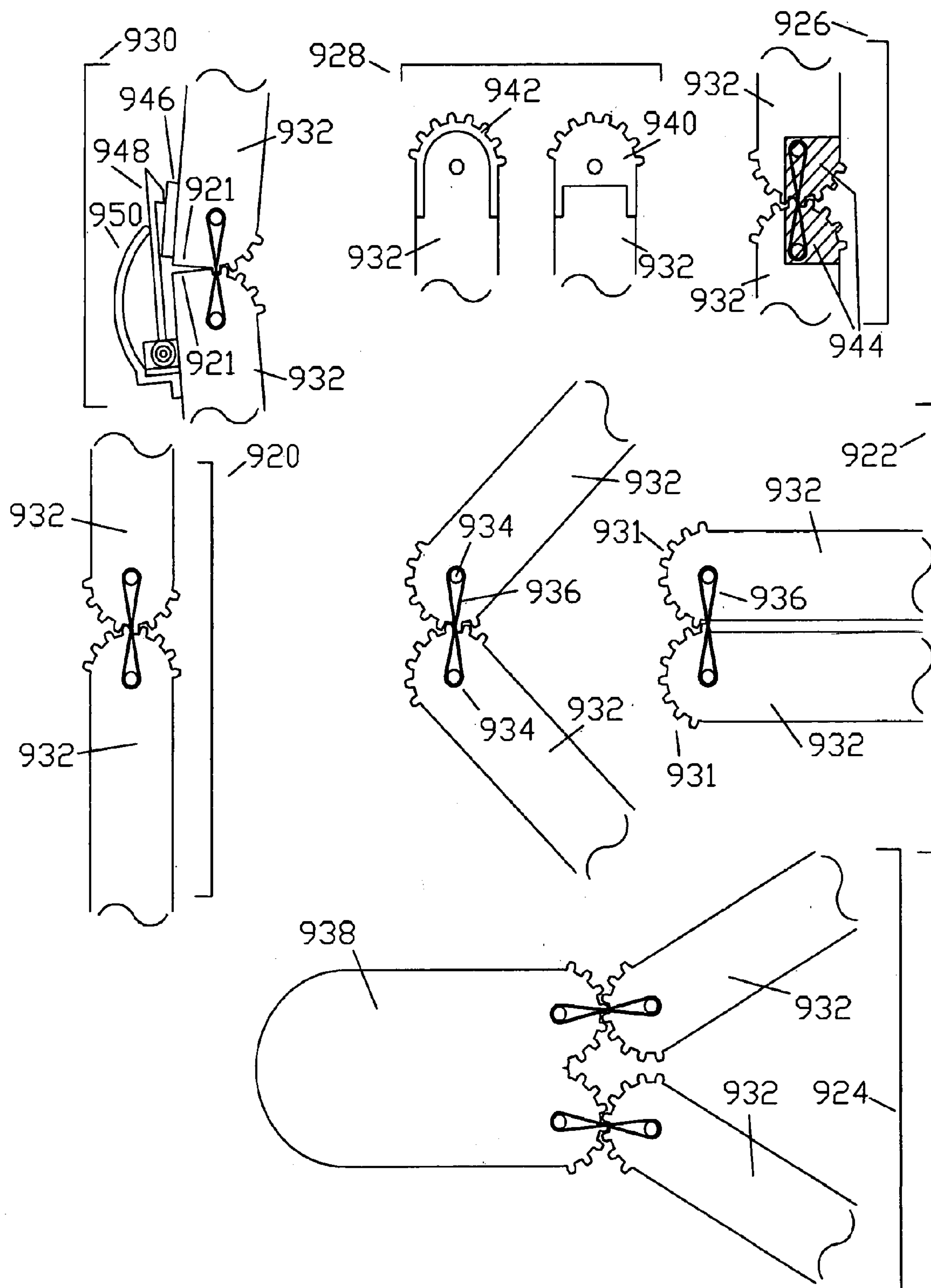
Figure 47. Tied Cogged Hinge Schematic Side Views
