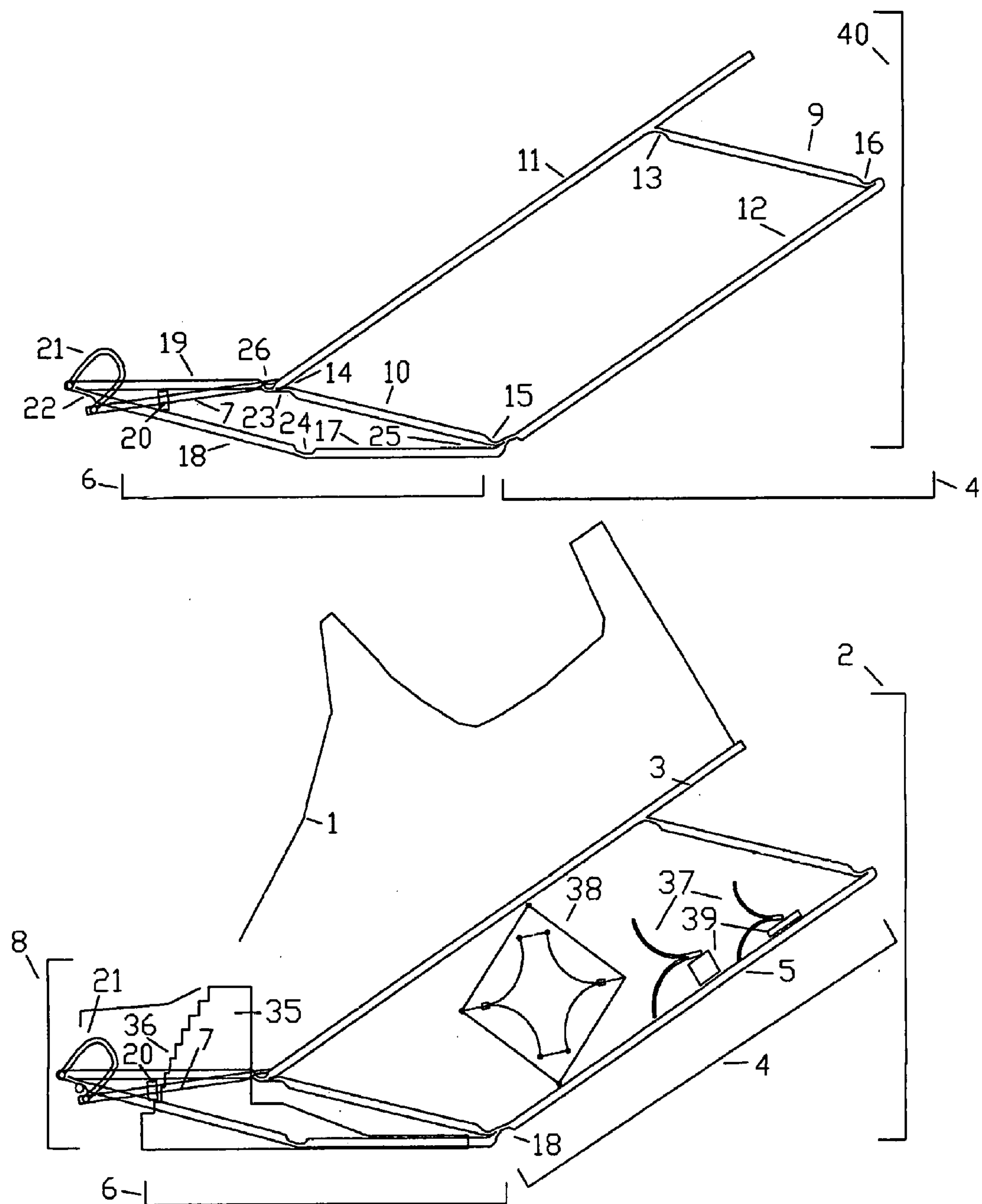
Figure 9. Parallelogram Heel-Pop Shoe Side view at toe-off
