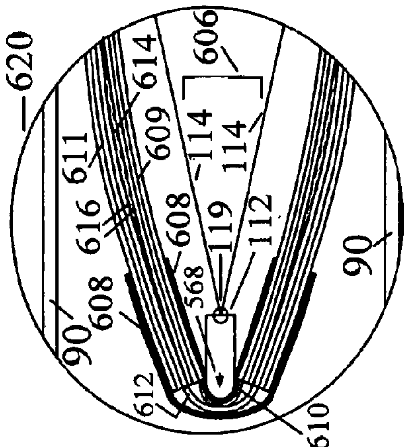
FIGURE 35B. Exploded View of Enhanced Natural Hinge Schematic Side View Compressed
