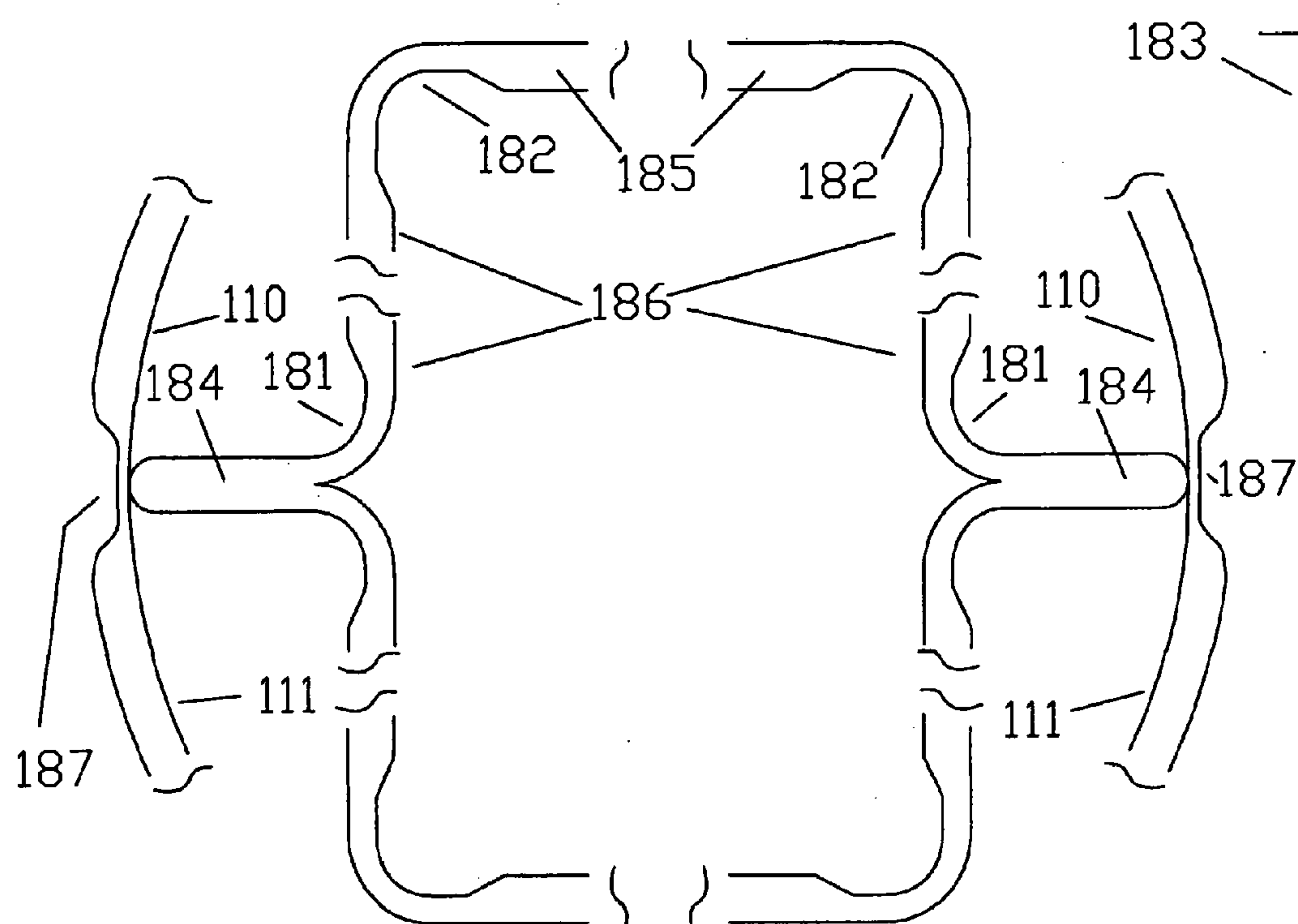
Figure 15. Monolithic Mirrored Spreader Linkage Schematic Side Views
