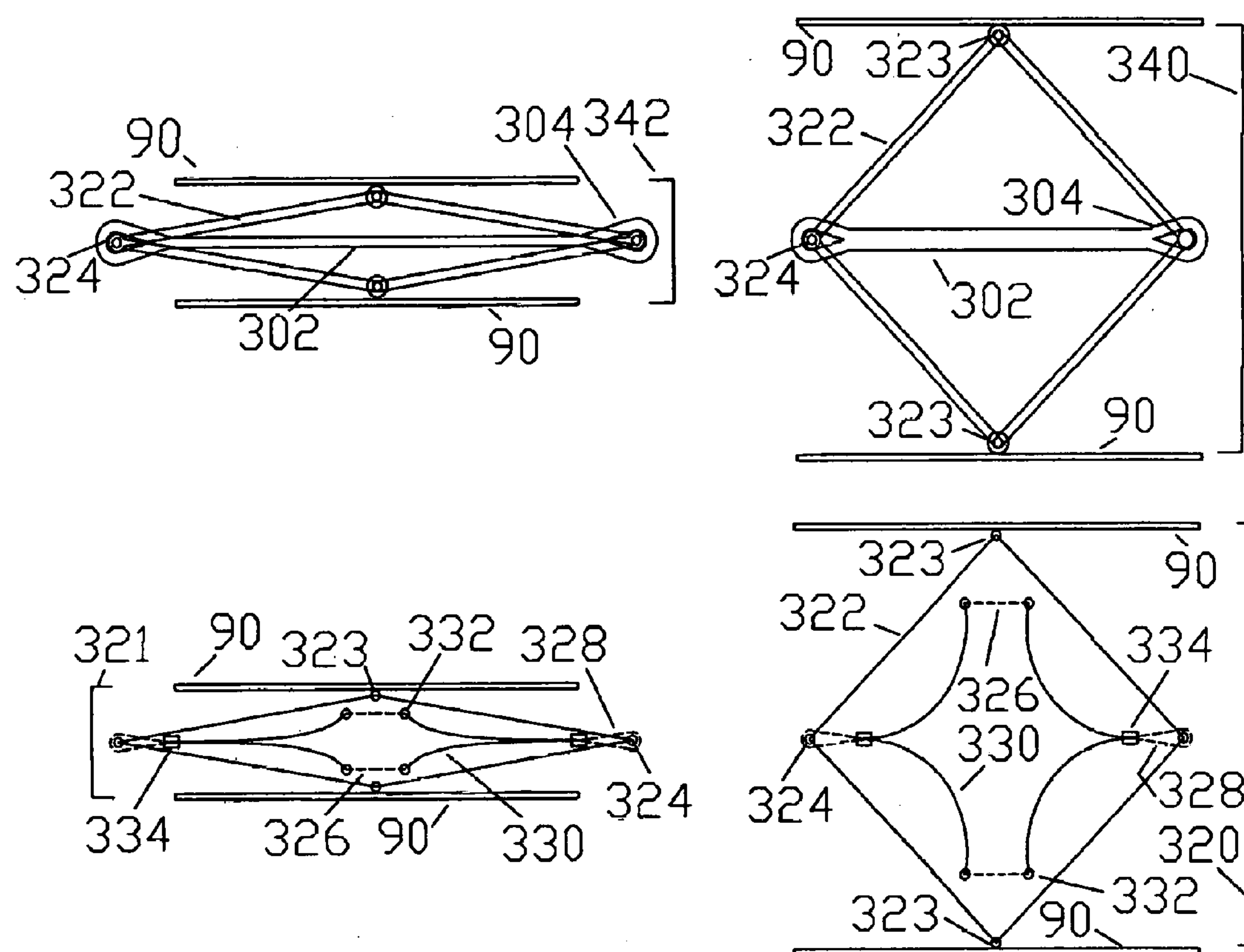
Figure 21. Tensioned Linkage Configurations Schematic Side Views
