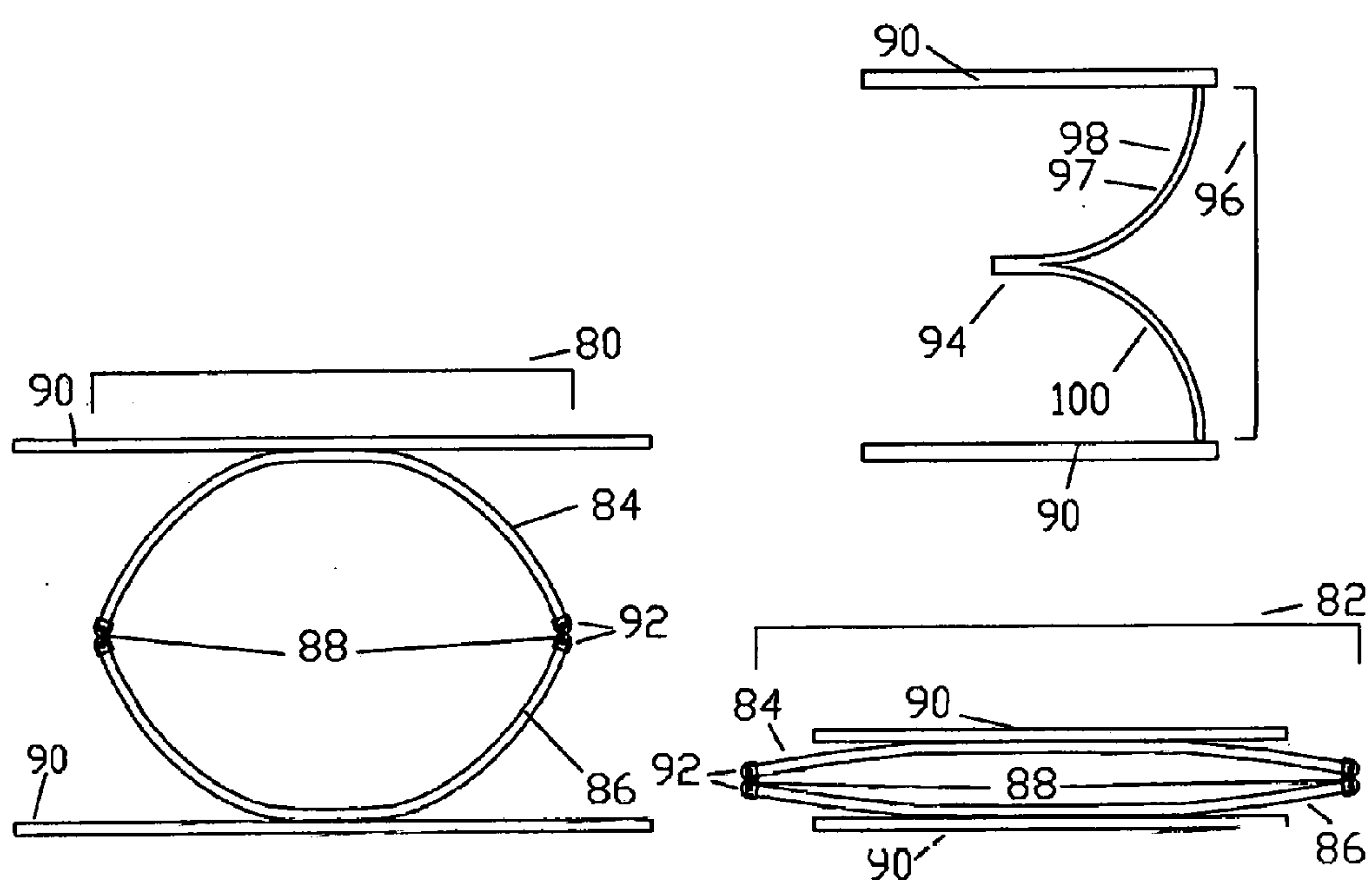
Figure 10. Mirrored Arch Spring and Curly V-Spring Schematic Side Views
