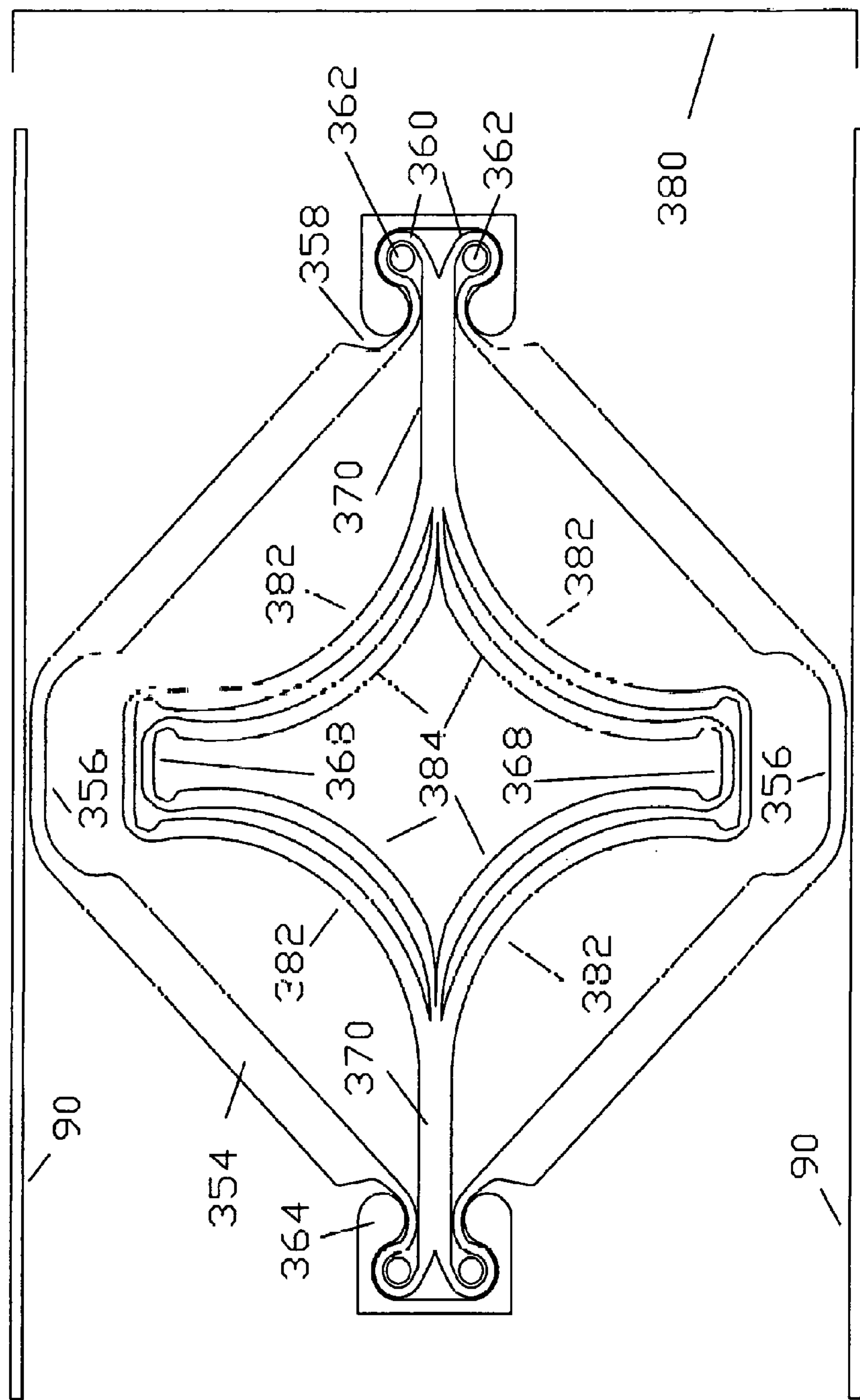
Figure 23. Monolithic Nested Tensioned Linkage Spring Schematic Side View
