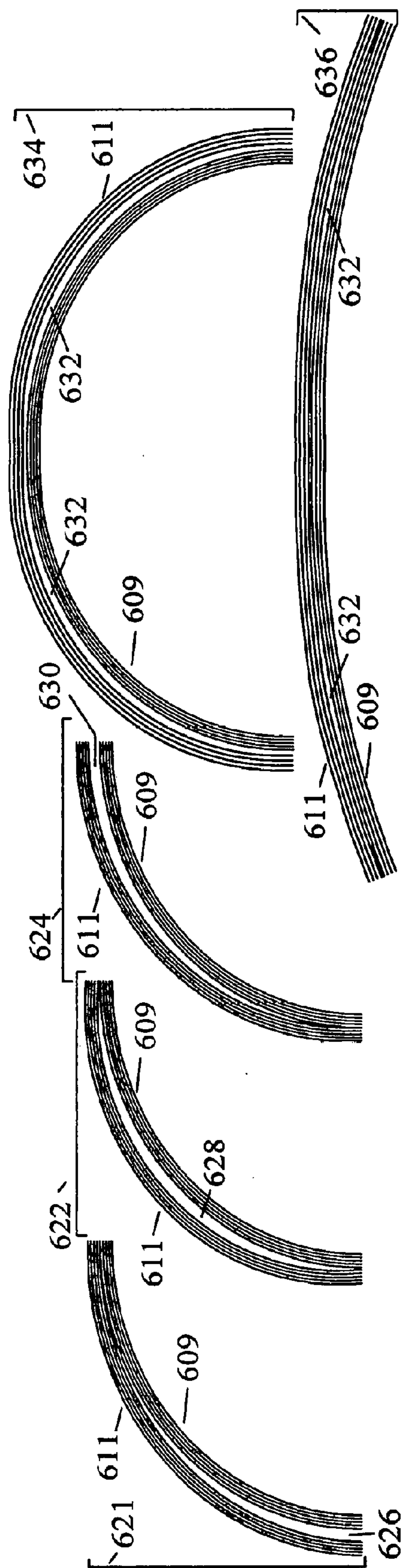
Figure 35C. Void Options for Merging Arms Schematic Side Views
