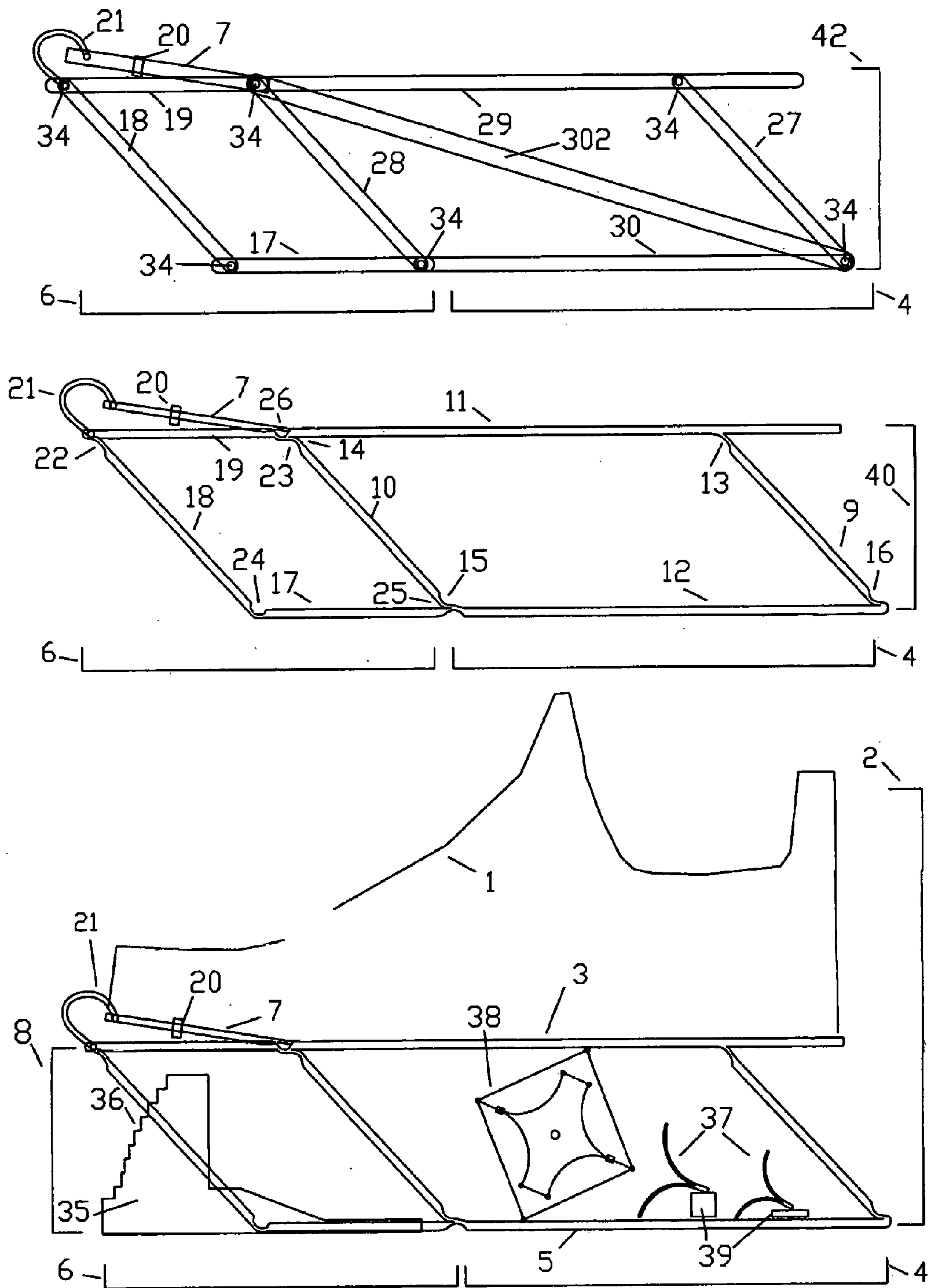
Figure 7. Parallelogram Heel-Pop Shoe Side view at heel strike
