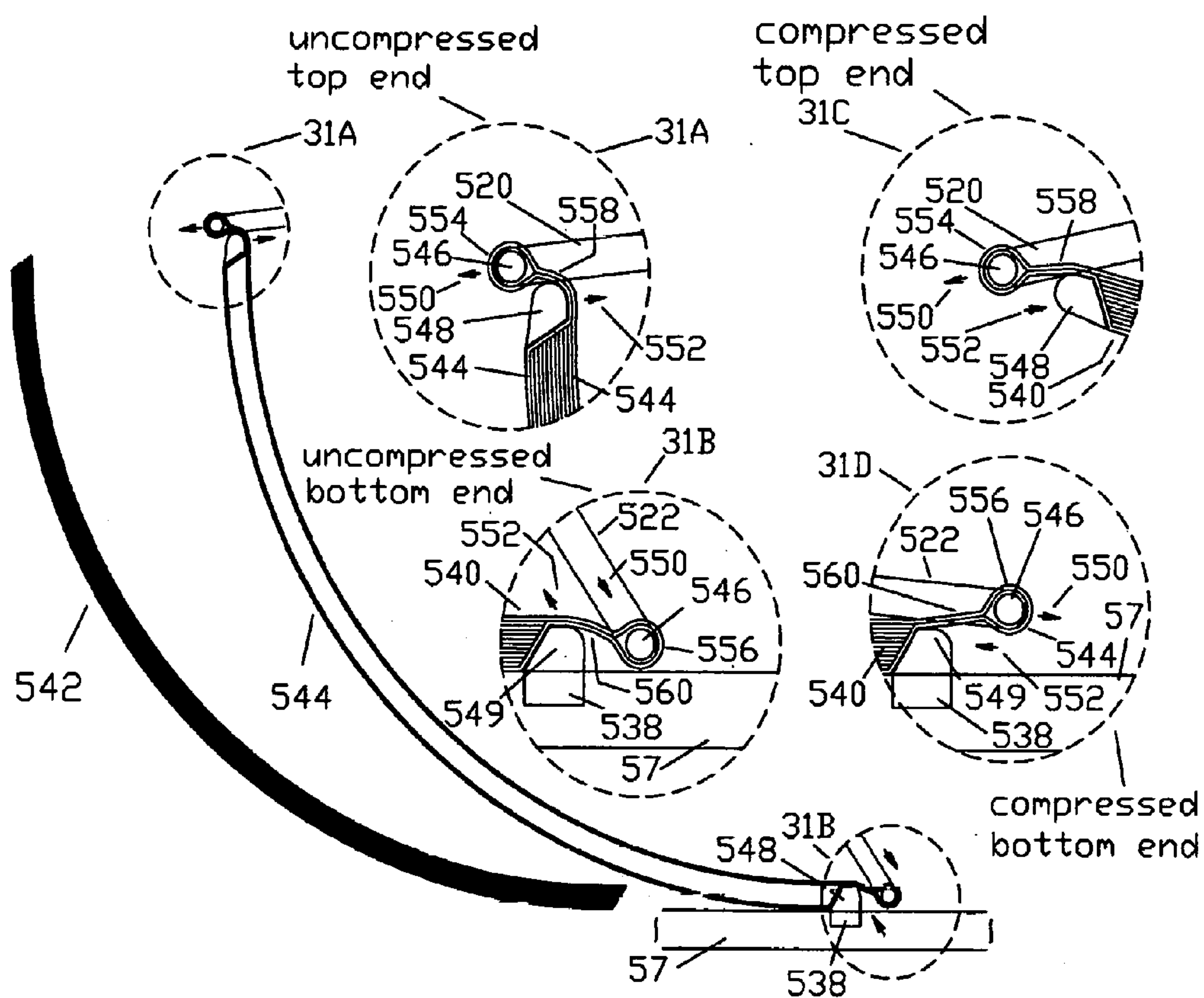
Figure 31. Details of Revised One-Sided Curved-Spring Linkage Schematic Side Views
