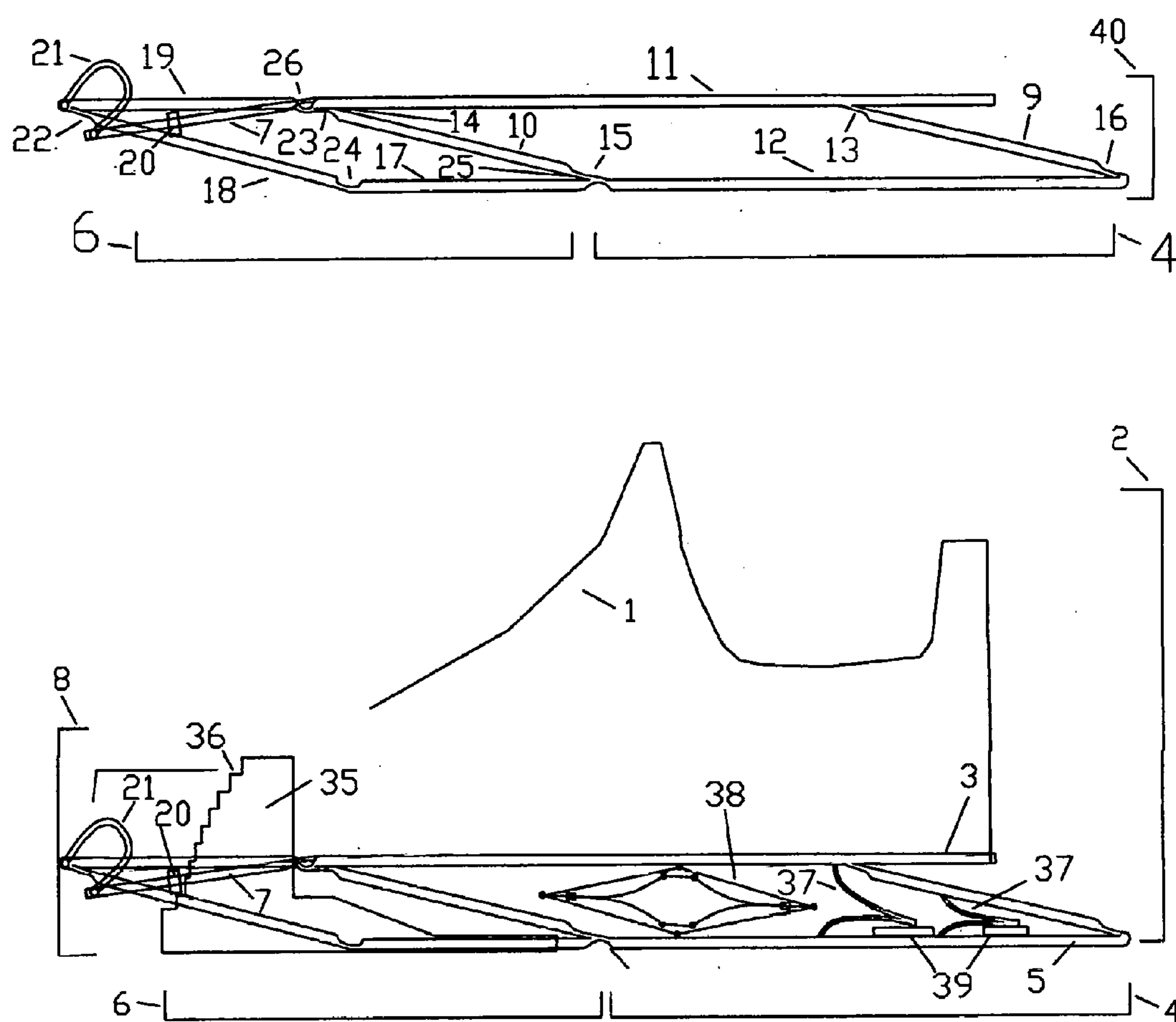
Figure 8. Parallelogram Heel-Pop Shoe Side view at full compression
