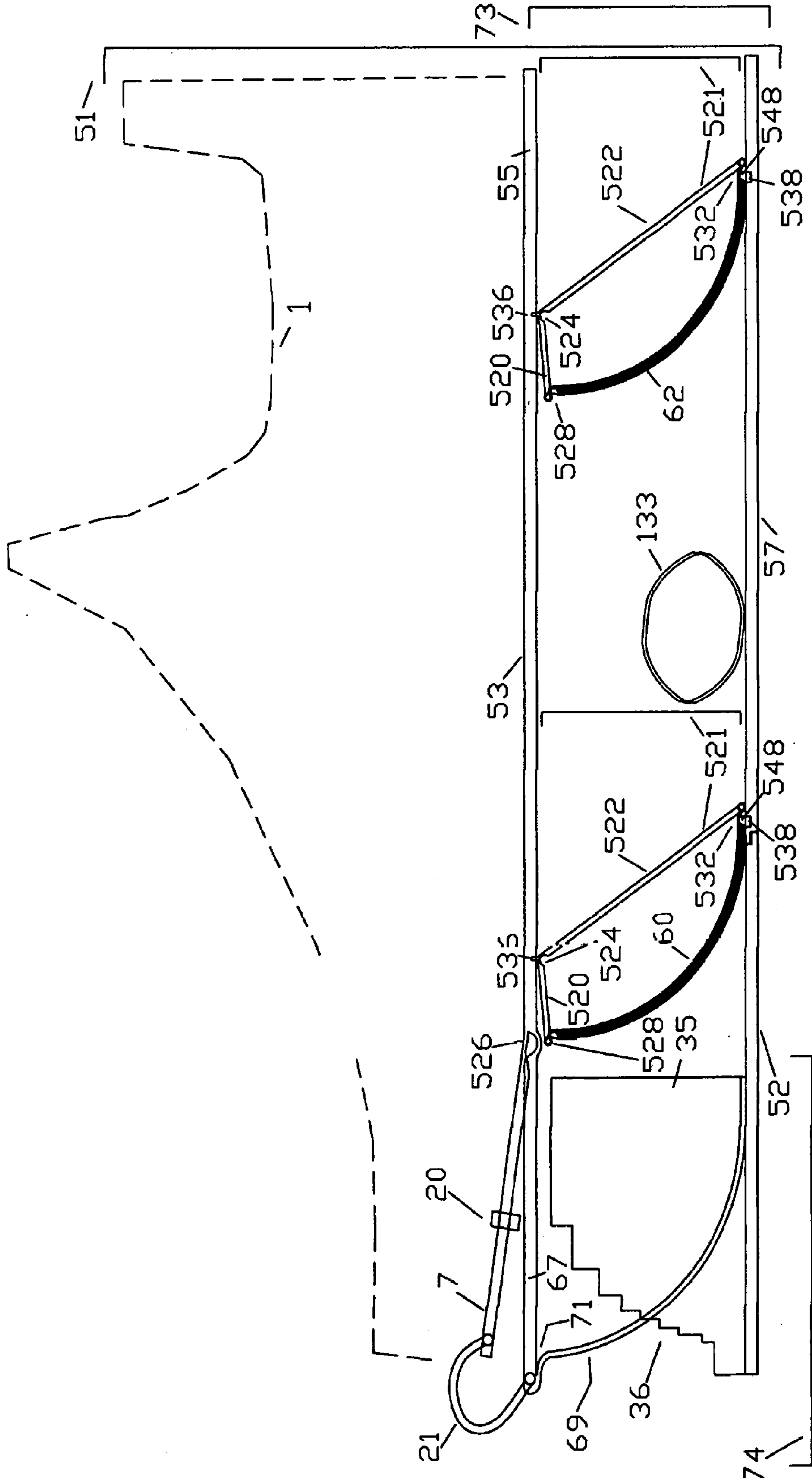
Figure 28. Linkage-Spread Curved-Spring Heel-Pop Shoe with Revised Linkage Schematic Side View at Heel Strike
