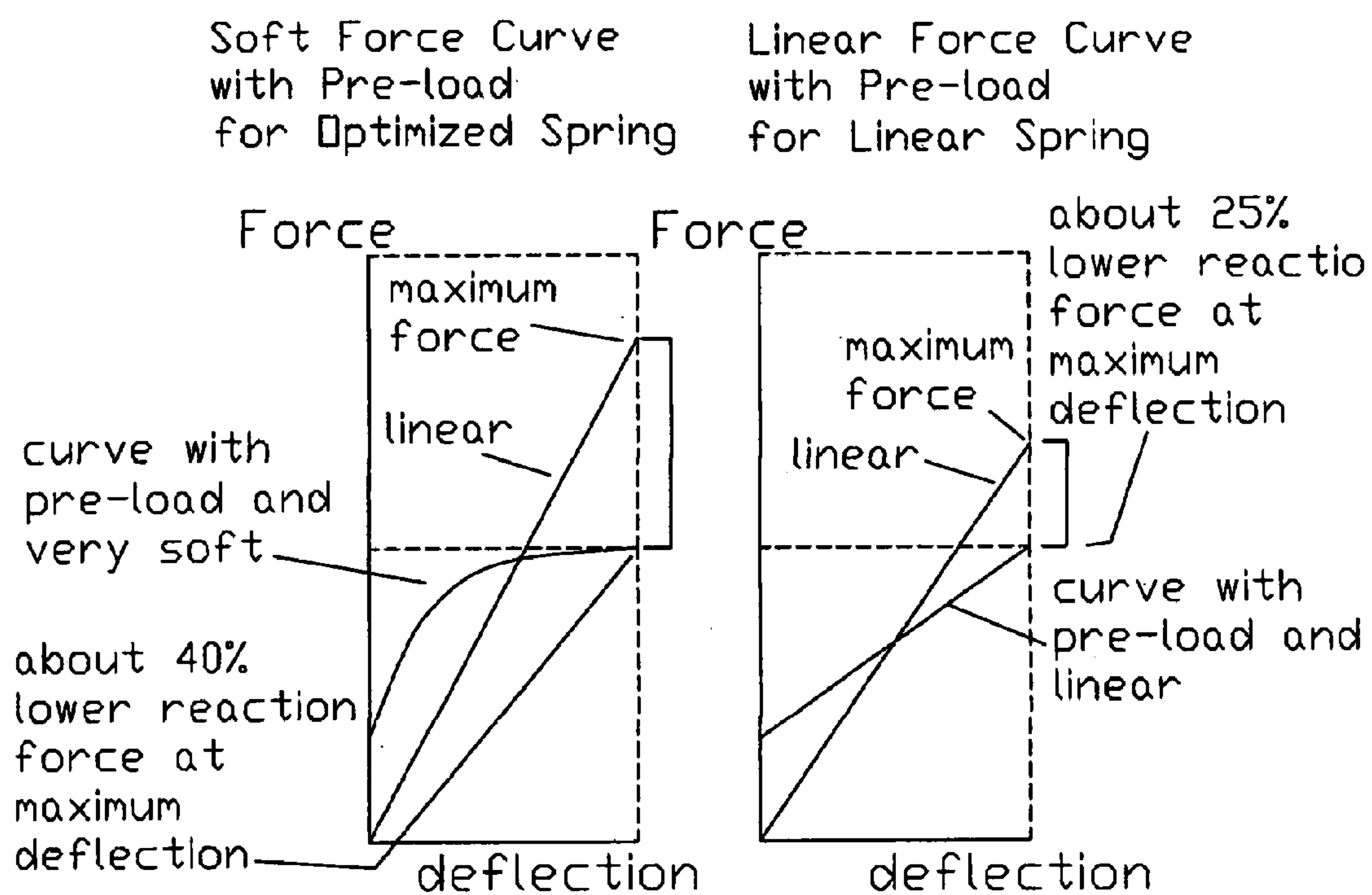
Figure 12. Study of Optimized Force Curves for Springs
