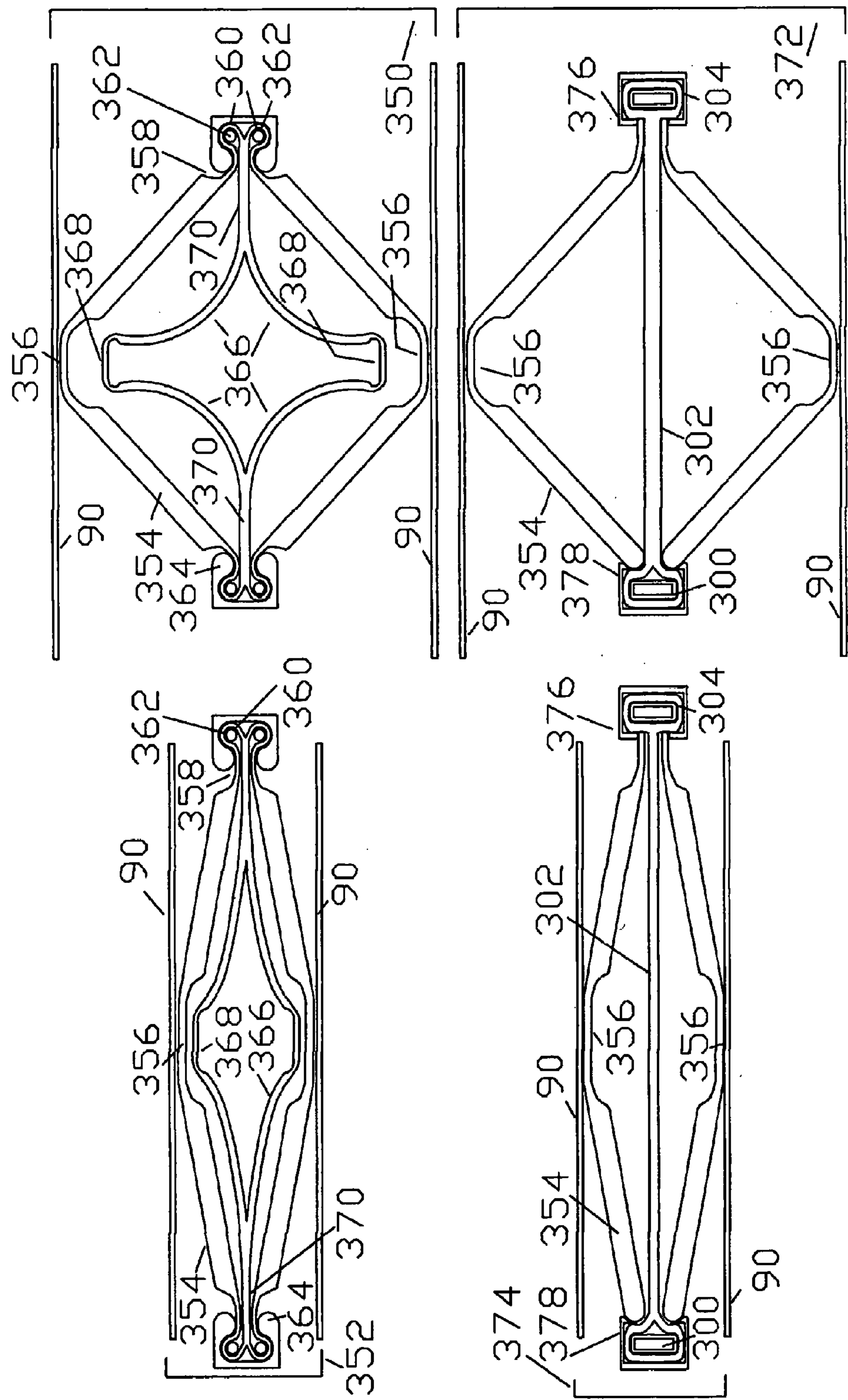
Figure 22. Monolithic Tensioned Linkage Configurations Schematic side Views
