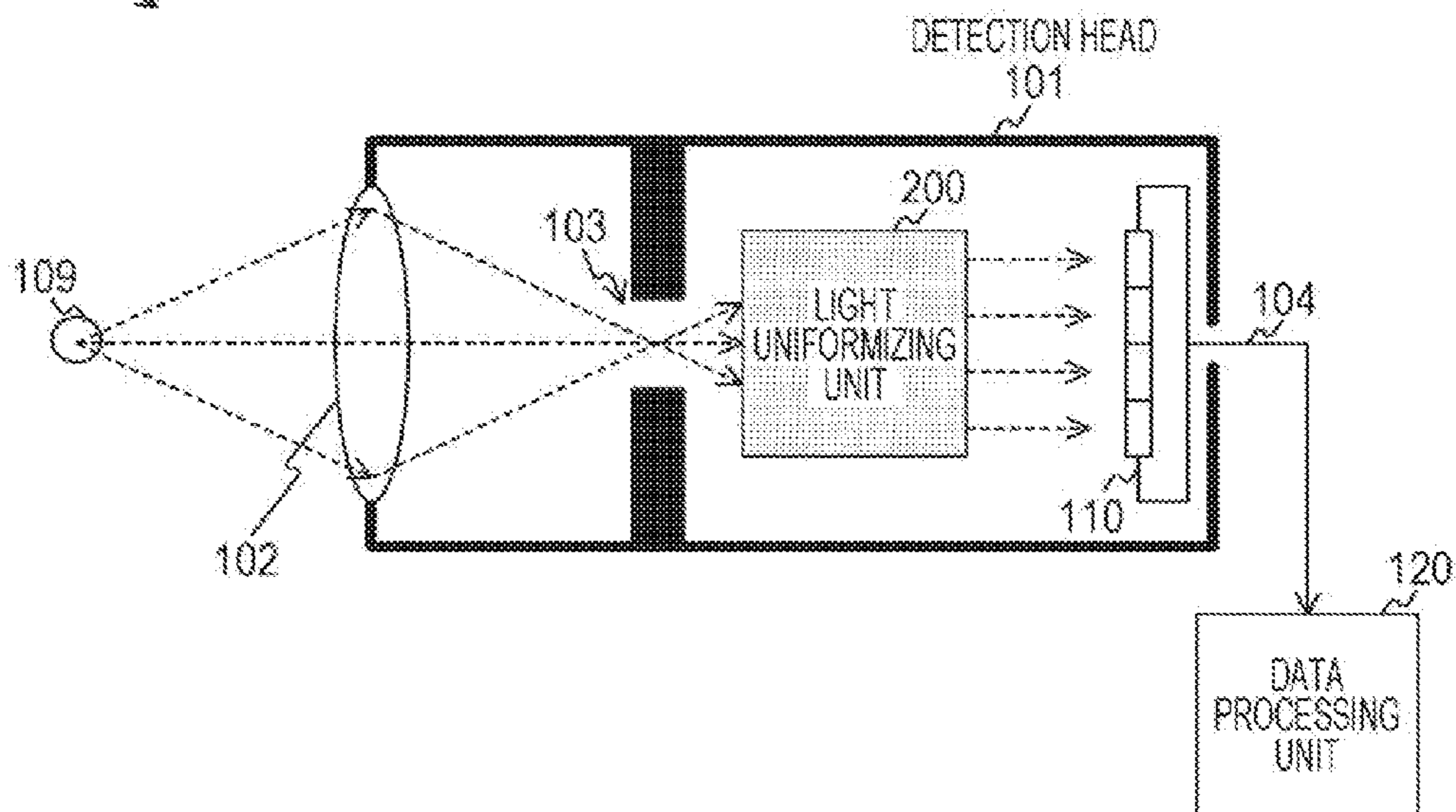
LIGHT DETECTION APPARATUS 10
