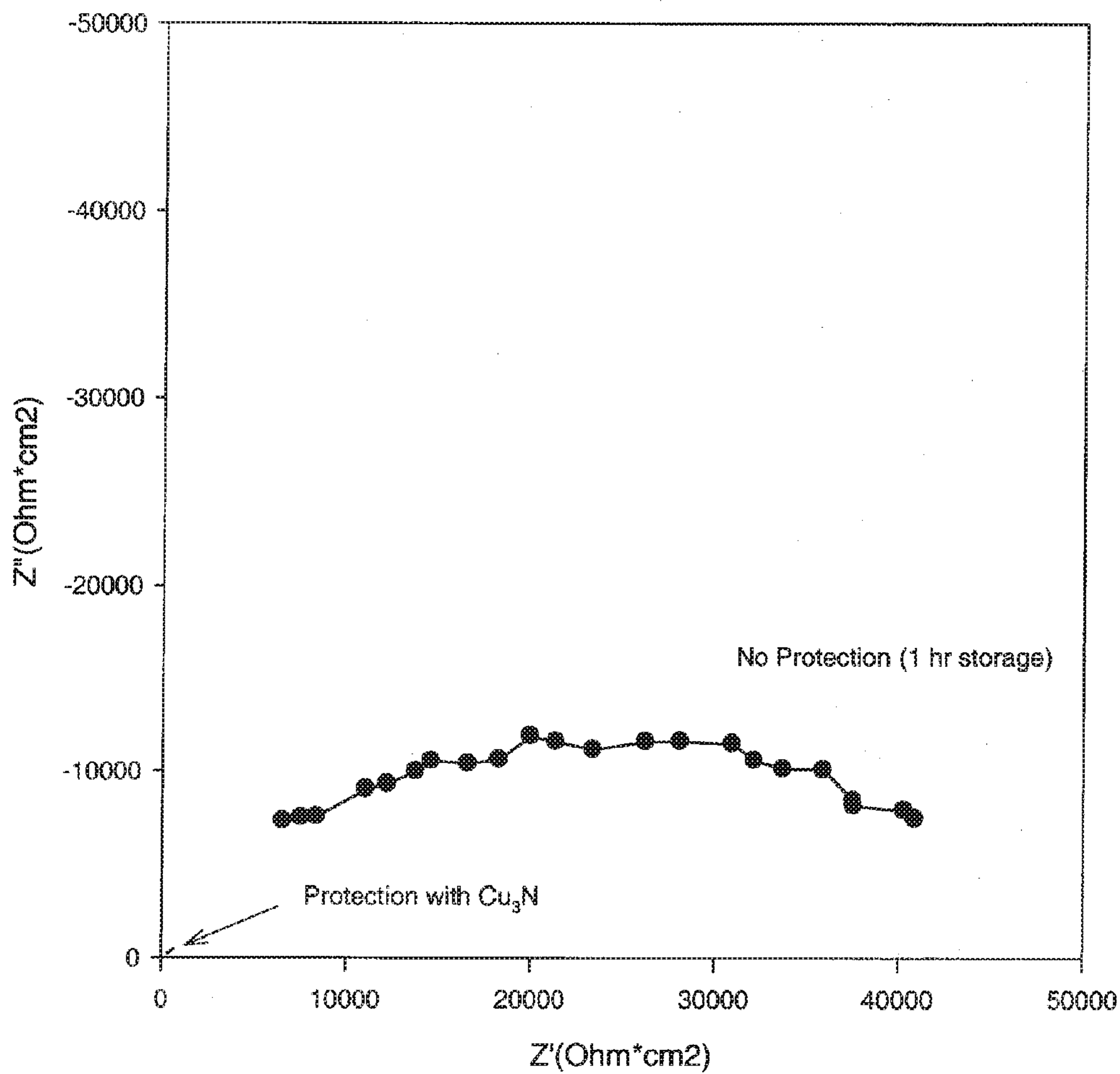
Impedance Plot for Cells Having Unprotected and \text{Cu}_3\text{N} -protected OHARA Material
