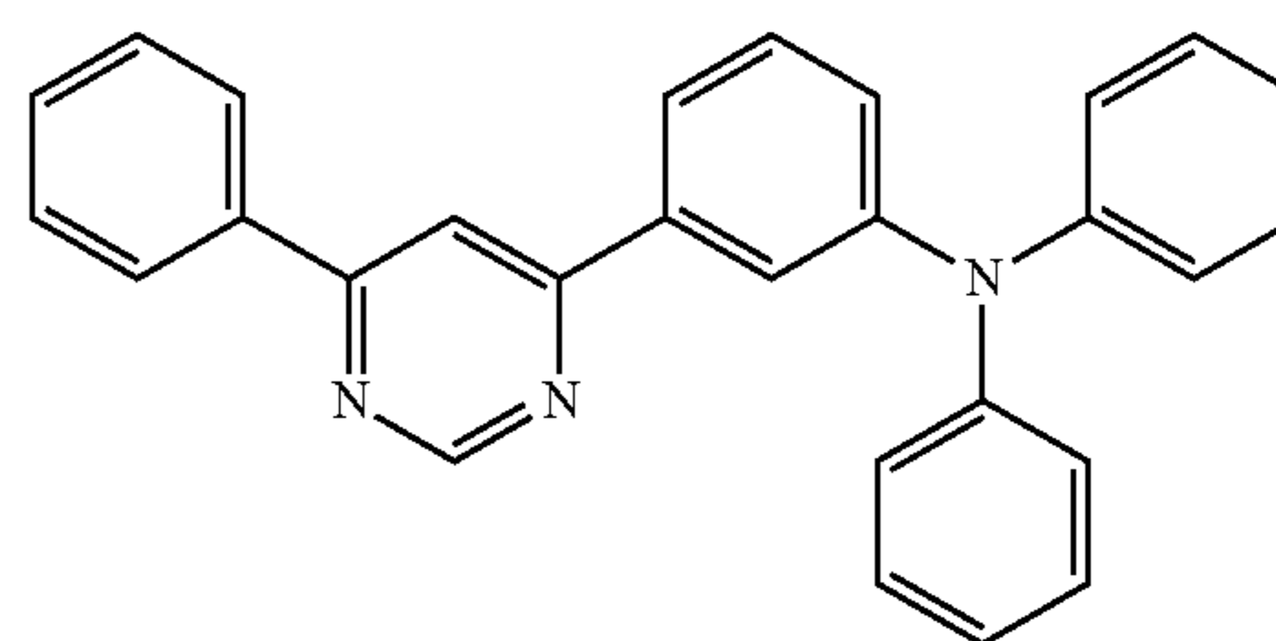
4mDPhAPPm
