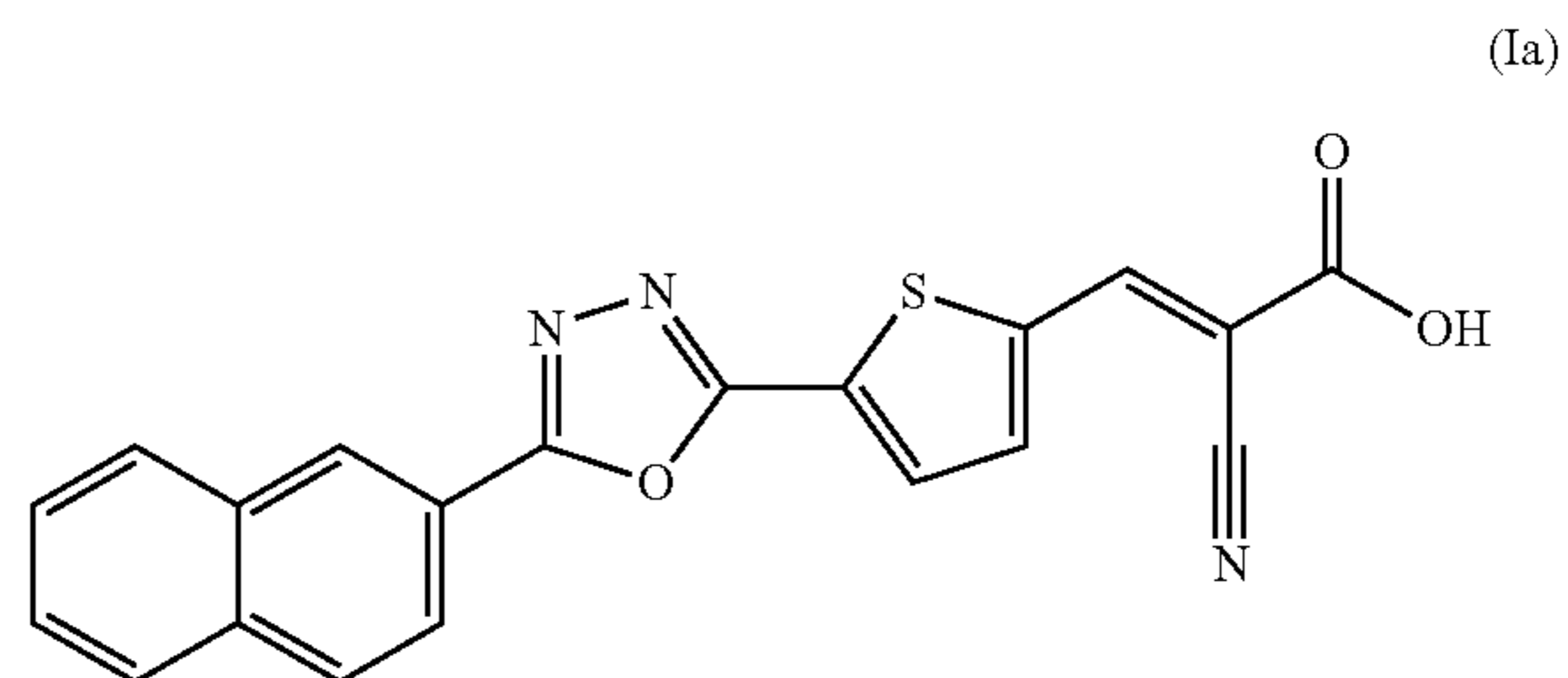
(E)-2-cyano-3-(5-(5-(naphthalen-2-yl)-1,3,4-oxadiazol-2-yl)thiophen-2-yl)cyanoacrylic acid
