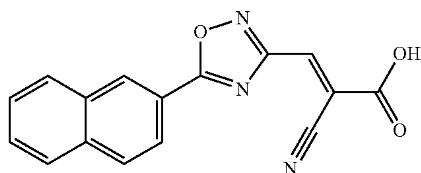
(E)-2-cyano-3-(5-(naphthalen-2-yl)-1,2,4-oxadiazol-3-yl)acrylic acid
