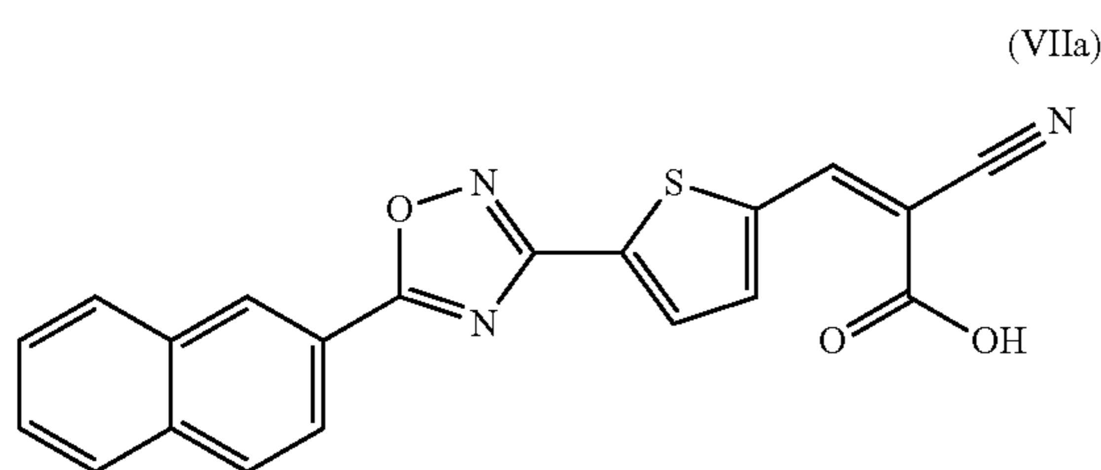
(Z)-2-cyano-3-(5-(5-(naphthalen-2-yl)-1,2,4-oxadiazol-3-yl)thiophen-2-yl)acrylic acid
