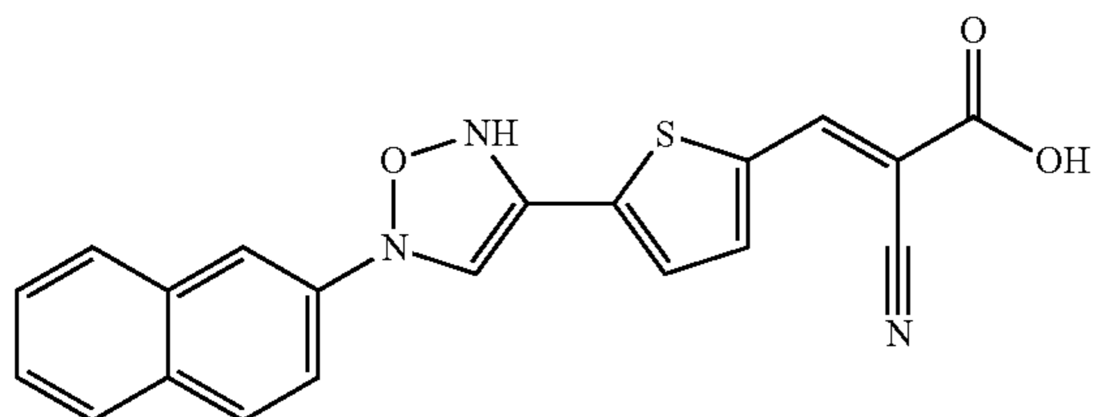
(E)-2-cyano-3-(5-(5-naphthalen-2-yl)-1,2,5-oxadiazol-3-yl)thiophen-2-ylcyanoacrylic acid
