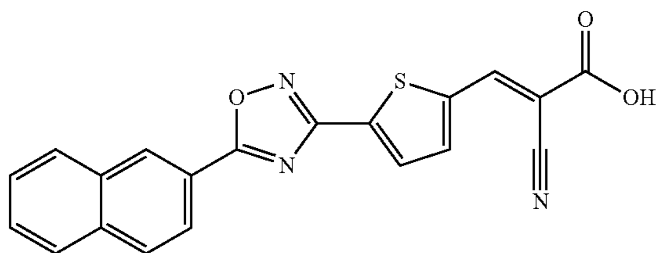
(E)-2-cyano-3-(5-(5-(naphthalen-2-yl)-1,2,4-oxadiazol-3-yl)thiophen-2-yl)cyanoacrylic acid
