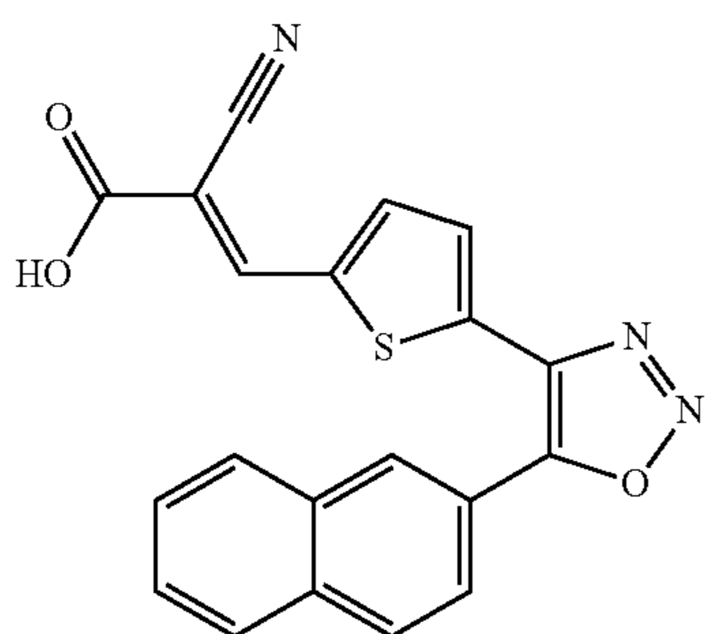
(E)-2-cyano-3-(5-(5-(naphthalen-2-yl)-1,2,3-oxadiazol-4-yl)thiophen-2-yl)cyanoacrylic acid
