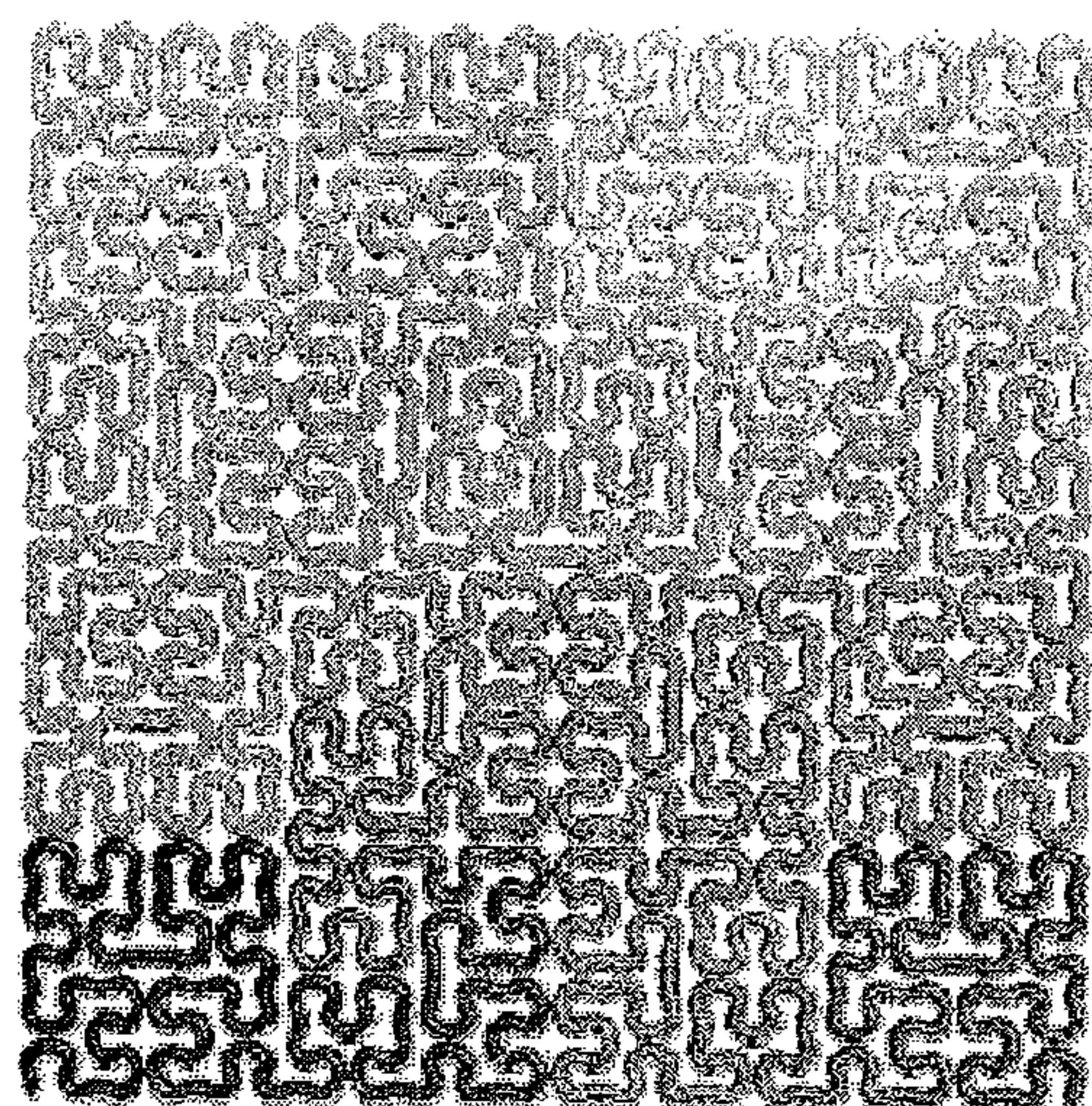
Peano Curve
