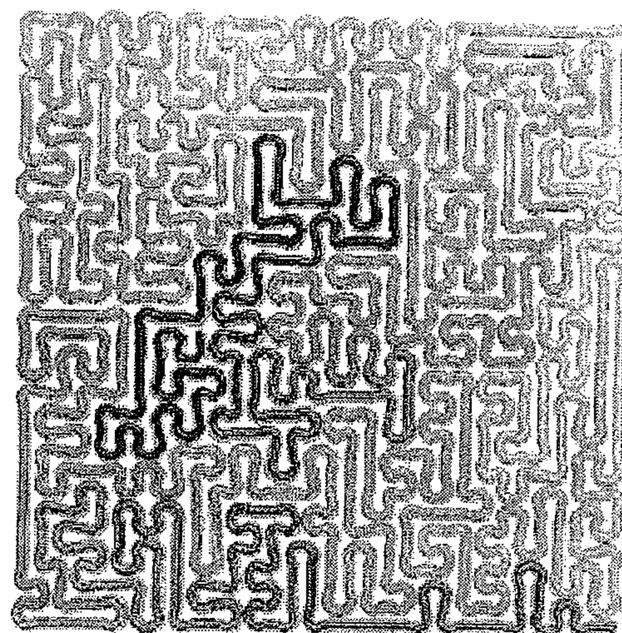
Hamiltonian Path
