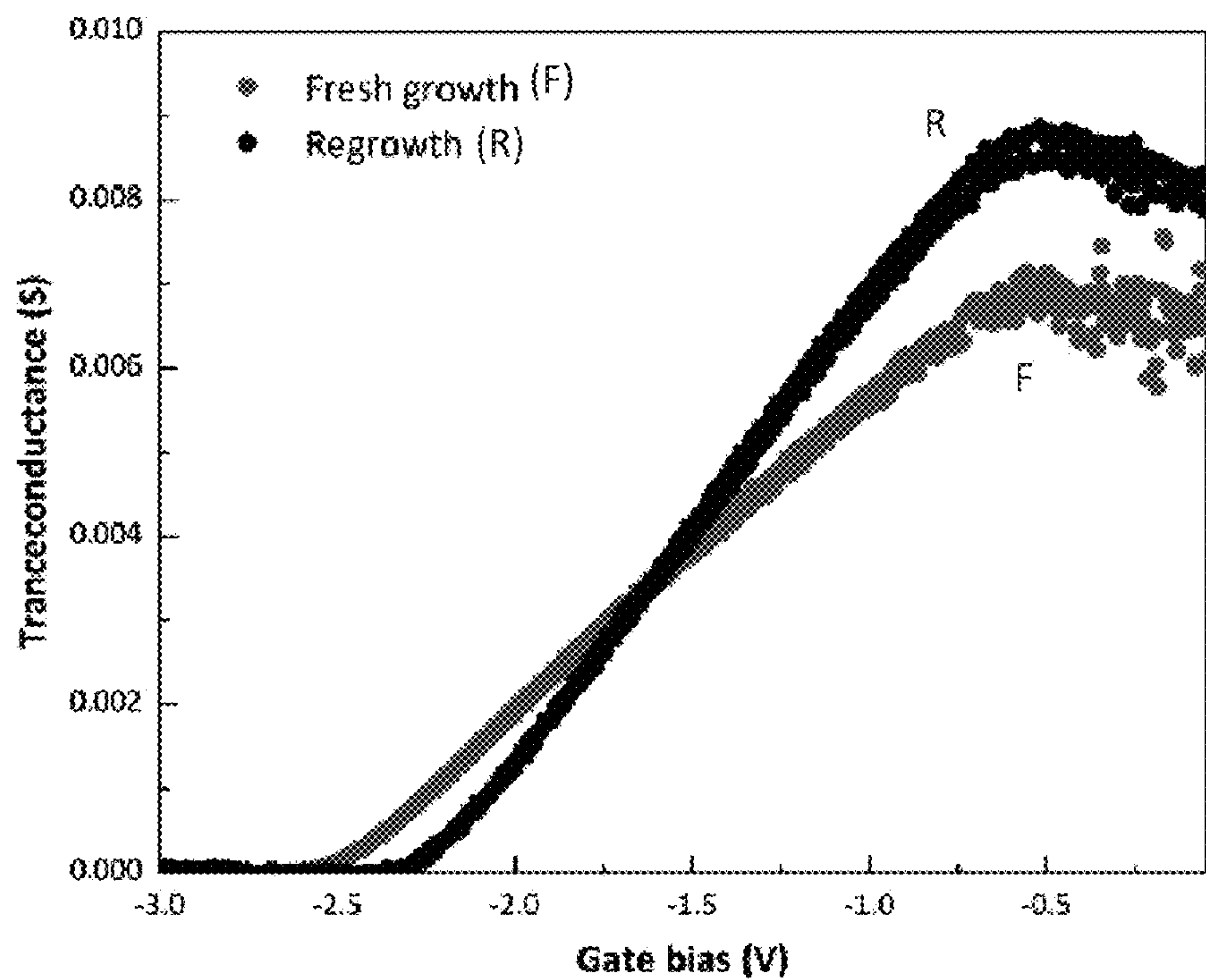
Gate bias (V) FIG. 19
