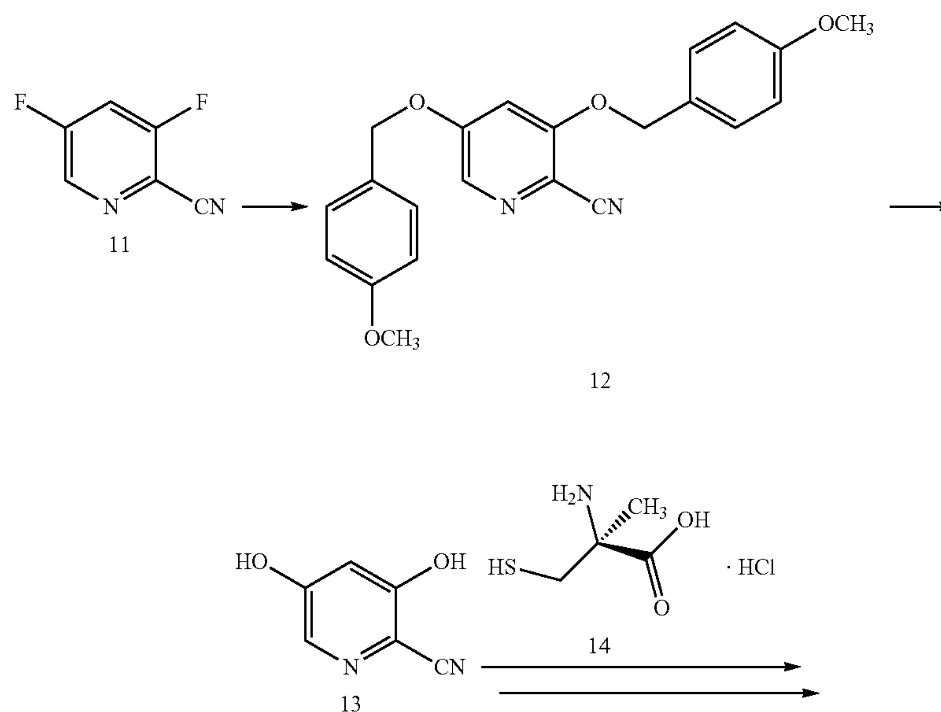
Scheme 1. Exemplary synthesis of I-1 and I-2.
