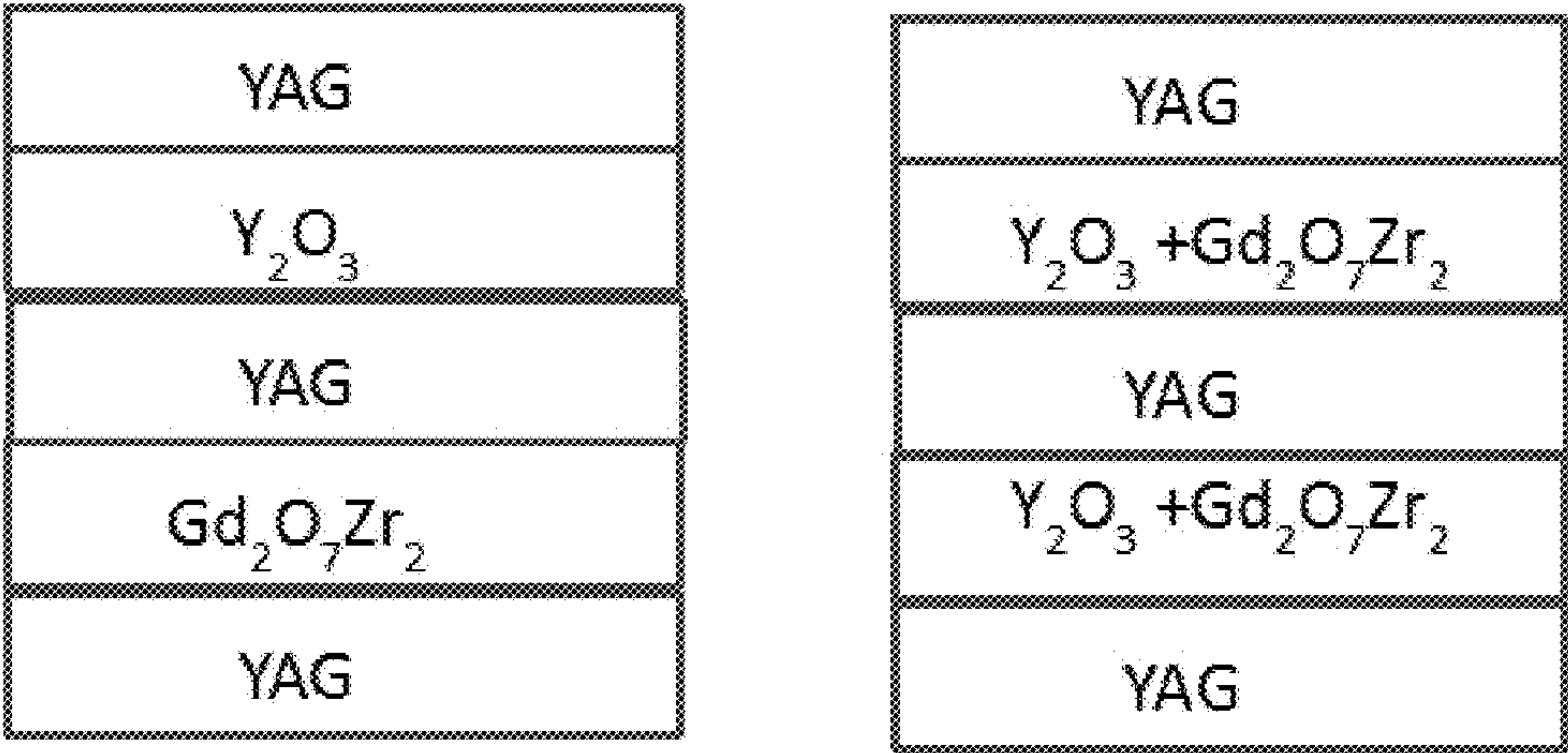
A- three component microstructure having layers of alternating materials
