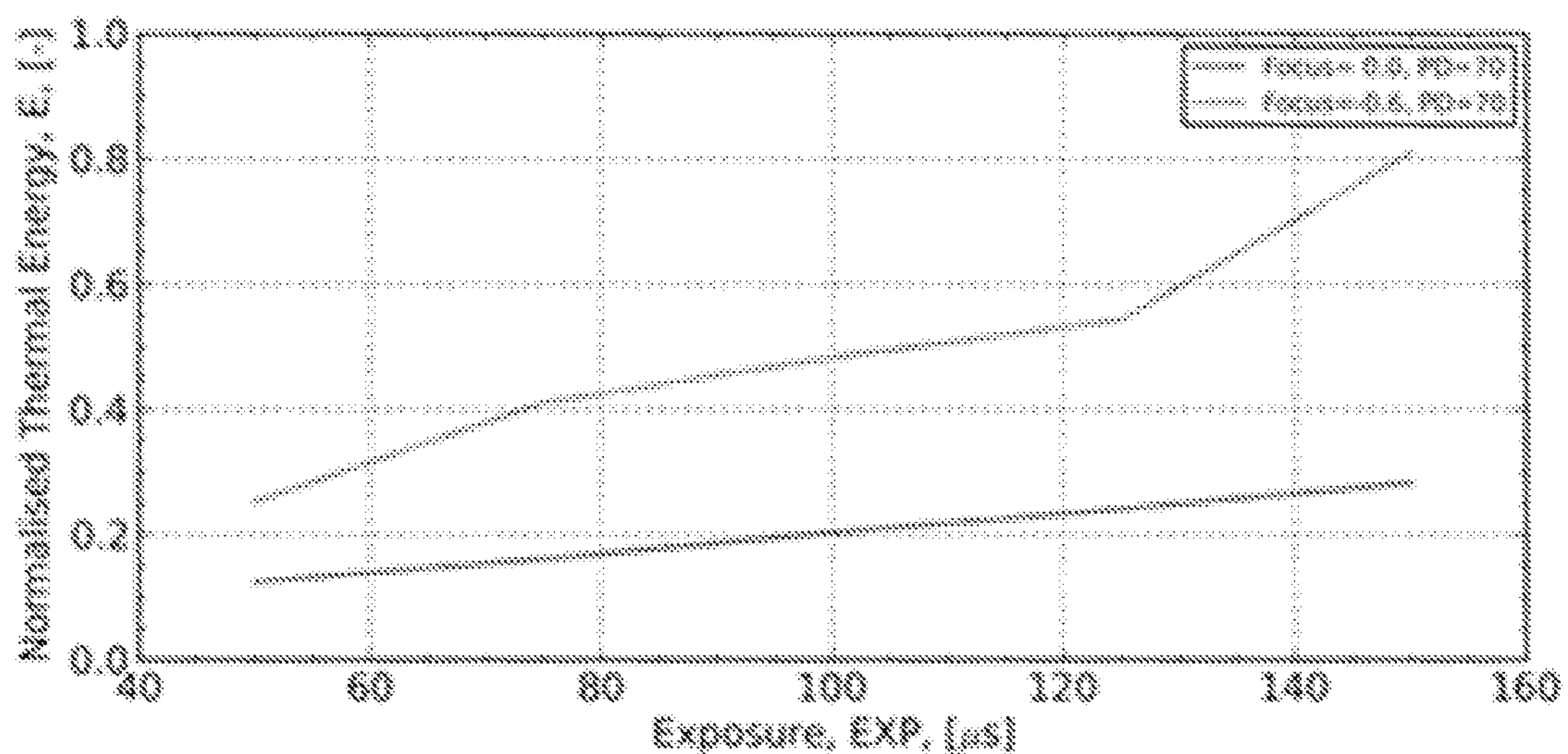
Thermal energy emitted for varying exposure length
