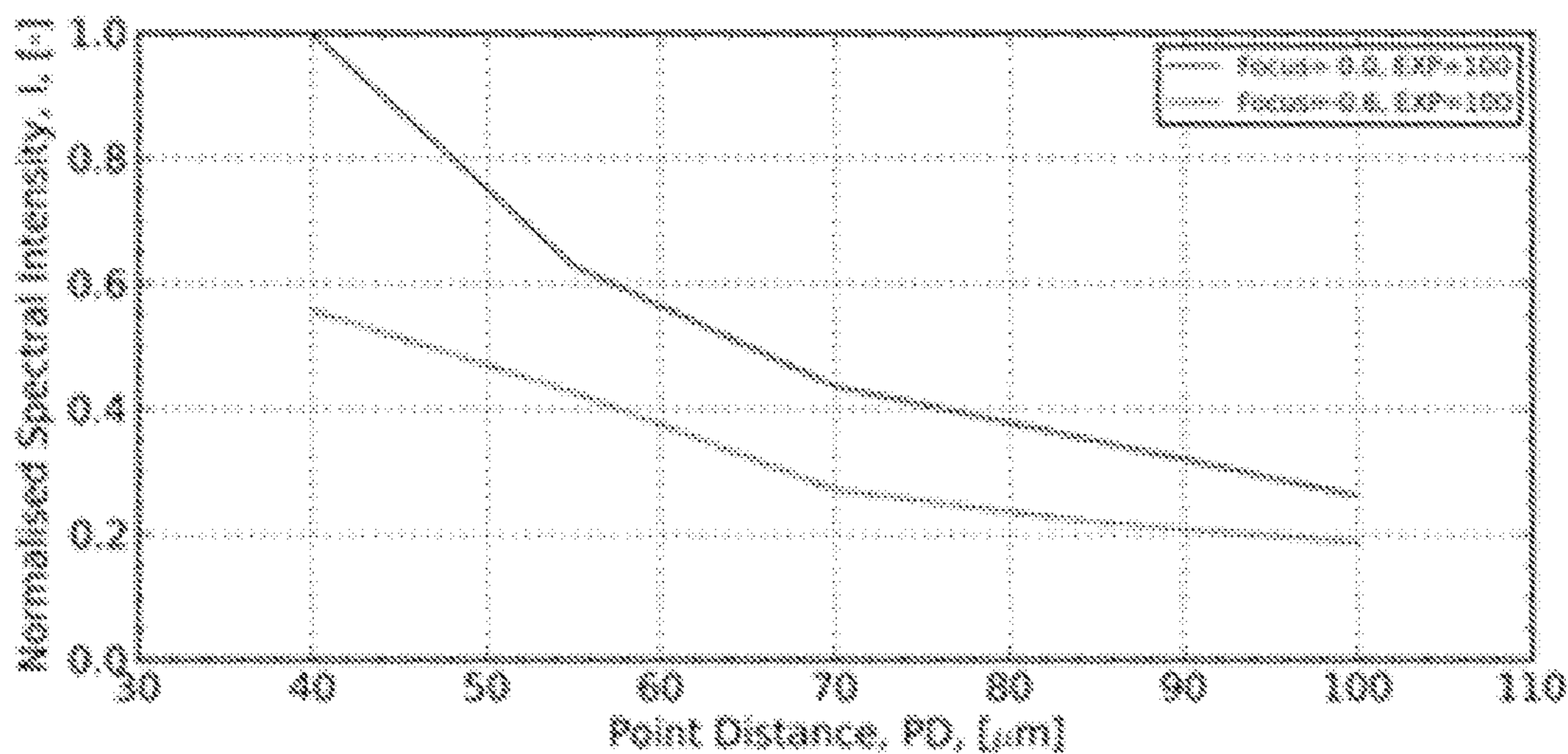
Spectral intensity for varying point distance
