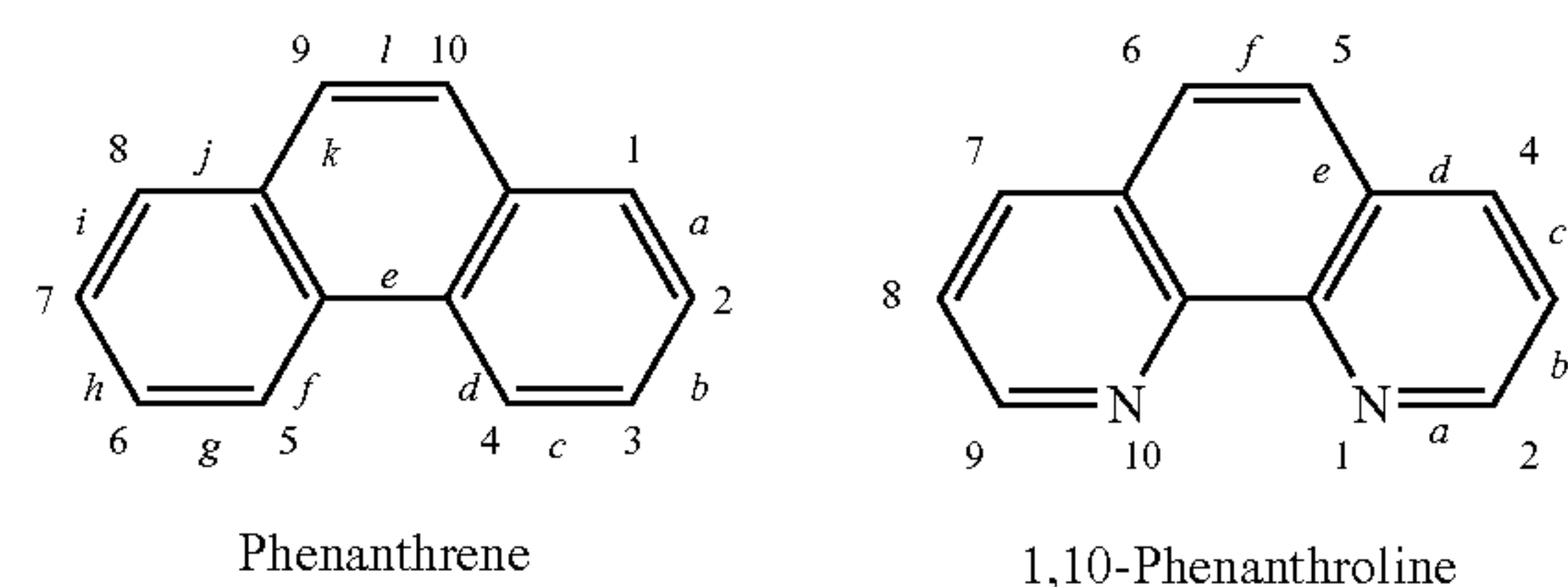
Scheme 1. Structures, atom labels, and ring-fused labels for phenanthrene and 1,10-phenanthroline.
