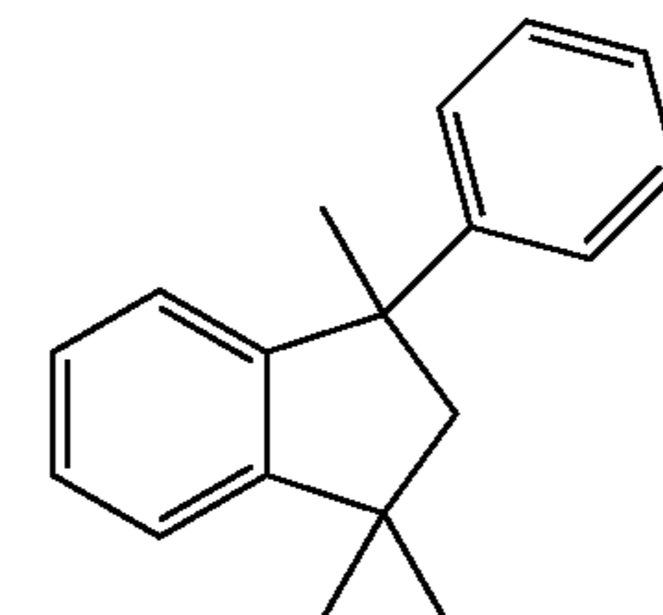
1-Phenyl-1,3,3-trimethylindane
