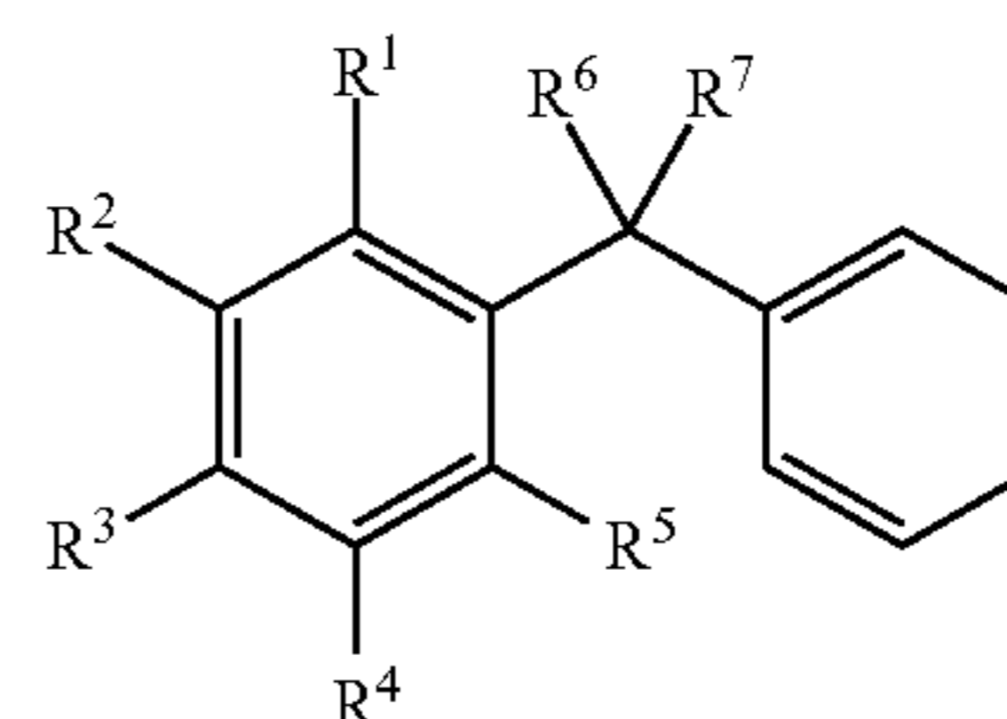
[Chem. 1]
