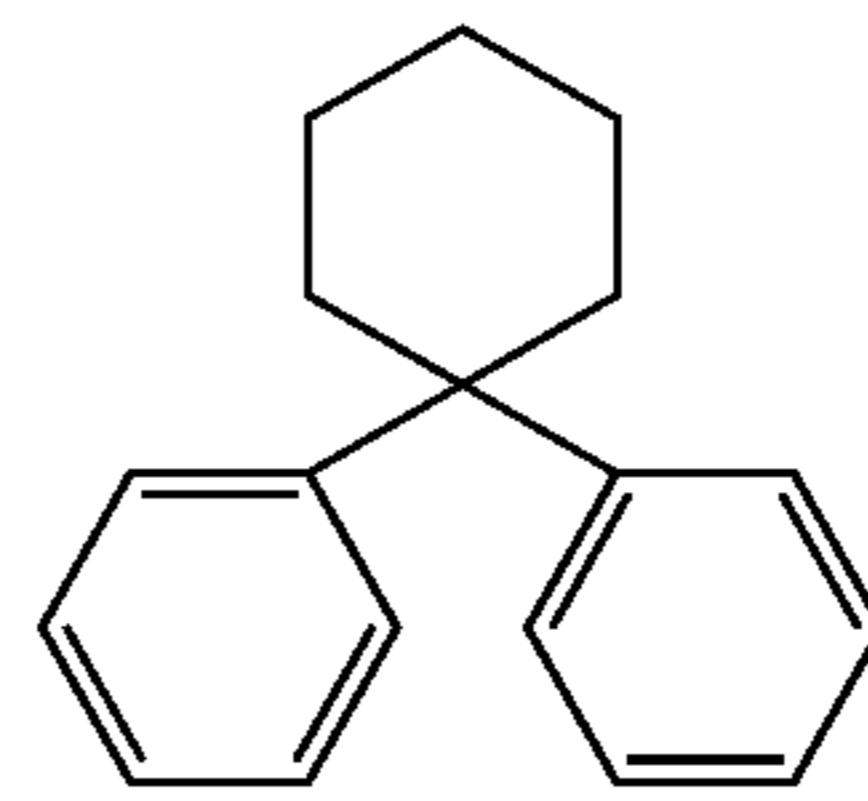
Diphenylcyclohexane
