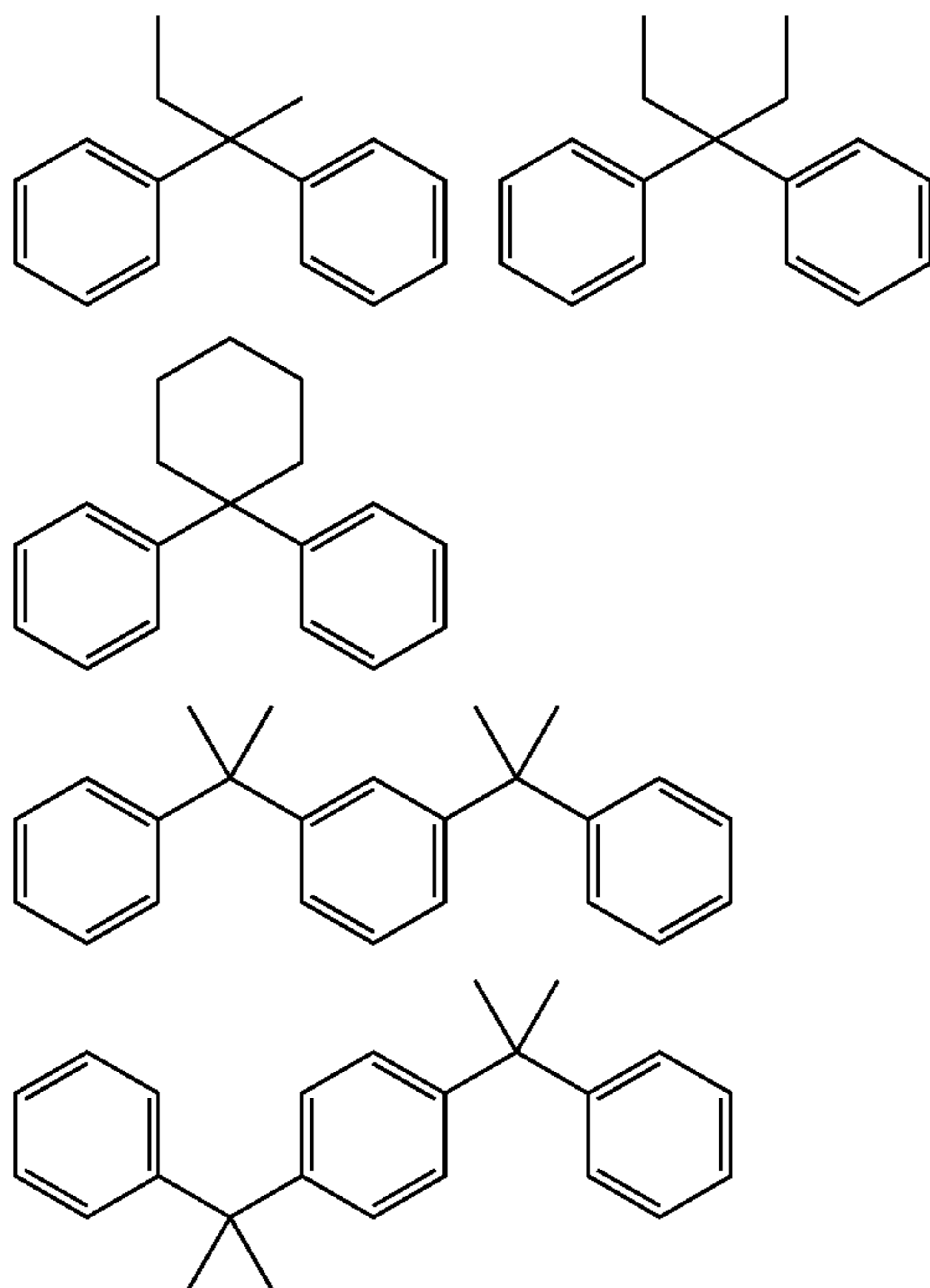
[Chem. 9]
