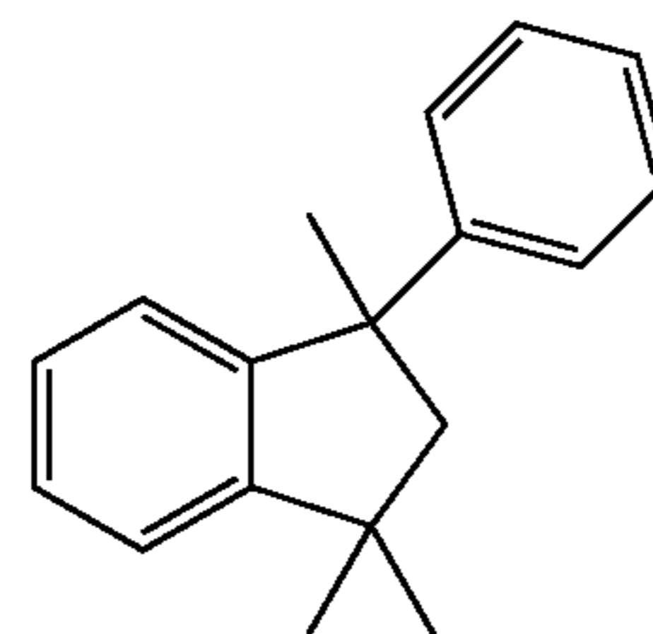
[Chem. 11]
