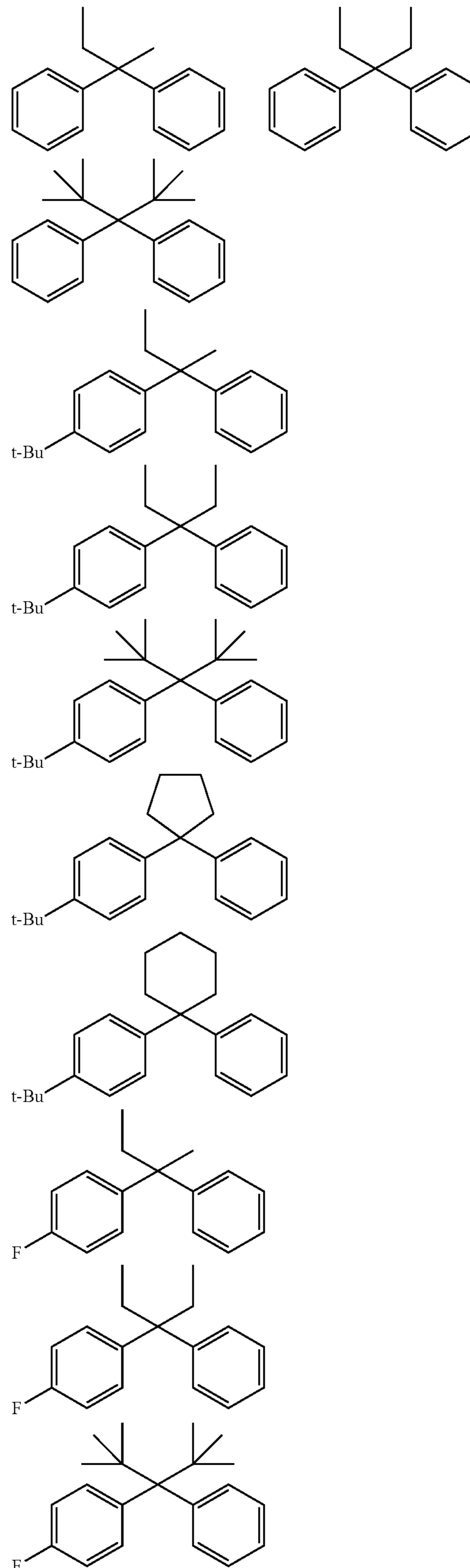
[Chem. 7]
