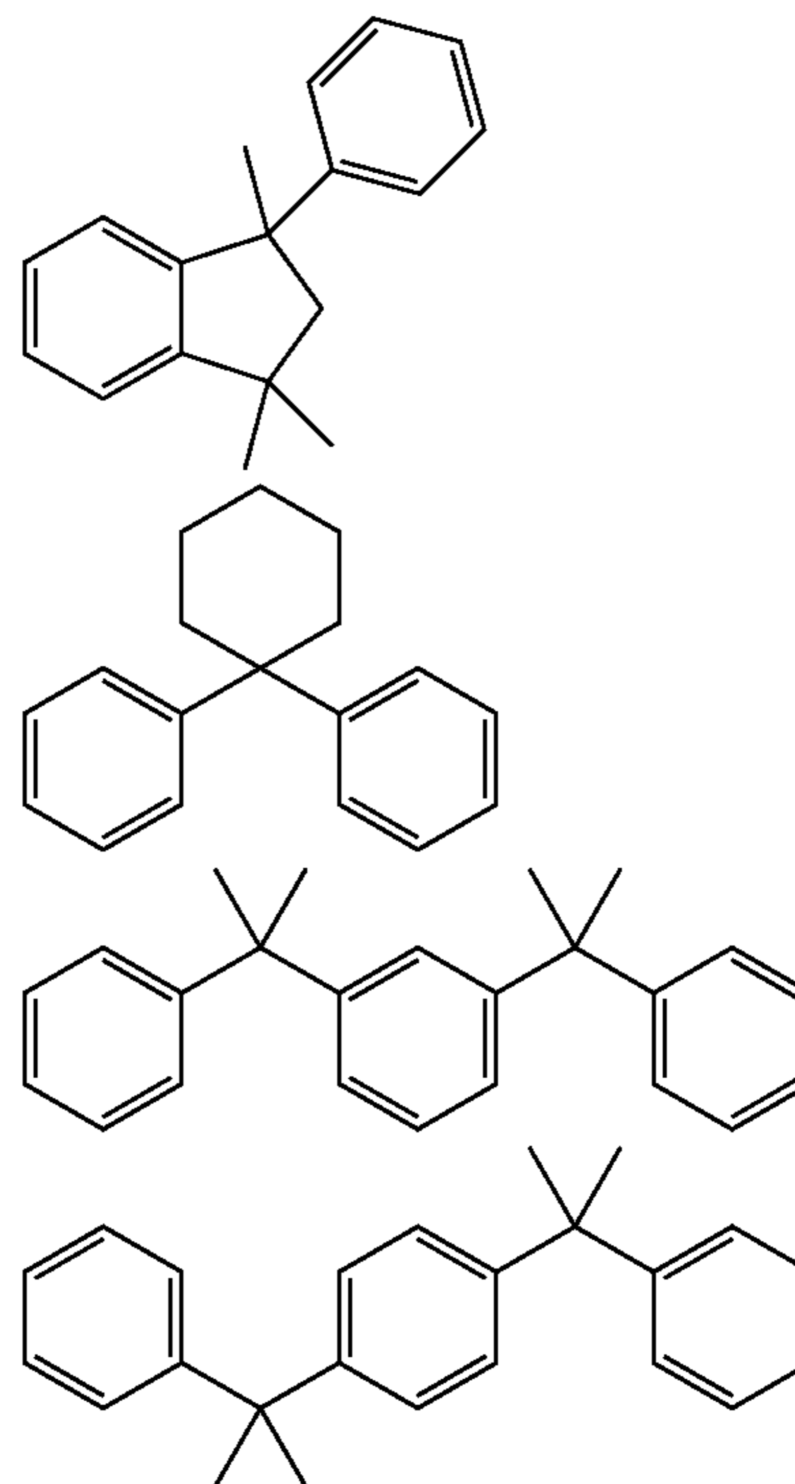
[Chem. 10]
