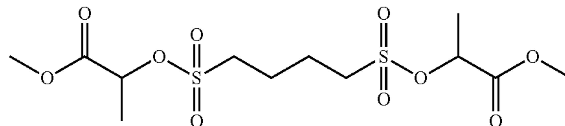
1-Methoxycarbonyl ethyl 1,4-butanedisulfonate
