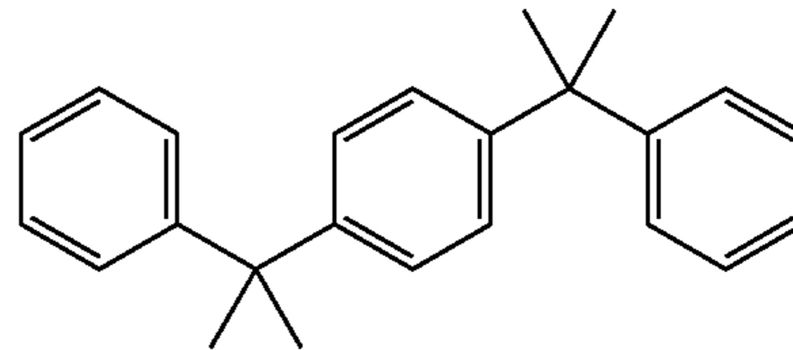
1,4-Bis(1-methyl-1-phenylethyl)-benzene
