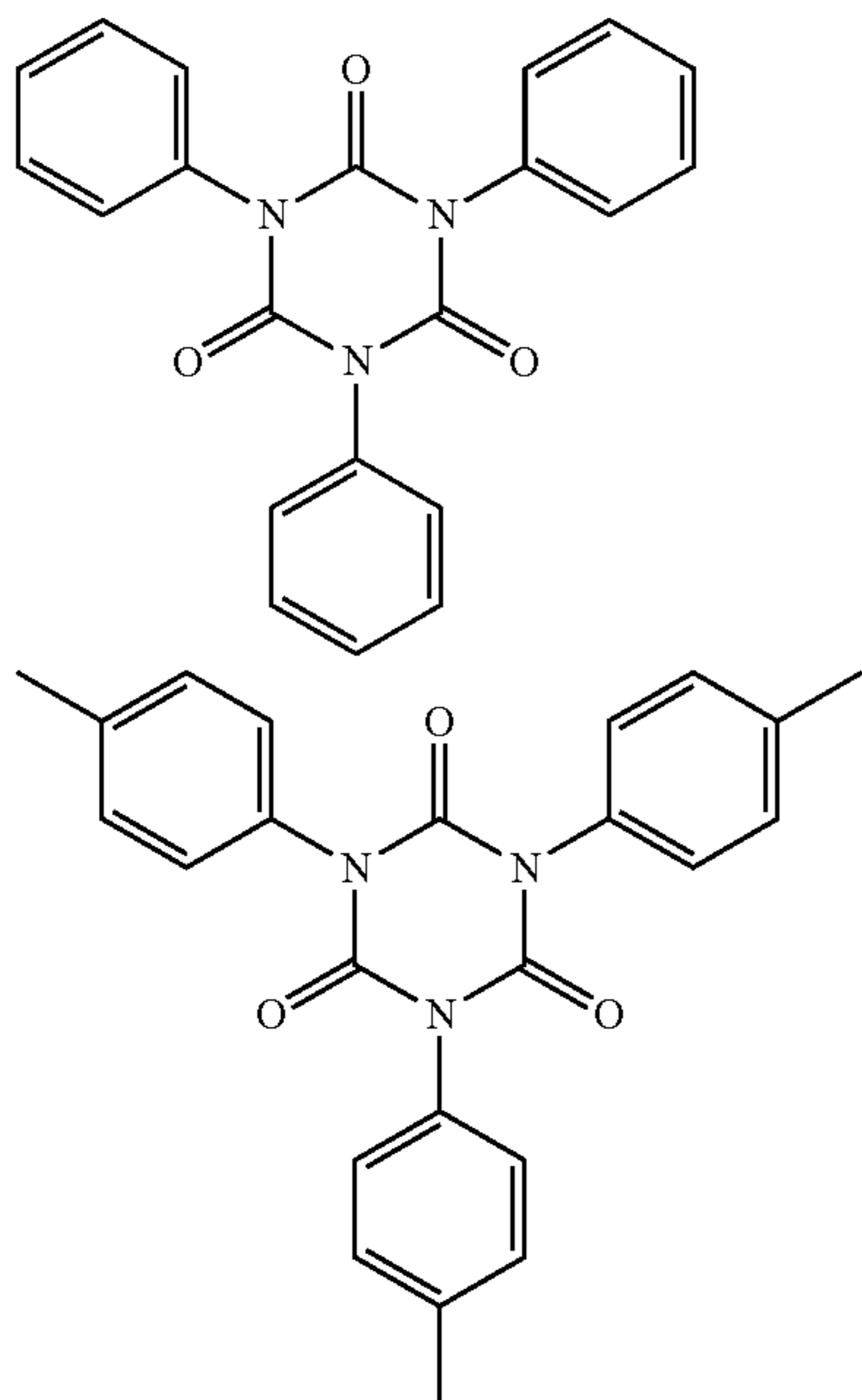
[Chem. 28]
