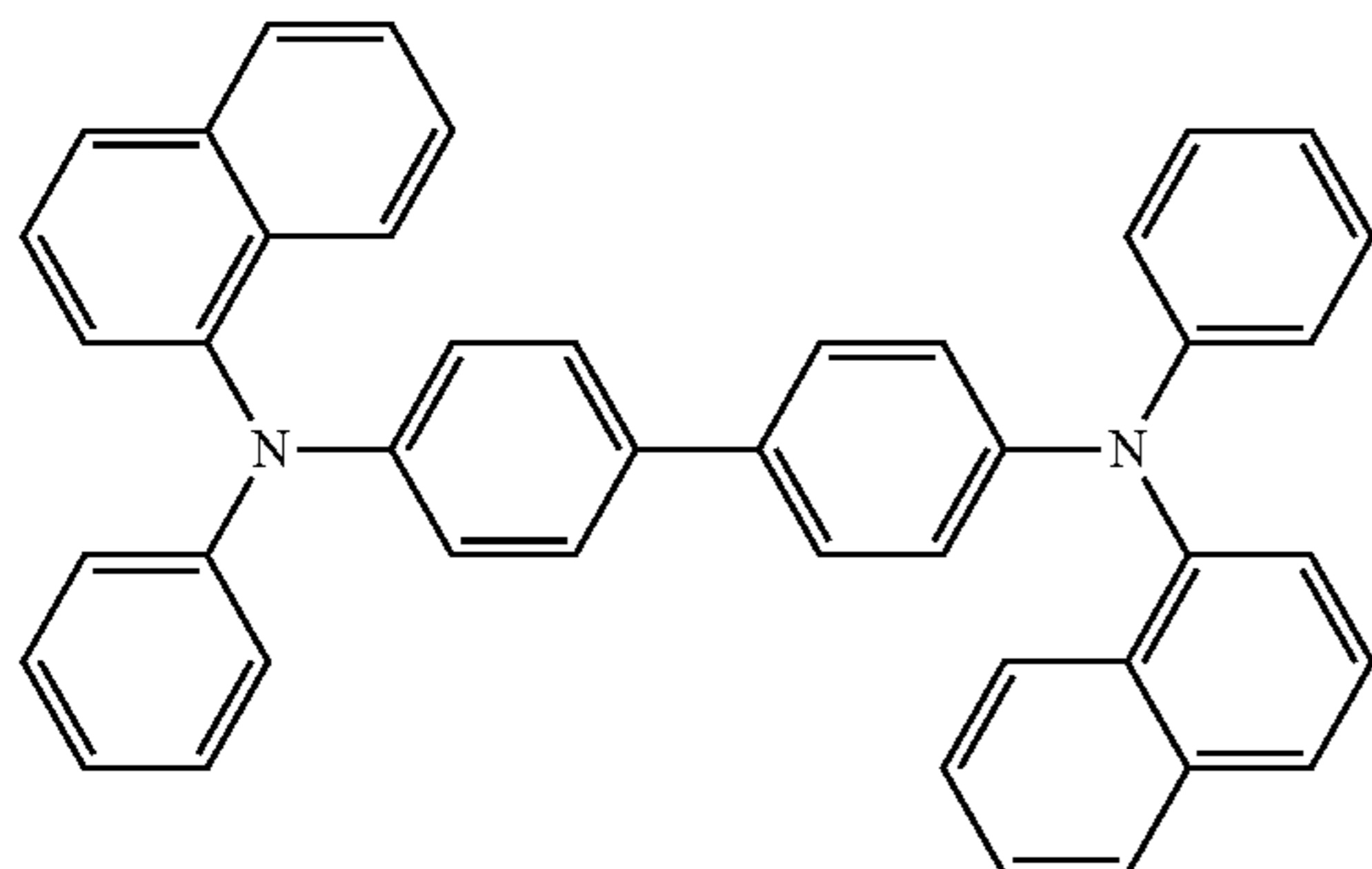
Compound A
