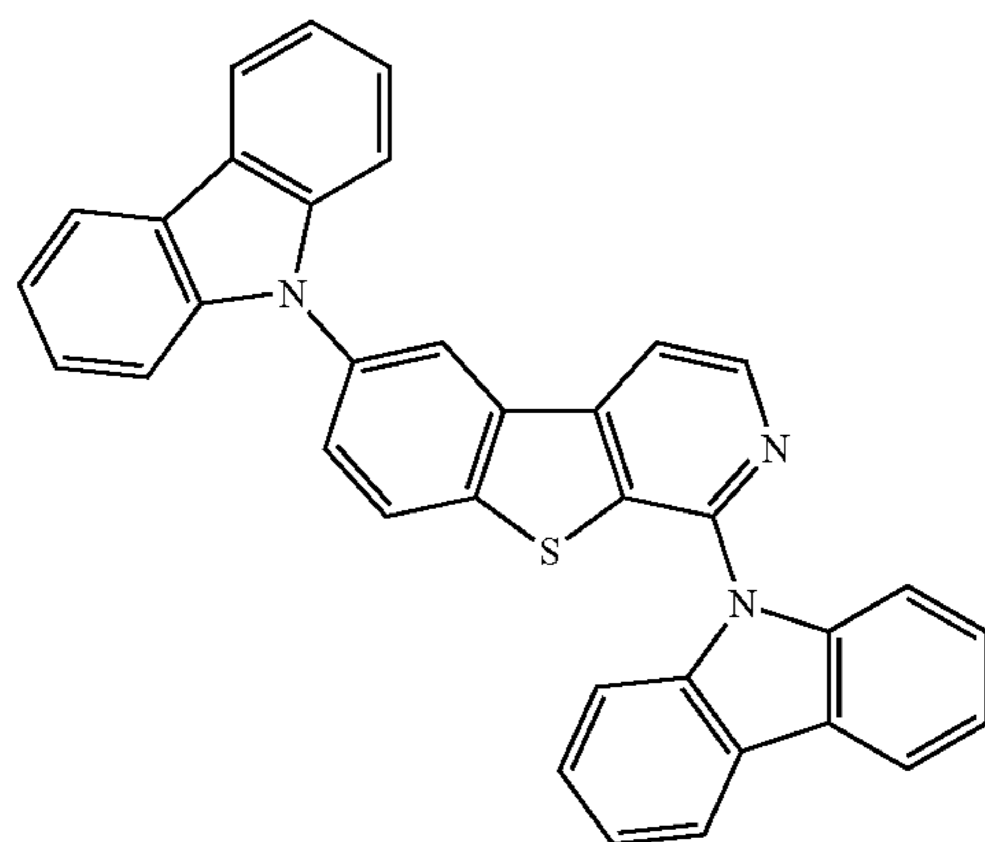
Compound D
