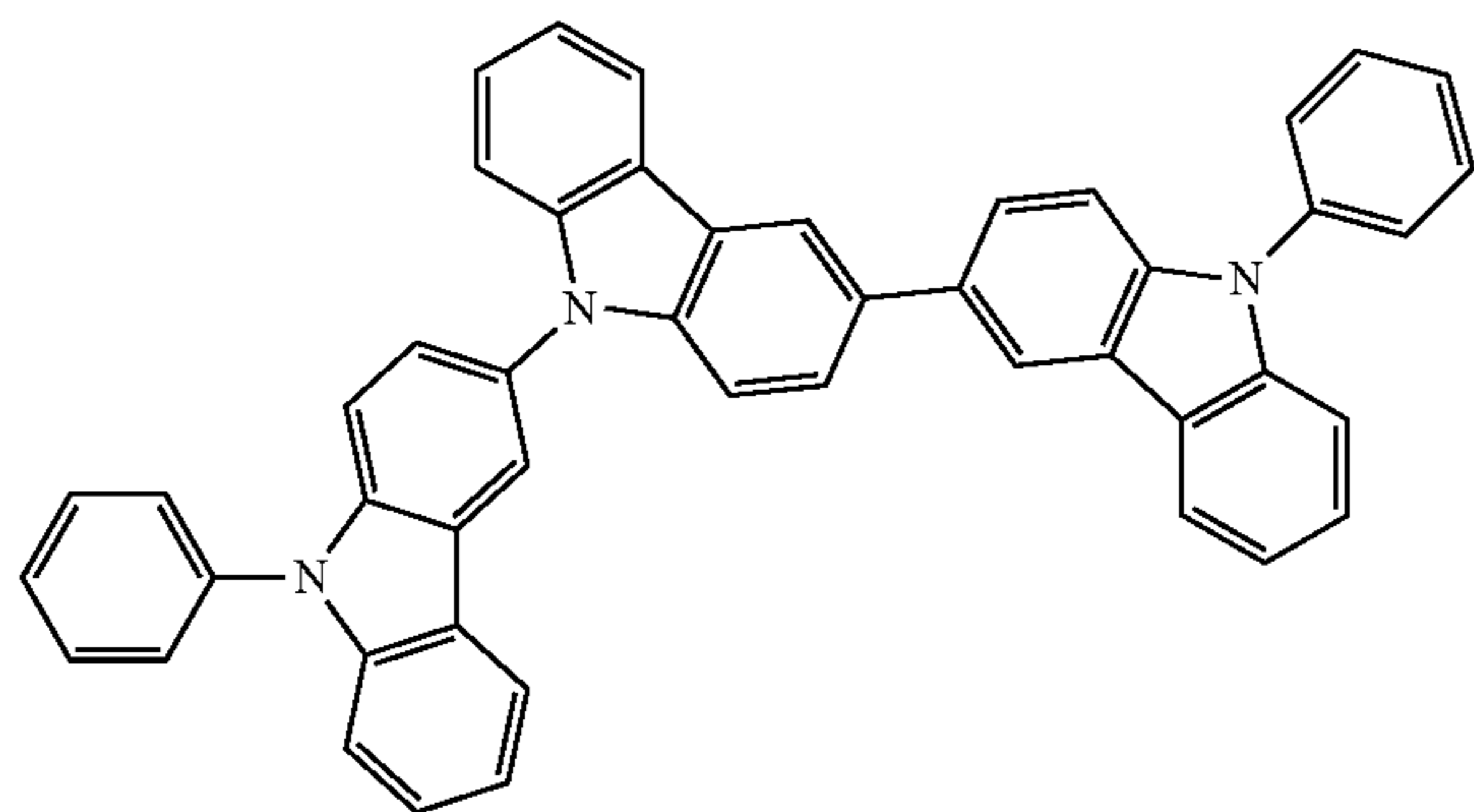
Compound B
