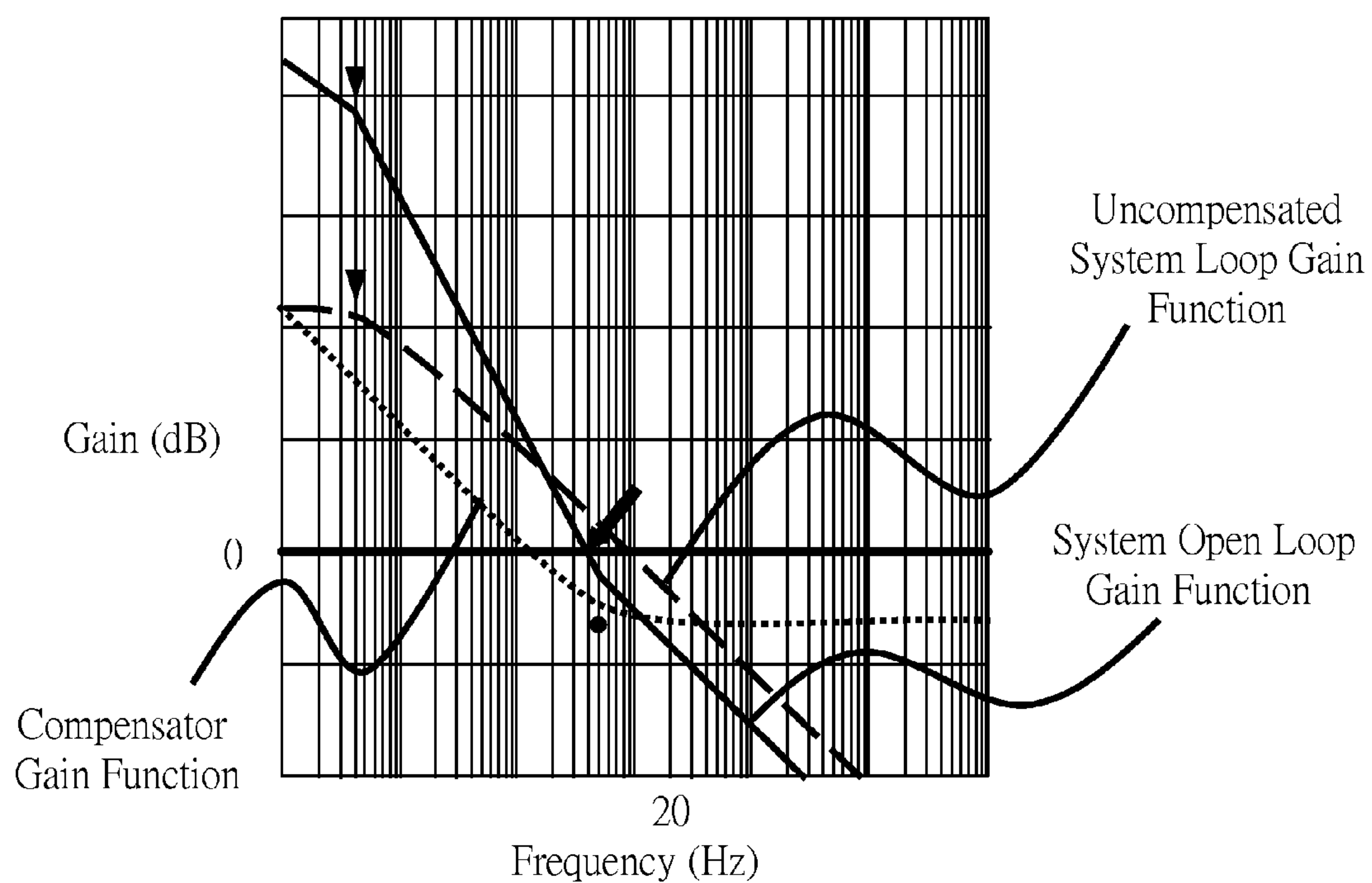
Fig. 6 (Prior Art)
