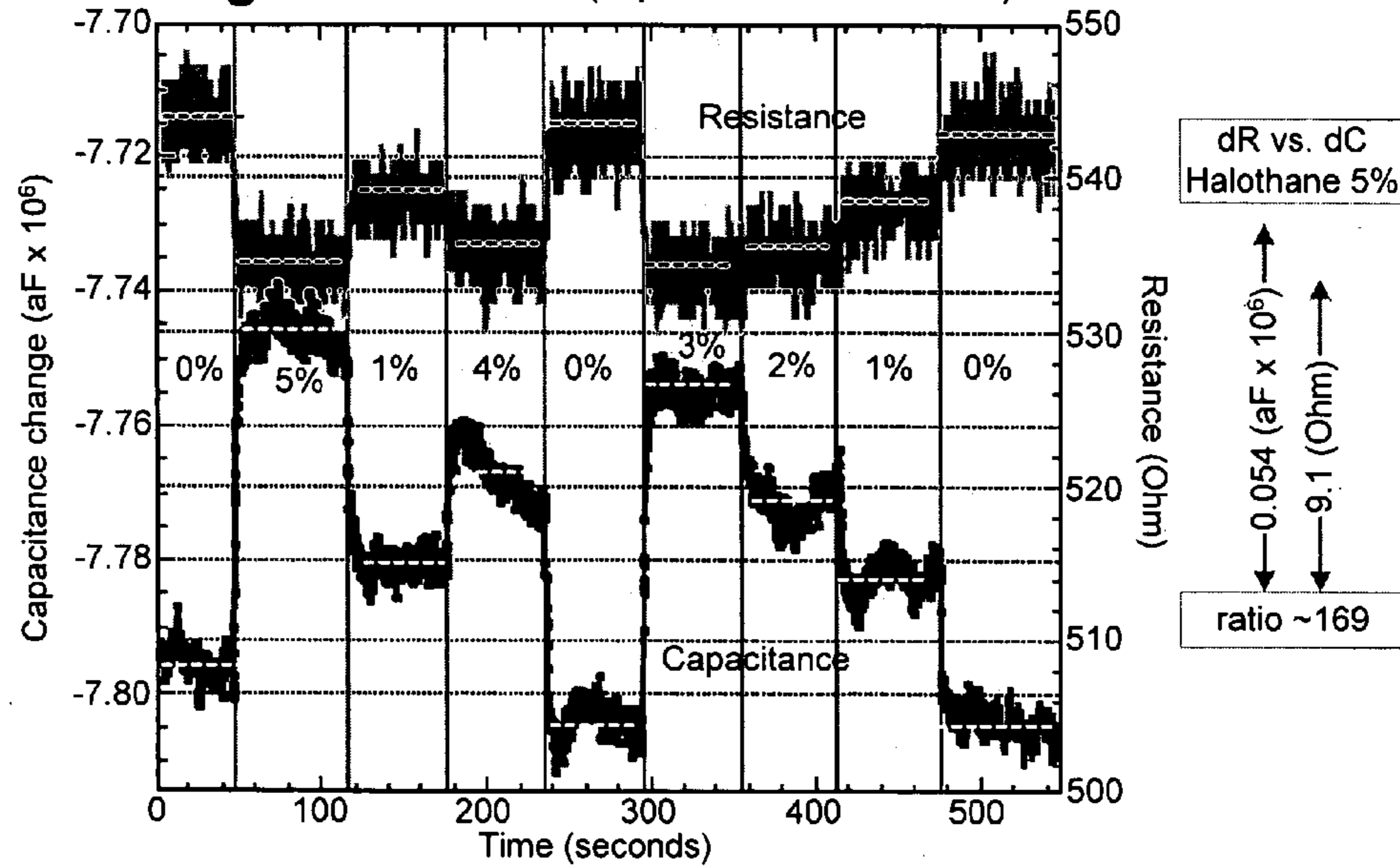
Fig. 5B - Halothane (capcintance & resistance)
