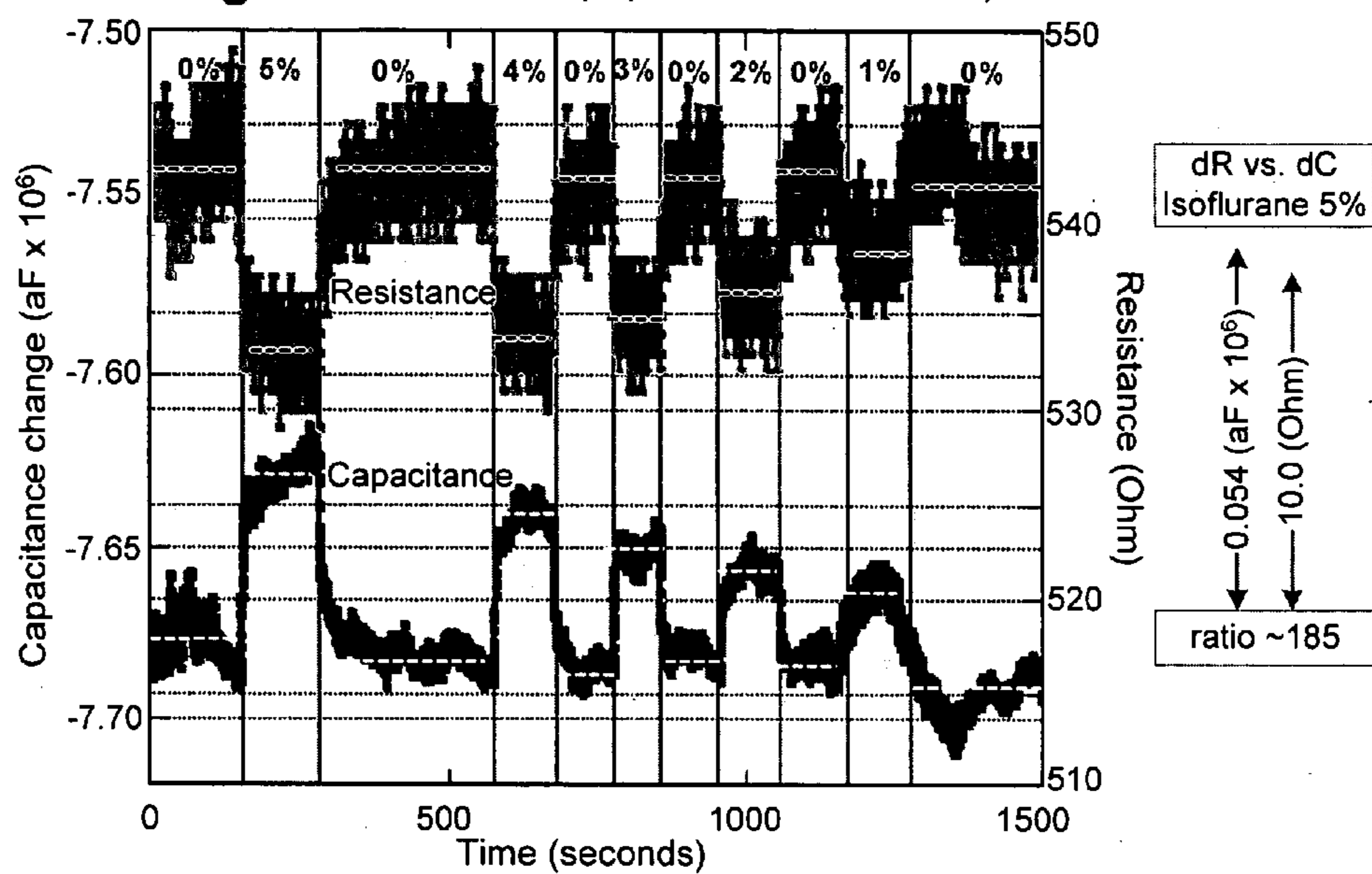
Fig. 5A - Isoflurane (capcintance & resistance)
