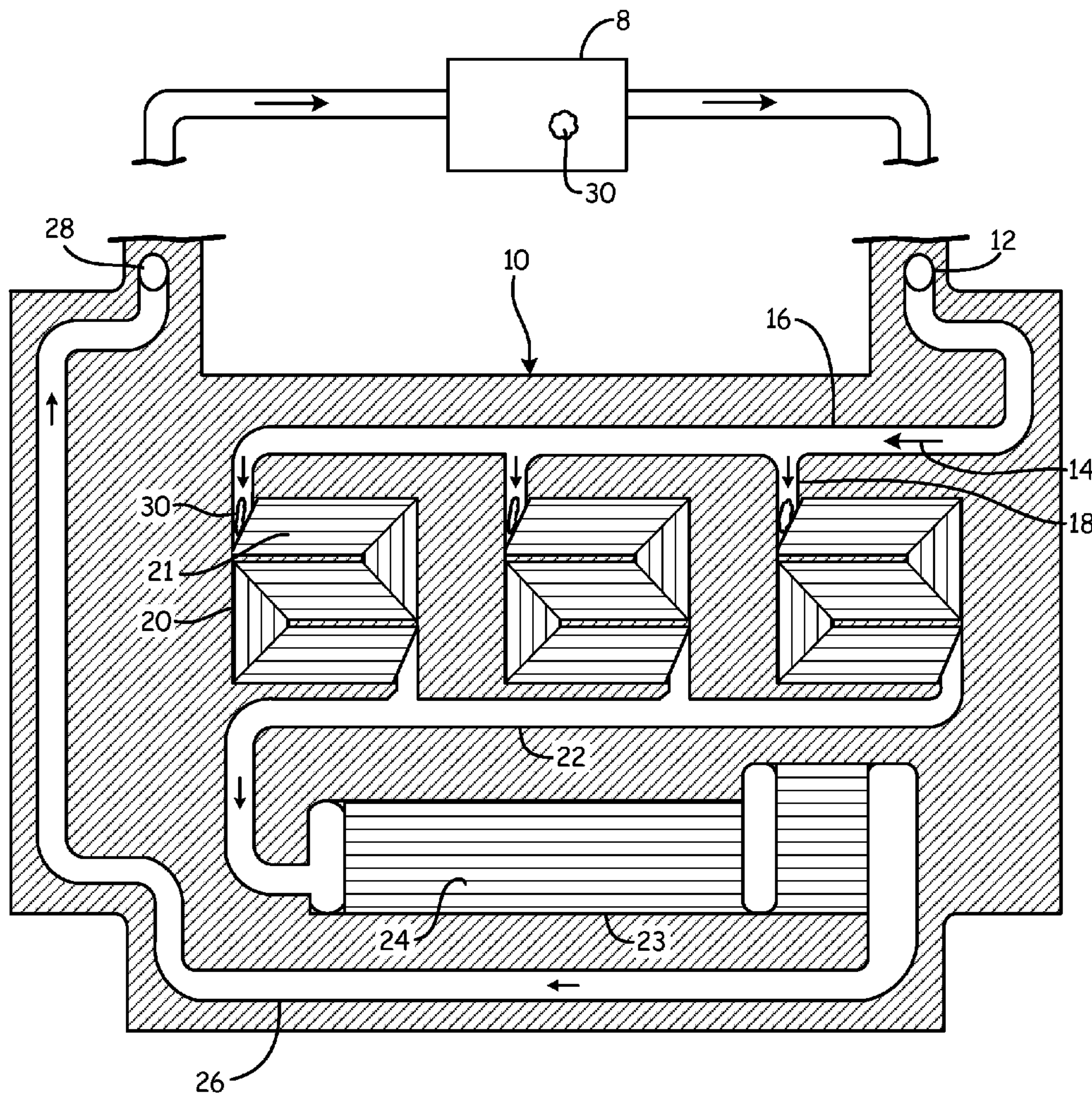
Fig. 1 PRIOR ART
