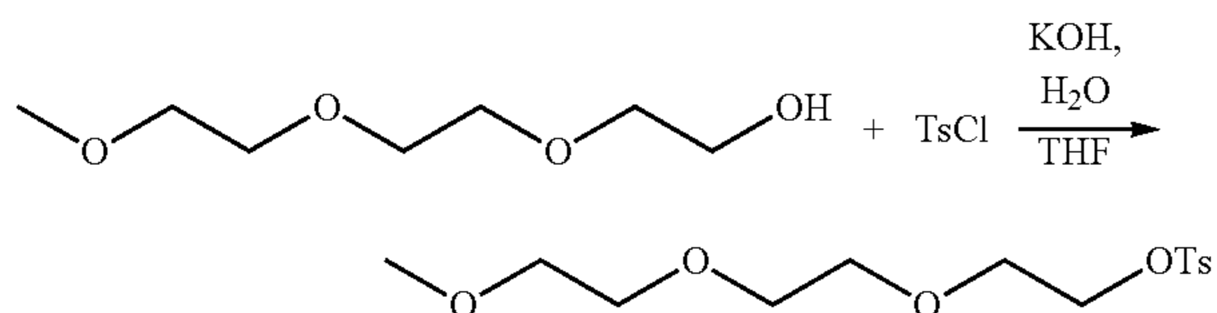
Scheme 1. Monomer synthesis
