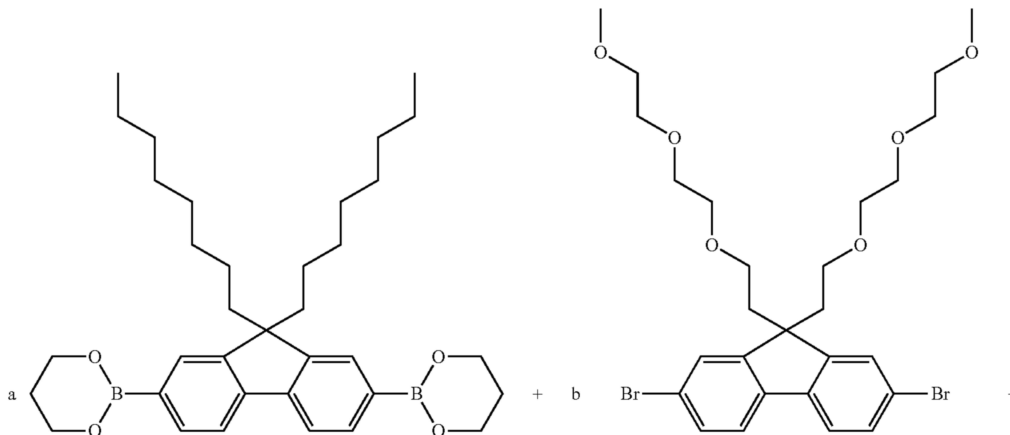
Scheme 4. Synthesis of PFPFOFOMB and PFPFOFOBA process
