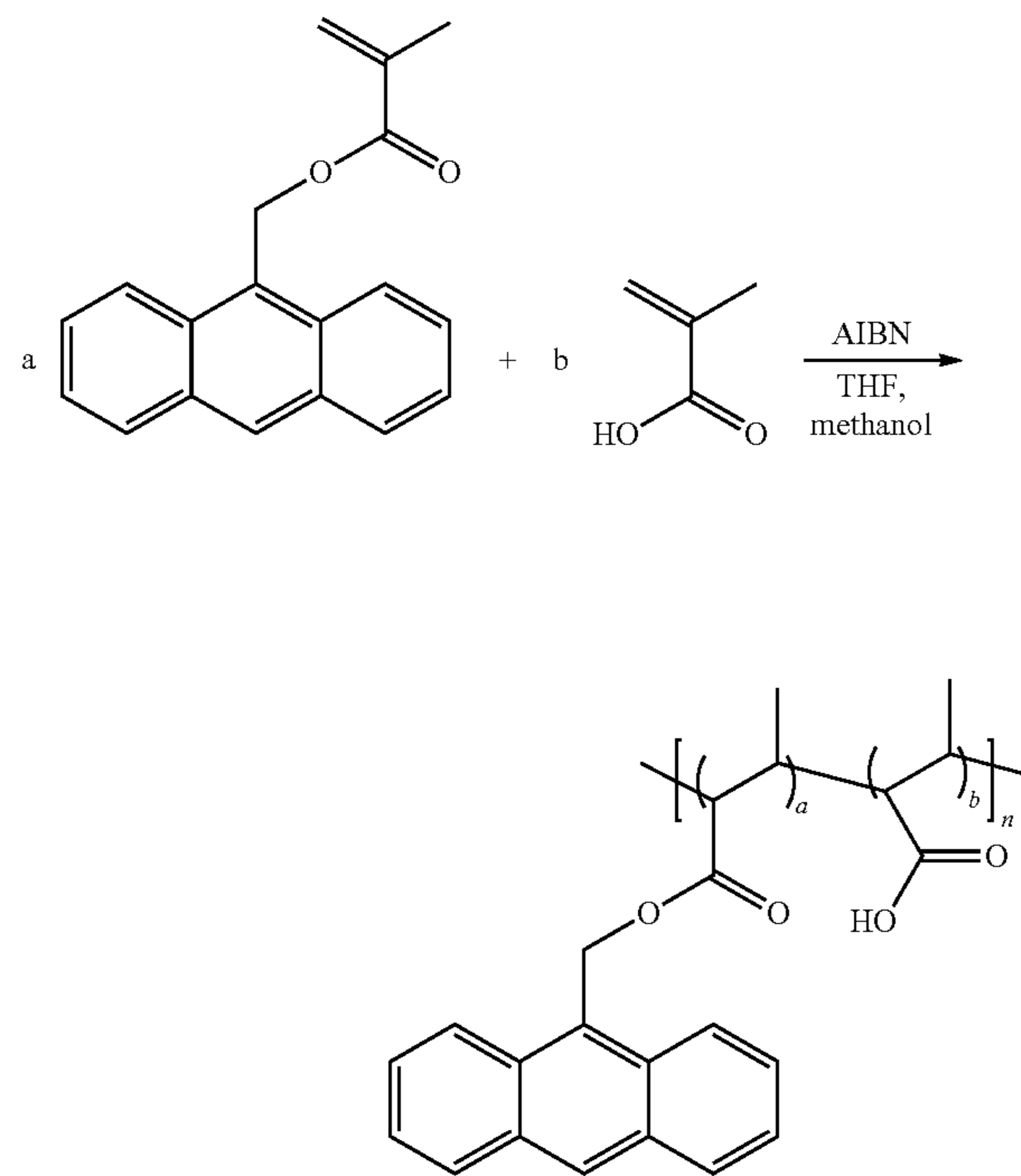
Scheme 5. Methacrylate anthracene and carboxylic acid polymer made by copolymerization process
