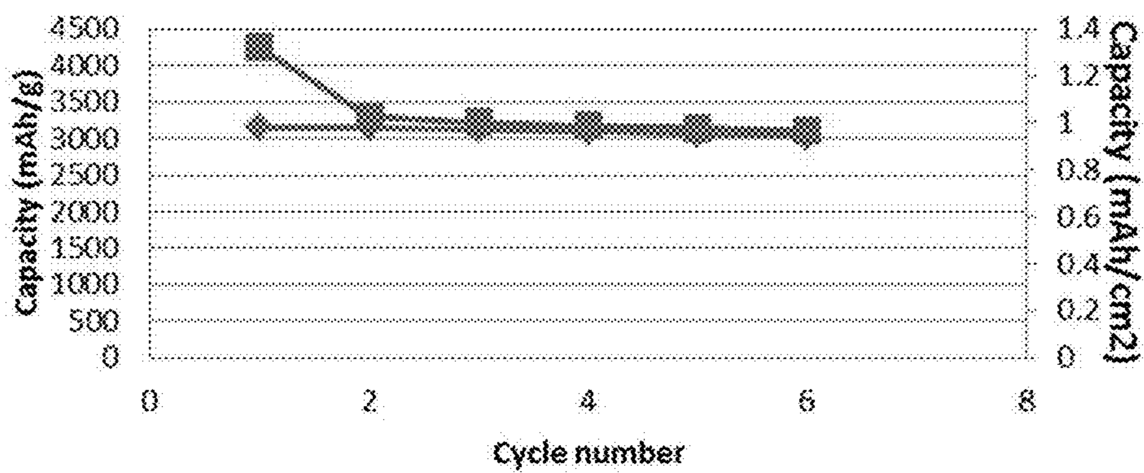
(a) Ant (5%):Si (95%) (0.31mg/cm 2 ) (Cycling rate: C/10)
