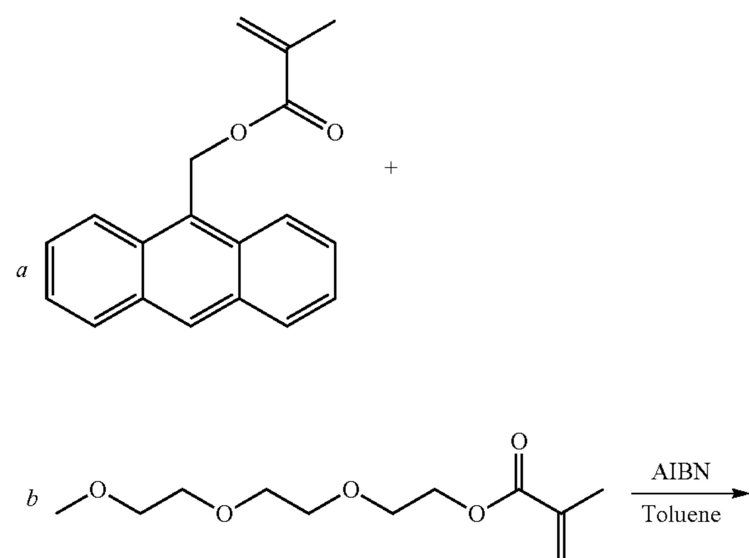
Scheme 6. Copolymer to include triethyleneoxide monomethylether branches
