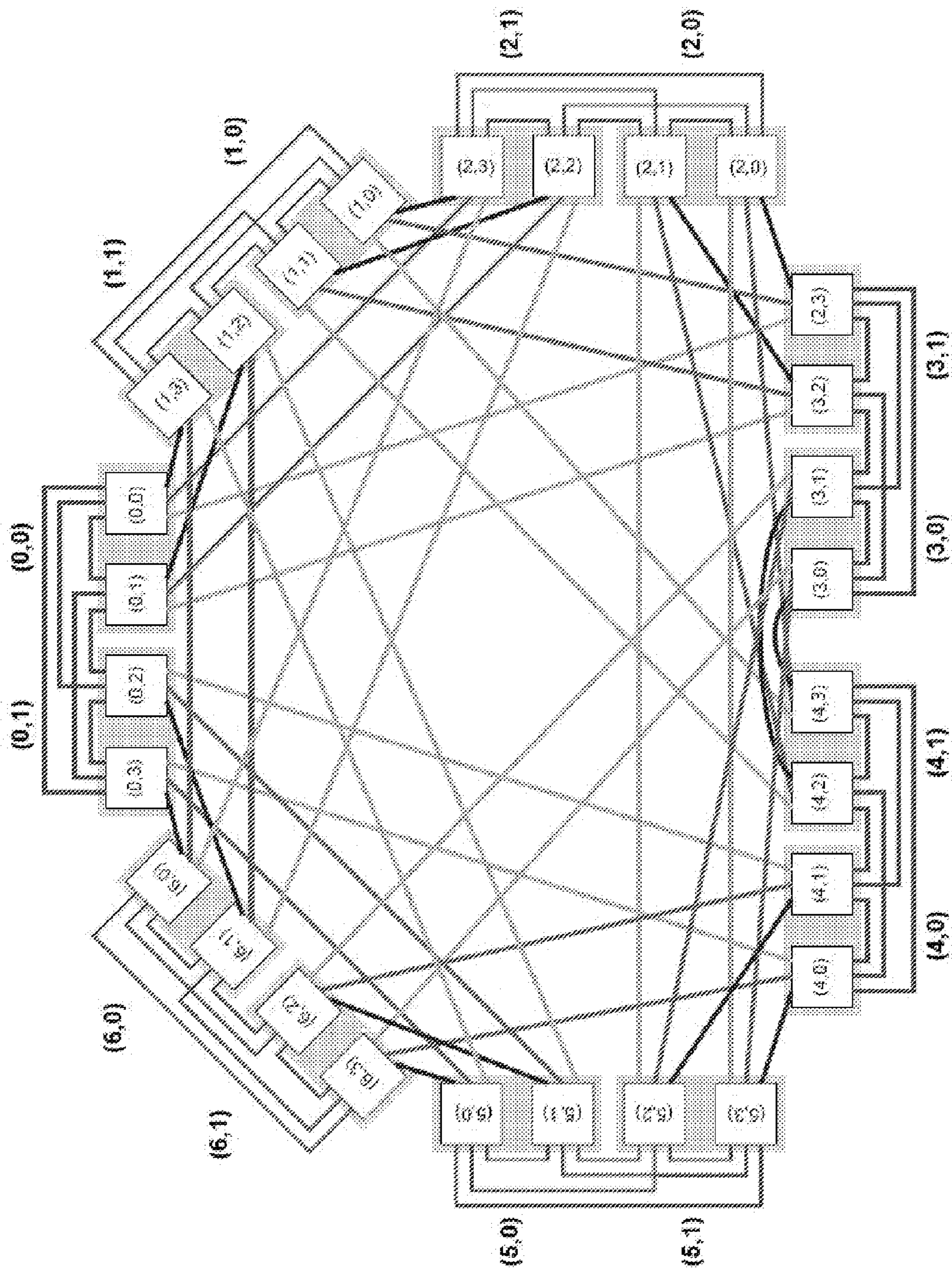
Figure 7 : EGDF( p; 3, 3; 1, 2 ).
