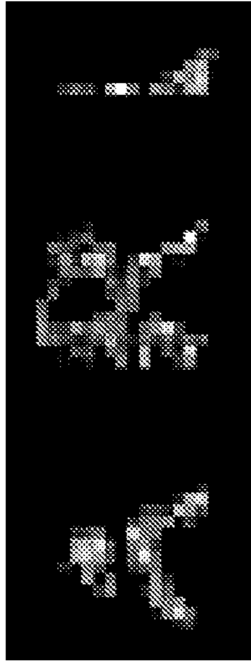
FIG. 12 Self Bucket G(2) GPSR with turbulence 10k Frames; Data normalized globally 0-1; tau=2.5e7; Tol=1e-6; NonZero=183
