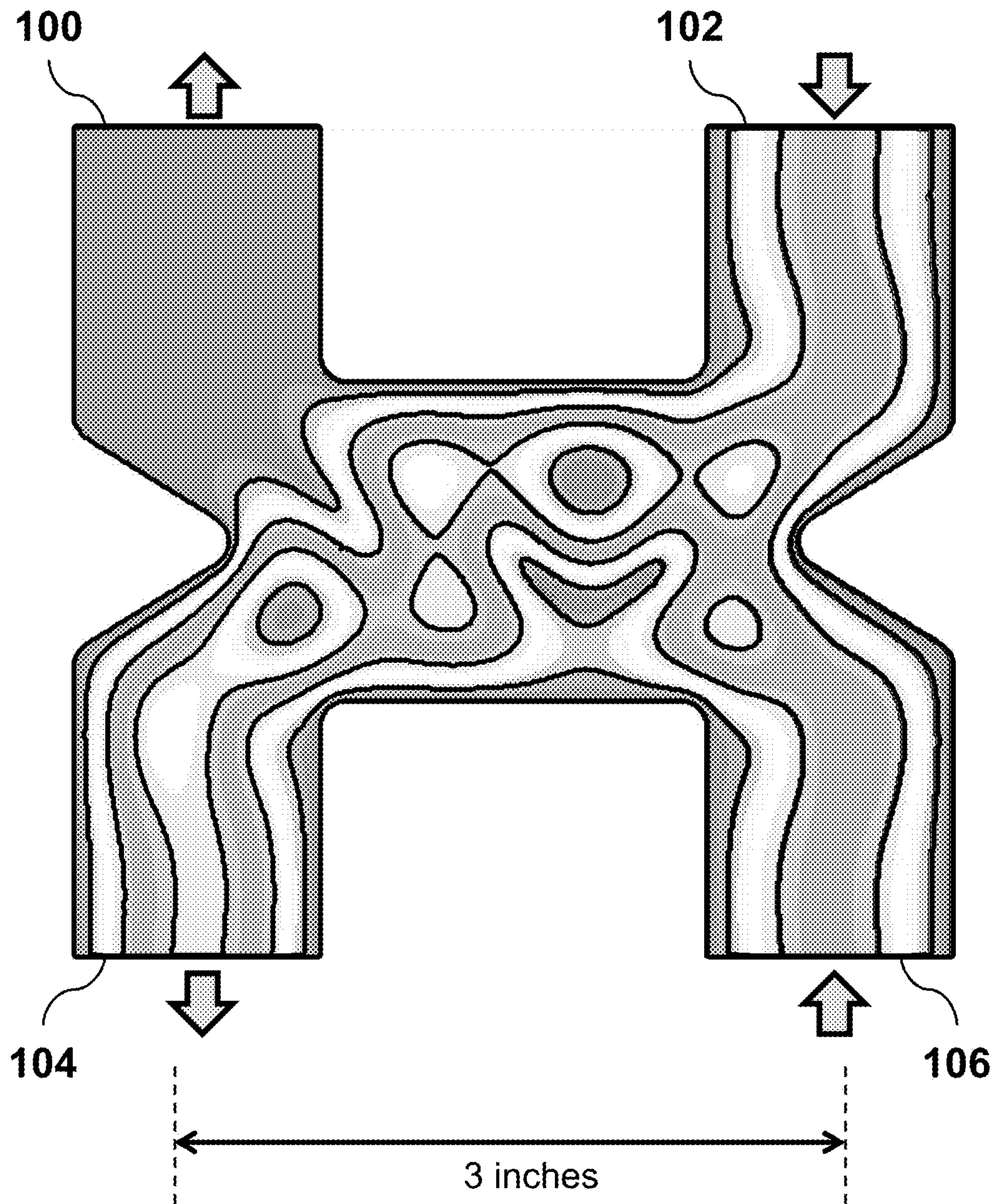
Fig. 1 (Prior Art)
