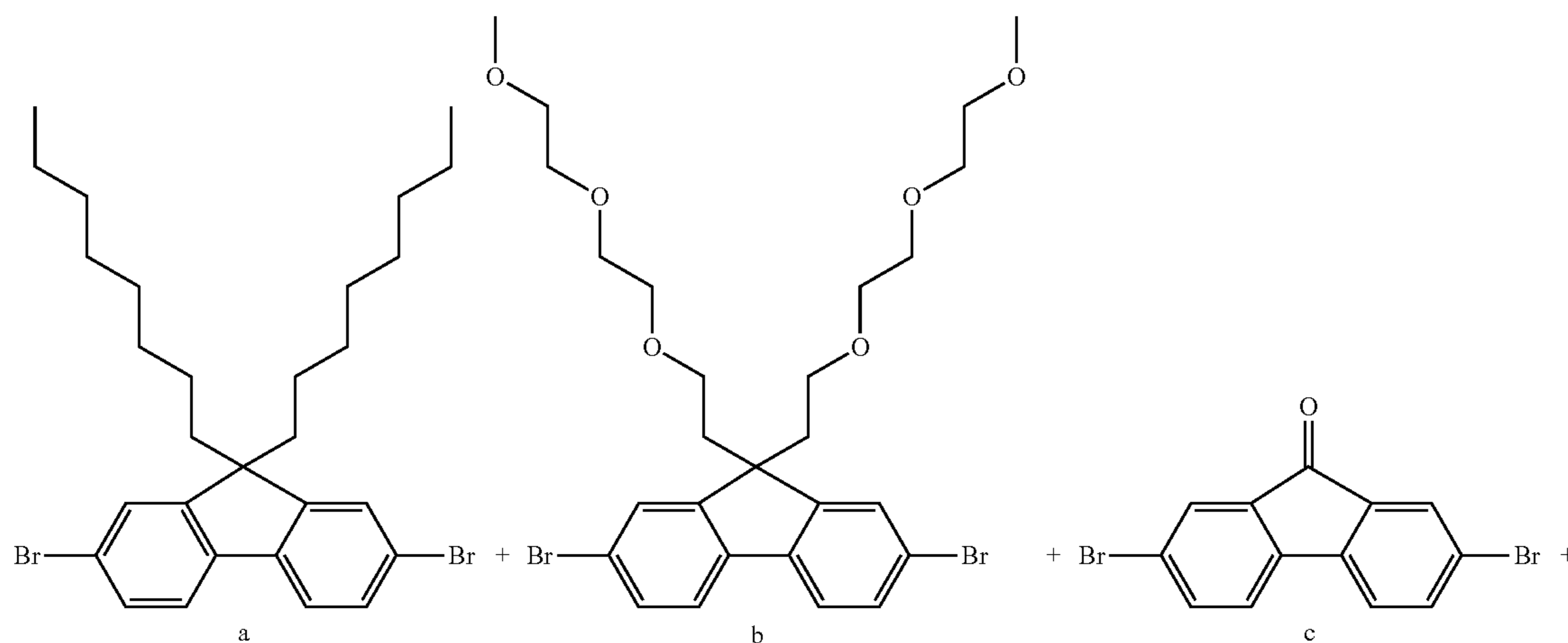
Scheme 5. An alternative synthesis process to make PFPFOFOMB and PFPFOFOBA
