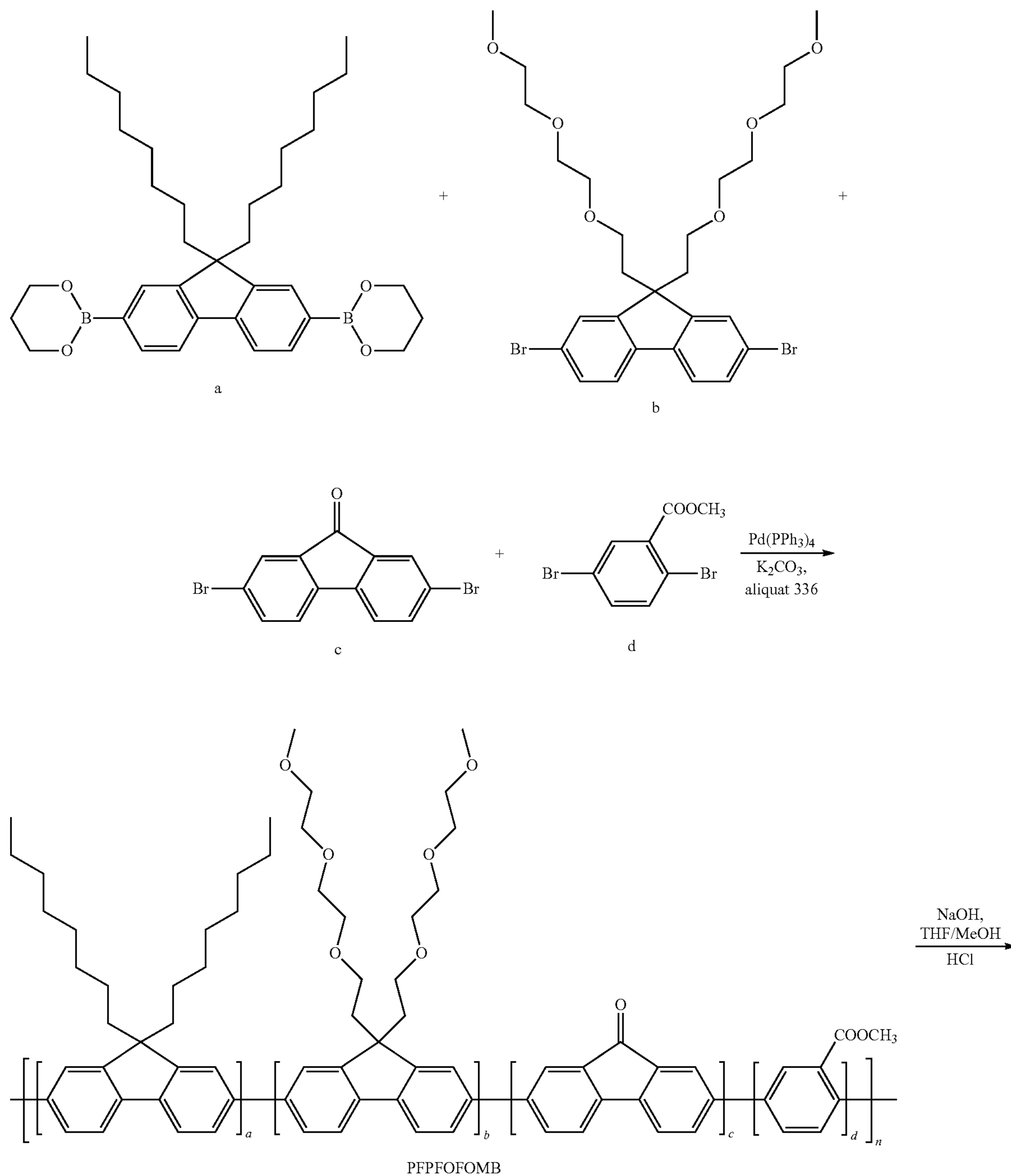
Scheme 4. Synthesis of PFPFOFOMB and PFPFOFOBA process
