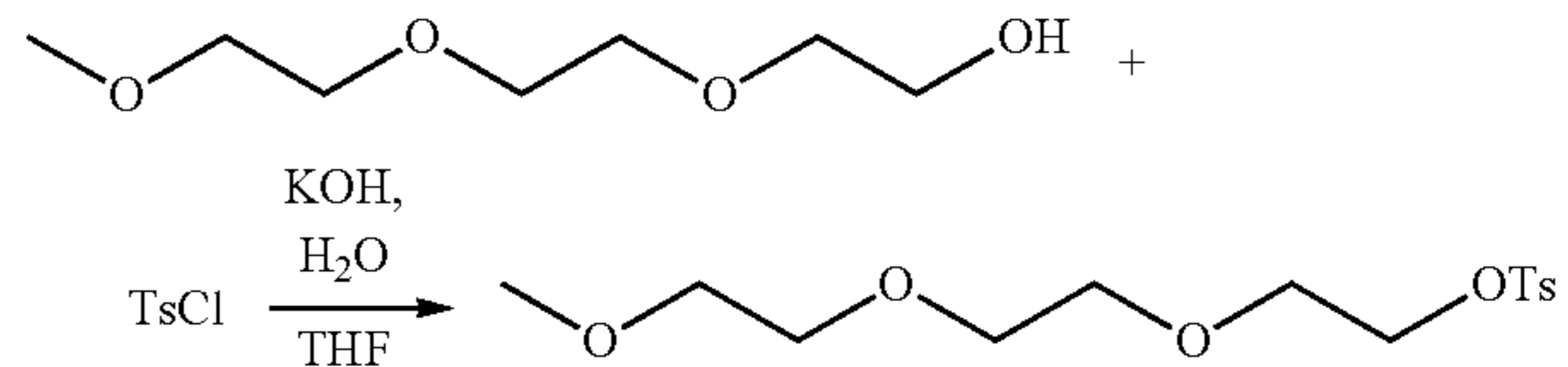
Scheme 1. Monomer synthesis
