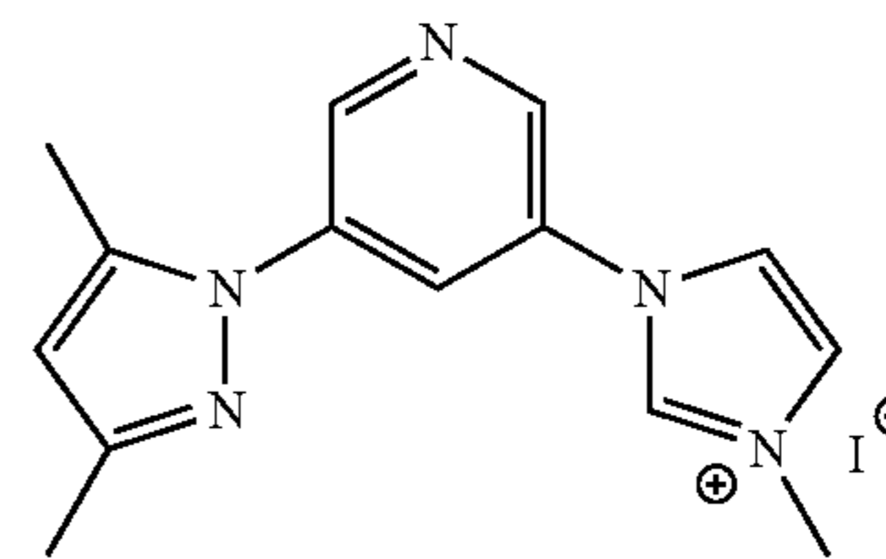
DMPz-Py-IMIz
