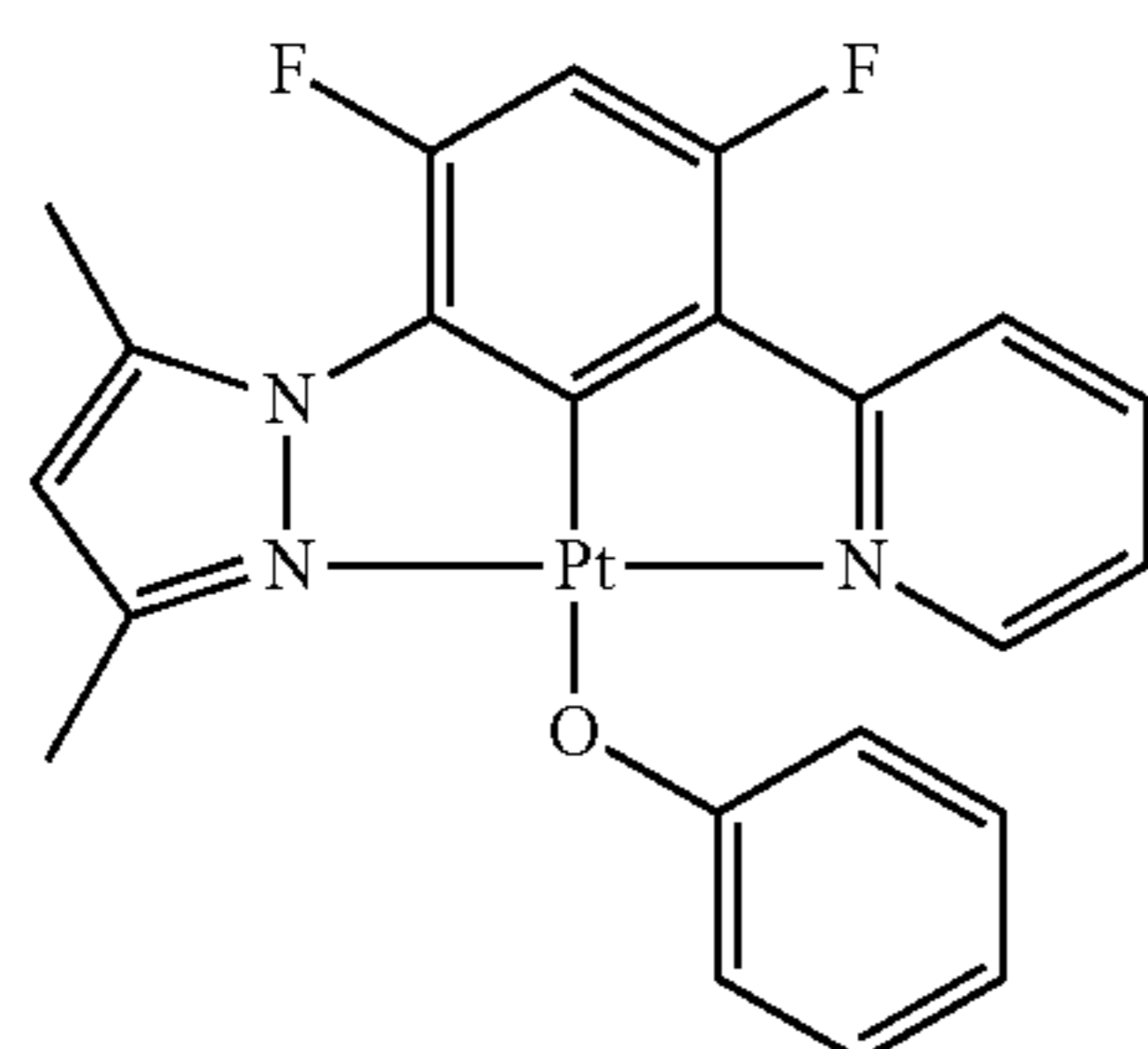
DMPz-DFPh-Py-PtOPh
