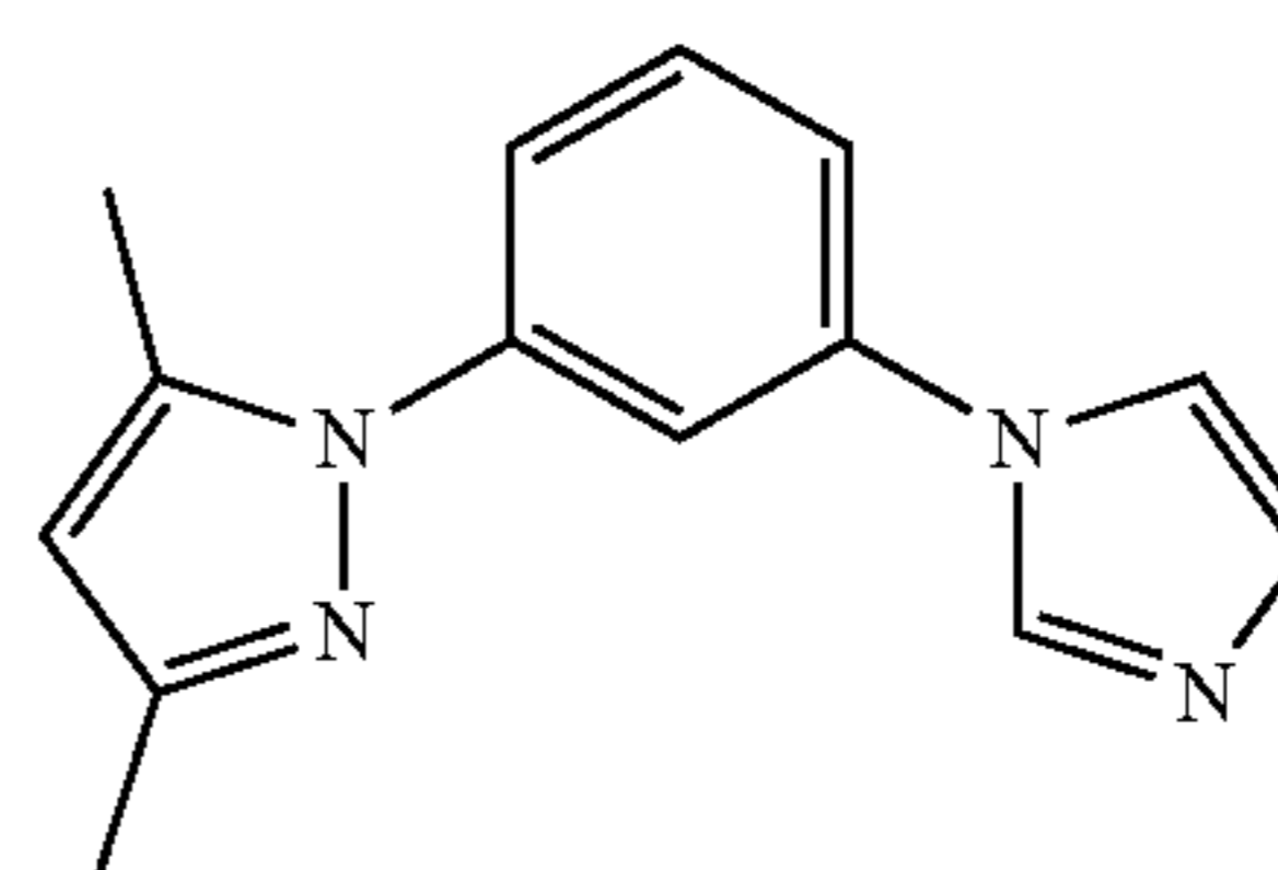
DMPz-Ph-Iz
