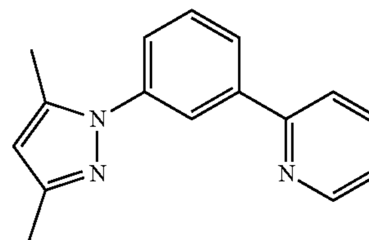
DMPz-Ph-Py
