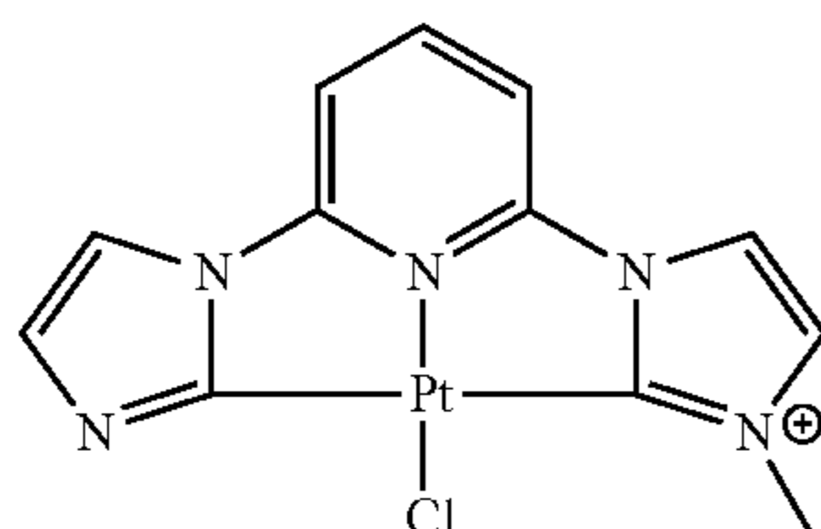
Iz-Py-MizCb-PtCl
