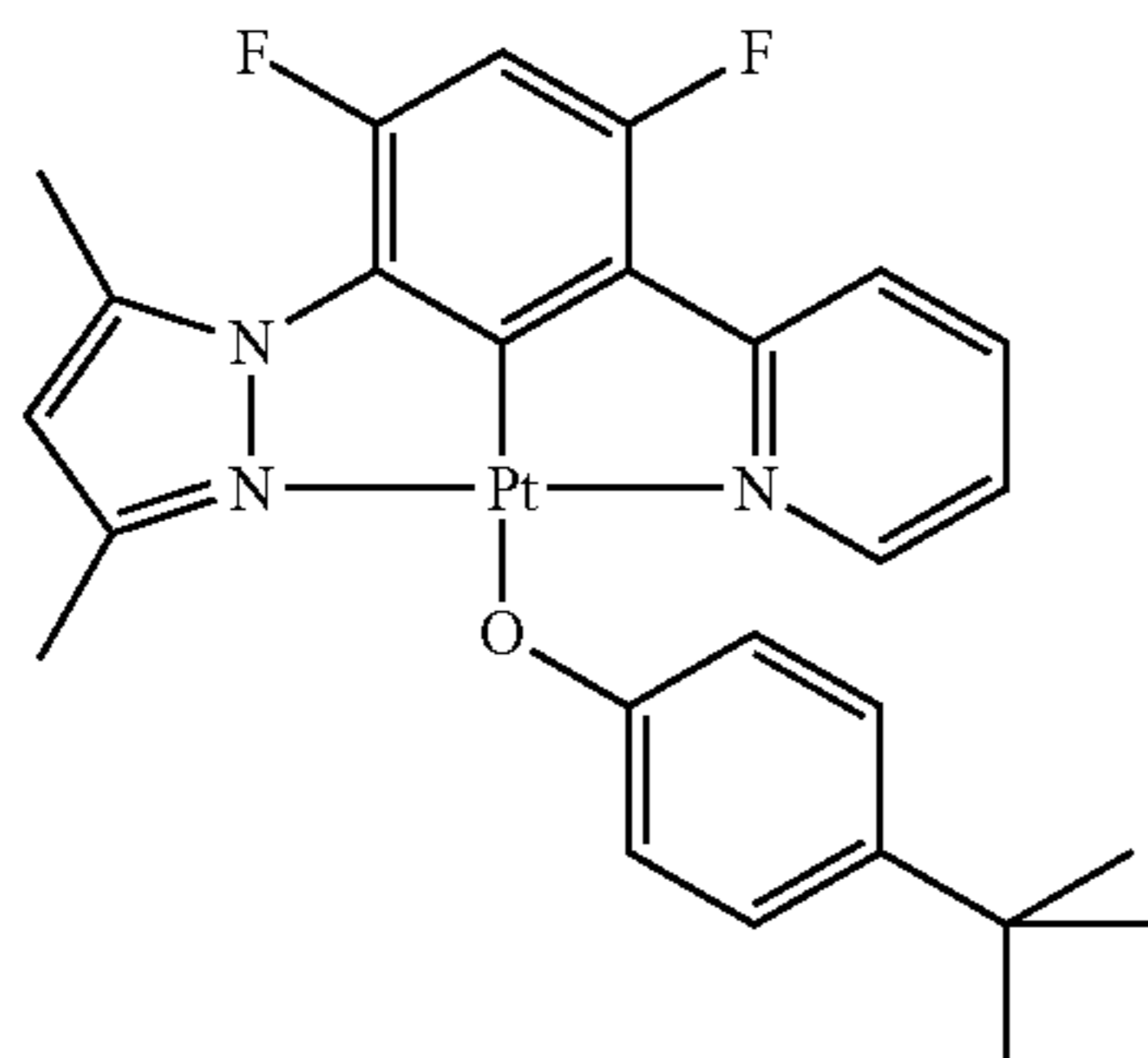
DMPz-DFPh-Py-PtOPhBu
