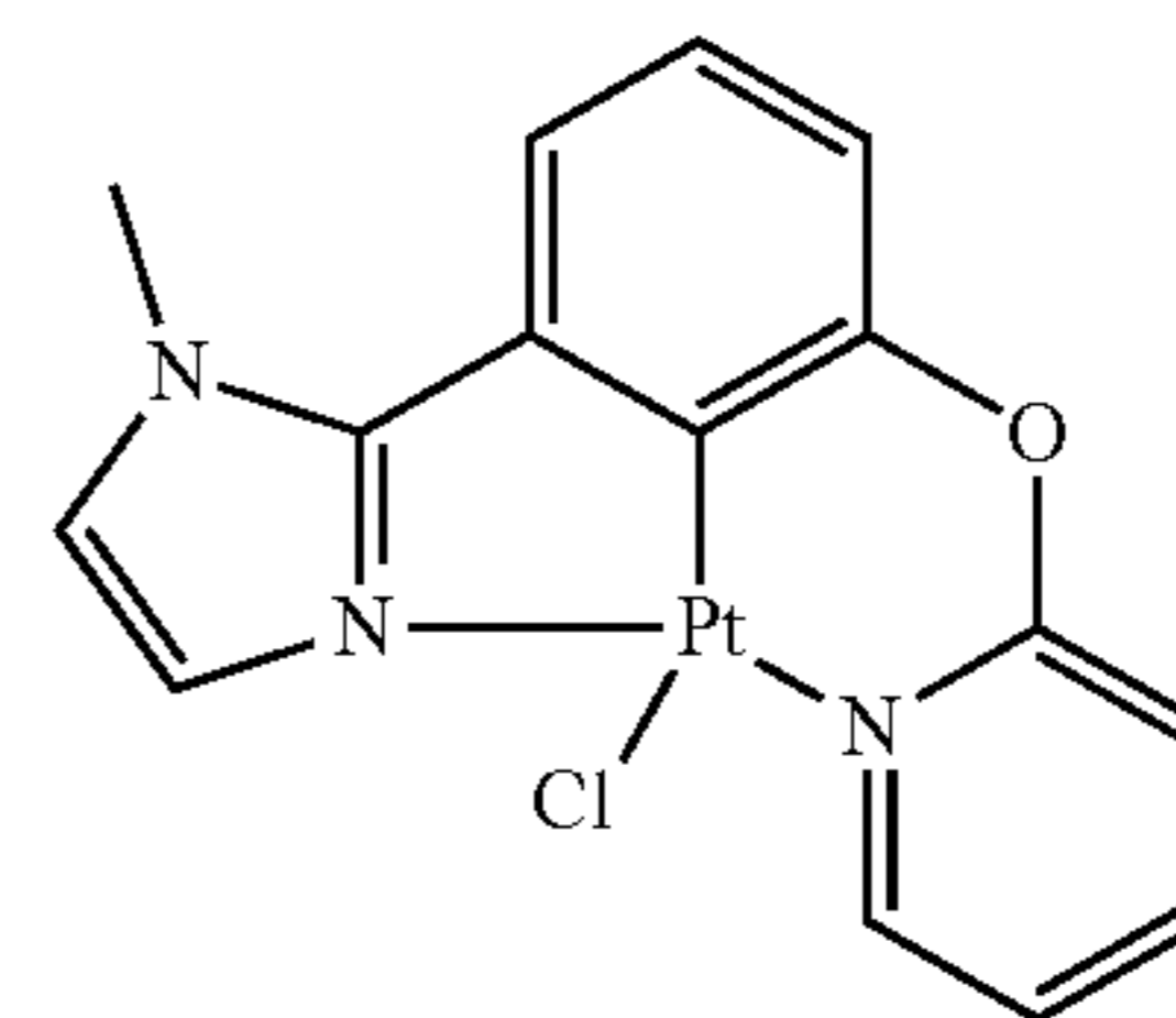
MIz-Ph-O-Py-PtCl
