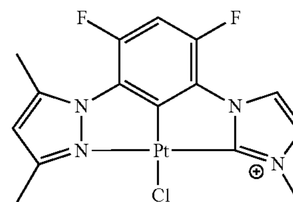
DMPz-Ph-MIzCb-PtCl
