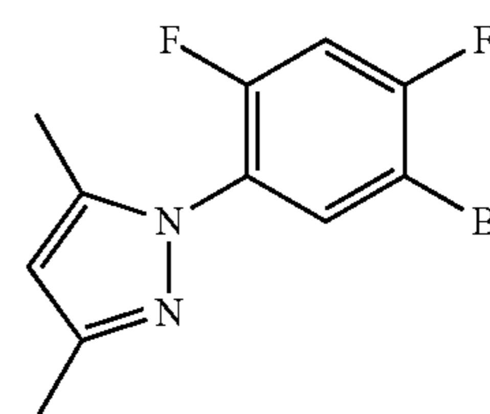
DMPz-DFPh-Br
