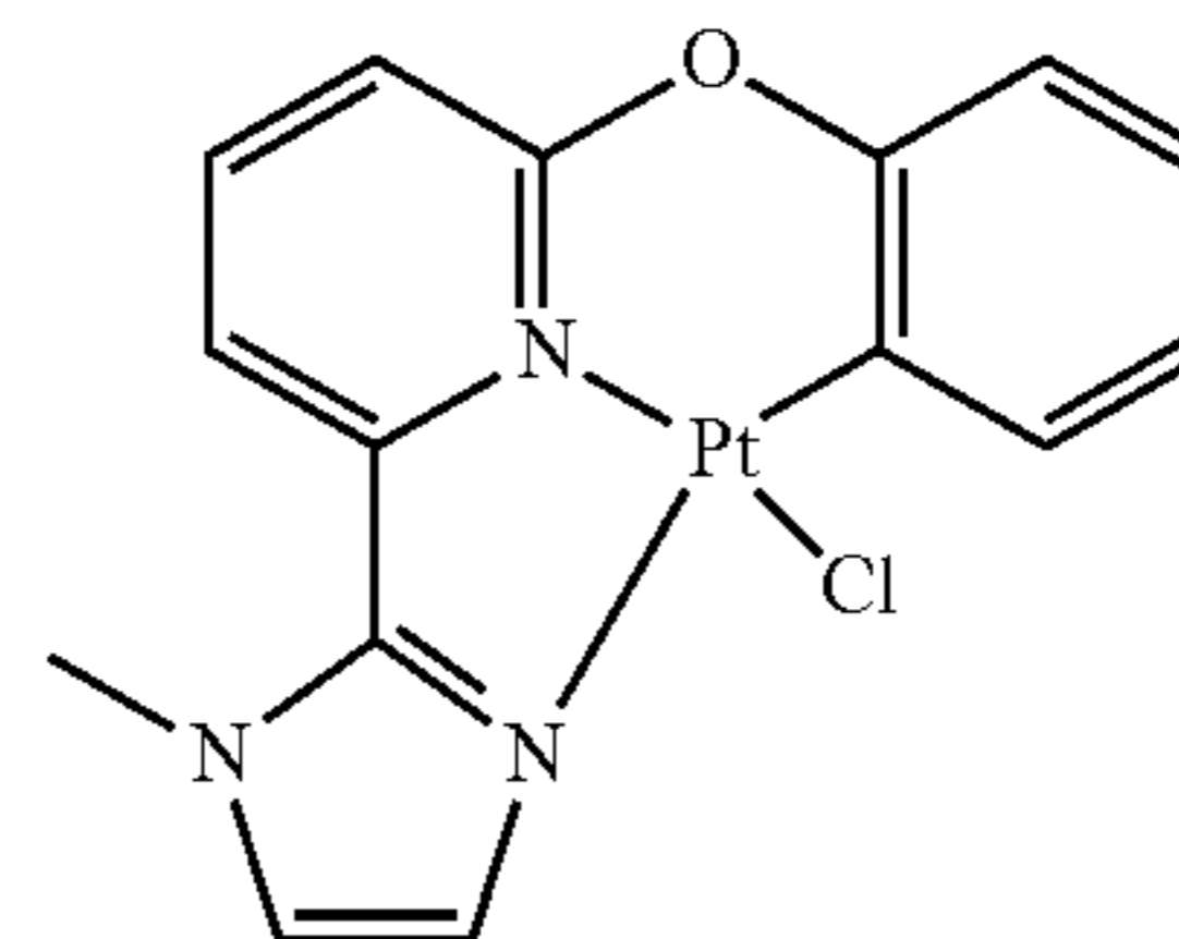
Miz-Py-O-Ph-PtCl
