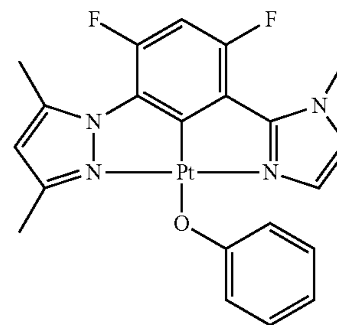
DMPz-DFPh-MIz-PtOPh
