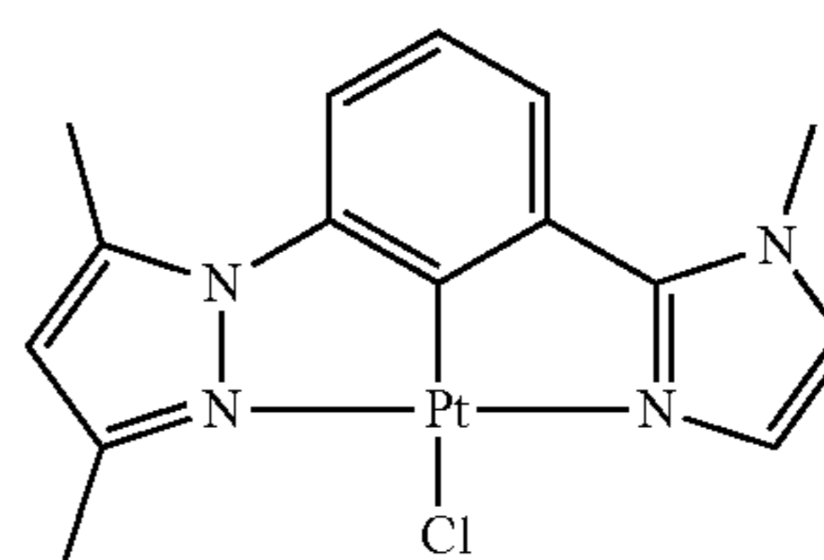
DMPz-Ph-MIz-PtCl
