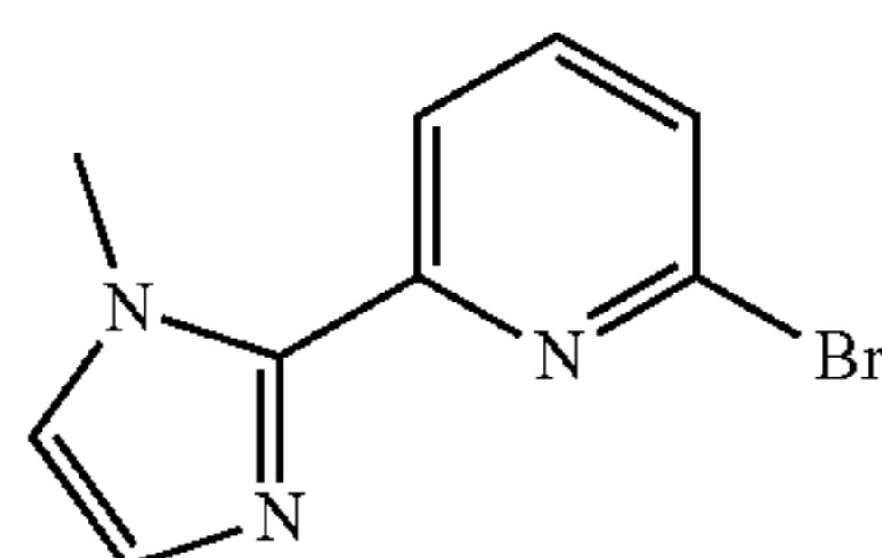
Miz-Py-Br
