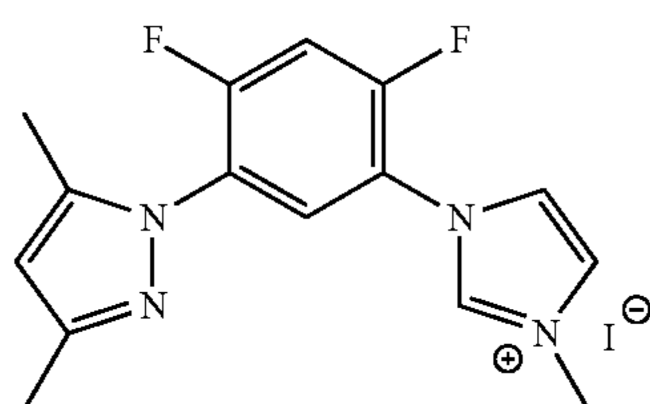
DMPz-Ph-IMIz
