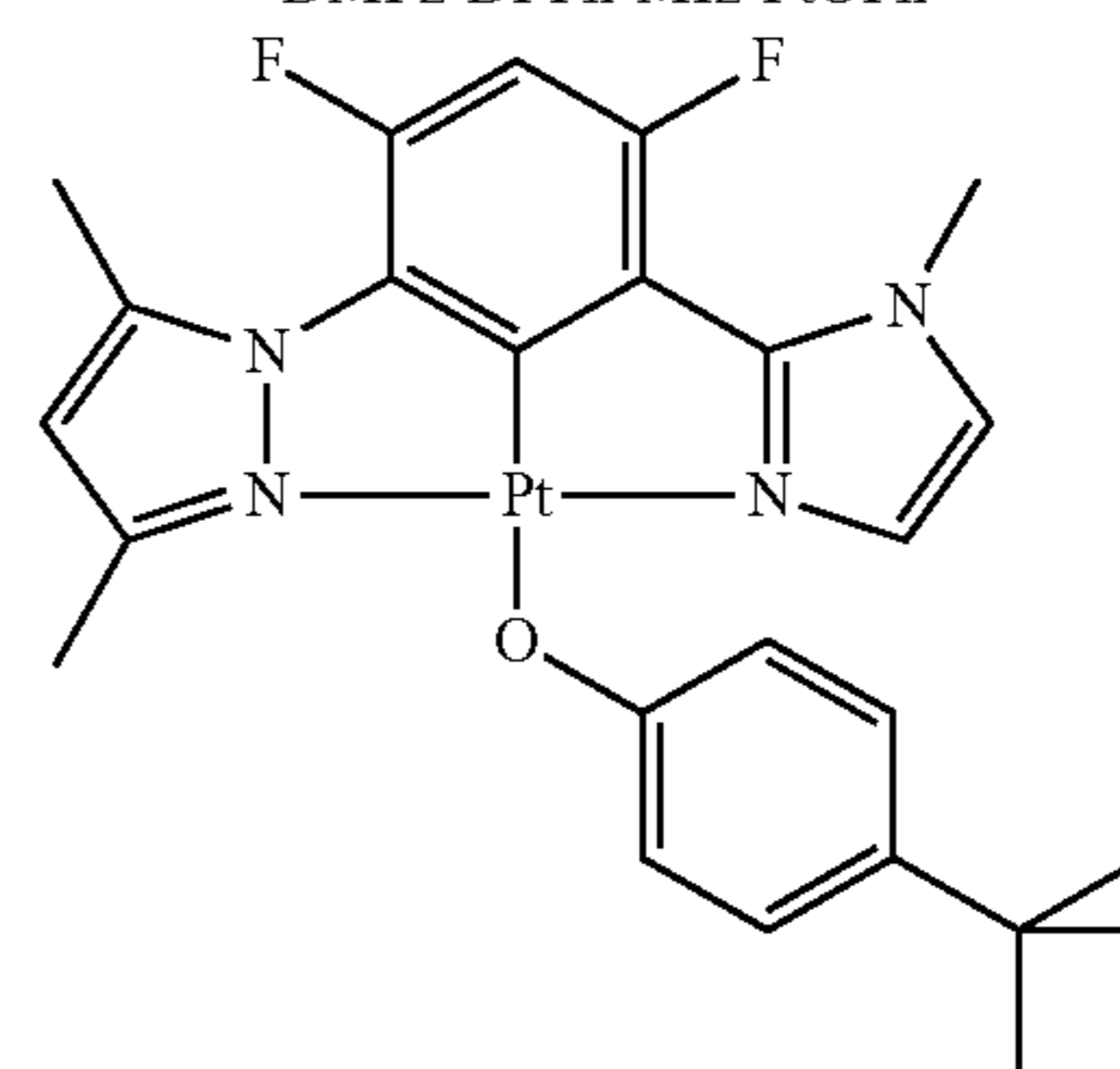
DMPz-DFPh-MIz-PtOPhBu
