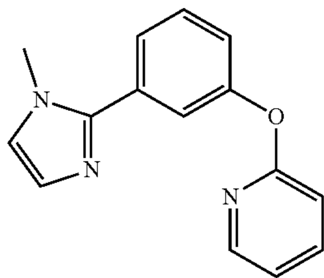
MIz-Ph-O-Py
