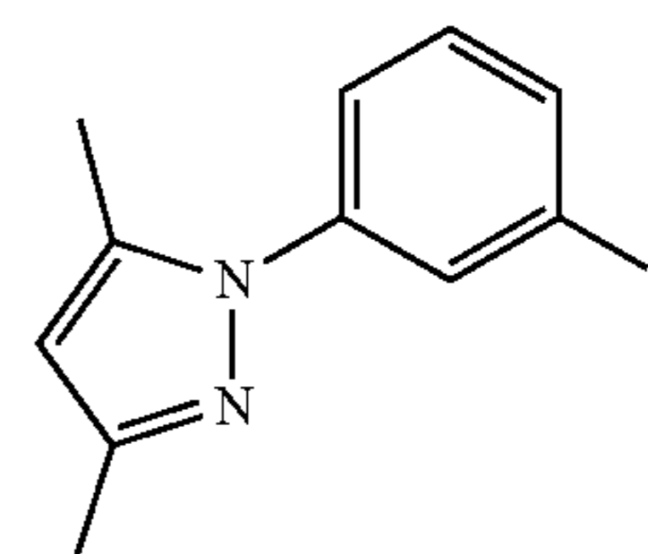
DMPz-Ph-I
