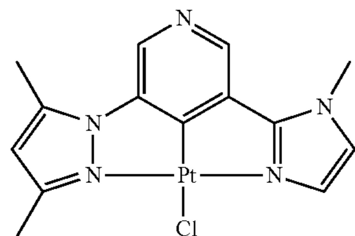
DMPz-Py-MIz-PtCl
