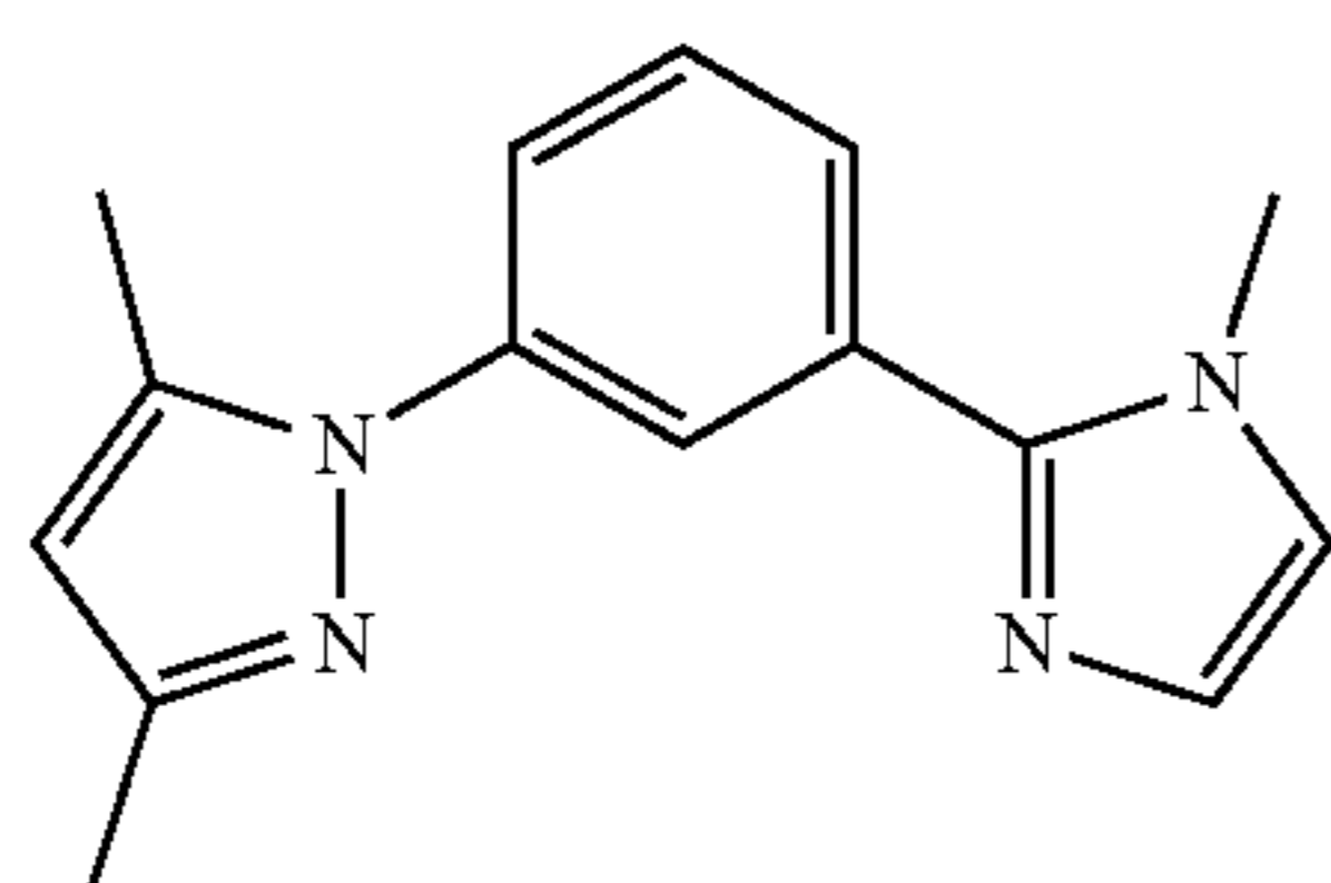
DMPz-Ph-MIz
