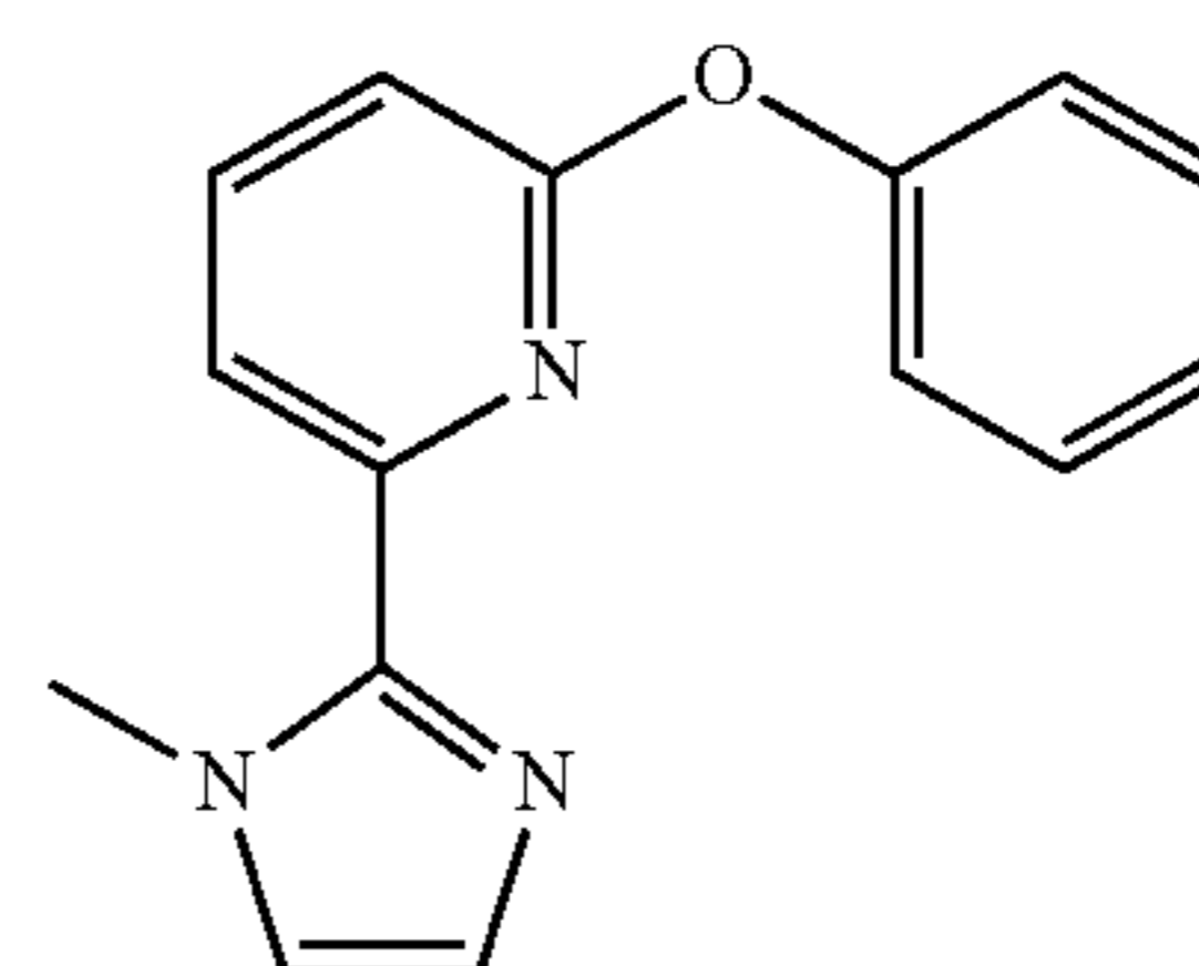
Miz-Py-O-Ph
