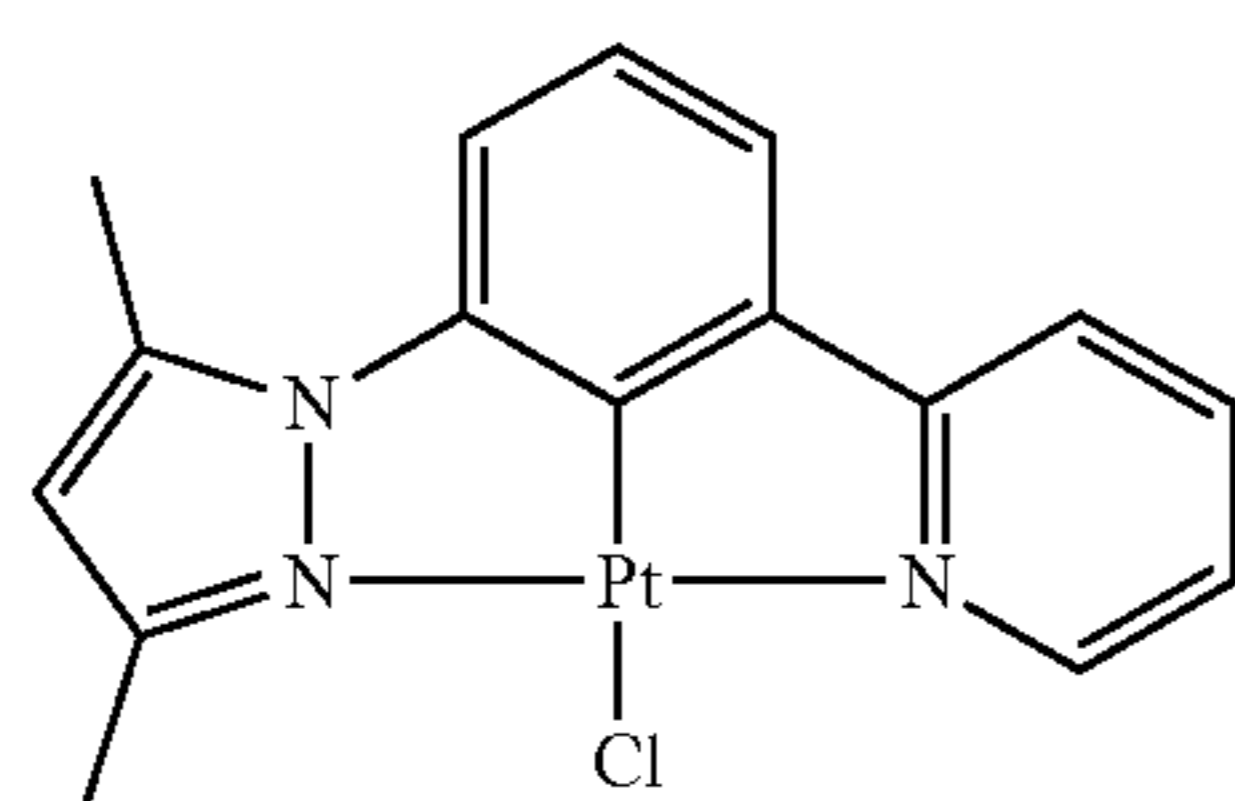
DMPz-Ph-Py-PtCl
