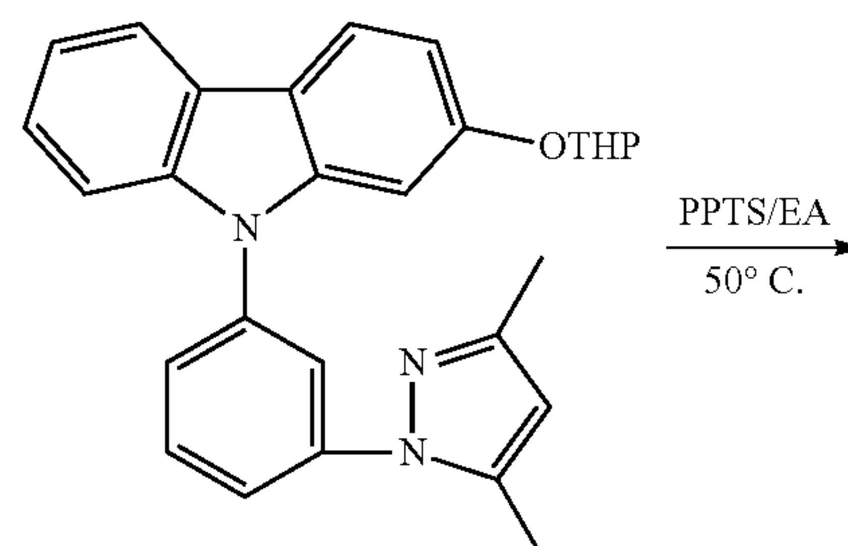
N-[3-(3,5-Dimethylpyrazolylphenyl)]-2-tetrahydropyranyloxy-carbazole
