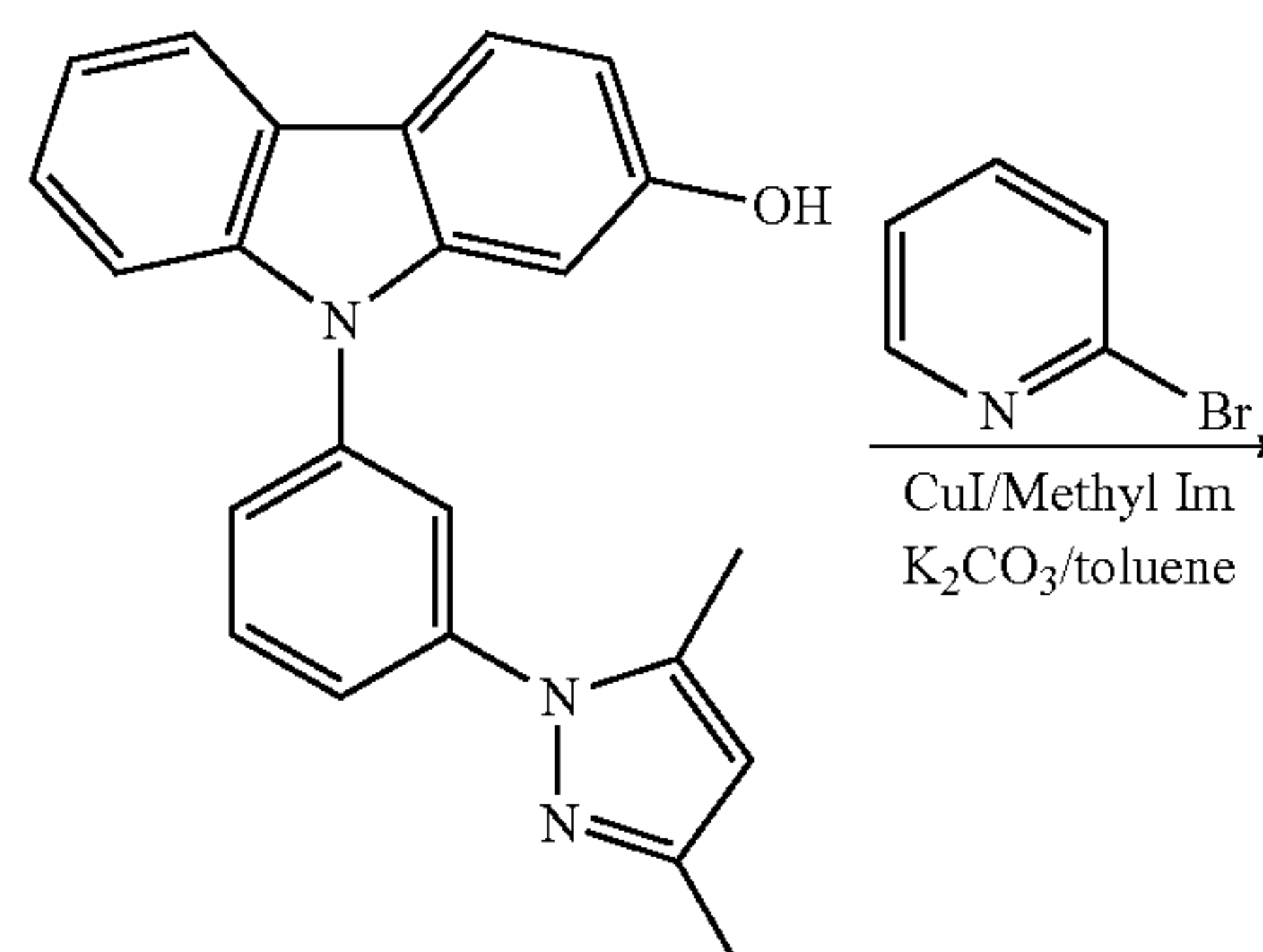
N-[3-(3,5-Dimethylpyrazolylphenyl)]-2-hydroxycarbazole
