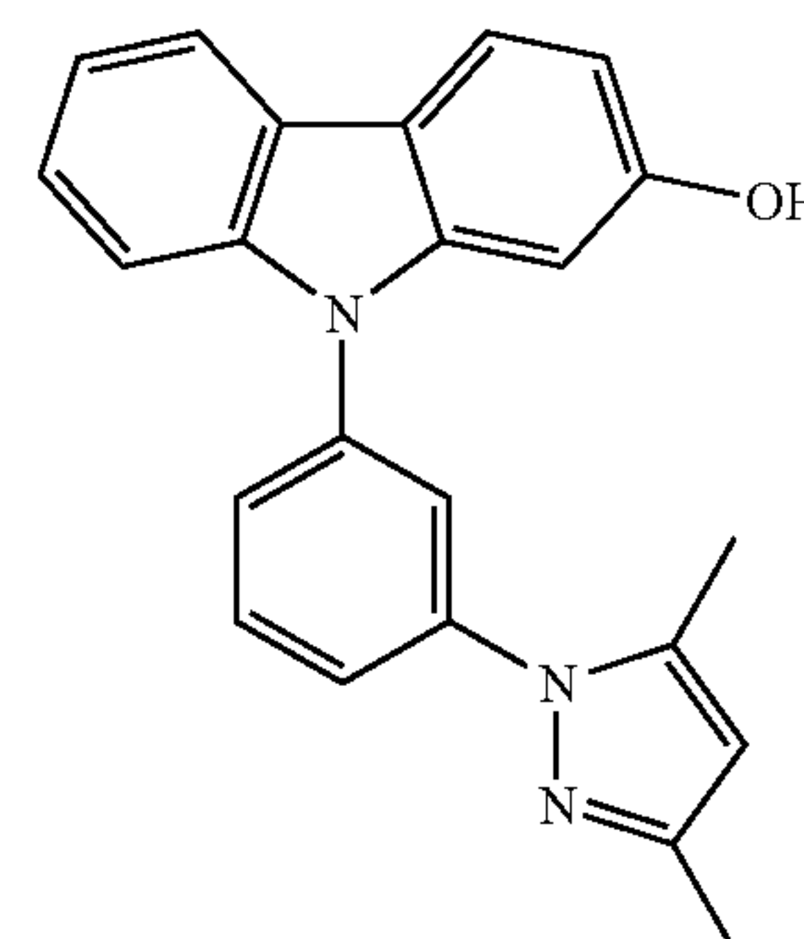
N-(3,5-Dimethylpyrazolylphenyl)-2-hydroxycarbazole
