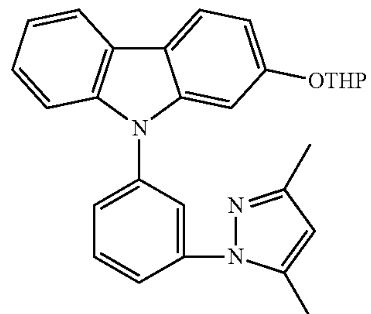
N-[3-(3,5-Dimethylpyrazolylphenyl)]-2-tetrahydropyranyloxy-carbazole
