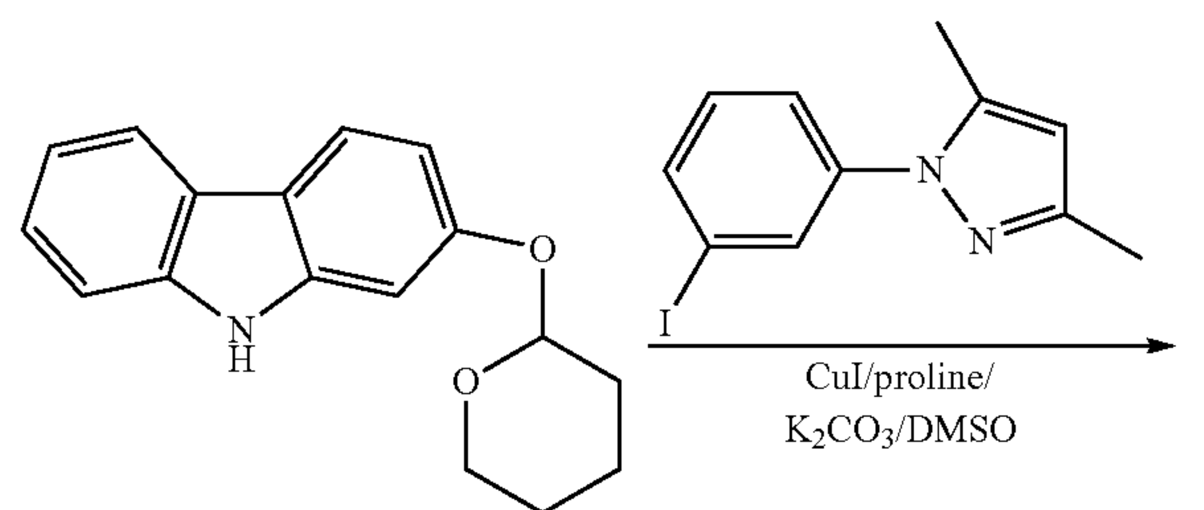
2-tetrahydropyranyloxy-carbazole
