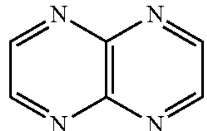
pyrazino[2,3-b]pyrazine
