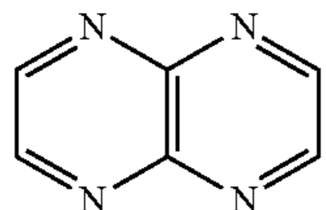
pyrazino[2,3-b]pyrazine
