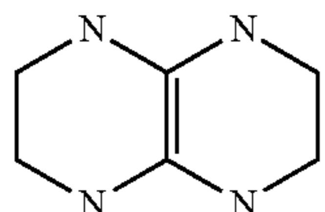
1,2,3,4,5,6,7,8-octahydropyrazino[2,3-b]pyrazine
