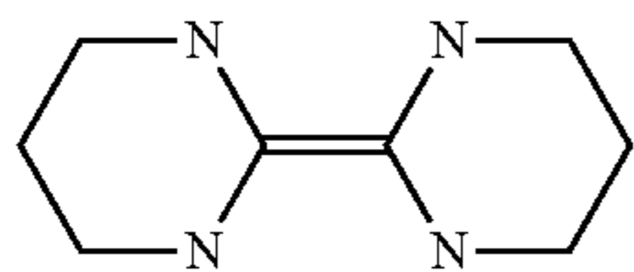
2-hexahydropyrimidin-2-ylidenehexahydropyrimidine
