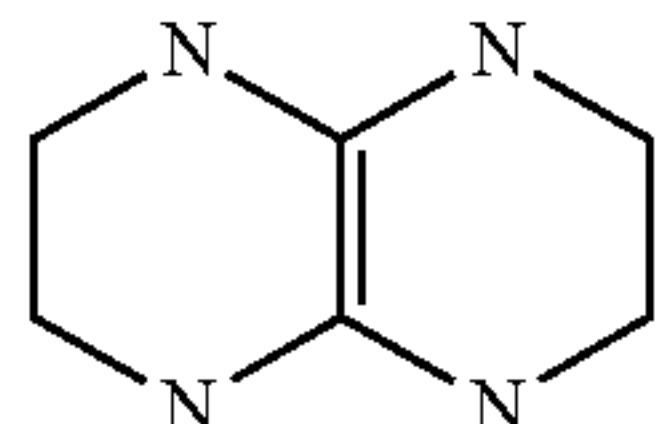
1,2,3,4,5,6,7,8-octahydropyrazino[2,3-b]pyrazine
