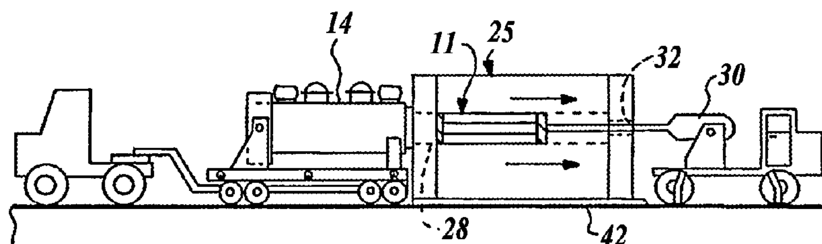
Fig. 4. (PRIOR ART)
