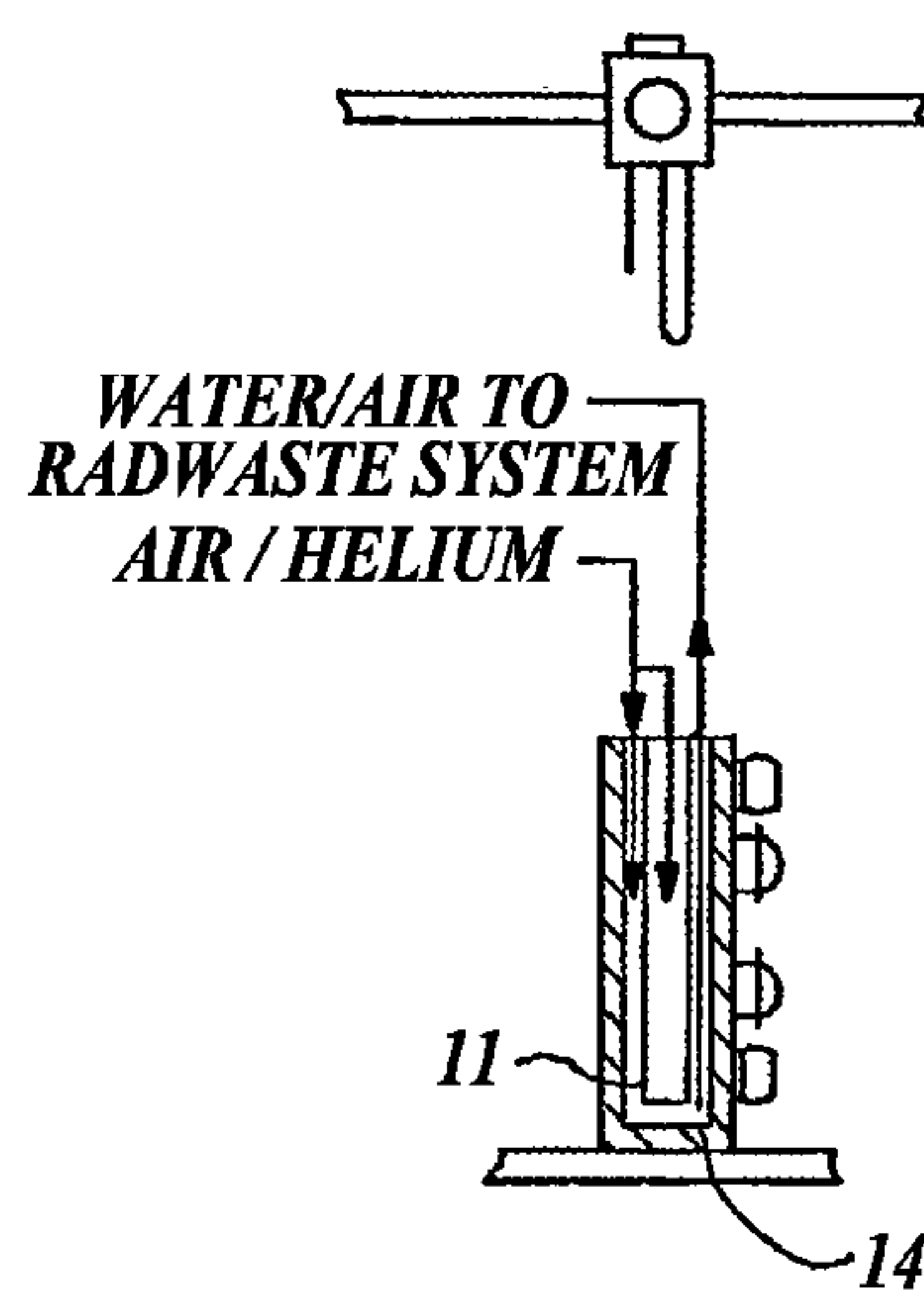
Fig. 2. (PRIOR ART)
