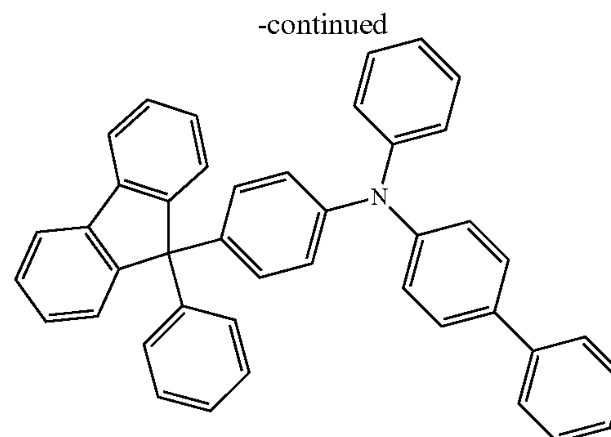
BPAFLP
