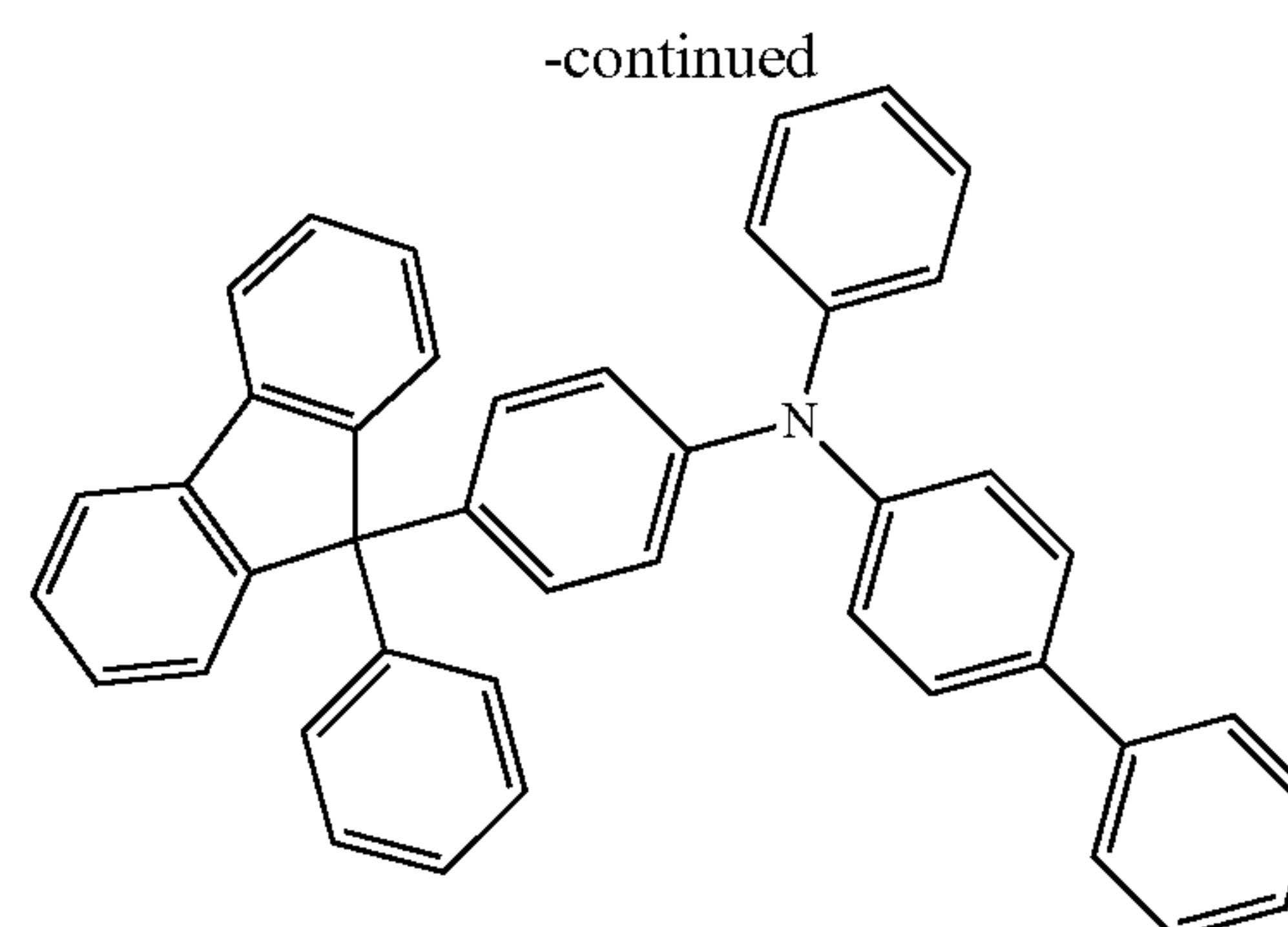
BPAFLP
