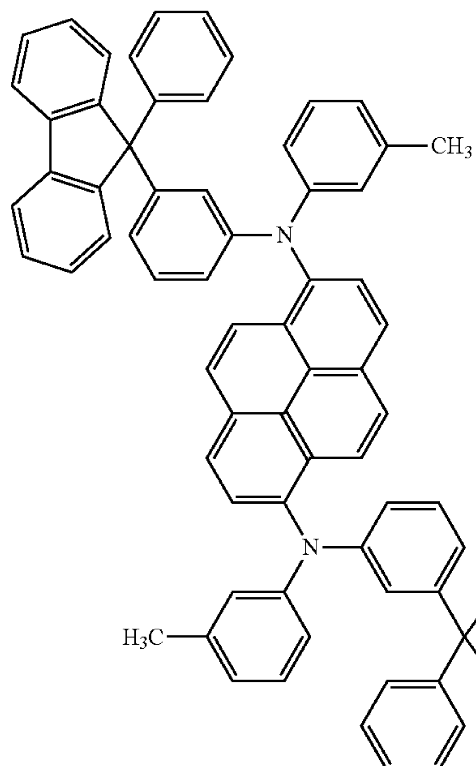
1,6mMemFLPAPrn
