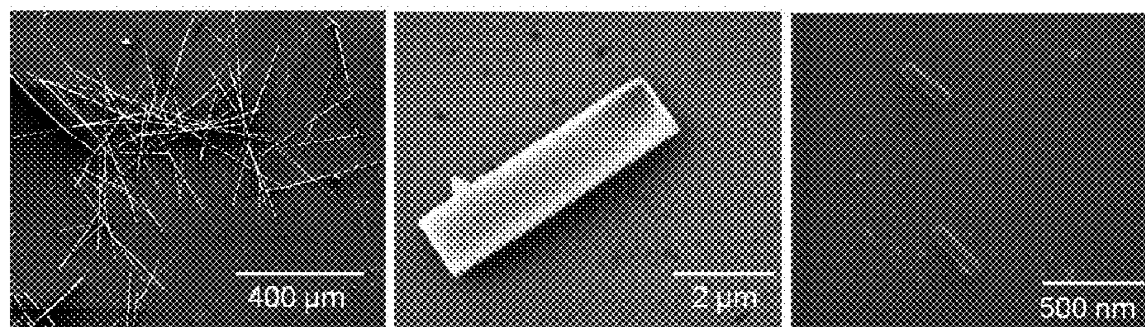
SEM images of CBPQT 2(+) -MV +
