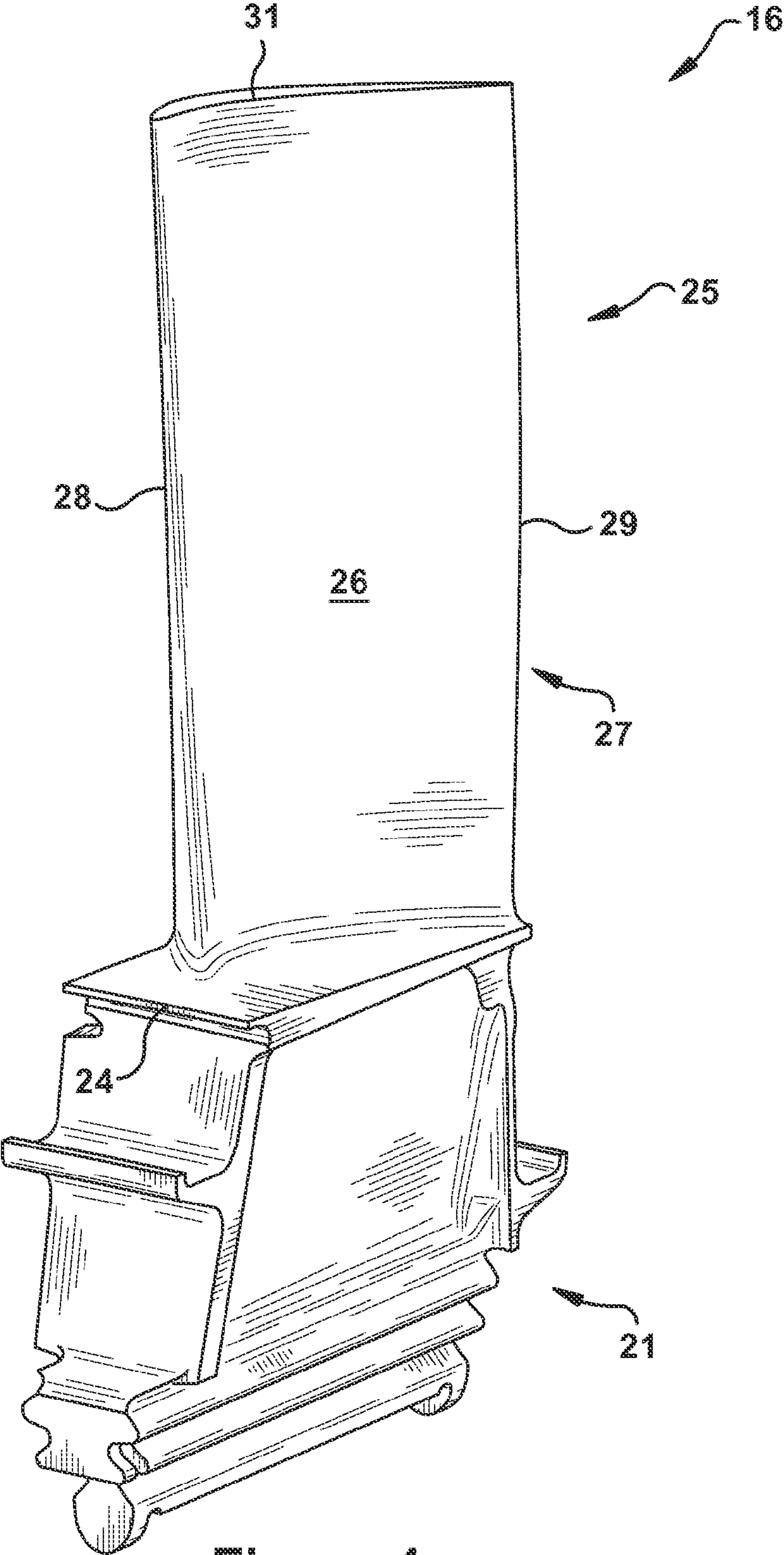
Figure 4 (Prior Art)
