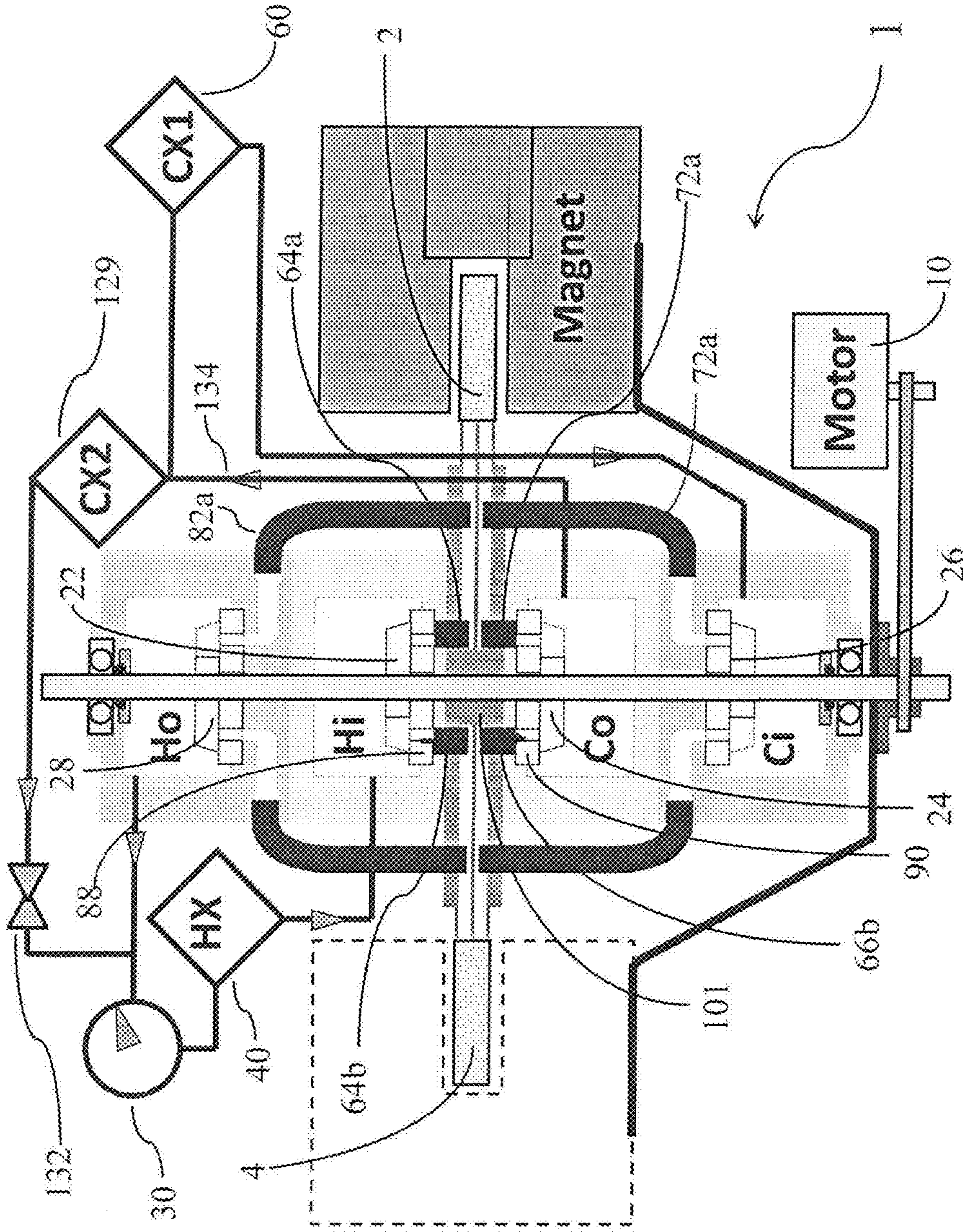
Fig. 11 (unbalanced flow)
