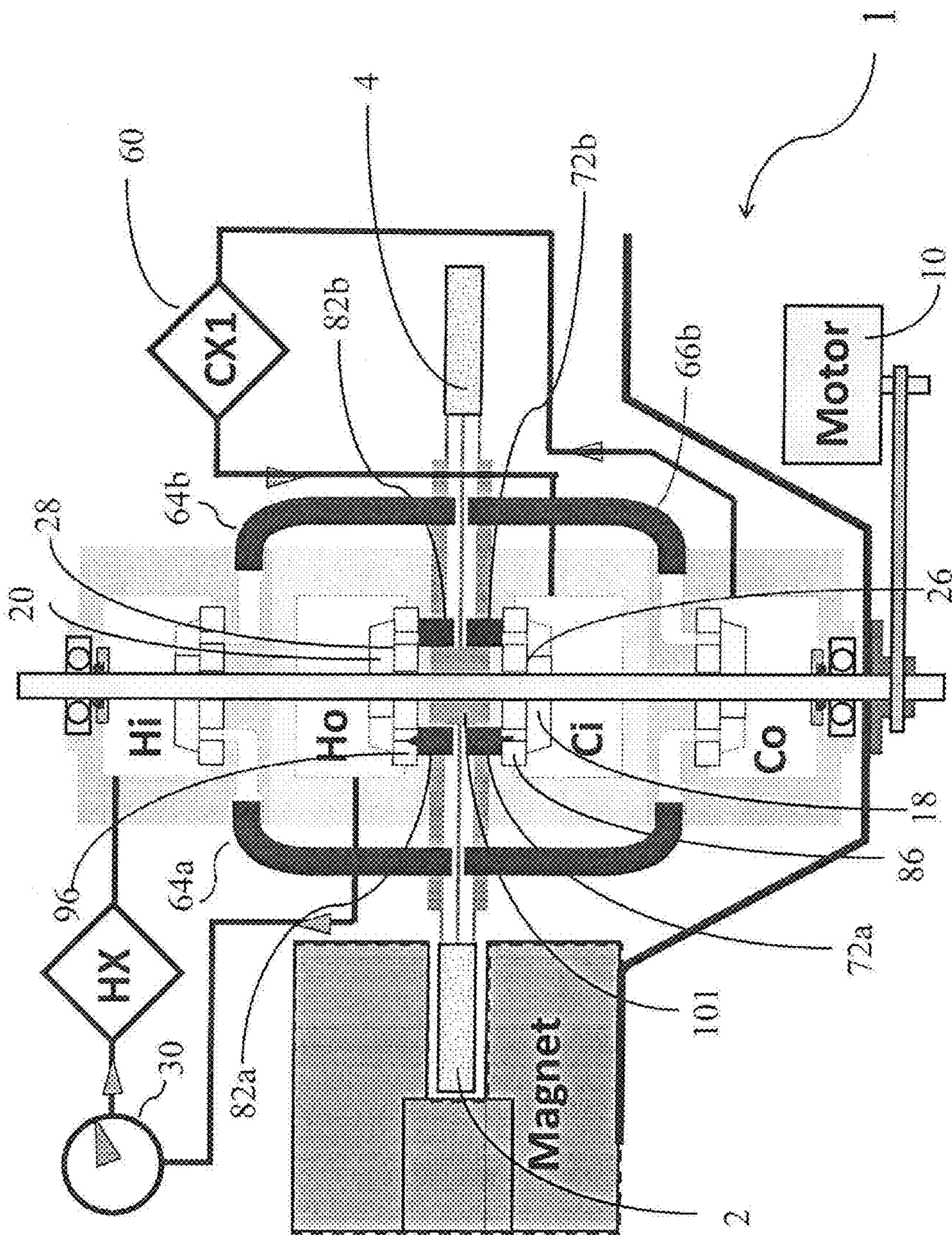
Fig. 10 (unequal blows)
