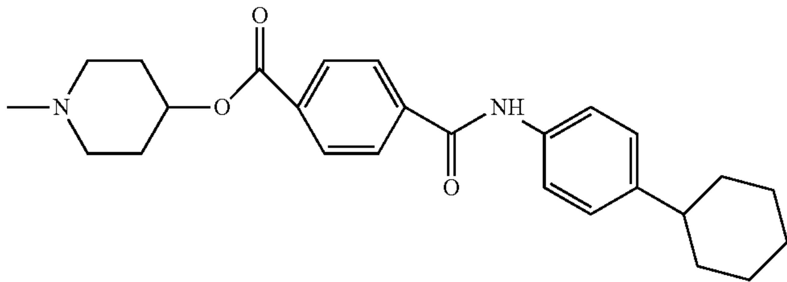
4-[4-(4-cyclohexyl-phenylcarbamoyl)-benzoyloxy]-piperidin-1-yl L(27)
