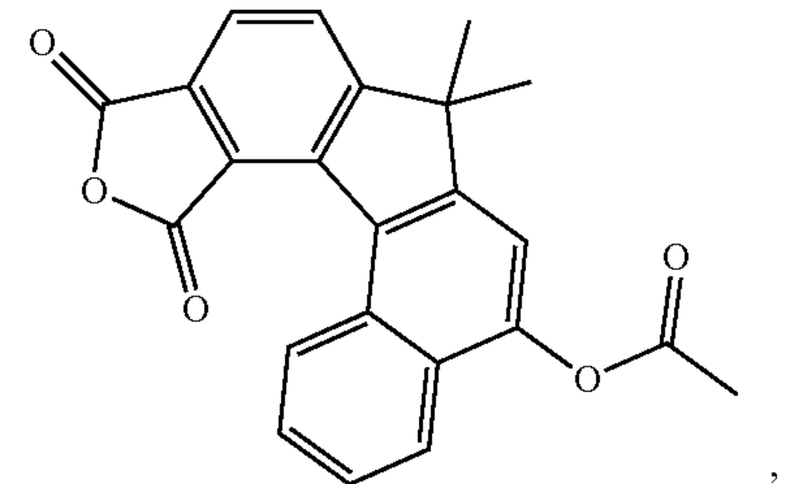
10,12-dioxo-7,7-dimethyl-10,12-dihydro-7H-furo [3',4':4,5]indeno[3,2-a]naphthalen-5-yl acetate
