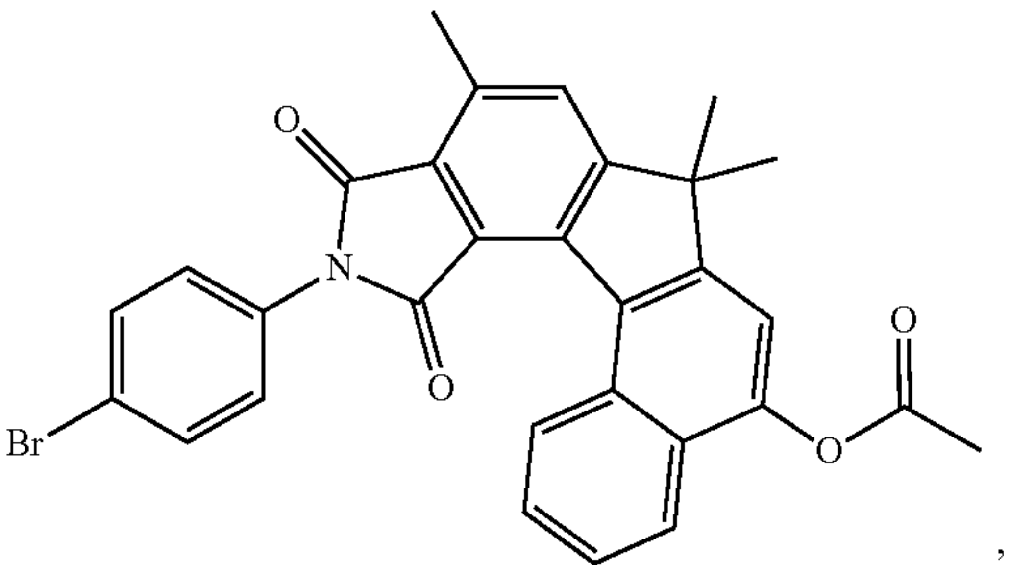
11-(4-bromophenyl)-10,12-dioxo-7,7,9-trimethyl-7,10,11,12- tetrahydropyrrolo[3',4':4,5]indeno[3,2-a]naphthalen-5-yl acetate
