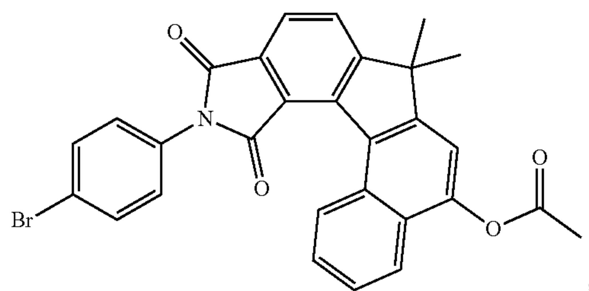
11-(4-bromophenyl)-10,12-dioxo-7,7,9-trimethyl-7,10,11,12-tetrahydropyrrolo[3',4':4,5]indeno[3,4-a]naphthalen-5-yl acetate
