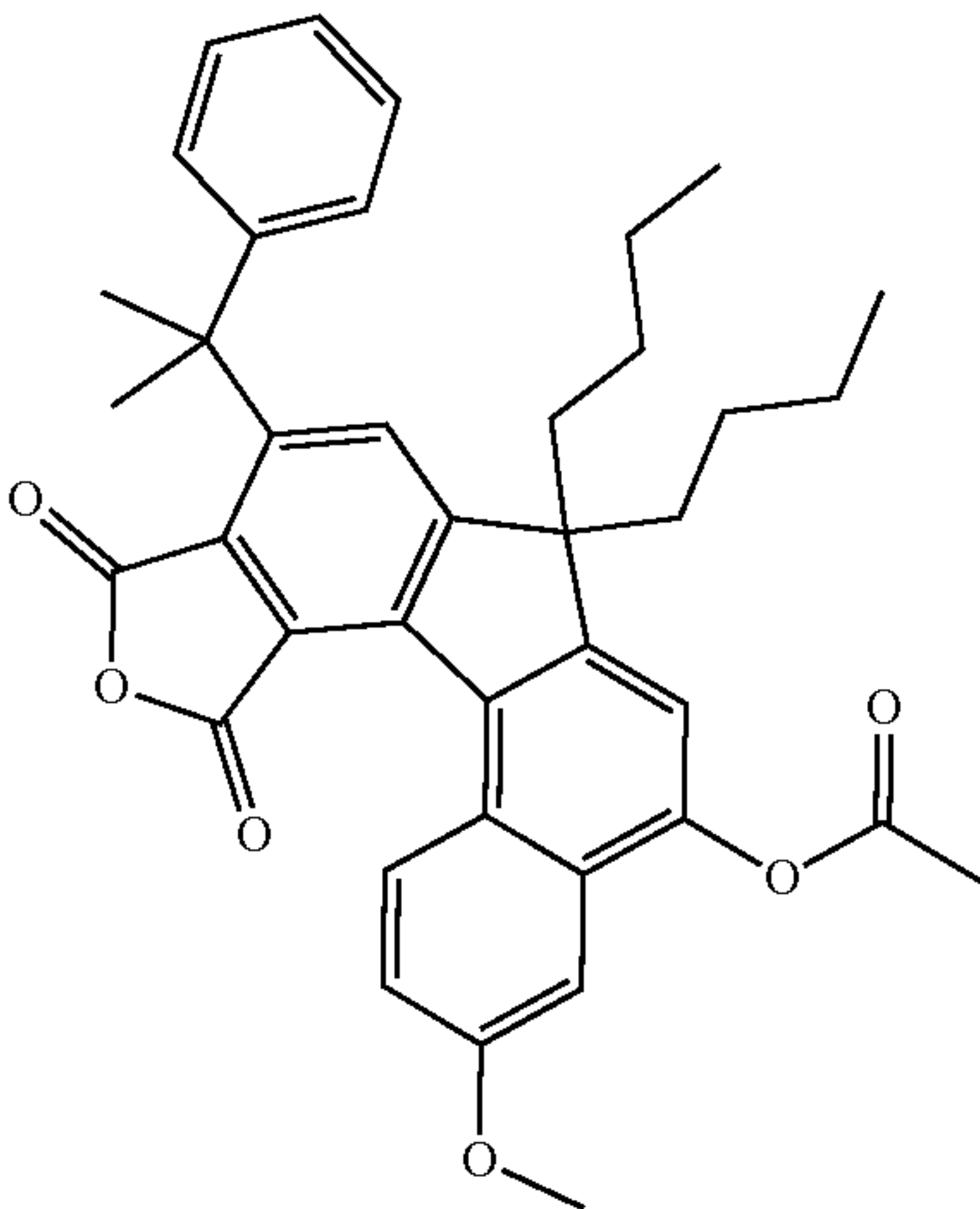
10,12-dioxo-7,7-dibutyl-3-methoxy-9- (2-phenylpropan-2-yl)-10,12-dihydro-7H-furo [3',4':4,5]indeno[3,2-a]naphthalen-5-yl acetate.
