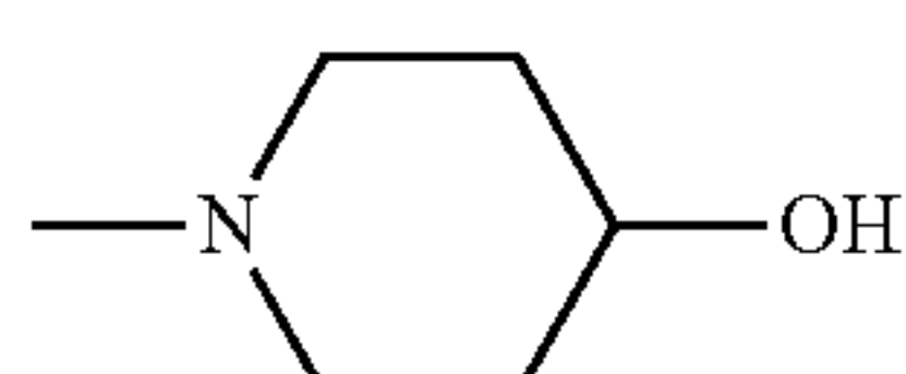
4-(4-phenylcarbamoyl-phenylcarbamoyl)-piperidin-1-yl
