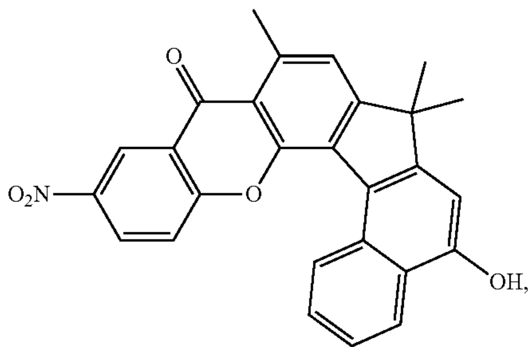
12-nitro-10-oxo-7,7,9-trimethyl-7H-chromeno [3',2':4,5]indeno[3,2-a]naphthalen-5-ol
