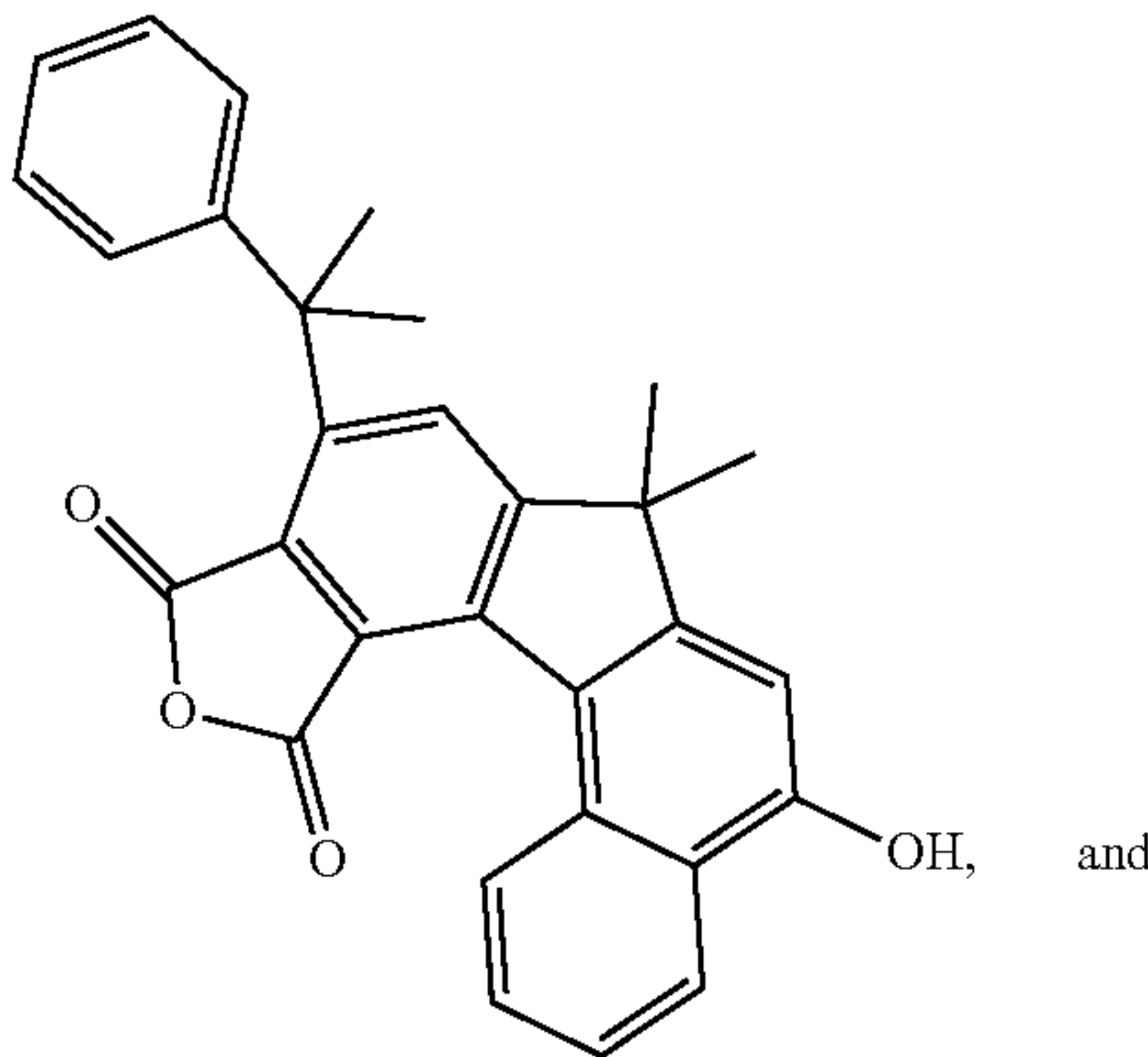
10,12-dioxo-7,7-dimethyl-9-(2-phenylpropan-2-yl)- 10,12-dihydro-7H-furo[3',4':4,5]indeno[3,2-a] naphthalen-5-ol.
