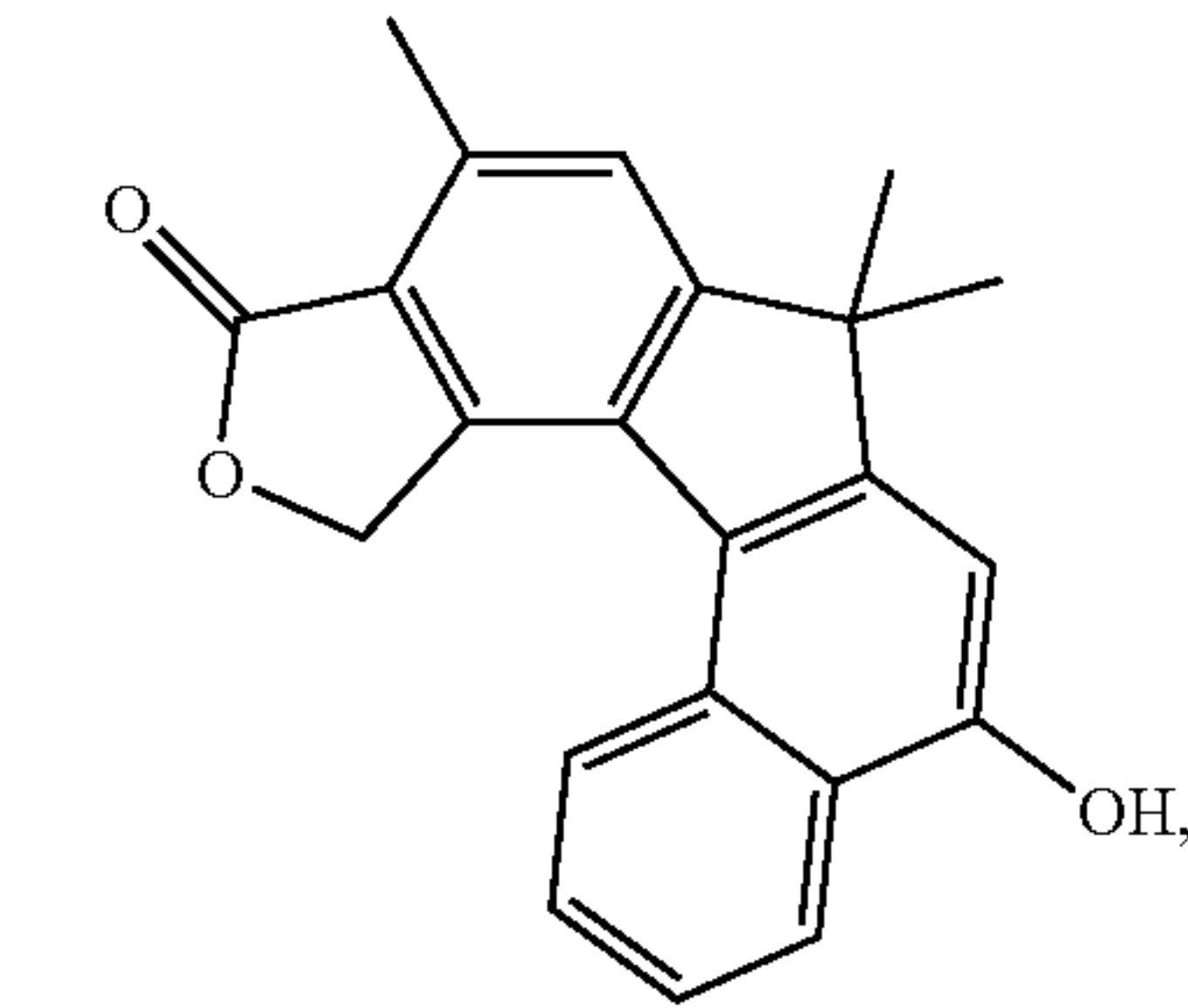
10-oxo-7,7,9-trimethyl-10,12-dihydro-7H-furo[3',4':4,5]indeno[3,2-a]naphthalen-5-ol
