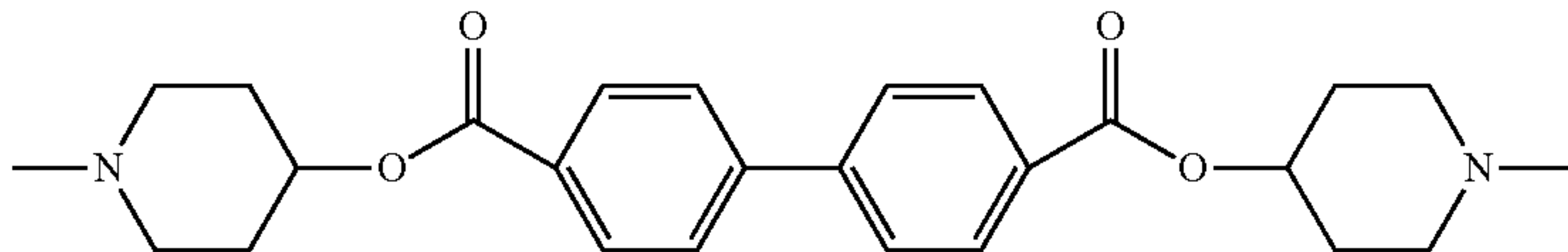
bis(1-yl-piperidin-4-yl) [1,1'-biphenyl]-4,4'-dicarboxylate (which links two separate photochromic PC groups)
