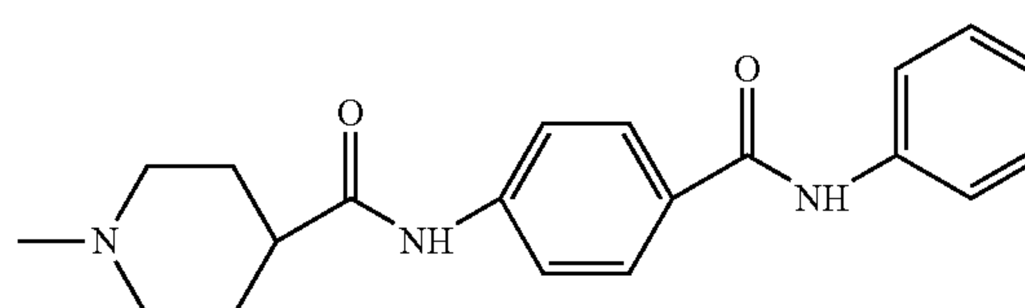
4-(4-(4-phenylpiperidin-1-yl)-benzoyloxy)-piperidin-1-yl
