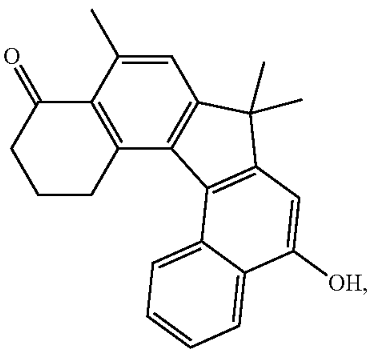
10-oxo-7,7,9-trimethyl-10,11,12,13-tetrahydro-7H-benzol[4,5]indeno[3,2-a]naphthalen-5-ol
