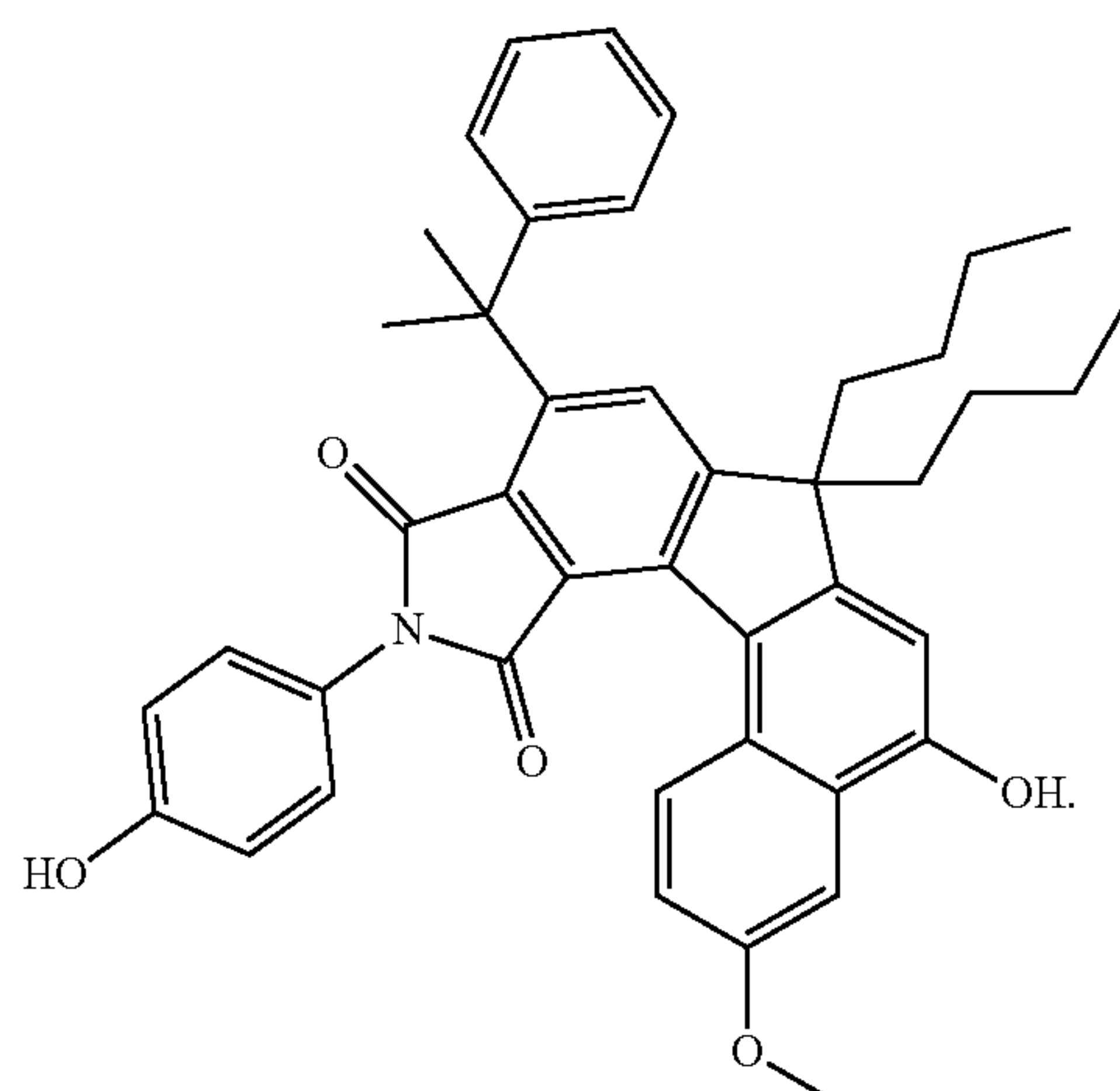
11-(4-hydroxyphenyl)-10,12-dioxo-7,7-dibutyl-3-methoxy-9-(2-phenylpropan-2-yl)-7,10,11,12-tetrahydropyrrolo[3',4':4,5]indeno[3,2-a]naphthalen-5-ol.
