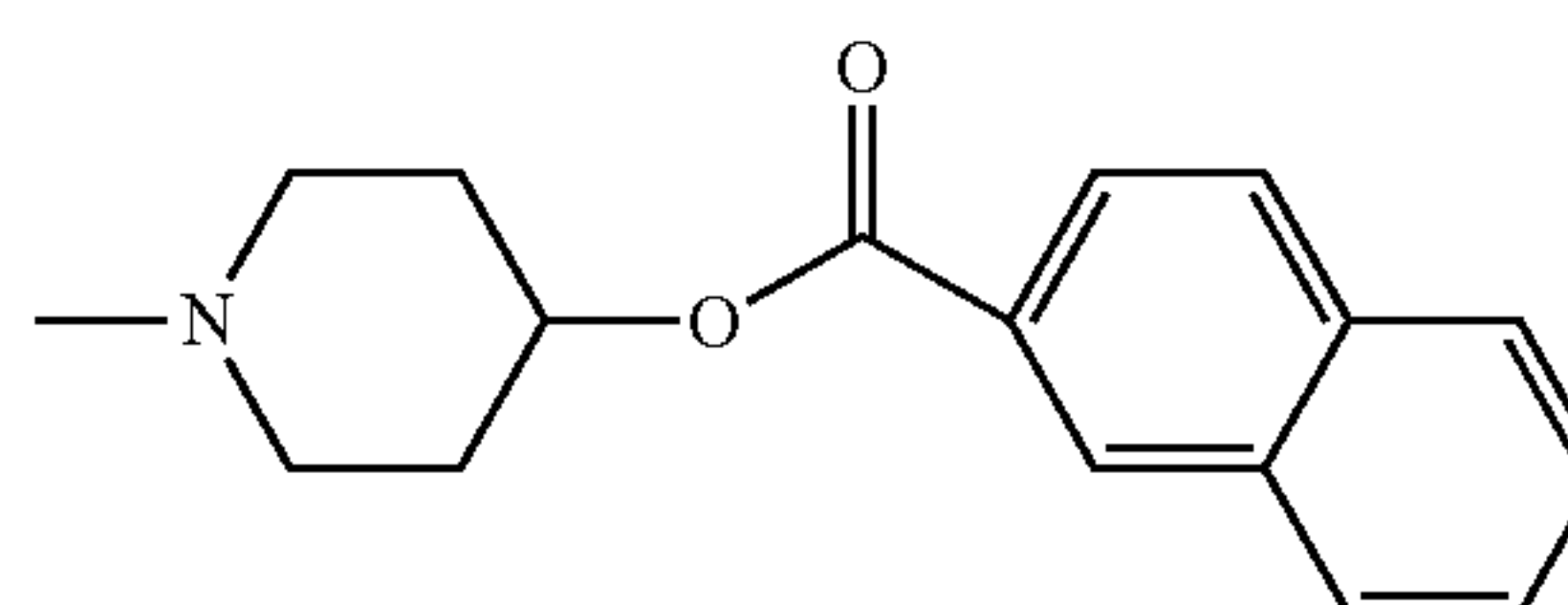
4-hydroxy-piperidin-1-yl
