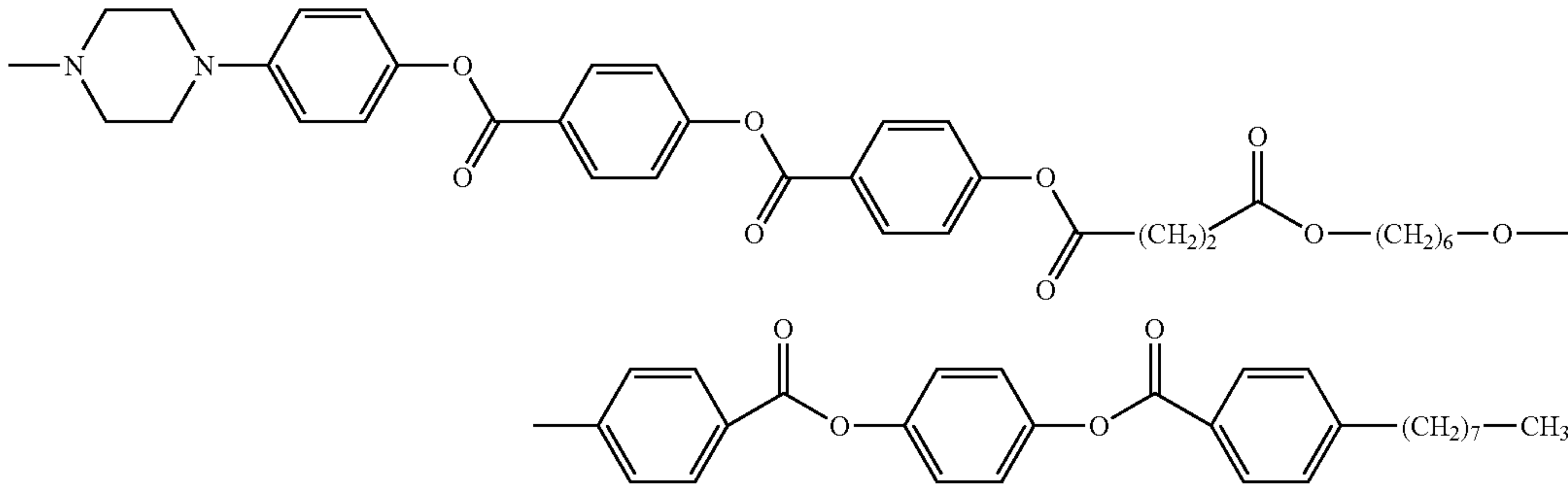
{4-[4-(4-{4-[4-(4-nonyl-benzoyloxy)-benzoyloxy]-benzoyloxy}-benzoyloxy)-phenyl]-piperazin-1-yl}
