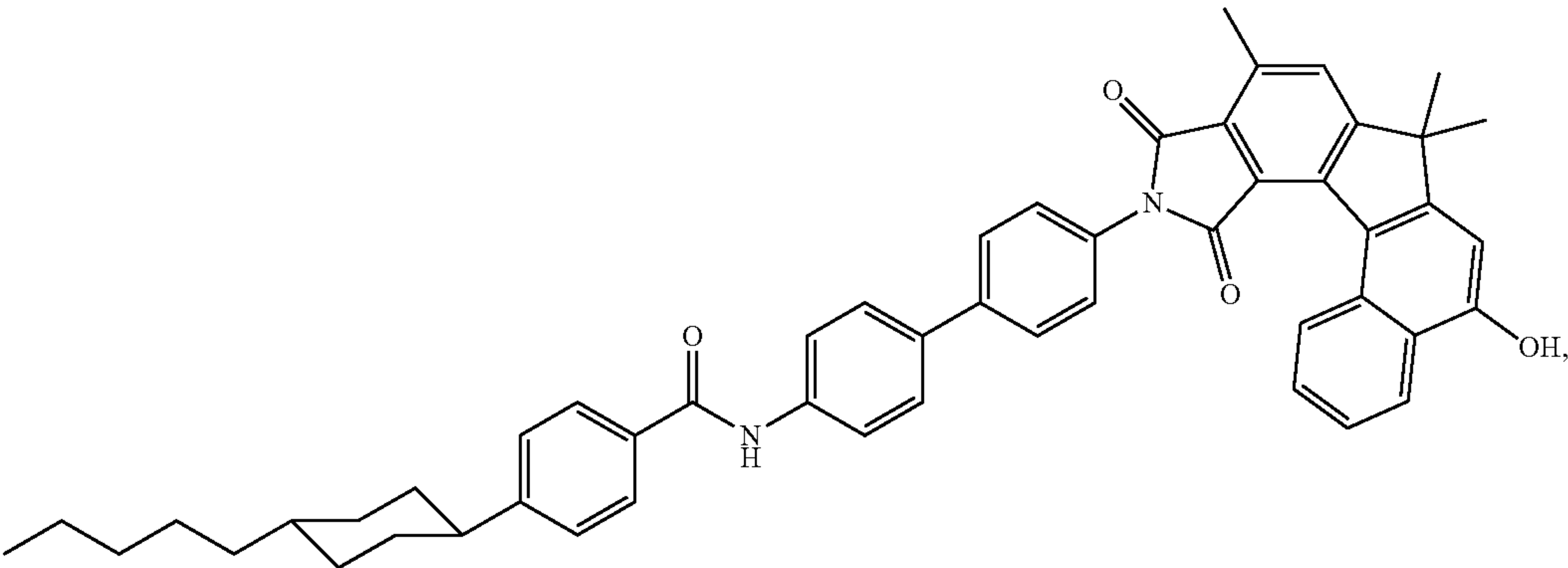
11-(4'-(4-(trans-4-pentylcyclohexyl)benzamido)-[1,1'-biphenyl])-10,12-dioxo- 7,7,9-trimethyl-7,10,11,12-tetrahydropyrrolo[3',4':4,5]indeno[3,2-a]naphthalen-5-ol
