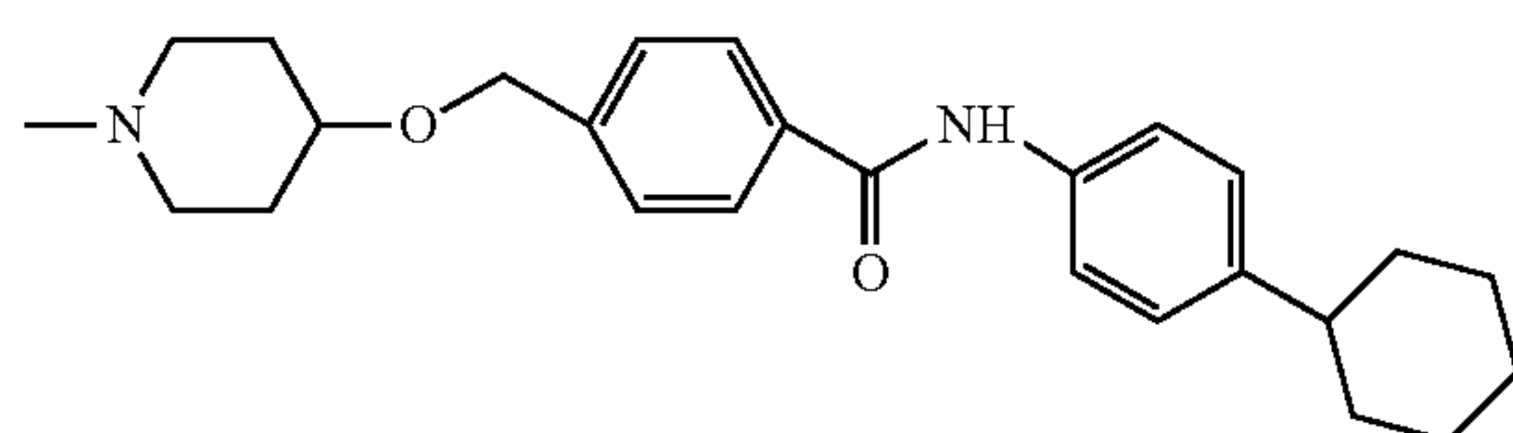
4-[4-(4-cyclohexyl-phenylcarbamoyl)-benzoyloxy]-piperidin-1-yl
