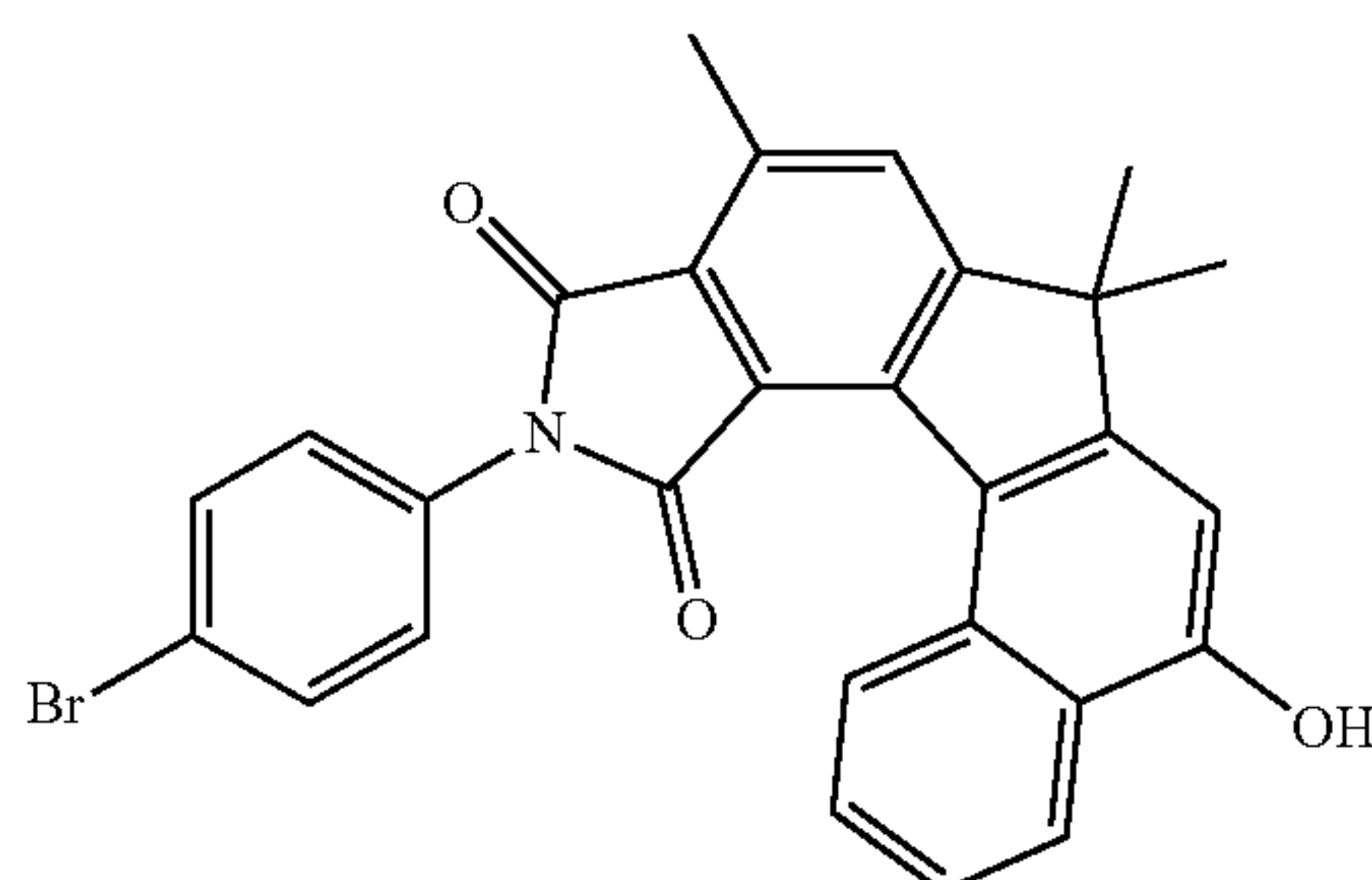
11-(4-bromophenyl)-10,12-dioxo-7,7,9-trimethyl-7,10,11,12-tetrahydropyrrolo[3',4':4,5]indeno[3,4-a]naphthalen-5-ol
