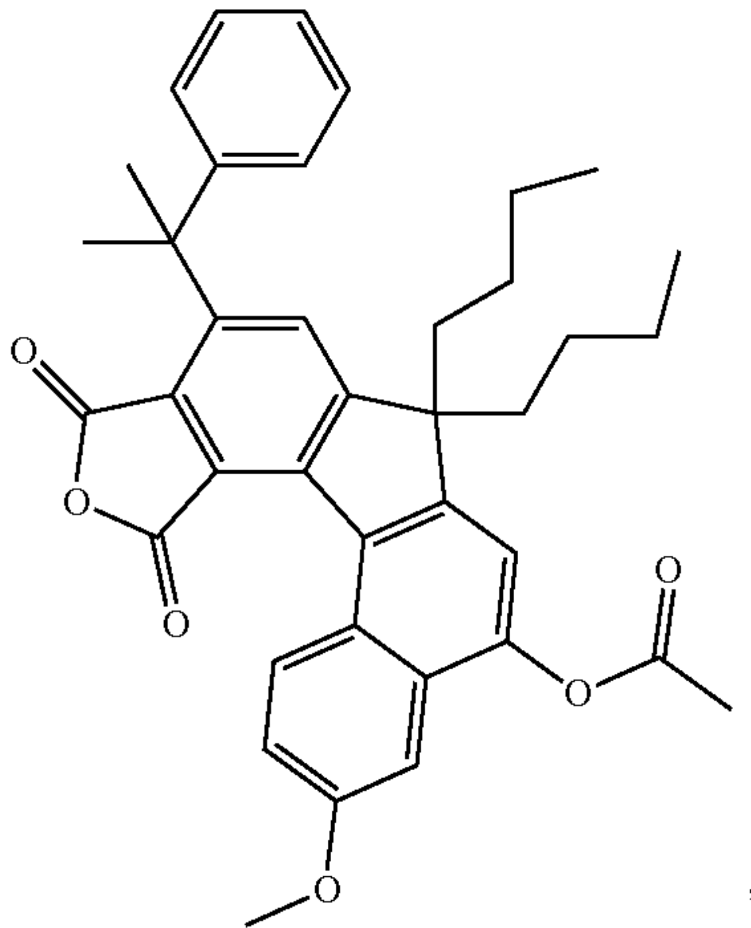
10,12-dioxo-7,7-dibutyl-3-methoxy-9-(2-phenylpropan-2-yl)-10,12-dihydro-7H-furo[3',4':4,5]indeno[3,2-a]naphthalen-5-yl acetate
