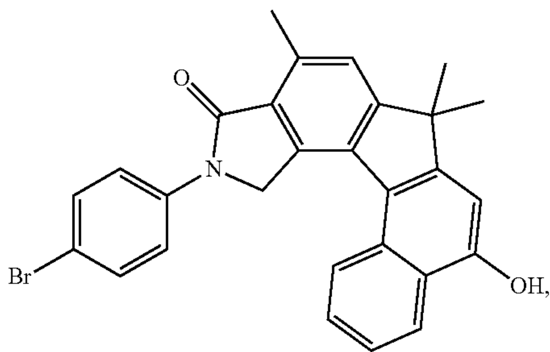
11-(4-bromophenyl)-10-oxo-7,7,9-trimethyl-7,10,11,12-tetrahydropyrrolo[3',4':4,5]indeno[3,4-a]naphthalen-5-ol
