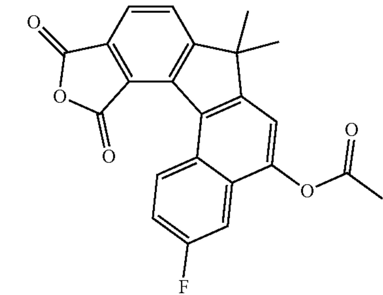
10,12-dioxo-7,7-dimethyl-3-fluoro-10,12-dihydro-7H-furo[3',4':4,5]indeno[3,2-a]naphthalen-5-yl acetate
