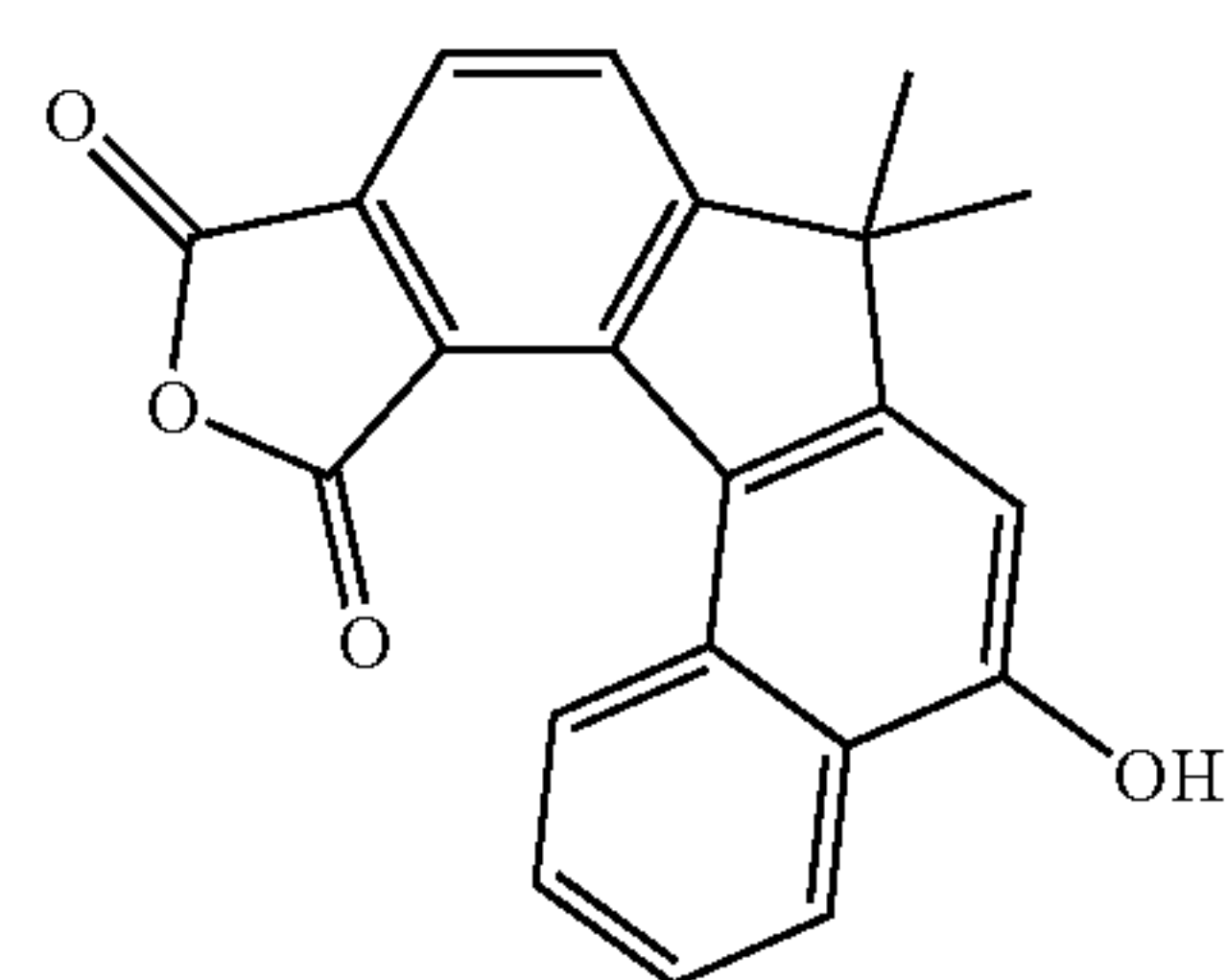
10,12-dioxo-7,7,9-trimethyl-10,12-dihydro-7H-furo[3',4':4,5]indeno[3,2-a]naphthalen-5-ol
