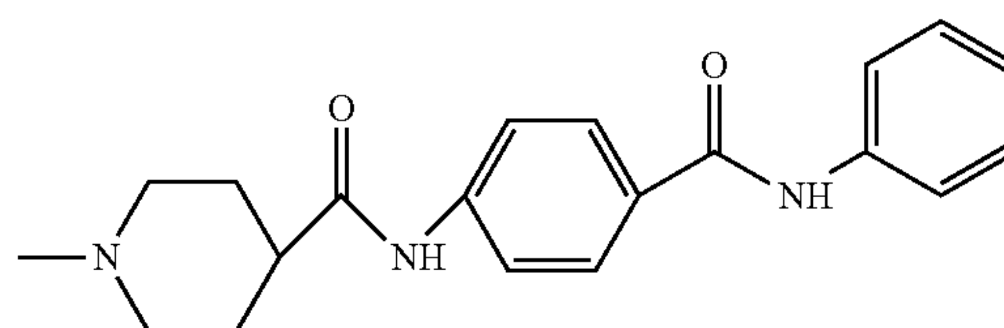
4-(4-phenylcarbomoyl-phenylcarbomoyl)-piperidin-1-yl
