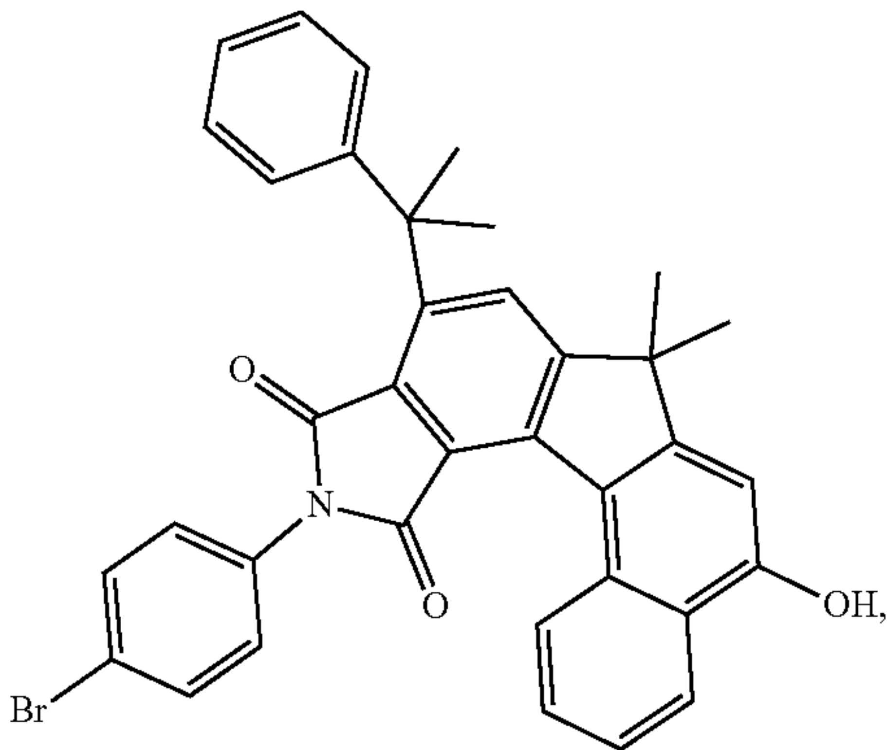
11-(4-bromophenyl)-10,12-dioxo-7,7-dimethyl-9-(2-phenylpropan- 2-yl)-7,10,11,12-tetrahydropyrrolo[3',4':4,5]indeno[3,2-a] naphthalen-5-ol.
