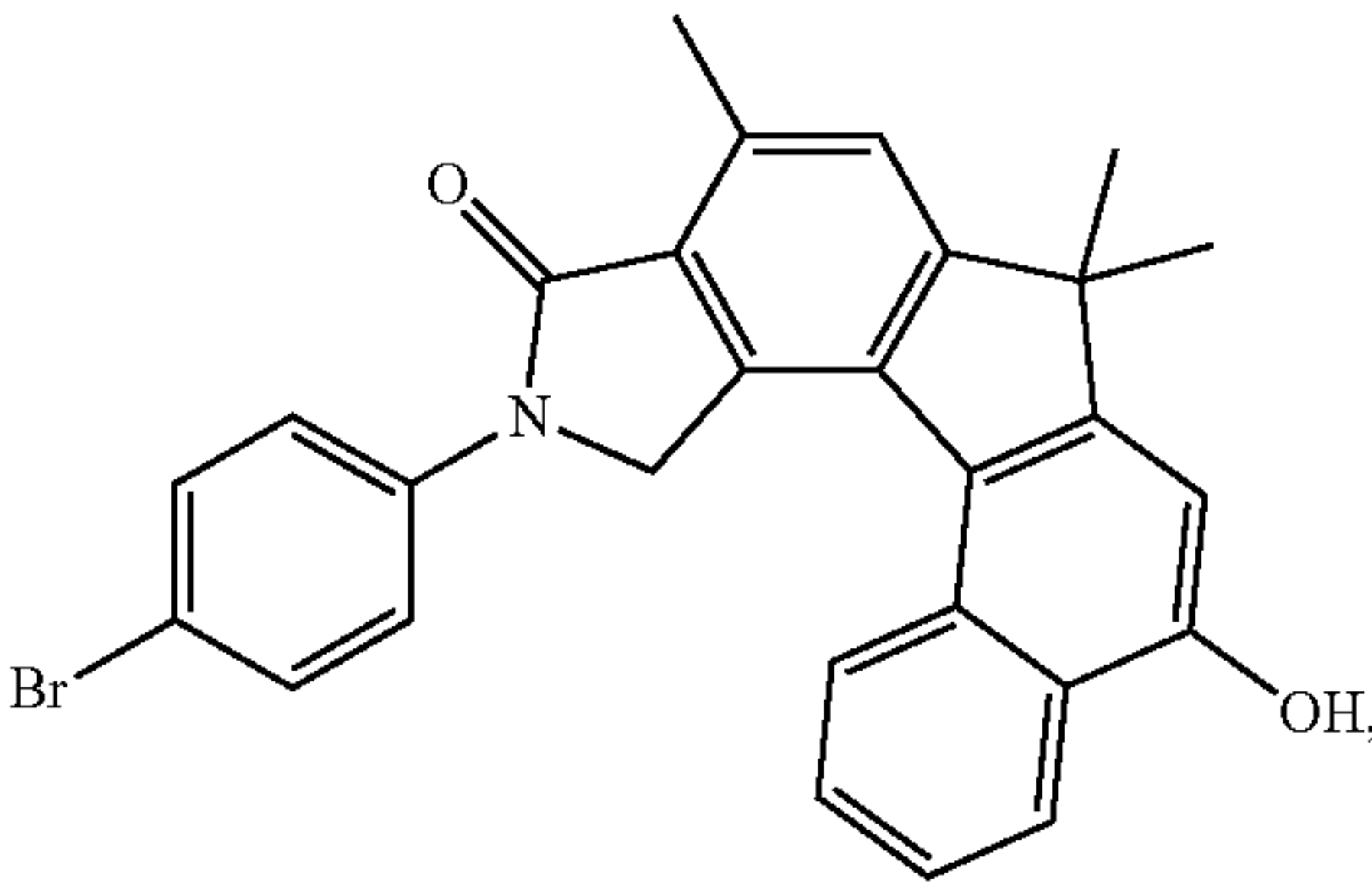
11-(4-bromophenyl)-10-oxo-7,7,9-trimethyl-7,10,11,12-tetrahydropyrrolo[3',4':4,5]indeno[3,2-a]naphthalen-5-ol
