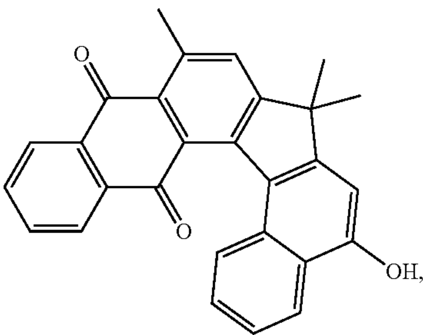
10,15-dioxo-7,7,9-trimethyl-10,15-dihydro-7H-naphthol[2',3':4,5]indeno[3,2-a]naphthalen-5-ol
