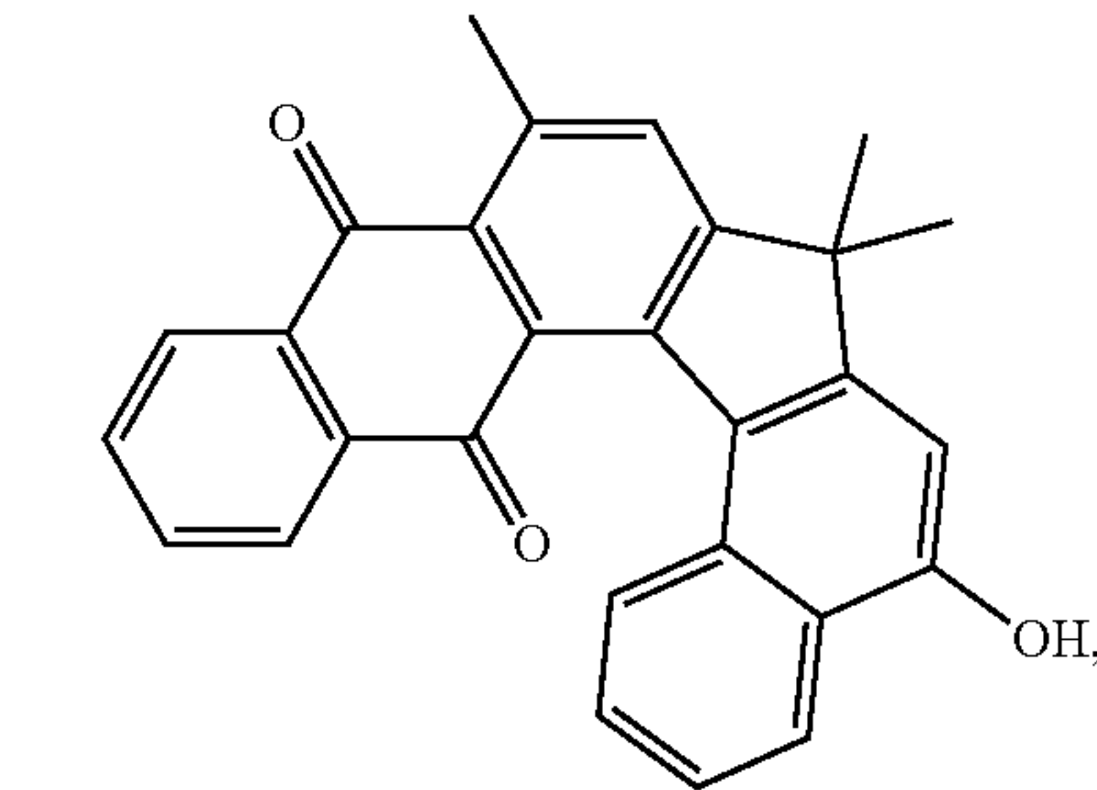
10,15-dioxo-7,7,9-trimethyl-10,15-dihydro-7H-naphtho[2',3':4,5]indeno[3,2-a]naphthalen-5-ol
