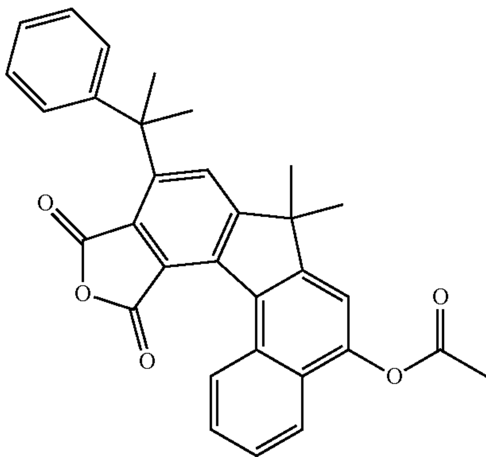
10,12-dioxo-7,7-dimethyl-9-(2-phenylpropan-2-yl)- 10,12-dihydro-7H-furo[3',4':4,5]indeno[3,2-a]naphthalen- 5-yl acetate.
