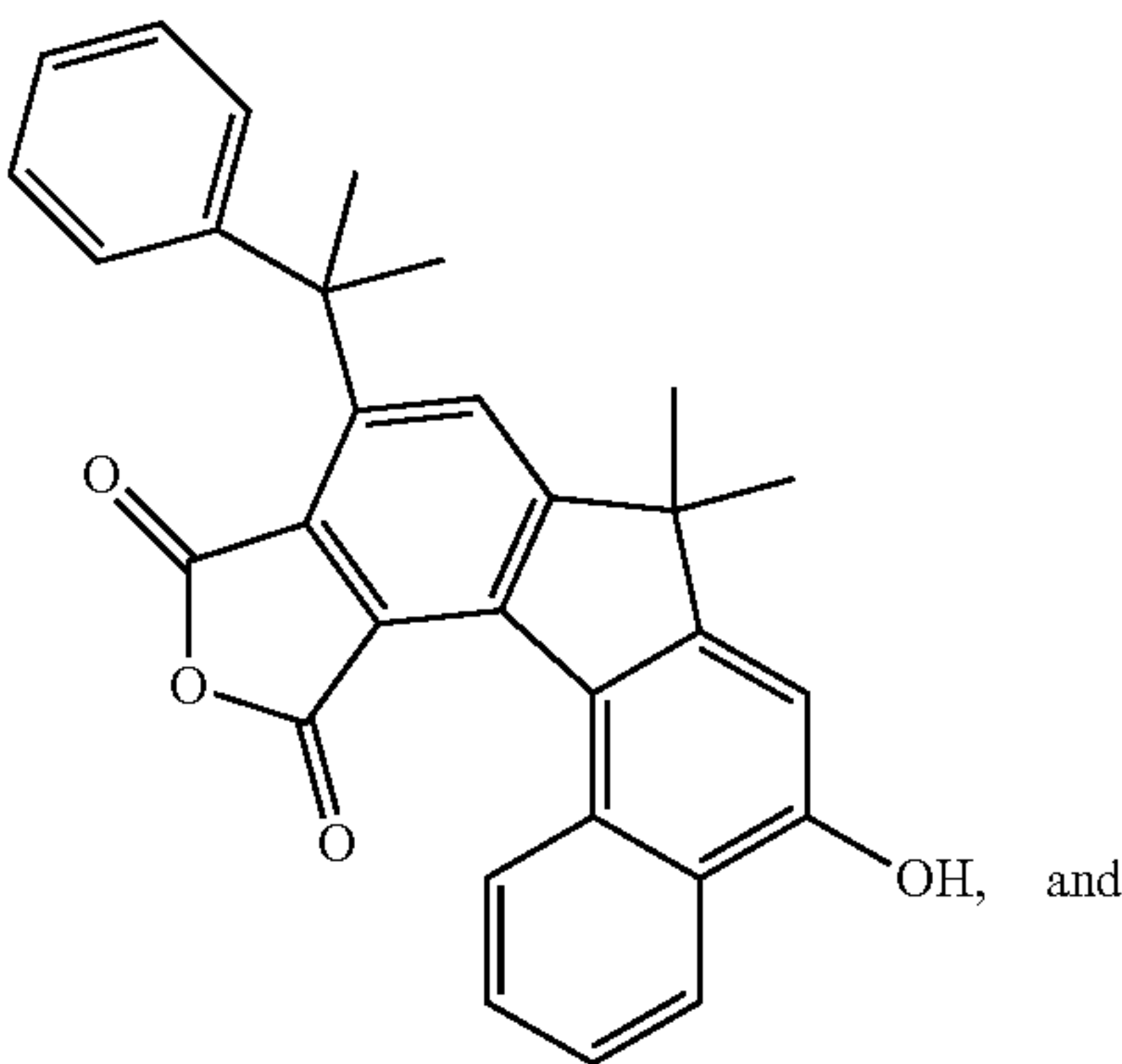
10,12-dioxo-7,7-dimethyl-9- (2-phenylpropan-2-yl)- 10,12-dihydro-7H-furo[3',4':4,5] indeno[3,2-a]naphthalen-5-ol.
