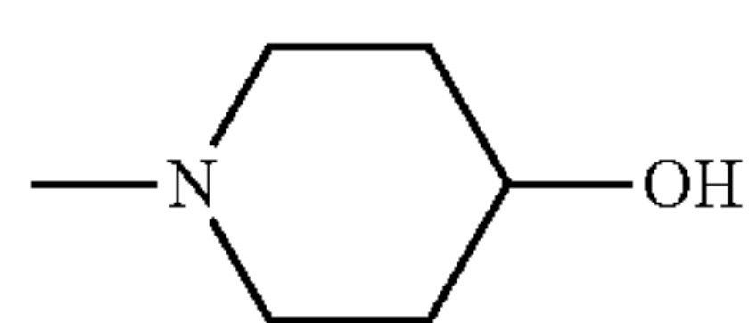
4-hydroxy-piperidin-1-yl
