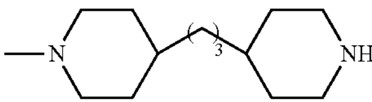
4-(3-piperidin-4-yl-propyl)-piperidin-1-yl
