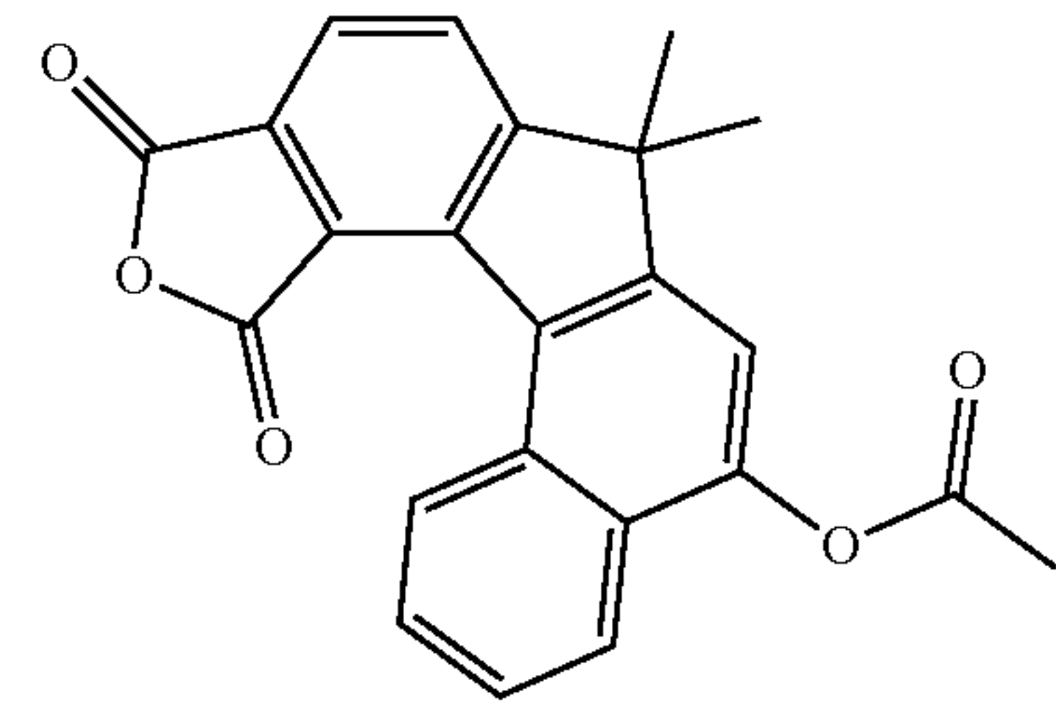
10,12-dioxo-7,7-dimethyl-10,12-dihydro-7H-furo[3',4':4,5]indeno[3,2-a]naphthalen-5-yl acetate
