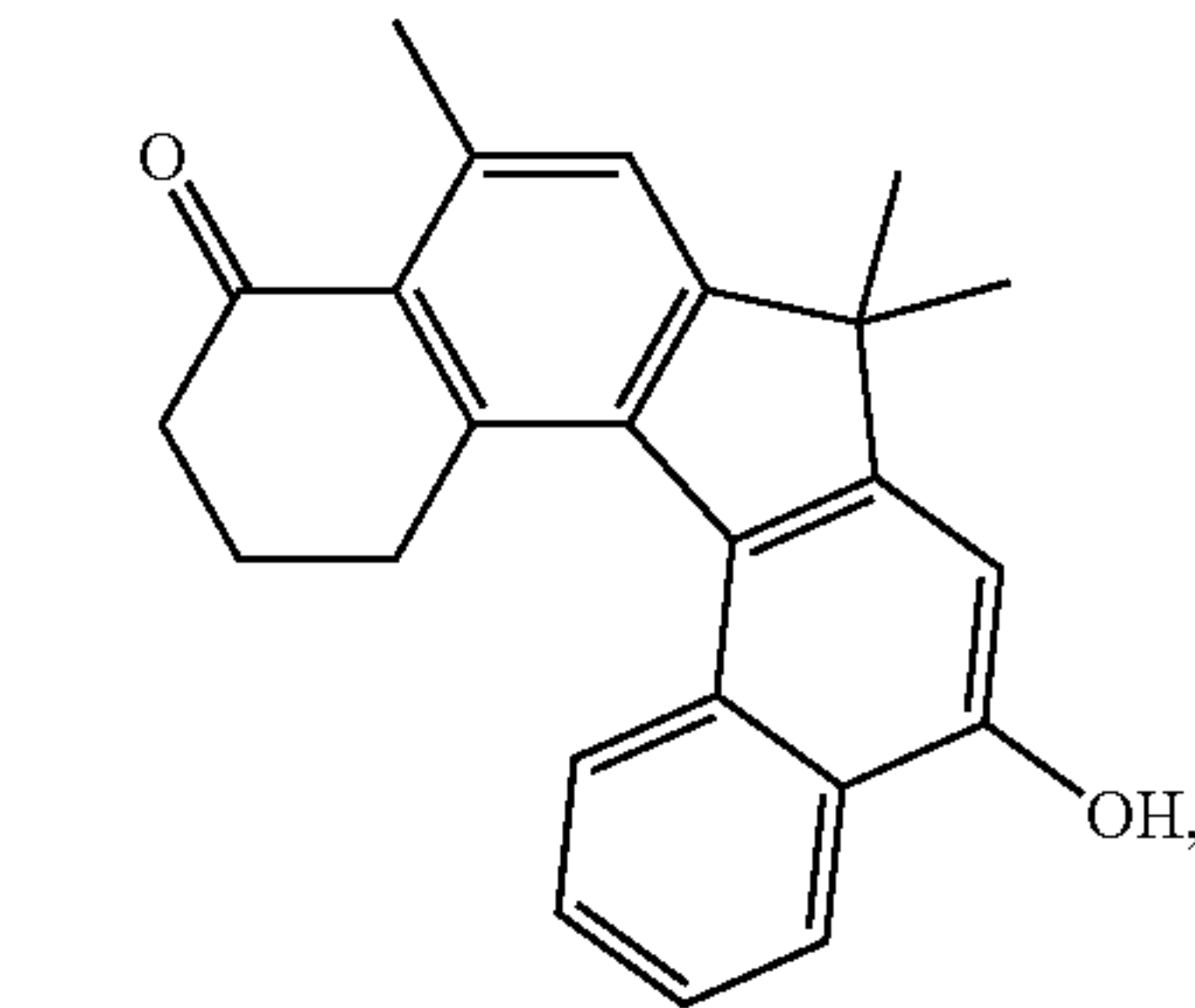
10-oxo-7,7,9-trimethyl-10,11,12,13-tetrahydro-7H-benzo[4,5]indeno[3,2-a]naphthalen-5-ol
