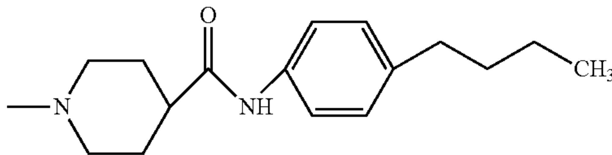
4-(4-butyl-phenylcarbamoyl)-piperidin-1-yl
