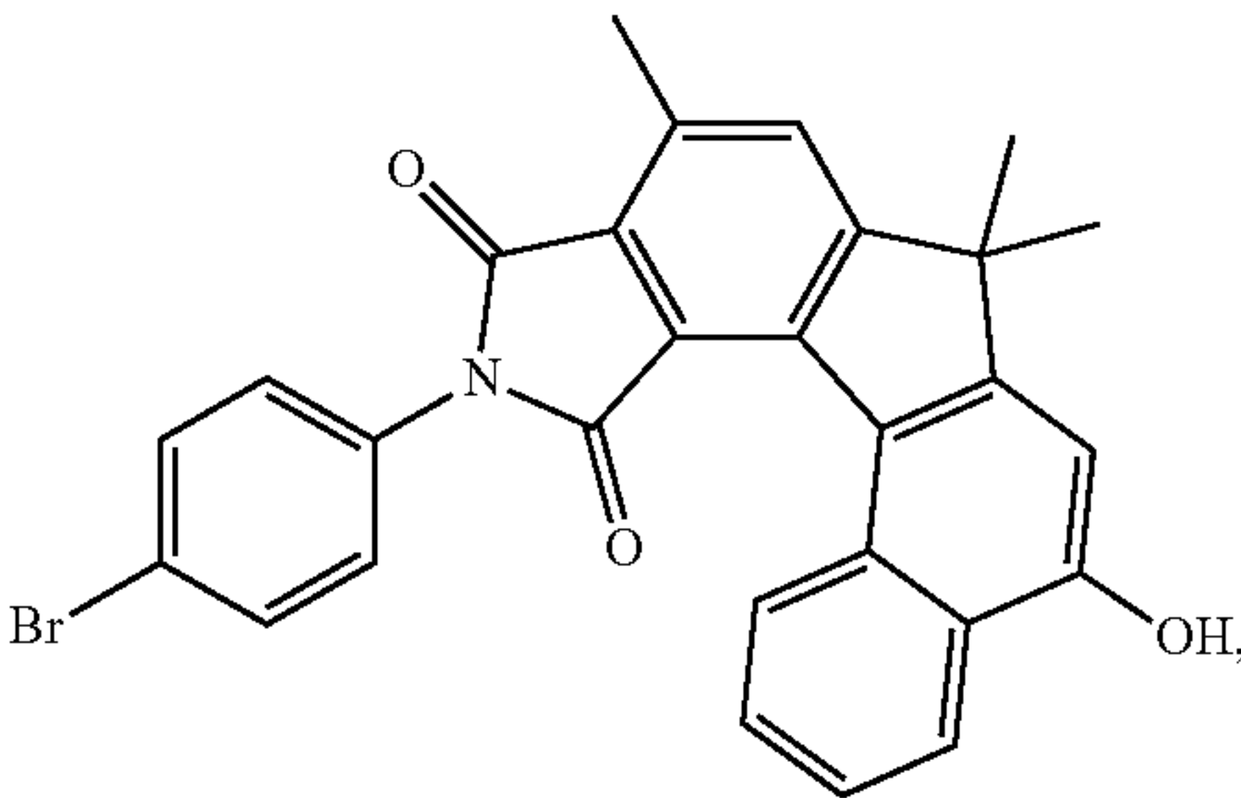
11-(4-bromophenyl)-10,12-dioxo-7,7,9-trimethyl-7,10,11,12- tetrahydropyrrolo[3',4':4,5]indeno[3,2-a]naphthalen-5-ol
