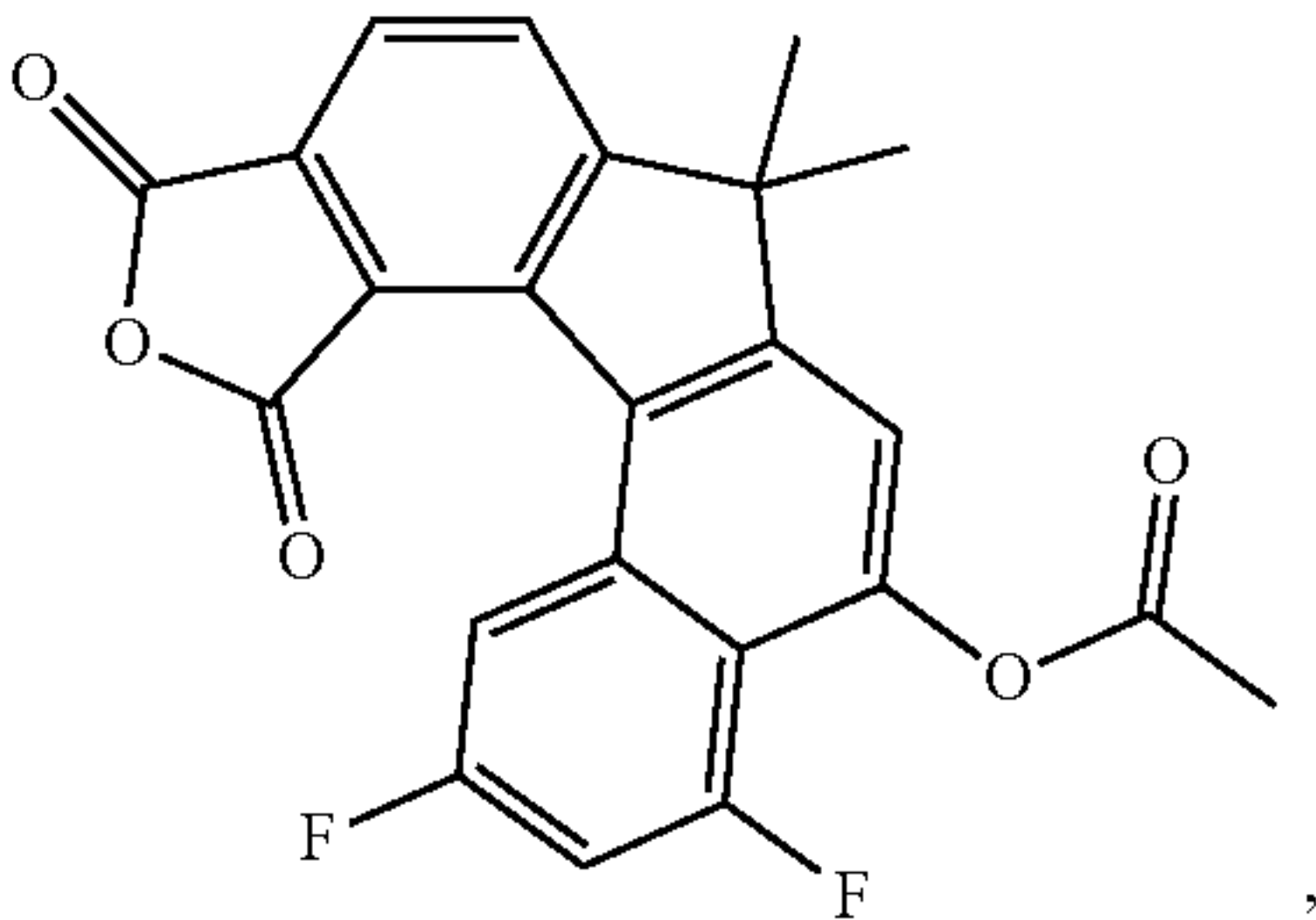
10,12-dioxo-7,7-dimethyl-2,4-difluoro-10,12-dihydro-7H-furo[3',4':4,5]indeno[3,2-a]naphthalen-5-yl acetate
