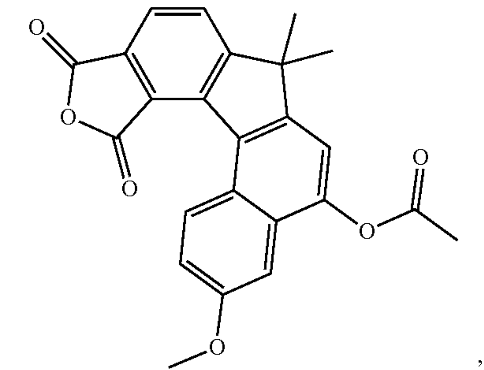
10,12-dioxo-7,7-dimethyl-3-methoxy-10,12-dihydro-7H-furo[3',4':4,5]indeno[3,2-a]naphthalen-5-yl acetate
