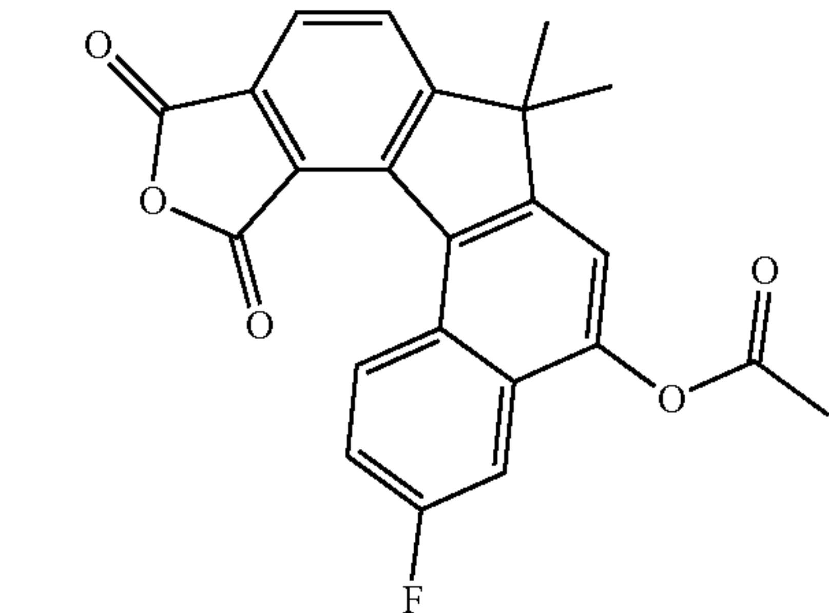
10,12-dioxo-7,7-dimethyl-3-fluoro-10,12-dihydro-7H-furo [3',4':4,5]indeno[3,2-a]naphthalen-5-yl acetate
