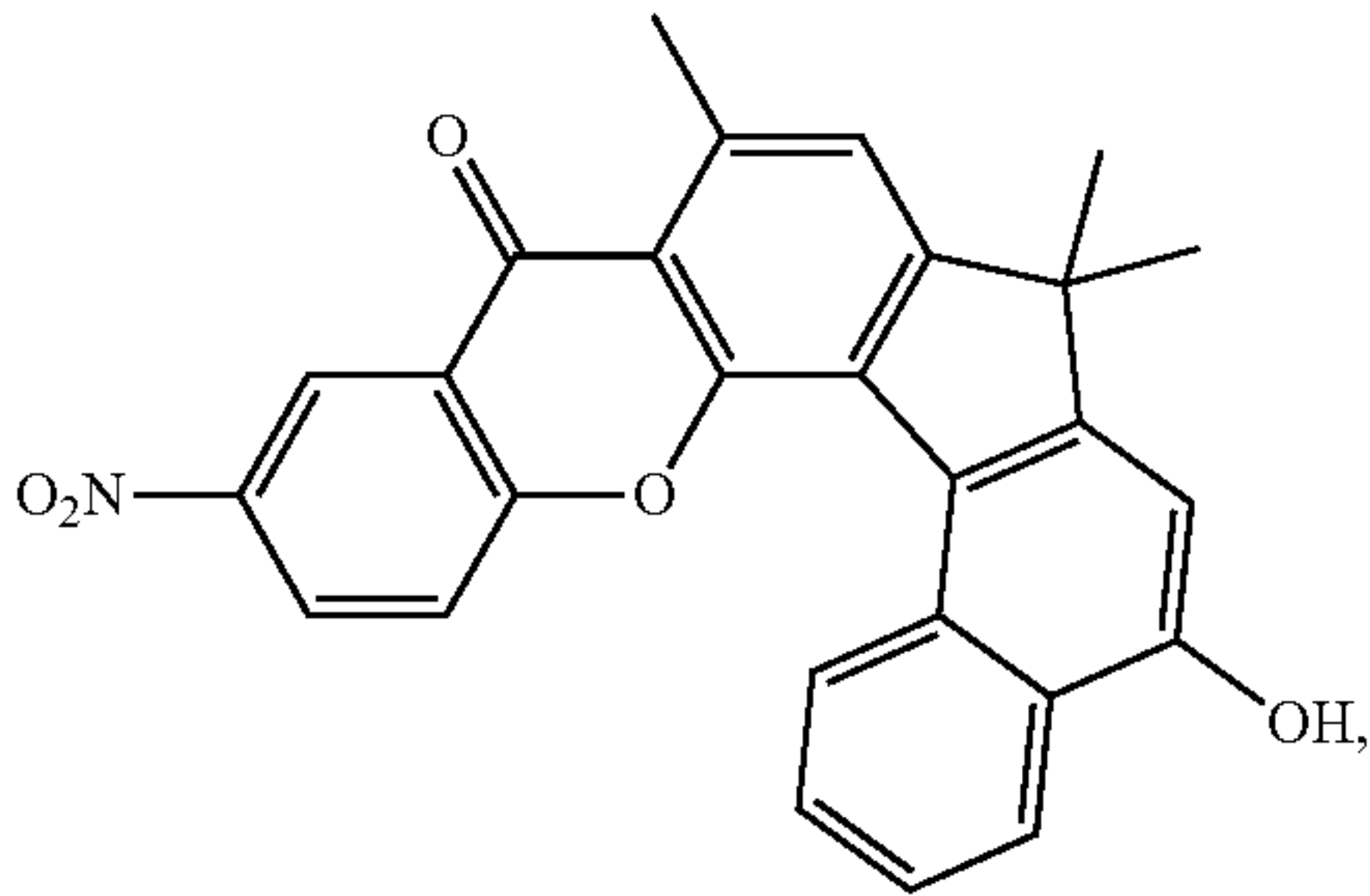
12-nitro-10-oxo-7,7,9-trimethyl-7H-chromeno [3',2':4,5]indeno[3,2-a]naphthalen-5-ol
