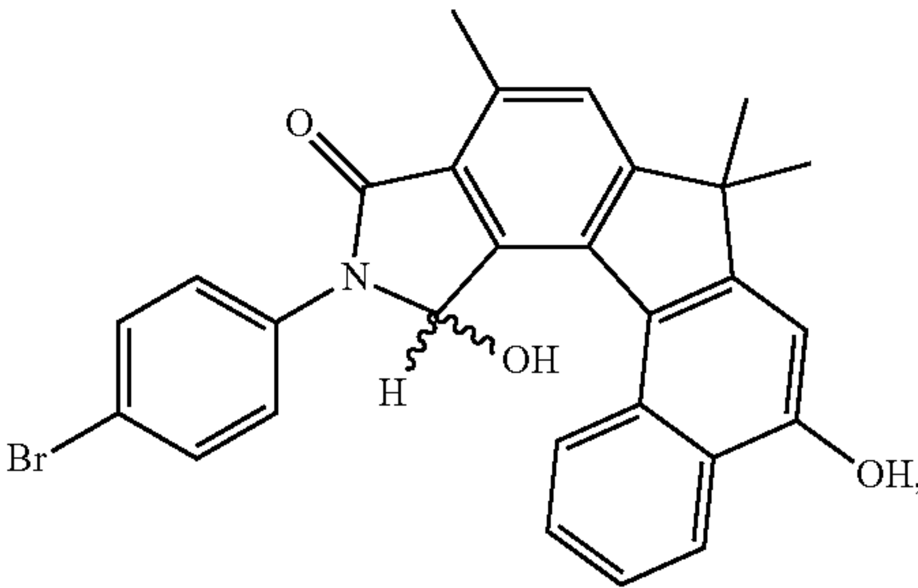
11-(4-bromophenyl)-12-hydroxy-10-oxo-7,7,9-trimethyl-7,10,11,12-tetrahydropyrrolo[3',4':4,5]indeno[3,2-a]naphthalen-5-ol
