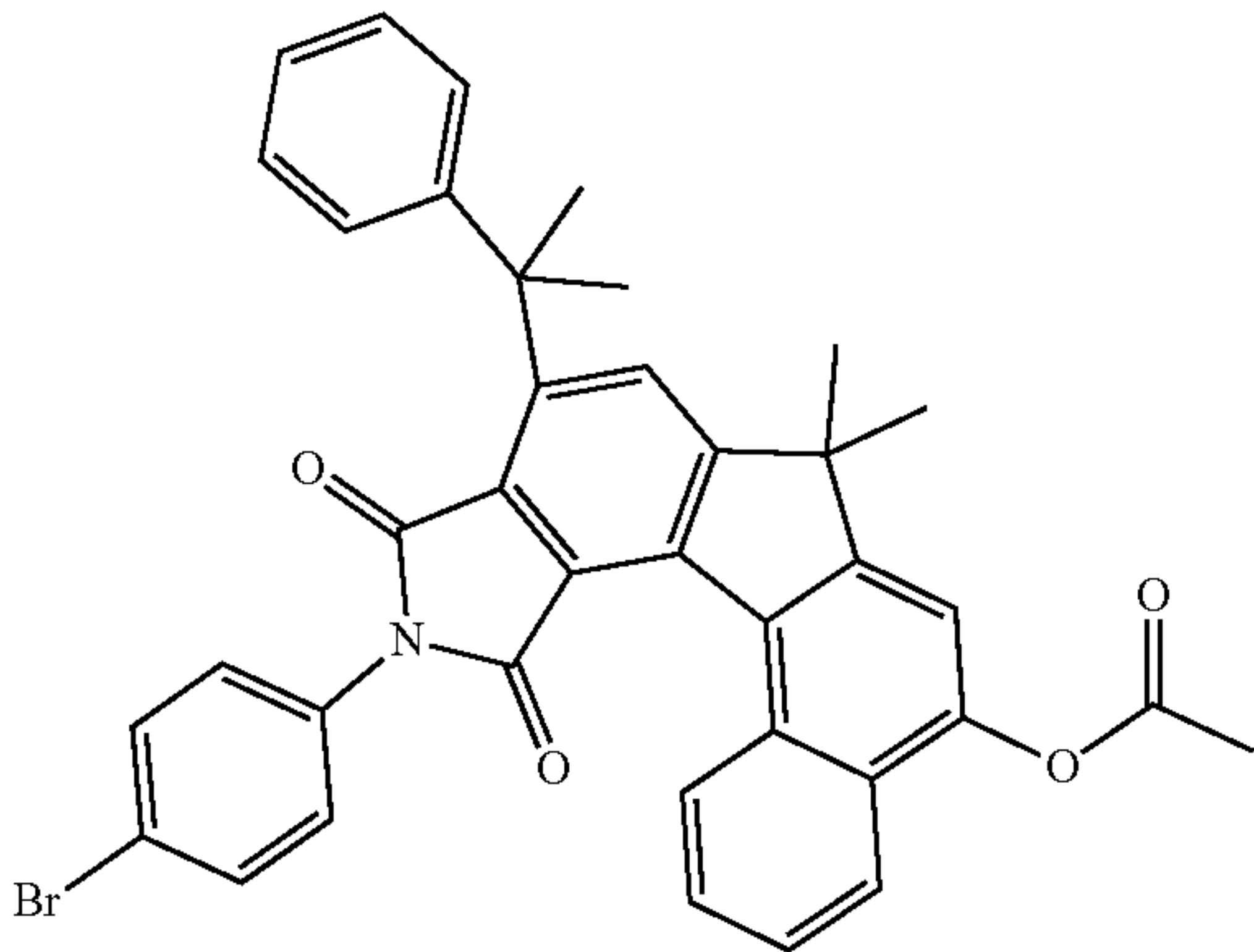
11-(4-bromophenyl)-10,12-dioxo-7,7-dimethyl-9-(2-phenylpropan- 2-yl)-7,10,11,12-tetrahydropyrrolo[3',4':4,5]indeno[3,2-a] naphthalen-5-yl acetate.
