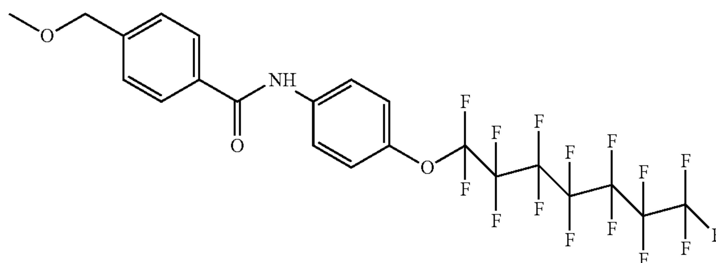
4-(4-pentadecafluoroheptyloxy-phenylcarbomoyl)-benzyloxy
