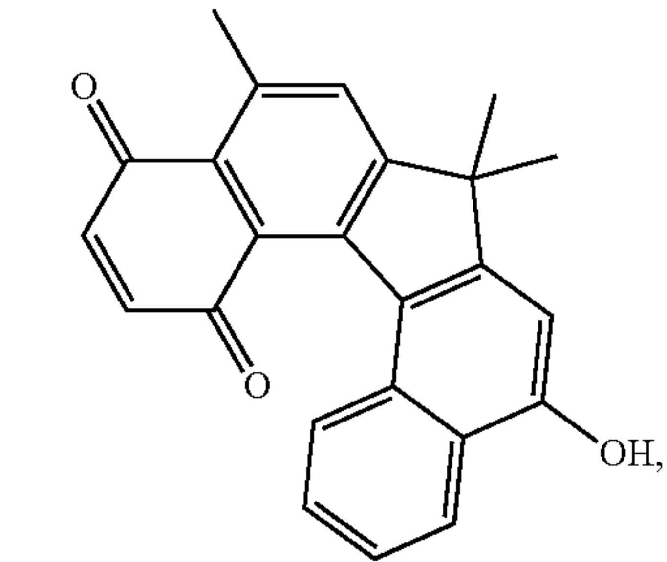
10,13-dioxo-7,7,9-trimethyl-10,13-dihydro-7H-benzo[4,5]indeno[3,2-a]naphthalen-5-ol
