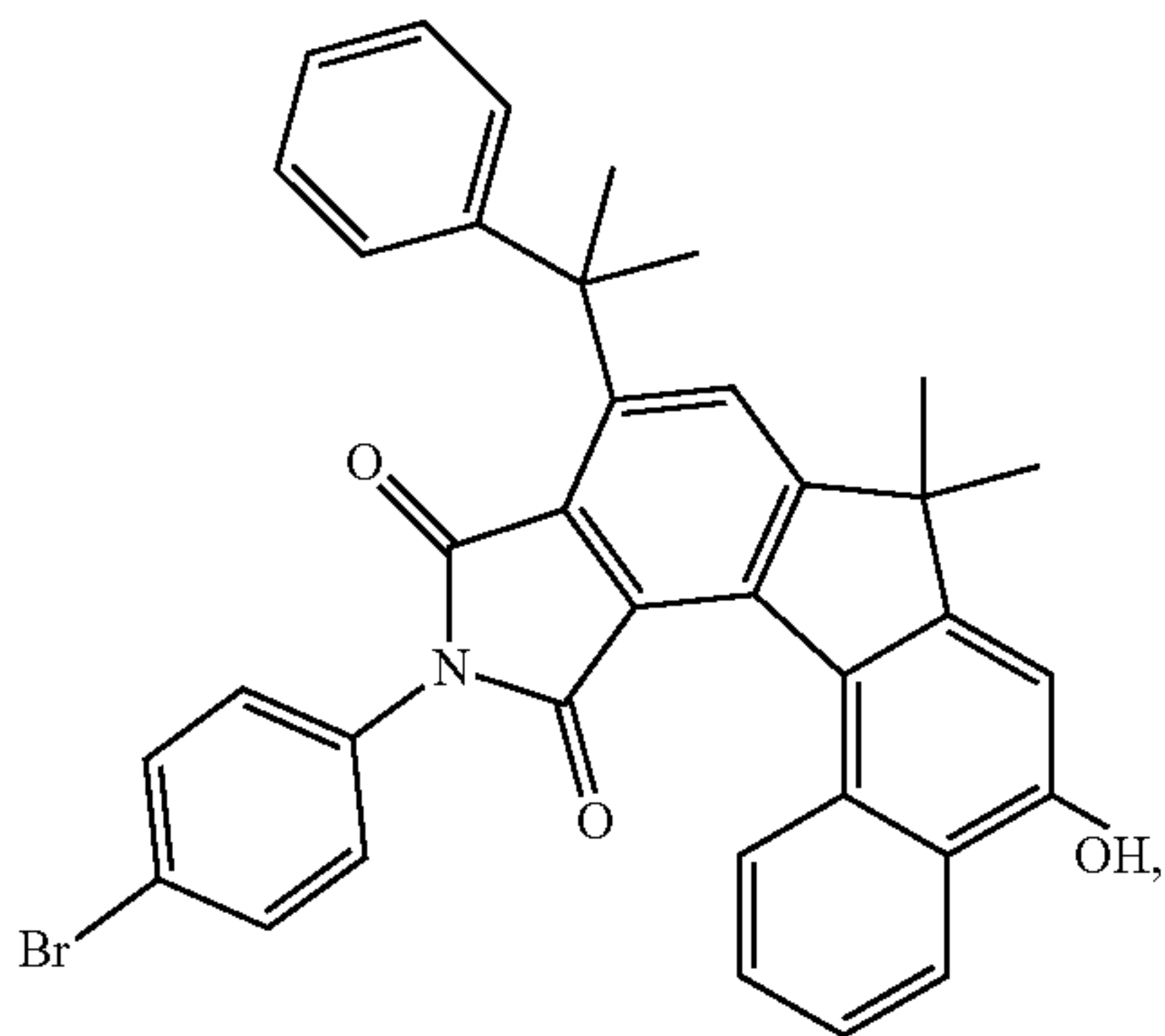
11-(4-bromophenyl)-10,12-dioxo-7,7-dimethyl-9- (2-phenylpropan-2-yl)-7,10,11,12-tetrahydropyrrolo [3',4':4,5]indeno[3,2-a]naphthalen-5-ol.
