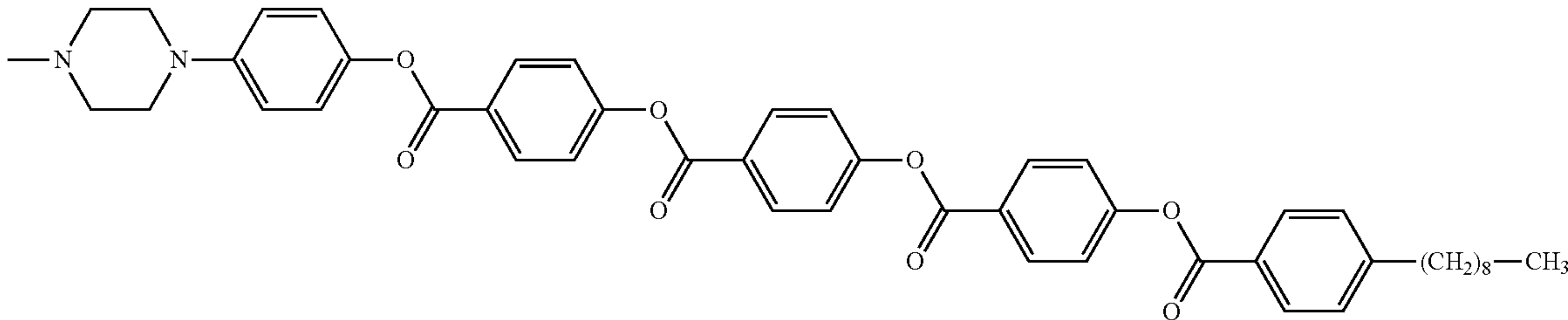
4-(4'-propyl-biphenyl-4-ylethynyl)-phenyl
