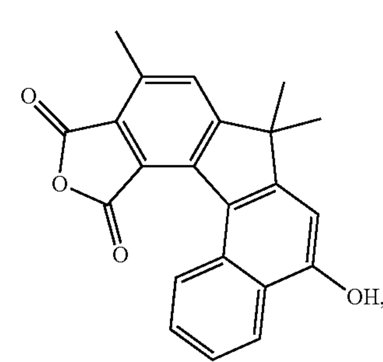
10,12-dioxo-7,7,9-trimethyl-10,12-dihydro-7H-furo [3',4':4,5]indeno[3,2-a]naphthalen-5-ol
