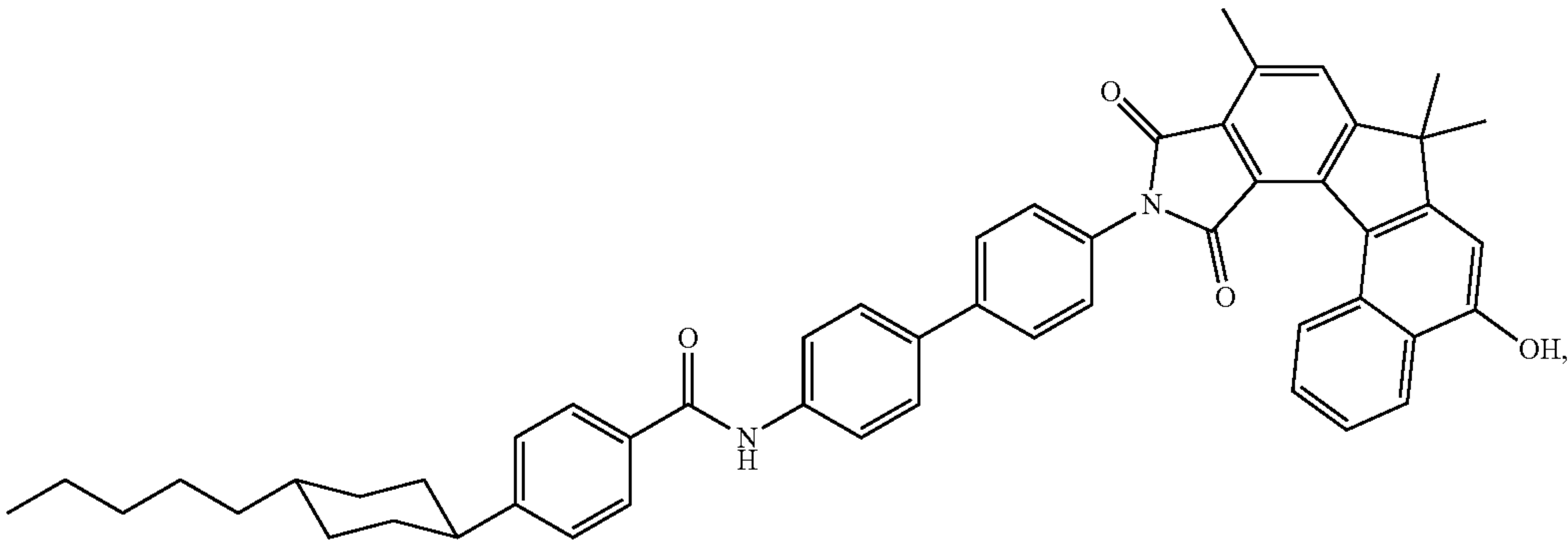
11-(4'-(4-(trans-4-pentylcyclohexyl)benzamido)-[1,1'-biphenyl])-10,12-dioxo-7,7,9-trimethyl-7,10,11,12-tetrahydropyrrolo[3',4':4,5]indeno[3,2-a]naphthalen-5-ol
