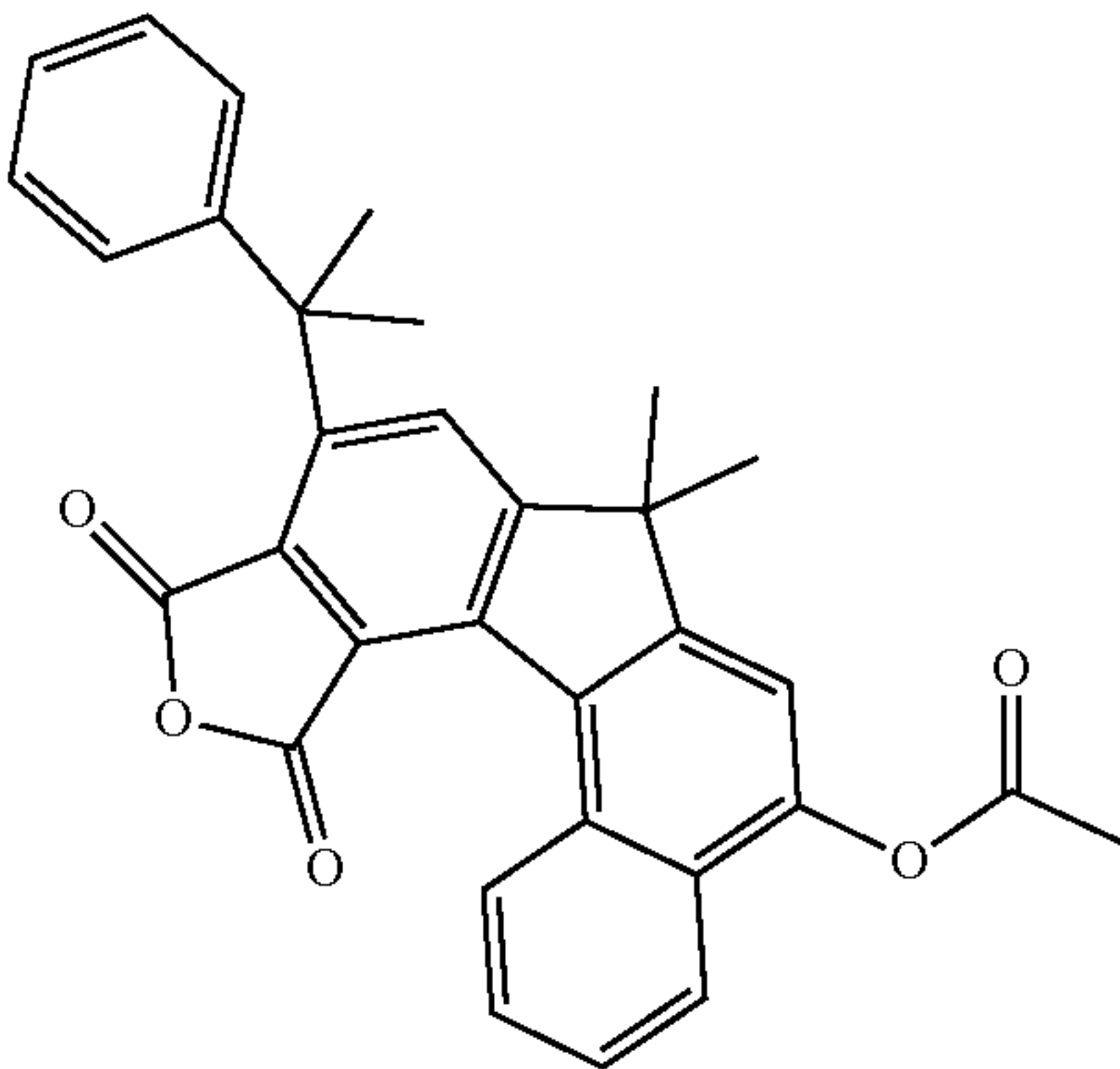
10,12-dioxo-7,7-dimethyl-9-(2-phenylpropan-2-yl)- 10,12-dihydro-7H-furo[3',4':4,5]indeno[3,2-a] naphthalen-5-yl acetate.
