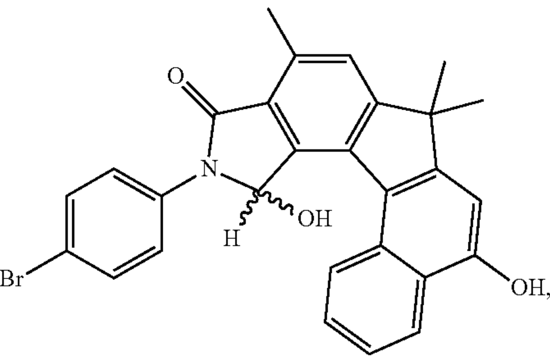
11-(4-bromophenyl)-12-hydroxy-10-oxo-7,7,9-trimethyl-7,10,11,12-tetrahydropyrrolo[3',4':4,5]indeno[3,4-a]naphthalen-5-ol
