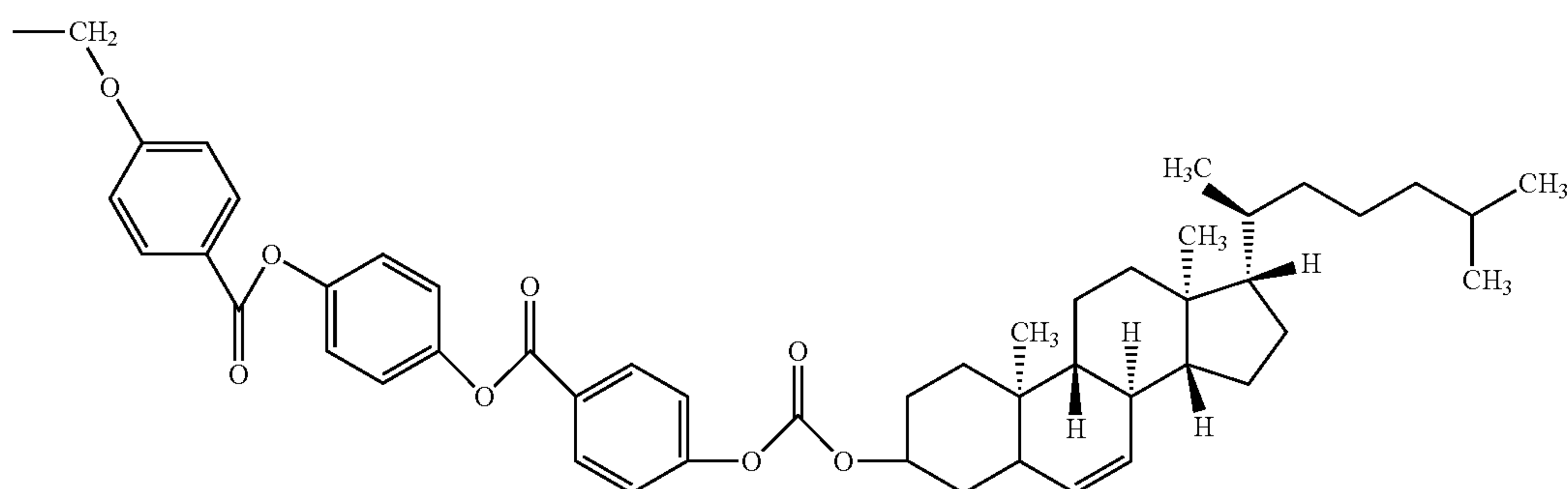
4-(4-{4-[17-(1,5-dimethyl-hexyl)-10,13-dimethyl-2,3,4,7,8,9,10,11,12,13,14,15,16,17-tetradecahydro-1H-cyclopenta[a]phenanthren-3-yloxy-carbonyloxy]-benzoyloxy}-phenoxy-carbonyl)-phenoxy-methyl
