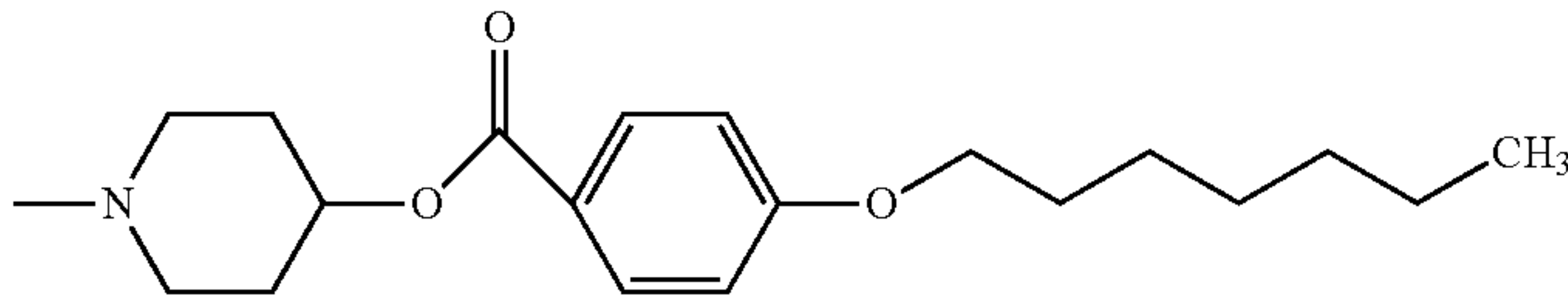
4-(4-hexyloxy-benzoyloxy)-piperidin-1-yl]
