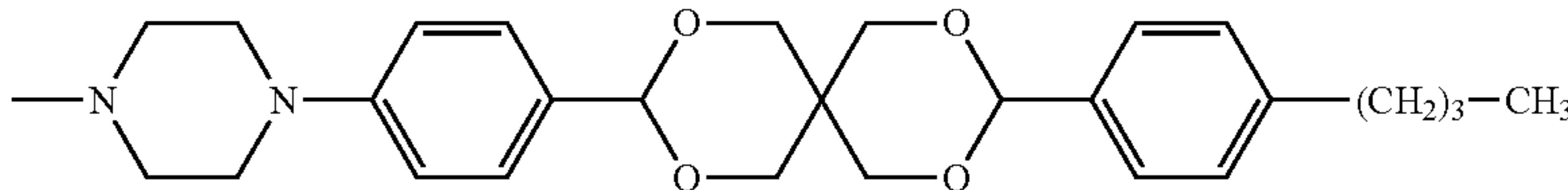
4-(4-(9-(4-butylphenyl)-2,4,8,10-tetraoxaspiro[5.5]undec-3-yl)phenyl)piperazin-1-yl
