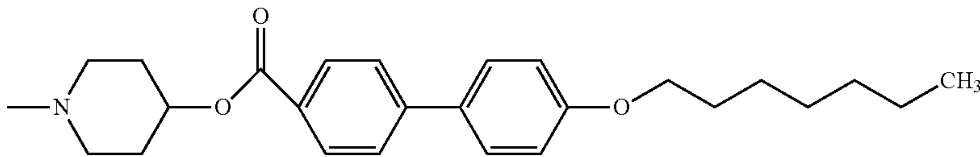
4-(4'-hexyloxy-biphenyl-4-carbonyloxy)-piperidin-1-yl
