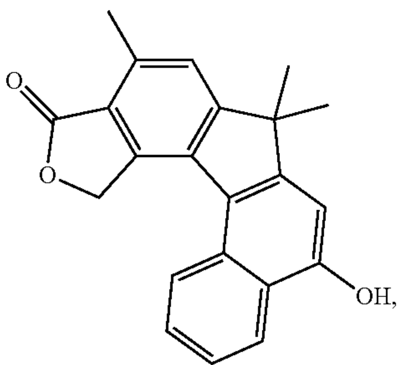
10-oxo-7,7,9-trimethyl-10,12-dihydro-7H-furo[3',4':4,5]indeno[3,2-a]naphthalen-5-ol
