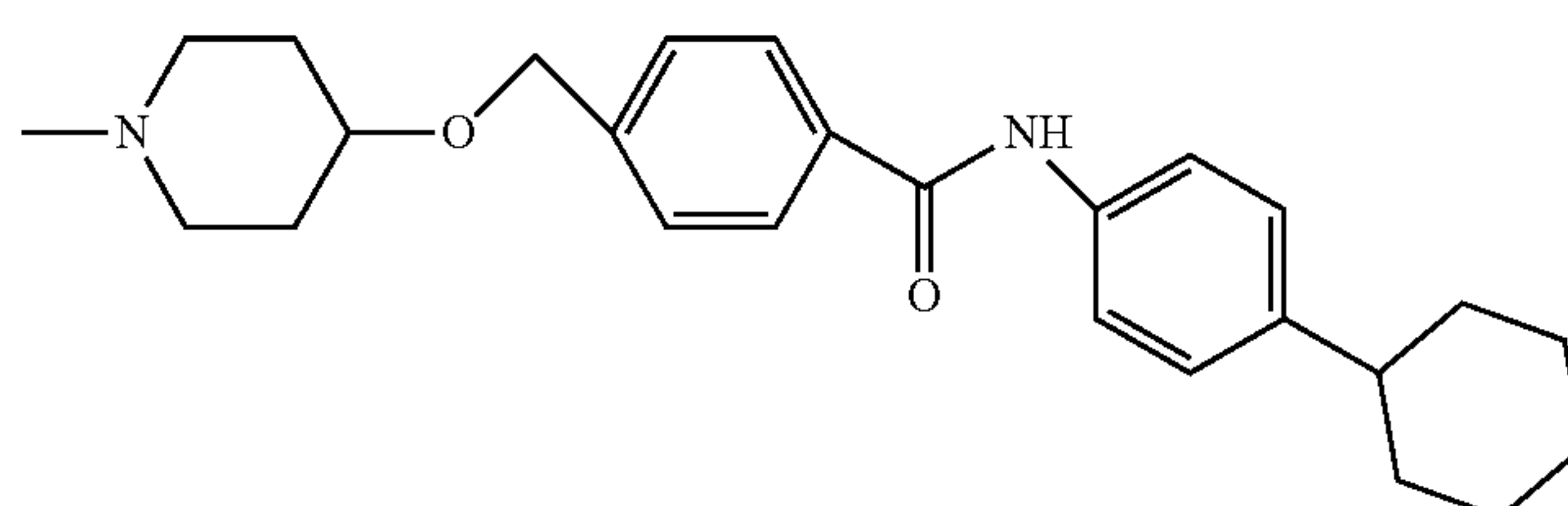
4-[4-(4-cyclohexyl-phenylcarbomoyl)-benzyloxy]-piperidin-1-yl
