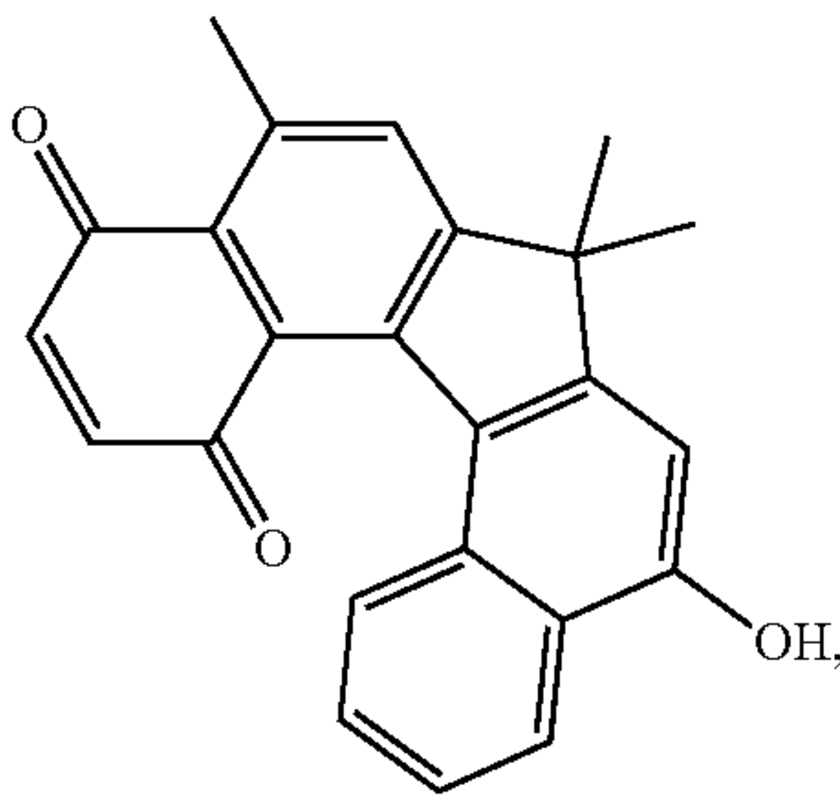
10,13-dioxo-7,7,9-trimethyl-10,13-dihydro-7H-benzol[4,5]indeno[3,2-a]naphthalen-5-ol
