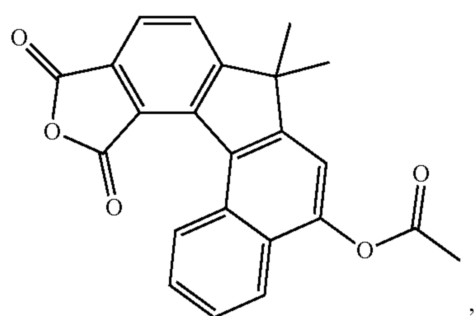
10,12-dioxo-7,7,9-trimethyl-10,12-dihydro-7H-furo[3',4':4,5]indeno[3,2-a]naphthalen-5-yl acetate
