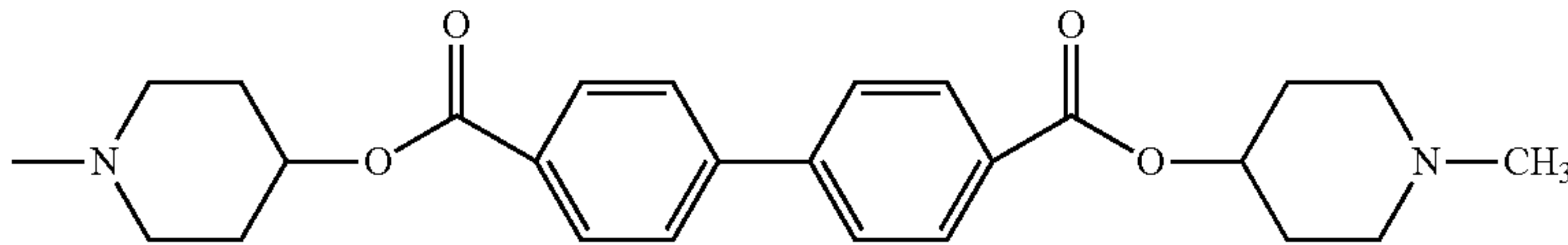
1-methyl-4((4'(((1-methylpiperidin-4-yl)oxy)carbonyl)-[1,1'-biphenyl]-4-carbonyl)oxy)piperidin-1-yl
