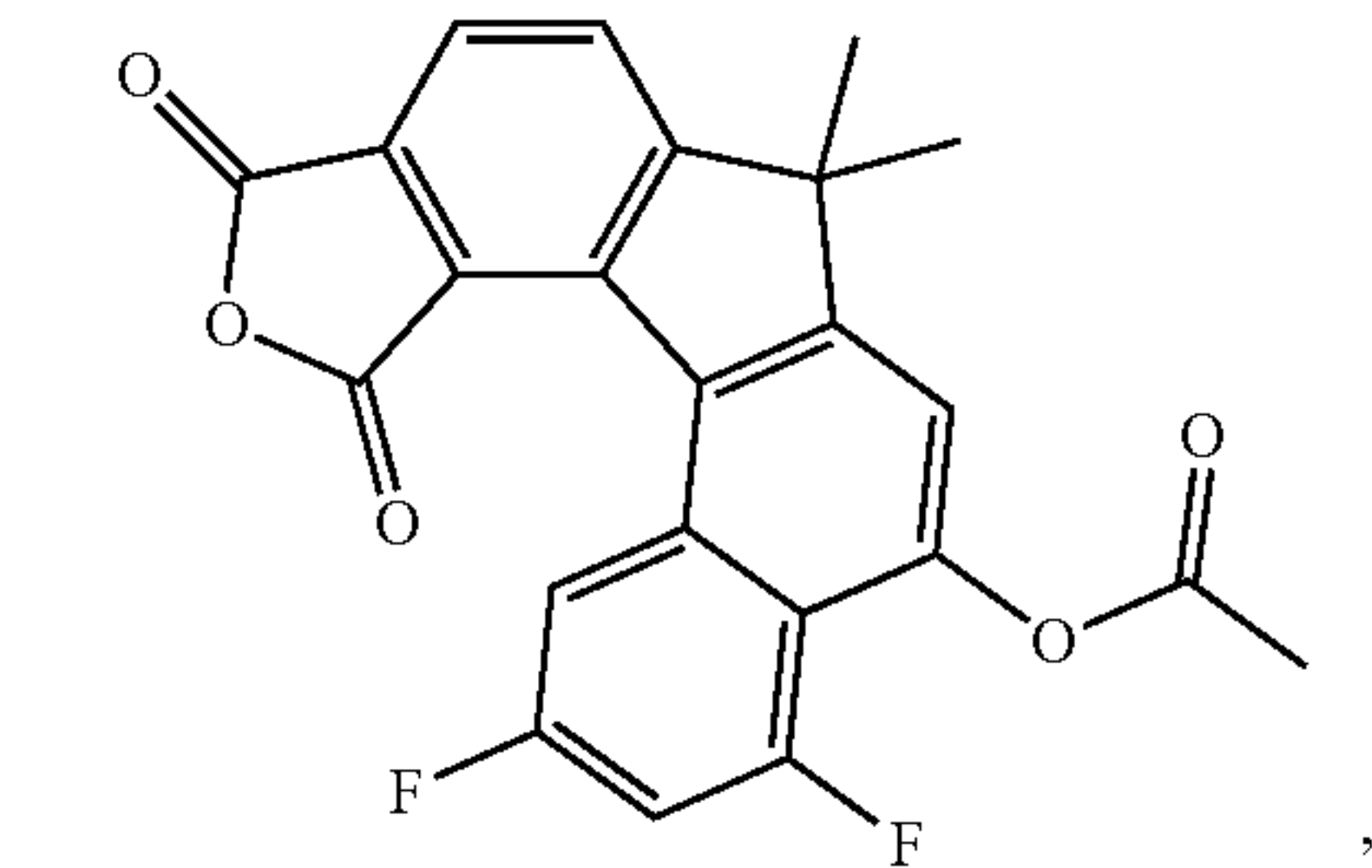
10,12-dioxo-7,7-dimethyl-2,4-difluoro-10,12-dihydro-7H-furo[3',4':4,5]indeno[3,2-a]naphthalen-5-yl acetate
