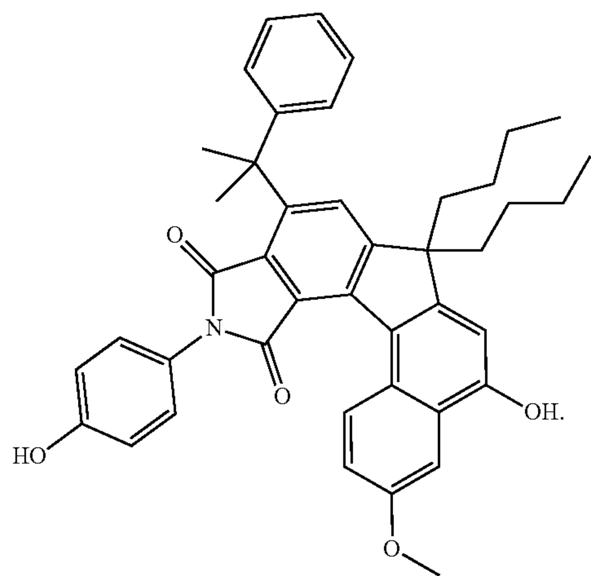
11-(4-hydroxyphenyl)-10,12-dioxo-7,7-dibutyl-3-methoxy-9-(2-phenylpropan-2-yl)-7,10,11,12-tetrahydropyrrolo [3',4':4,5]indeno[3,2-a]naphthalen-5-ol.
