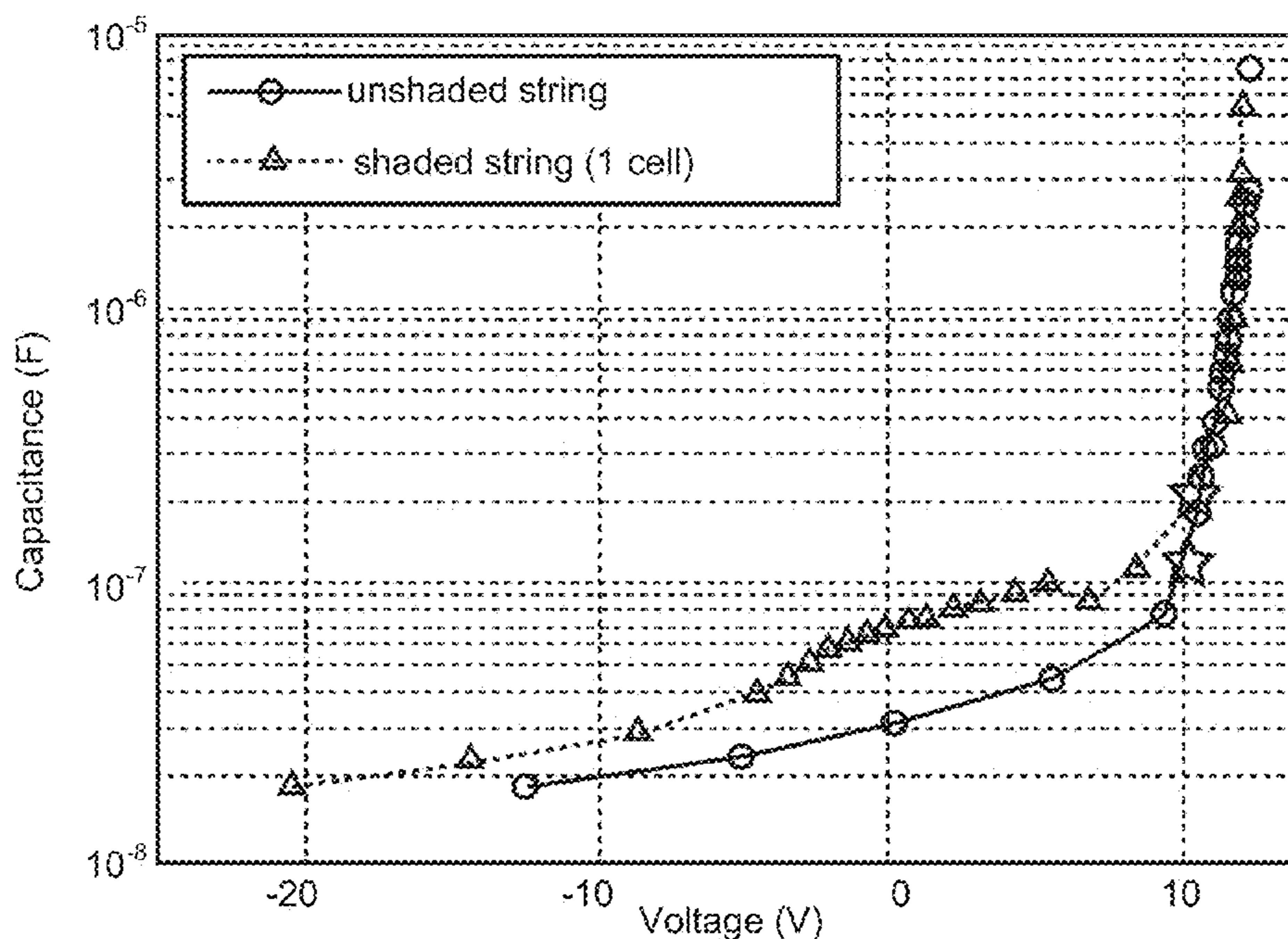
(b) calculated capacitance vs. string voltage
