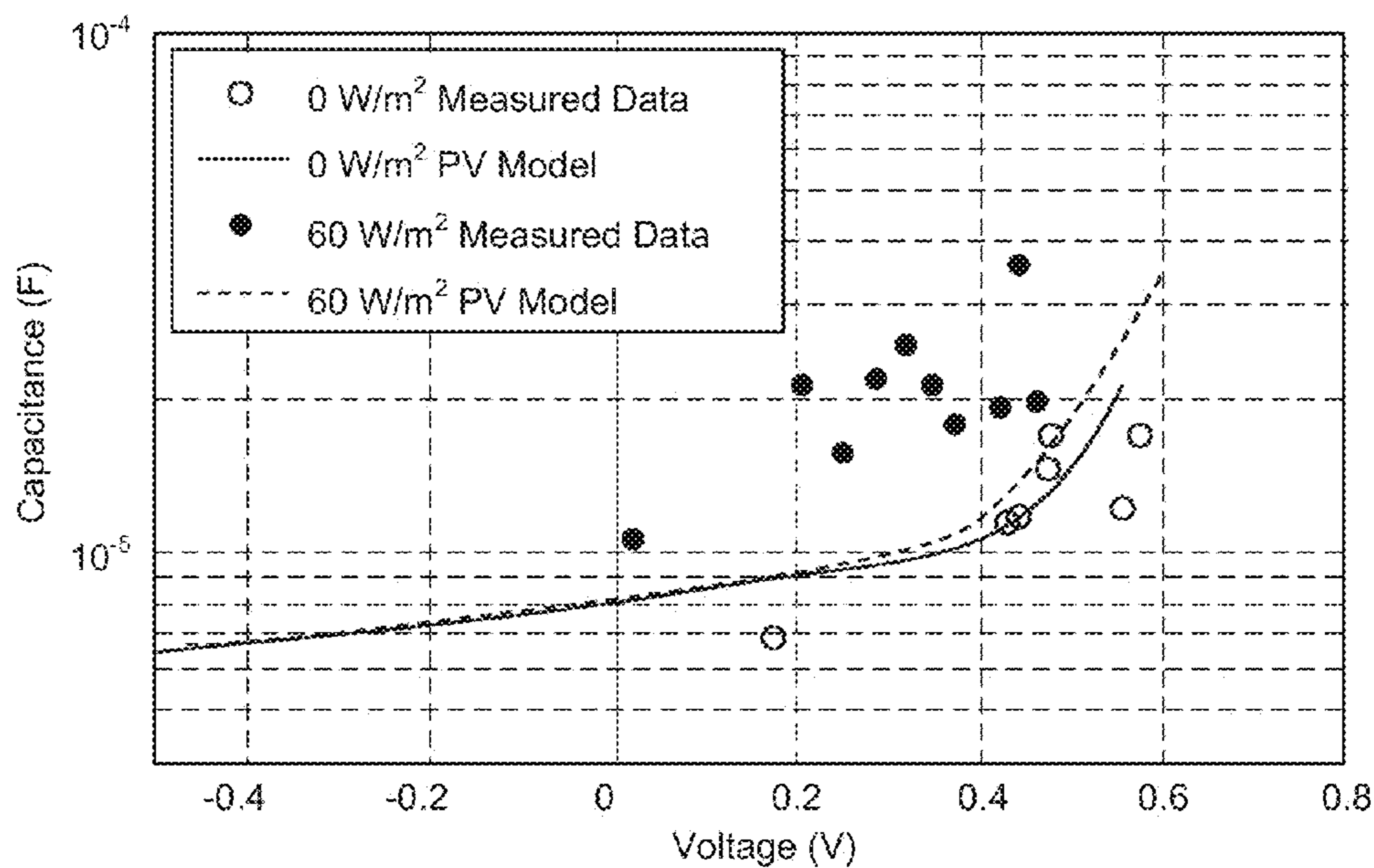
(b) Capacitance vs Voltage
