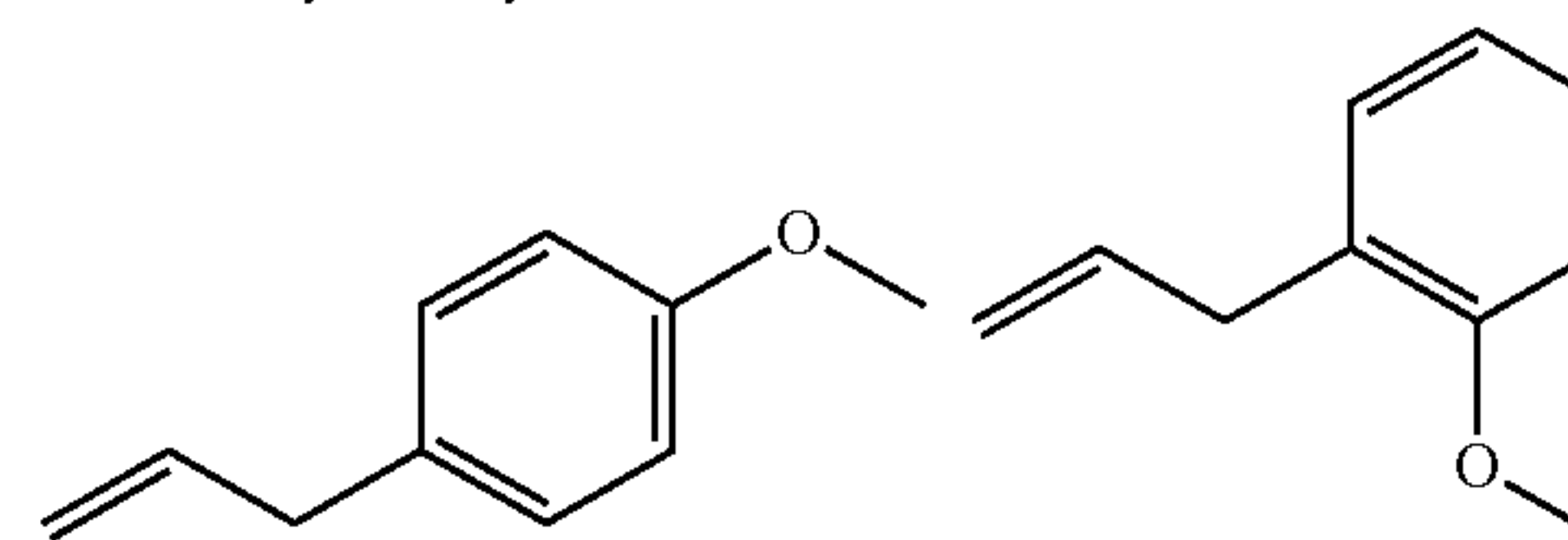
p-allylanisole
