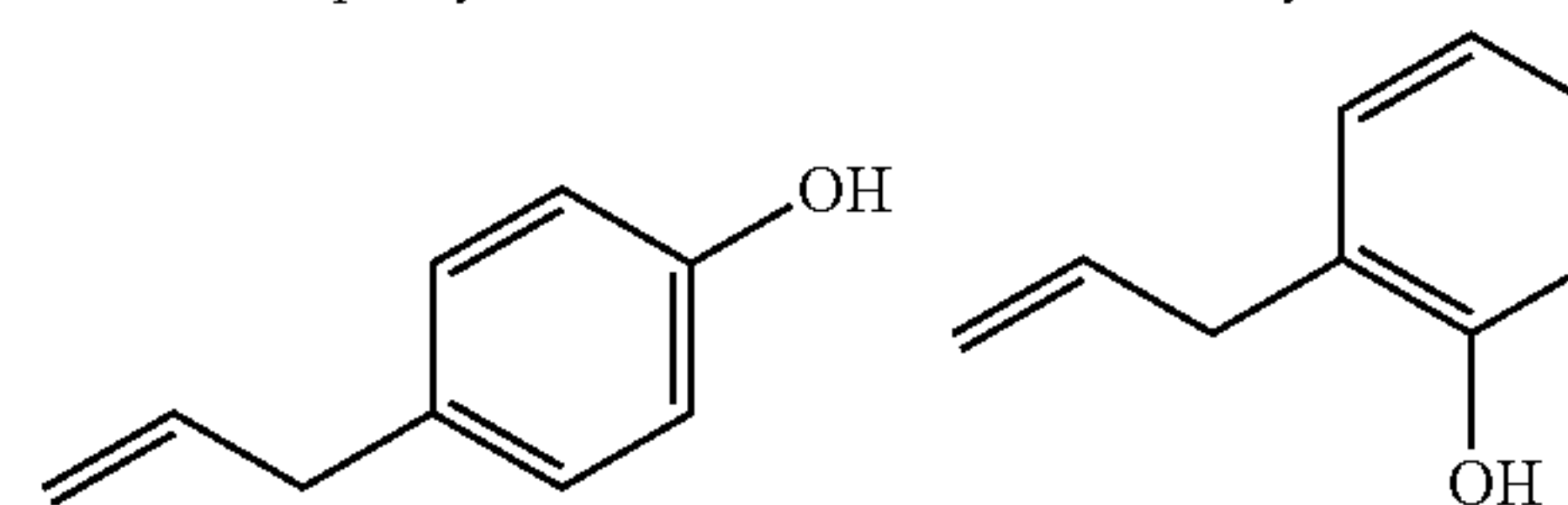
p-allylphenol
