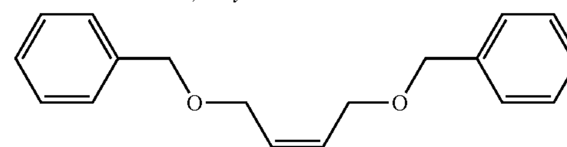
cis-1,4-bisbenzoyloxy-2-butene
