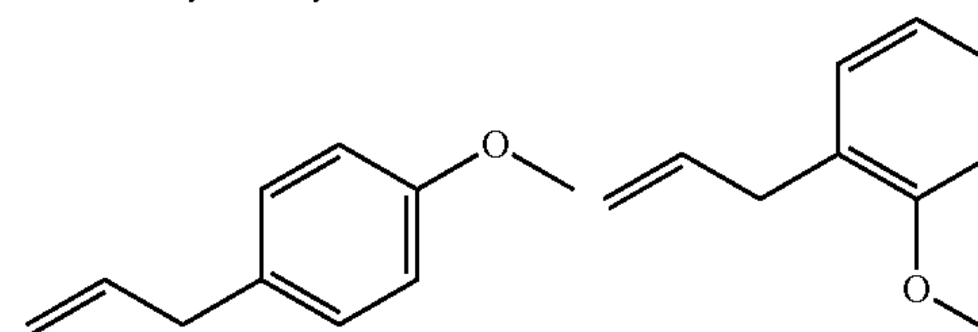
p-allylanisole
