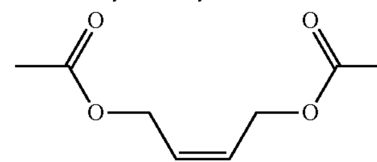
cis-2-butene-1,4-diyl-diacetate
