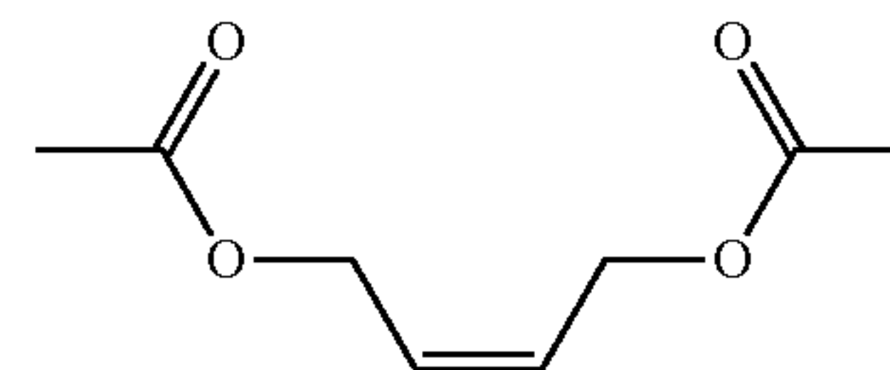
cis-2-butene-1,4-diyl-diacetate
