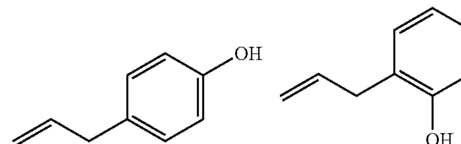
p-allylphenol
