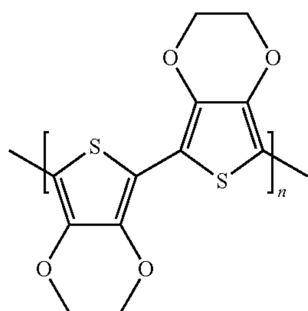
PDOT = poly(3,4-ethylenedioxythio-phenene)
