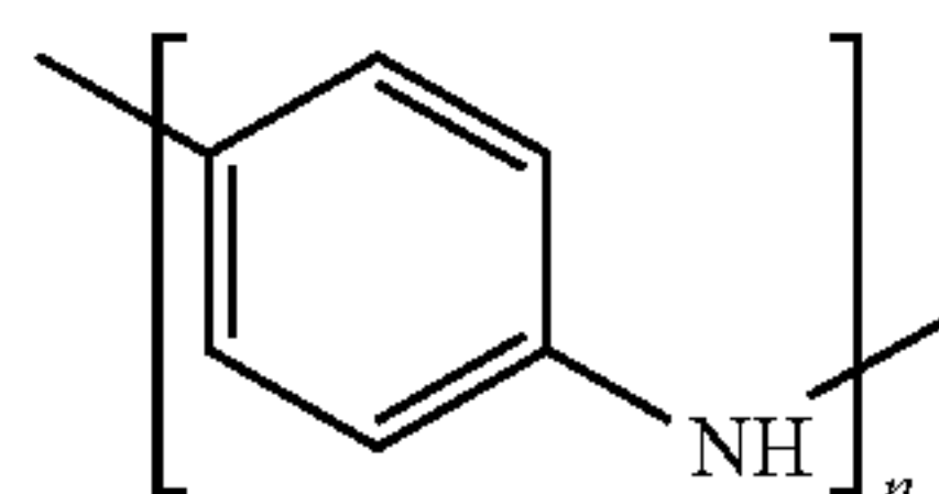
PANI = polyaniline
