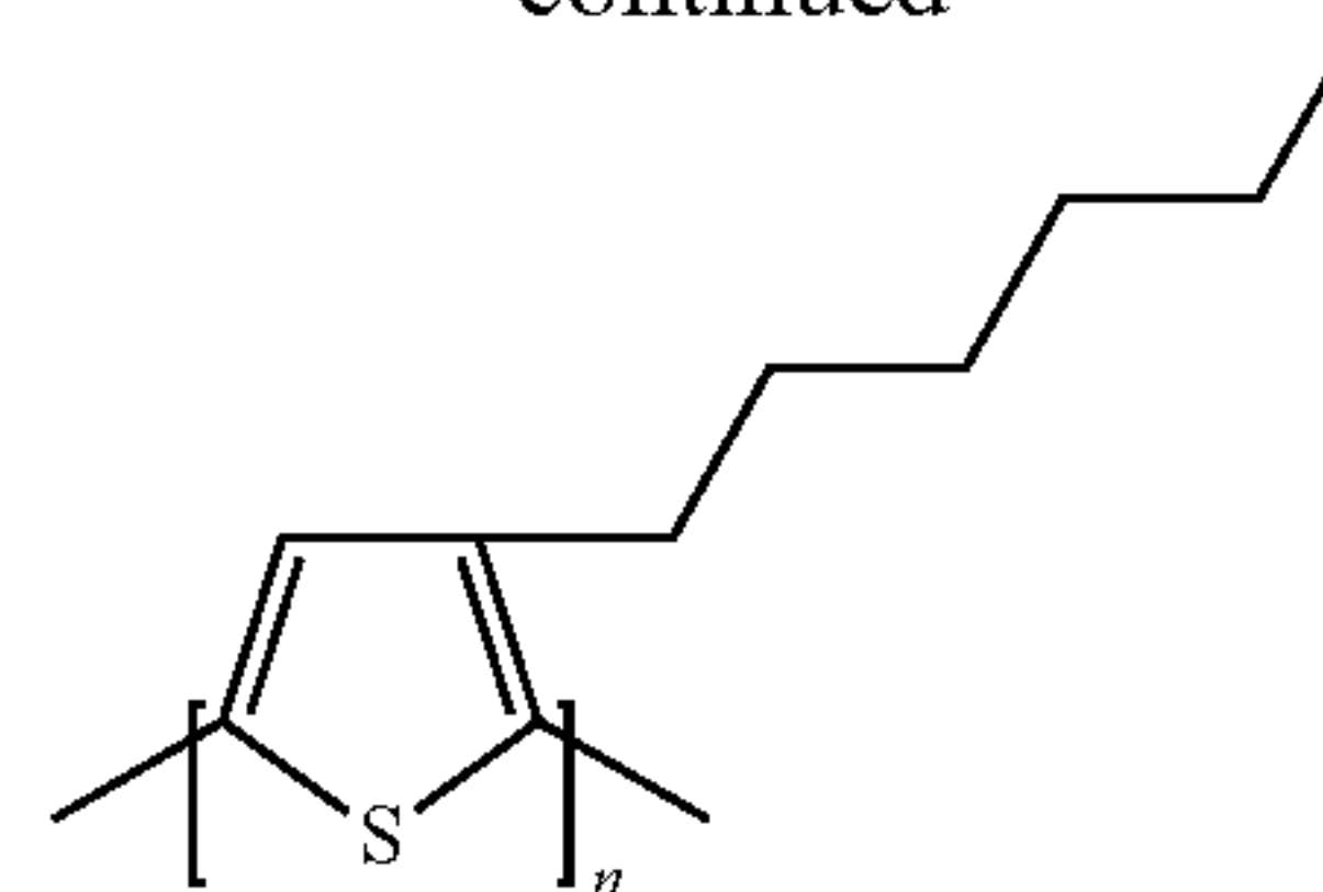
P3HT = poly(3-hexylthiophene)
