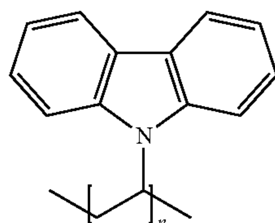
PVK = poly(9-vinylcarbazole)
